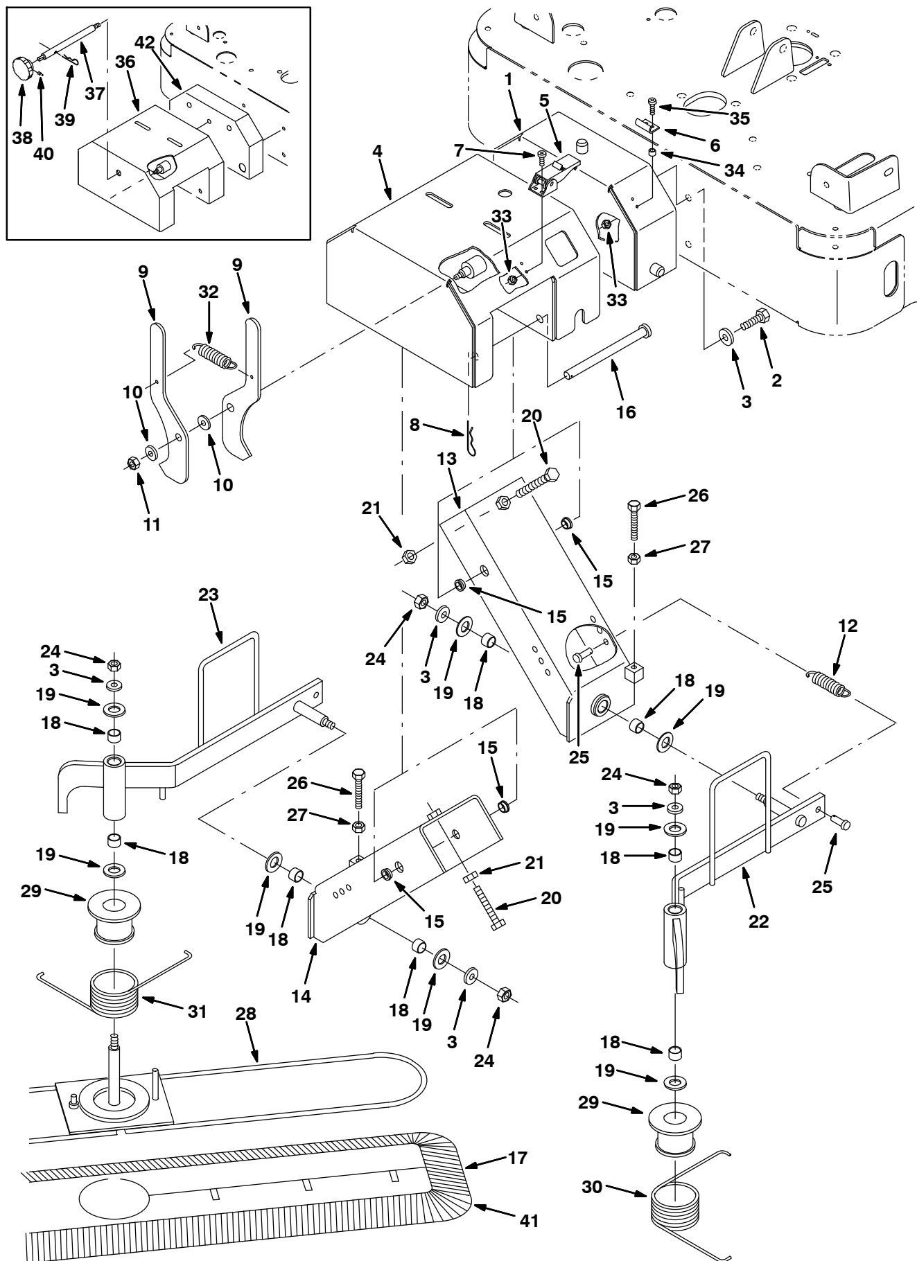
Fig. 1 – Quick Mop Kit (0001–4000) — Quick Mop Satz (0001–4000) — Jeu de pièces Quick Mop (0001–4000)
