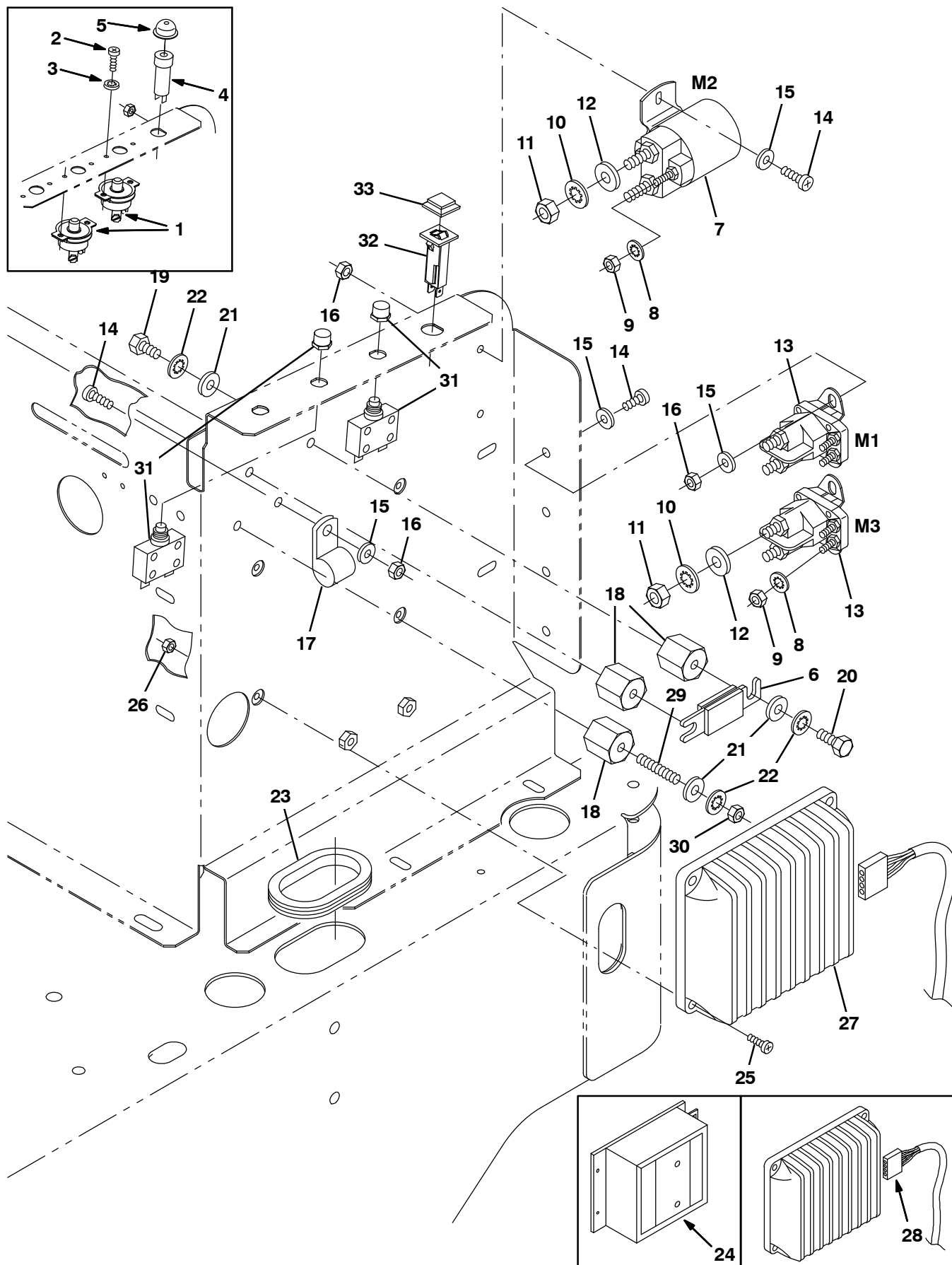
Fig. 7 – Electrical Panel Group (0001–3011) — Elektronik-Schaltfeld-Gruppe (0001–3011) — Assemblage tableau électronique (0001–3011)
