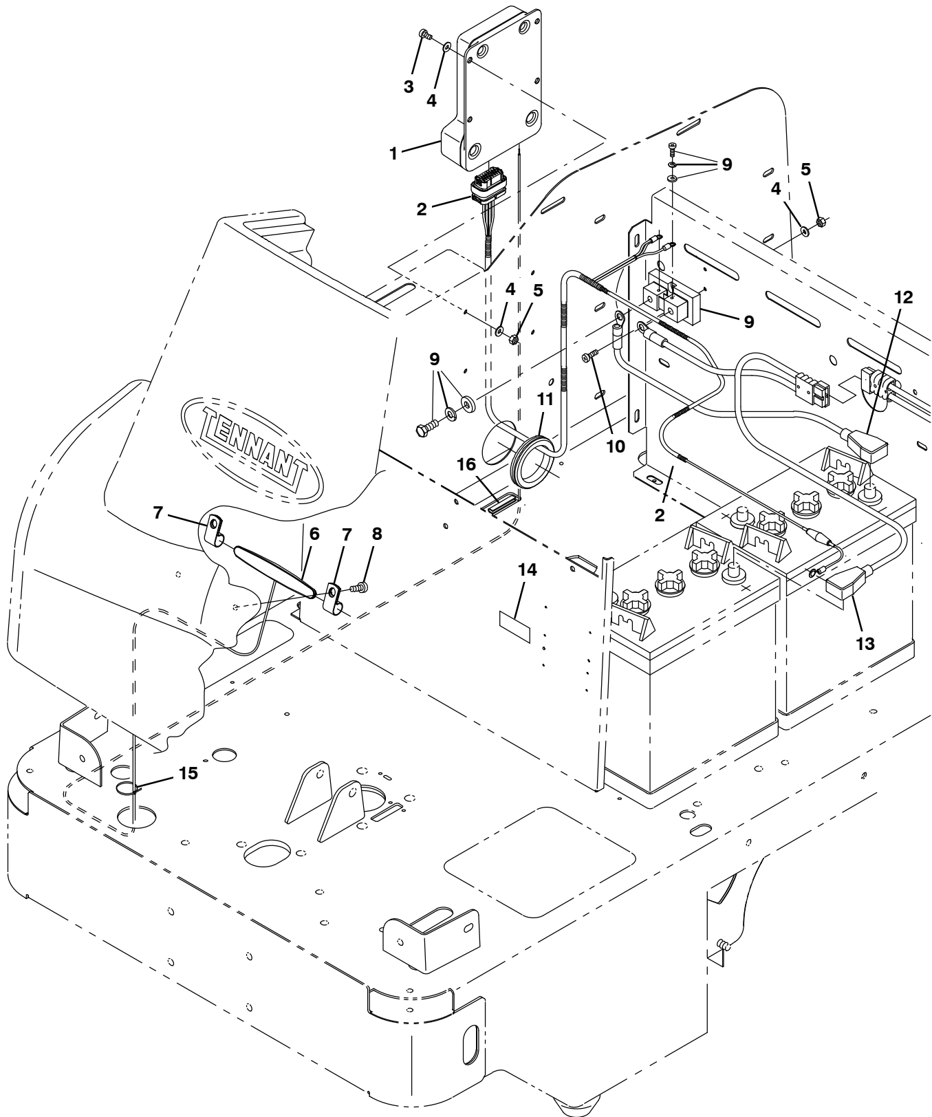
Fig. 27 – Telemetry Group
