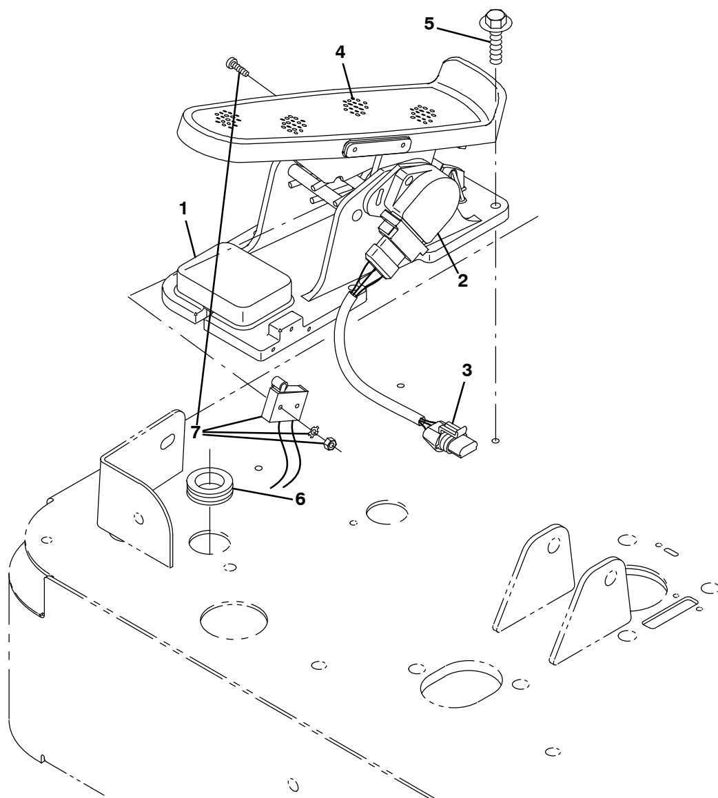
Fig. 16 – Directional Pedal Group (6100 1280– ) — Fahrpedal-Gruppe (6100 1280– ) — Groupe pedale de direction (6100 1280– )
