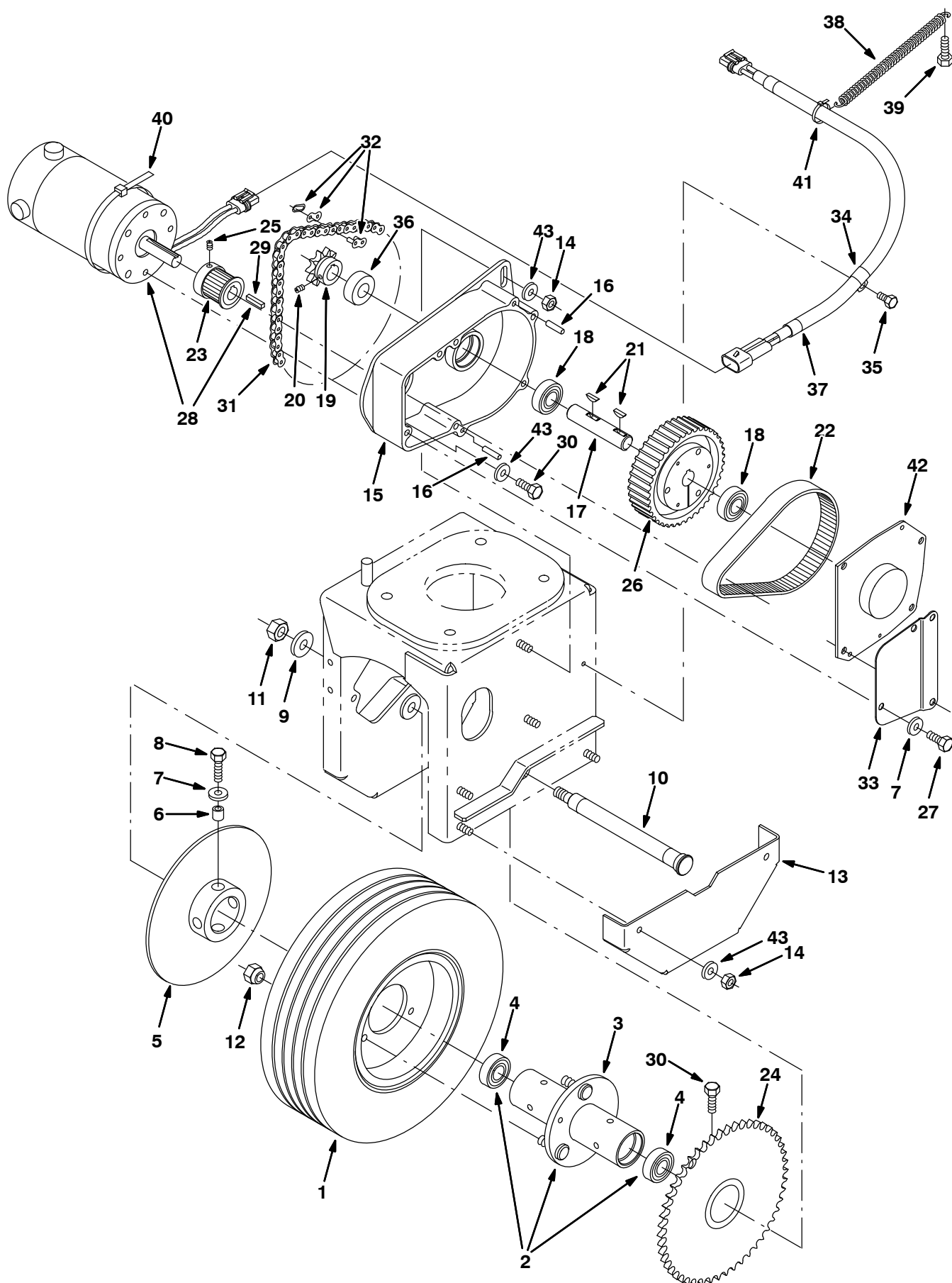
Fig. 10 – Front Drive Wheel Group (6100530 001–728) — Vorderantrieb-Rad-Gruppe (6100530 001–728) — Groupe roues motrices avant (6100530 001–728)
