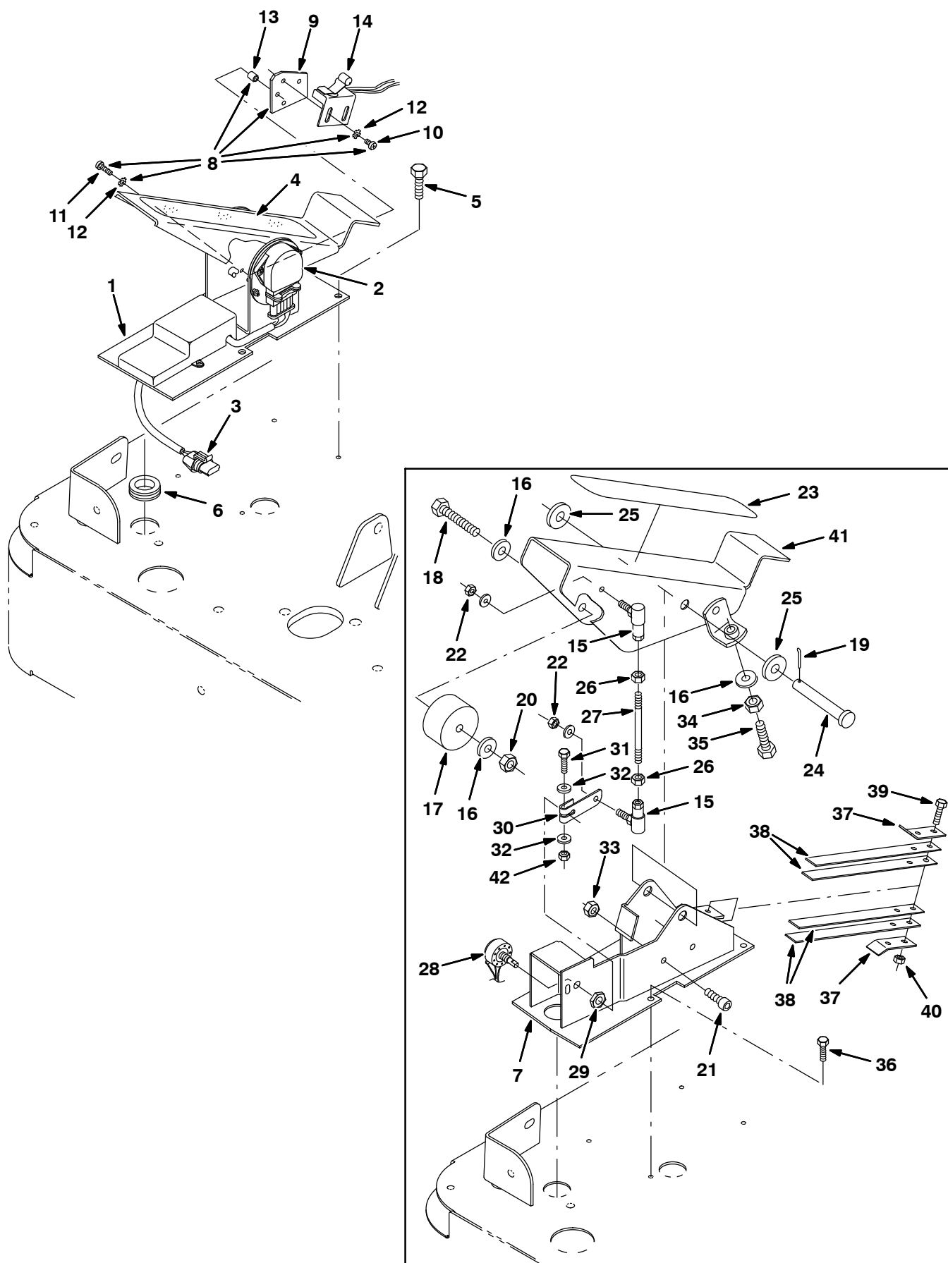
Fig. 15 – Directional Pedal Group (6100 001–1279) — Fahrpedal-Gruppe (6100 001–1279) — Groupe pedale de direction (6100 001–1279)
