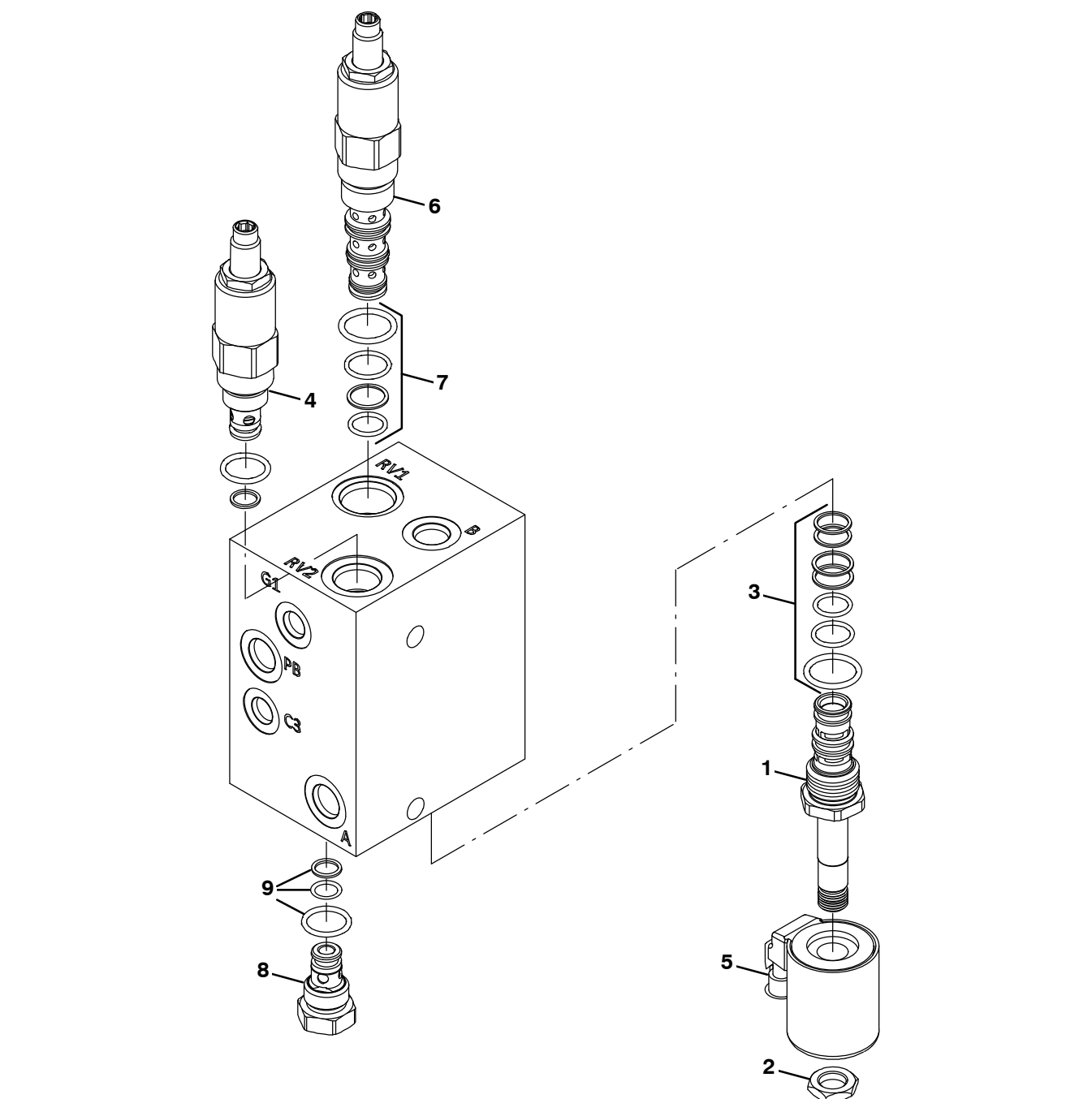
Fig. 8 – Hydraulic Solenoid Valve Breakdown, 1237088
