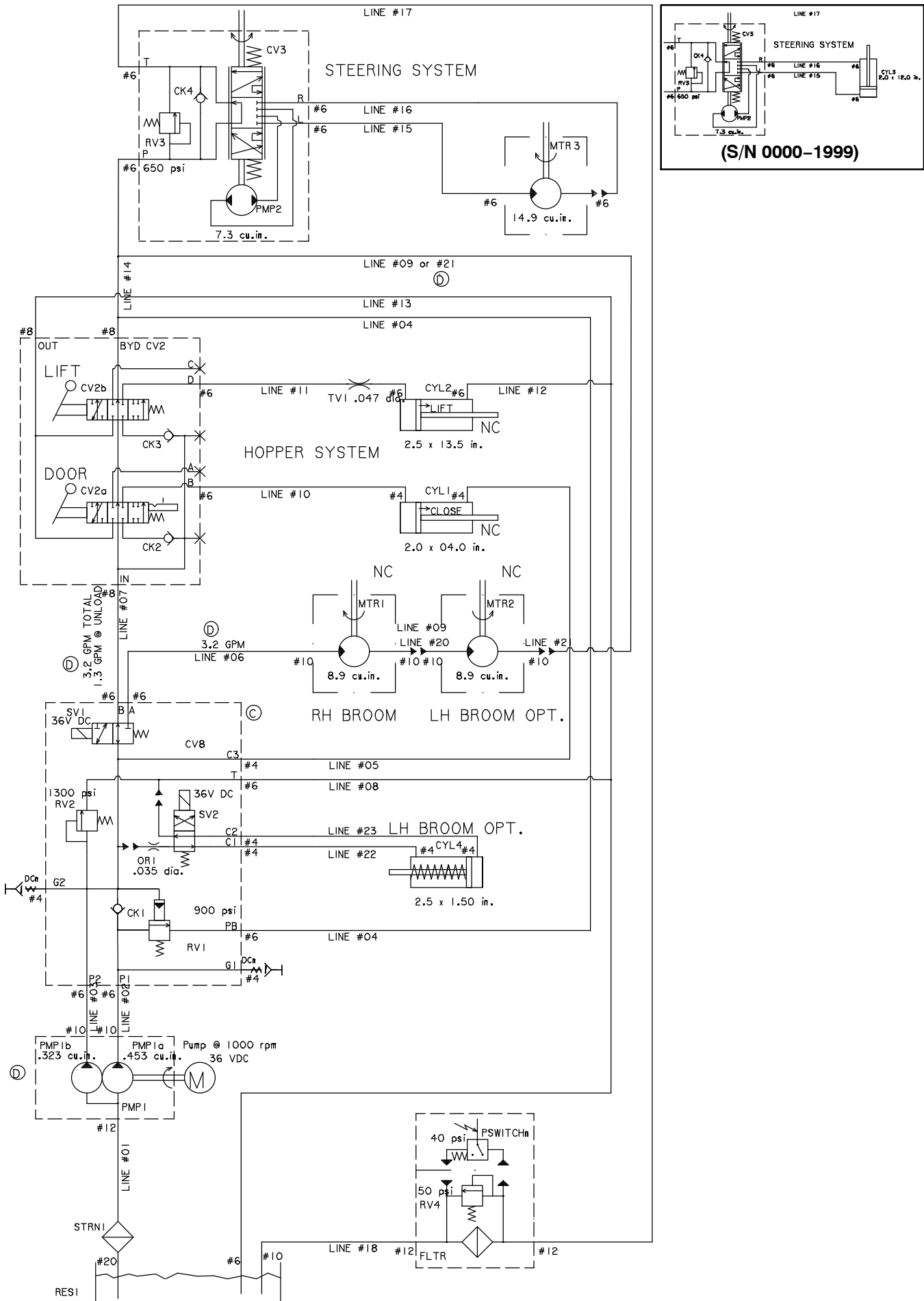
Fig. 31 – Hydraulic Schematic
