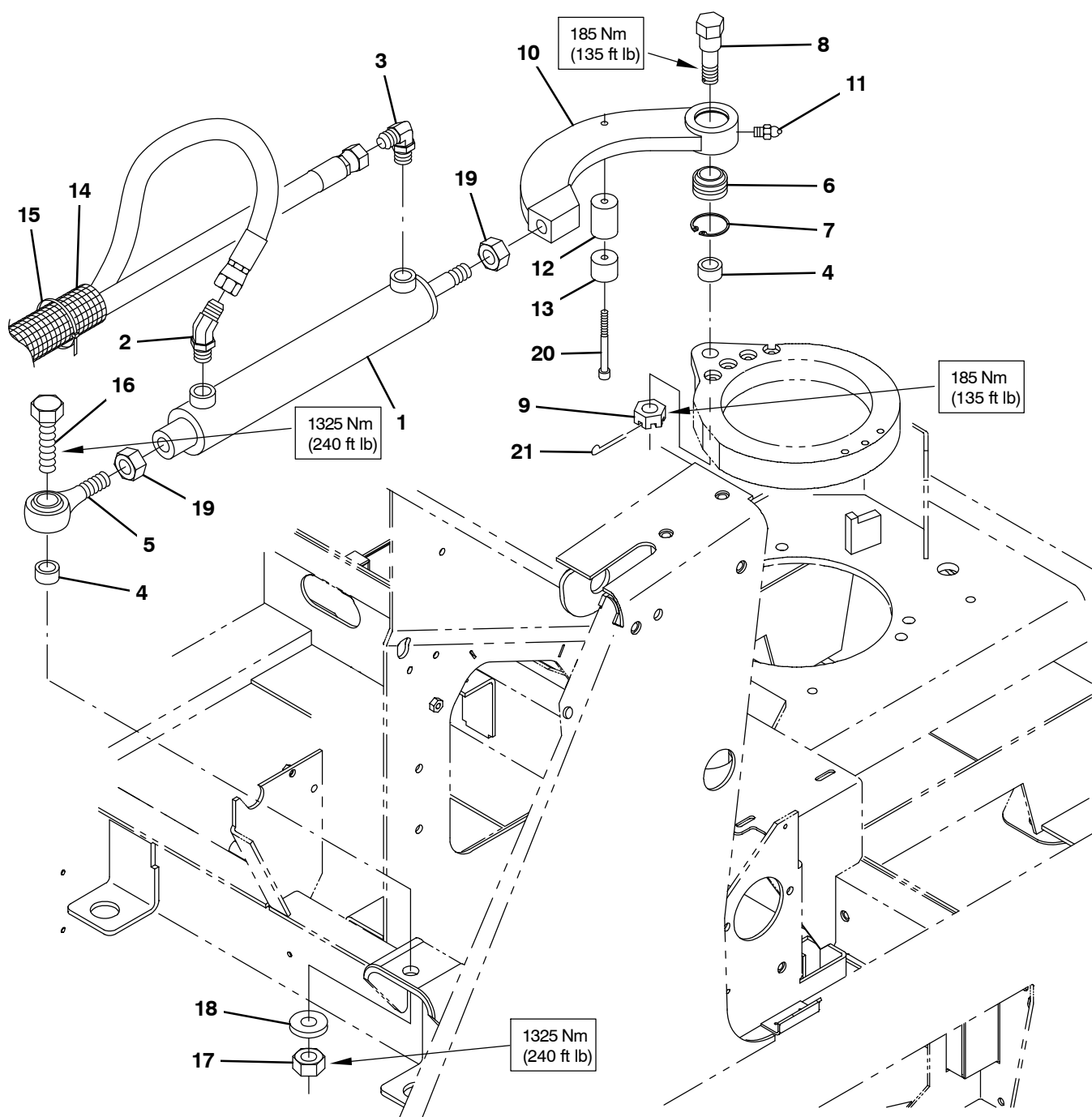
Fig. 13 – Steering Cylinder Group (0000–1999)
