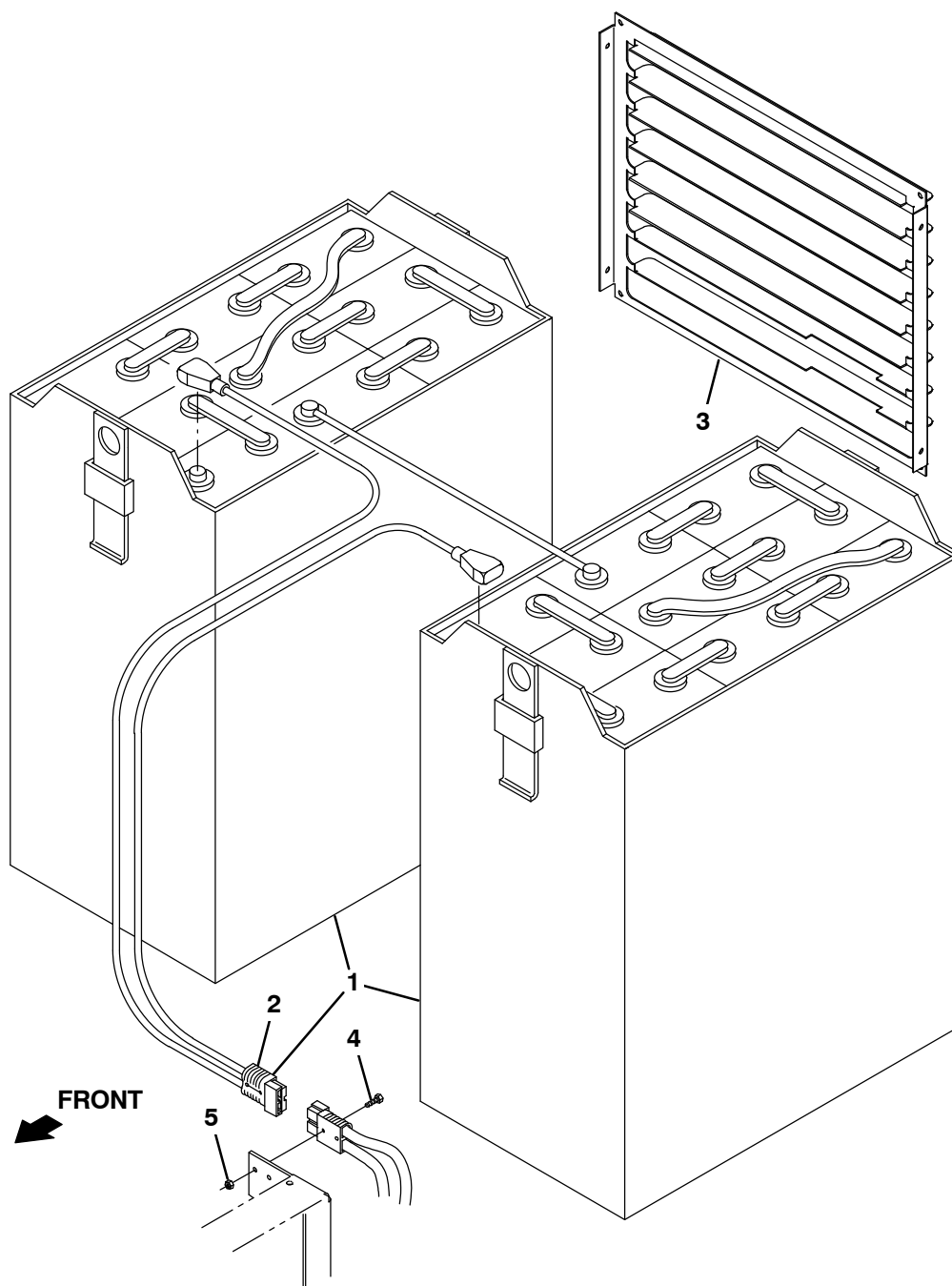
Fig. 18 – Battery Group, 36VDC 340 AH
