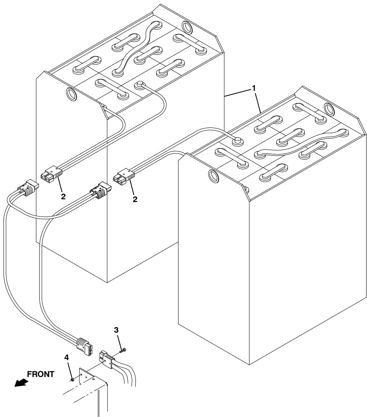
Fig. 20 – Battery Group 36V 425Ah
