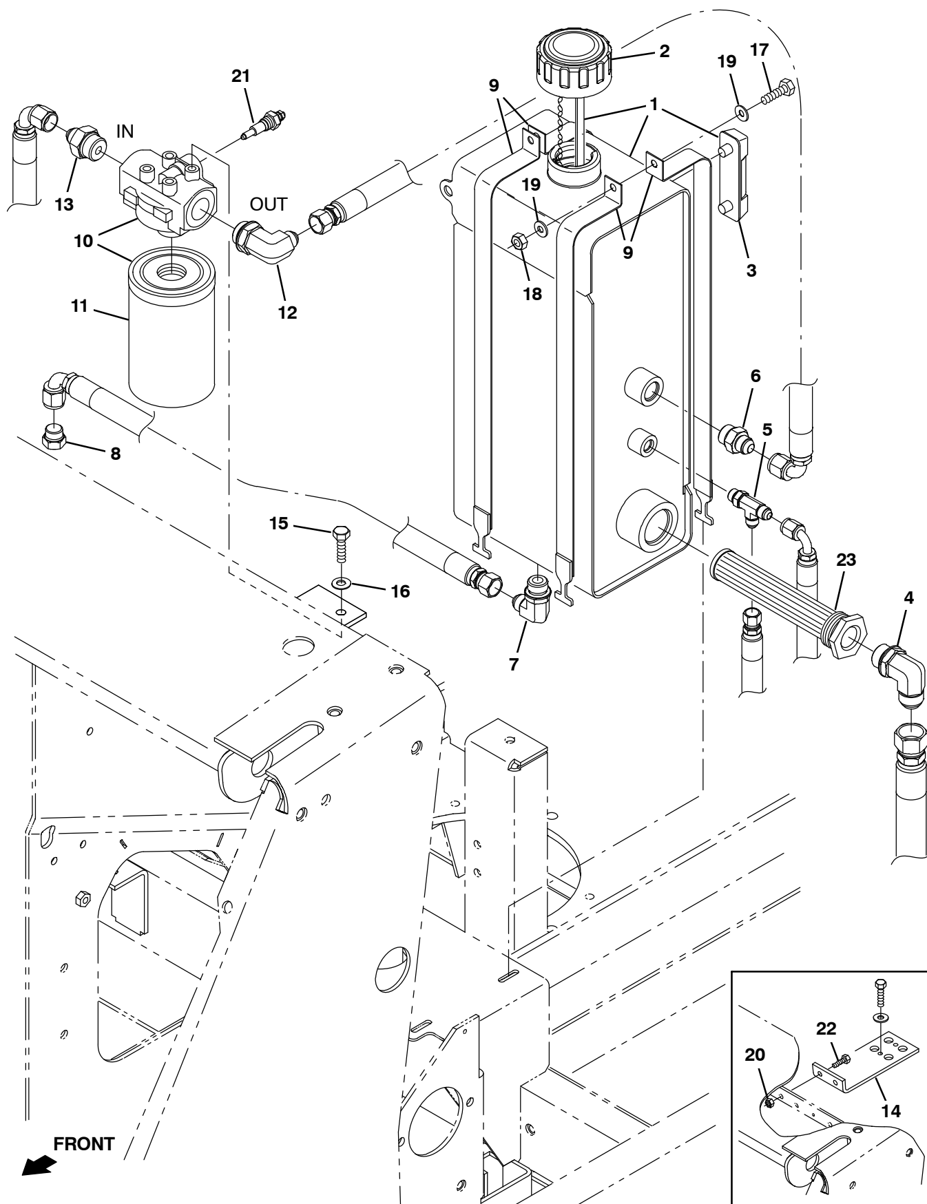
Fig. 33 – Hydraulic Reservoir Group
