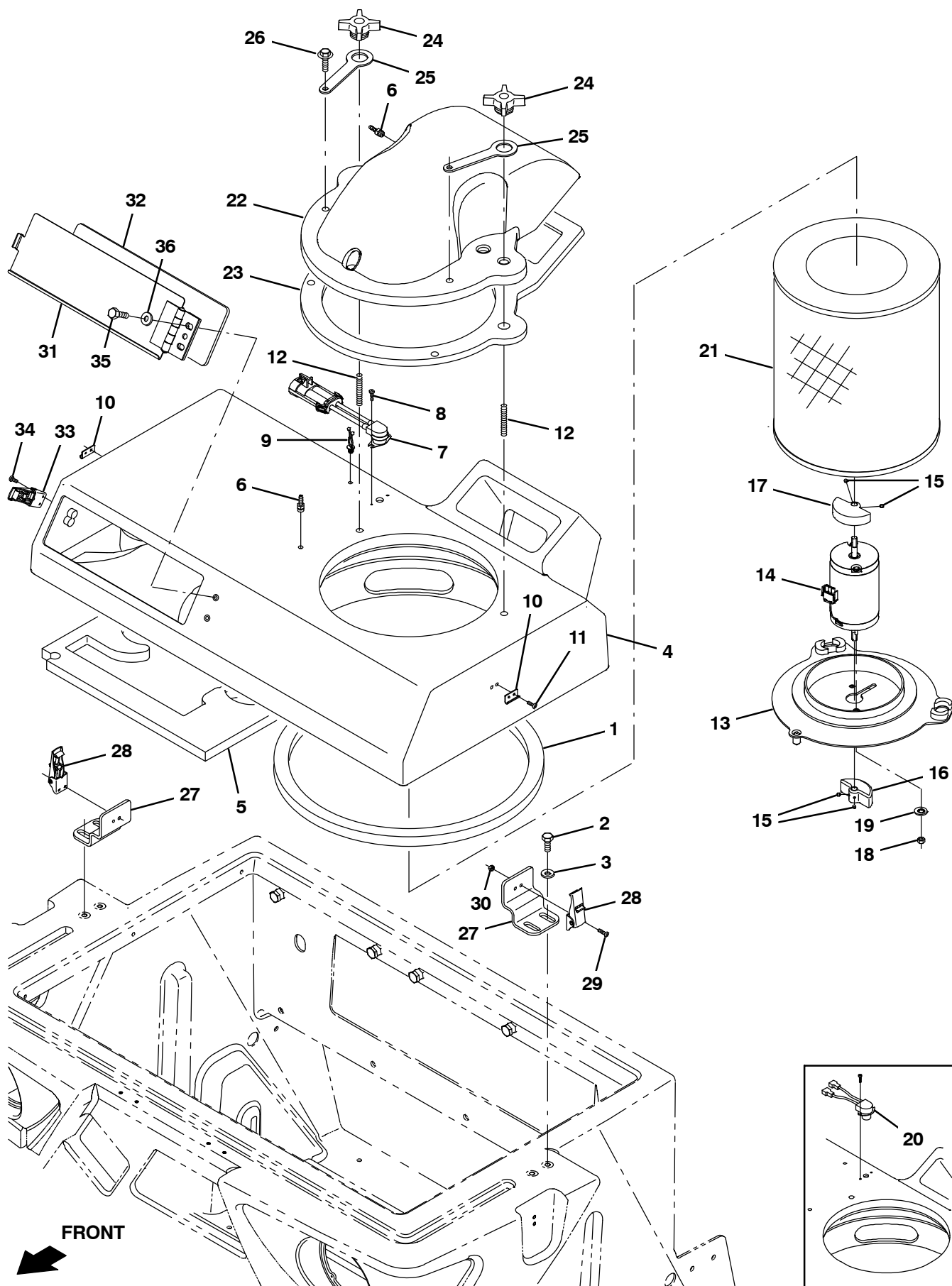
Fig. 30 – Hopper Filter Shaker Cover Group
