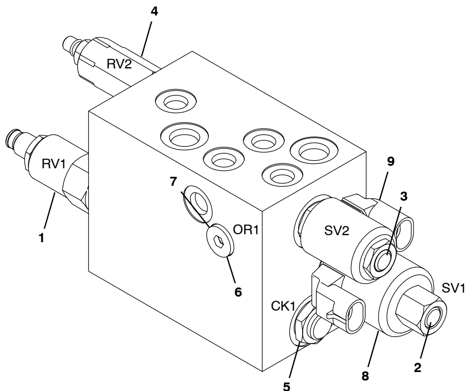
Fig. 7 – Hydraulic Solenoid Valve Breakdown, 1045994
