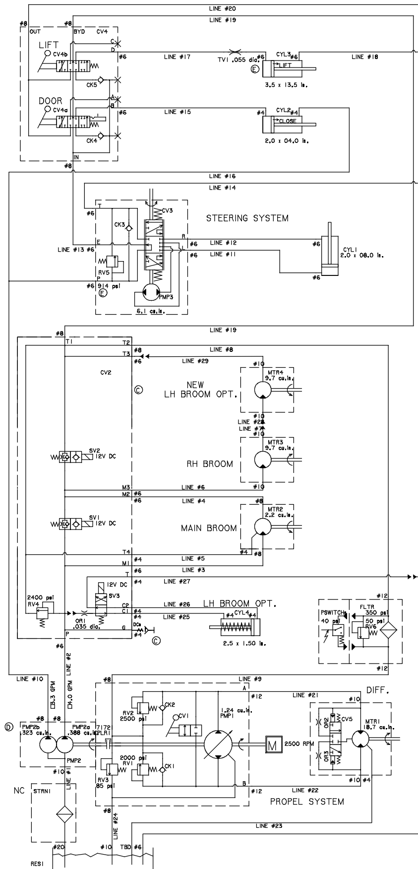
Fig. 37 - Hydraulic Schematic
