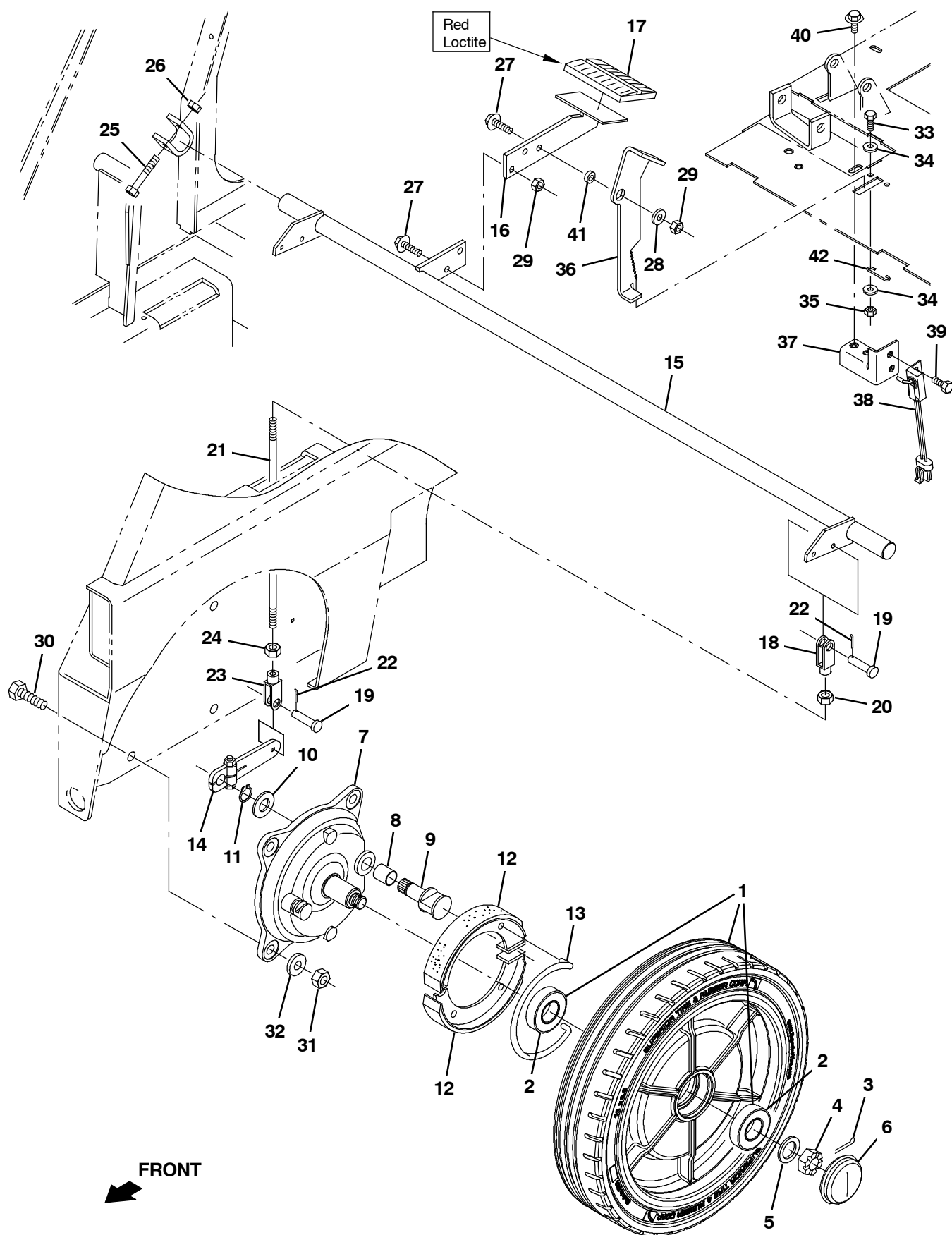
Fig. 19 - Wheel and Brake Group, Front
