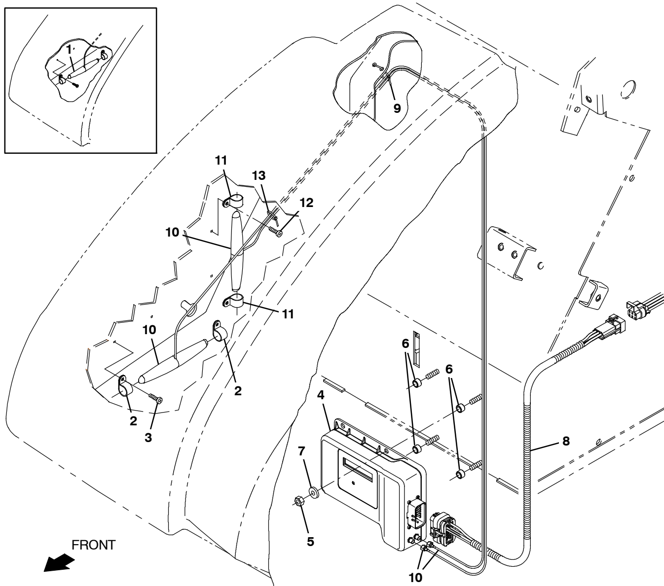
Fig. 21 - Telemetry Group
