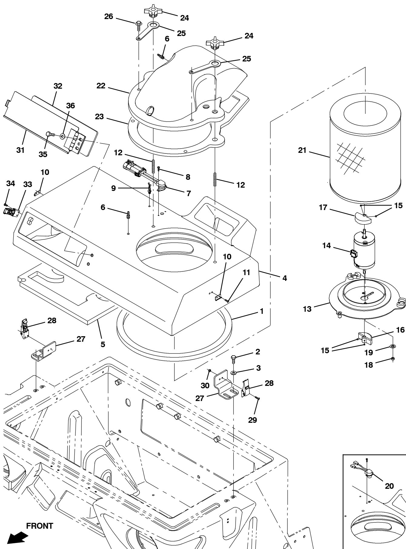
Fig. 35 - Hopper Filter Shaker Group
