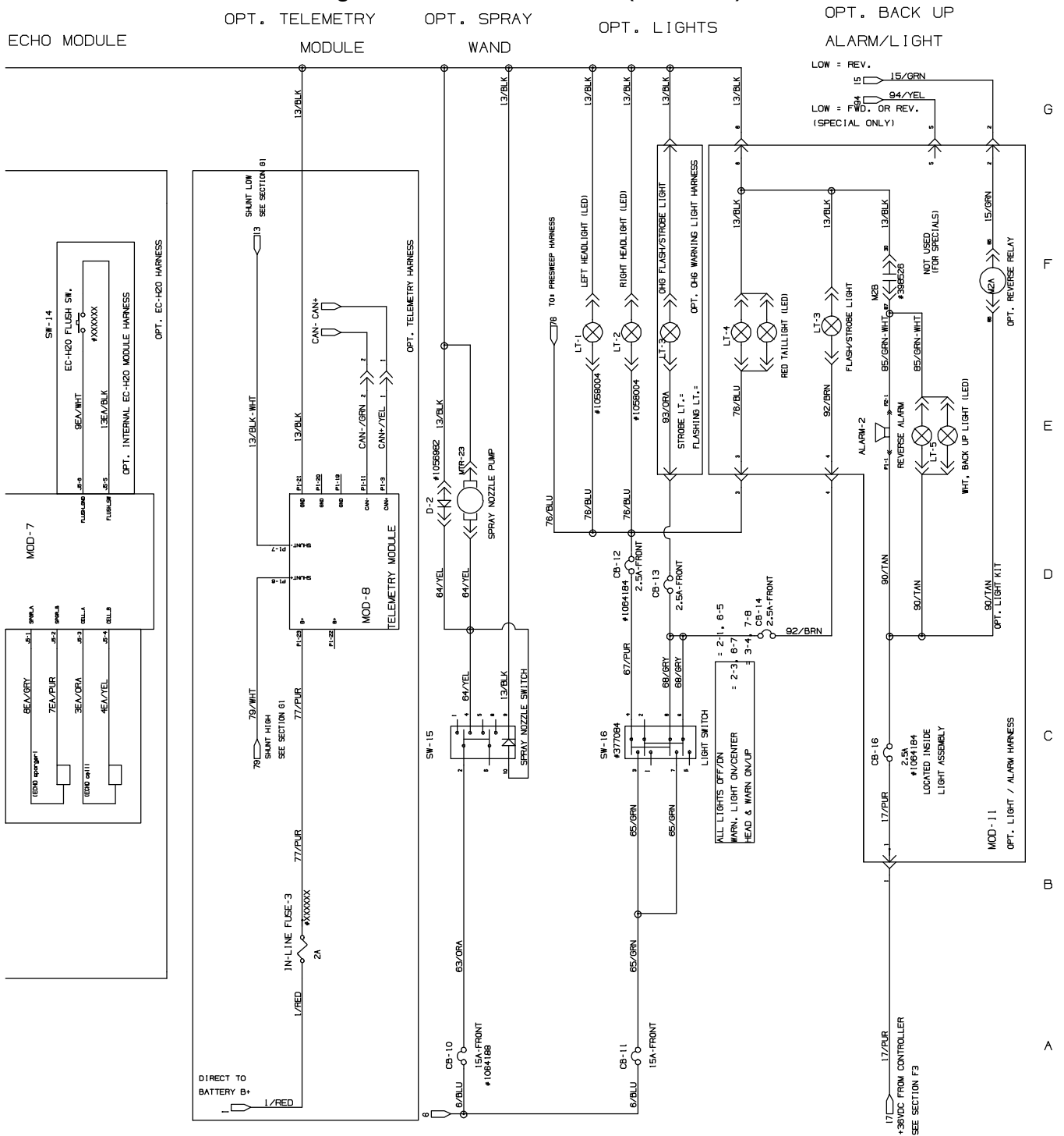
Fig. 35 – Electrical Schematic (0400-1199)
