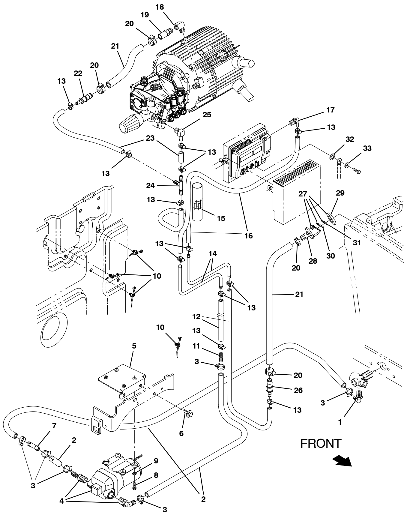
Fig. 51 – Pressure Washer Solution Supply Group (1200– )
