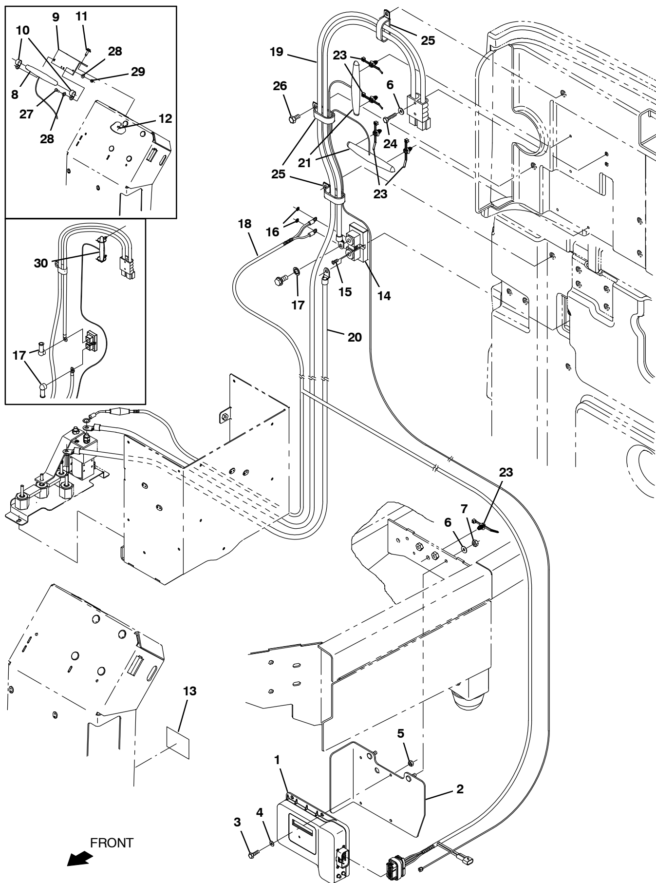
Fig. 40 – Telemetry Group
