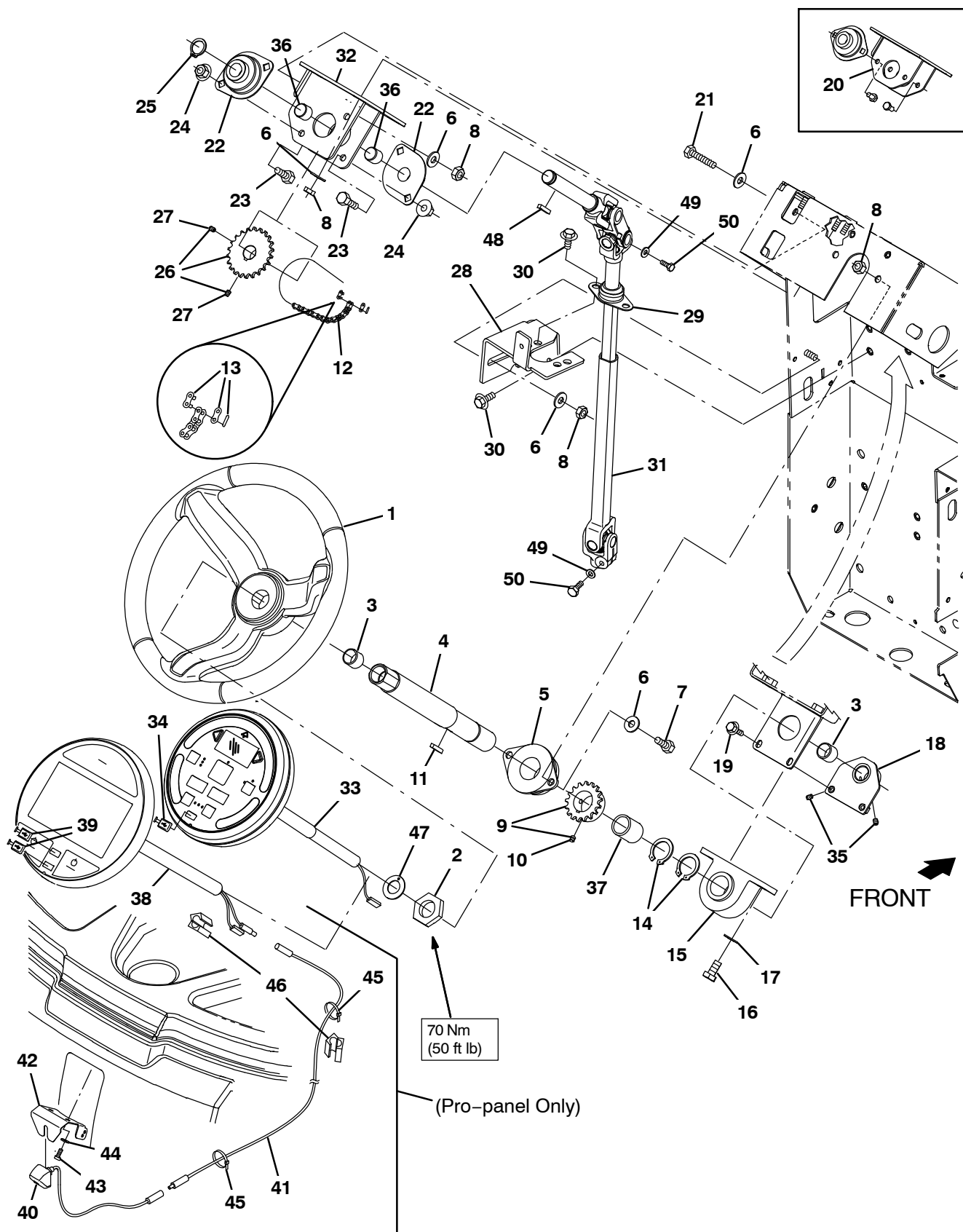
Fig. 5 – Steering Group
