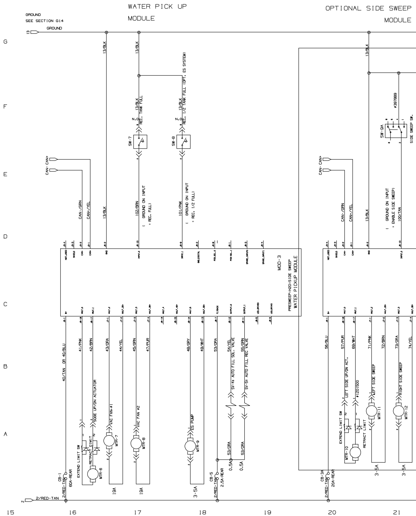
Fig. 34 – Electrical Schematic (0000–0399)
