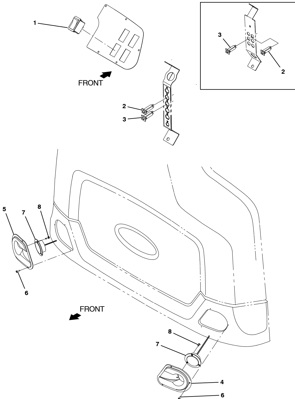
Fig. 1 – Headlight Group
