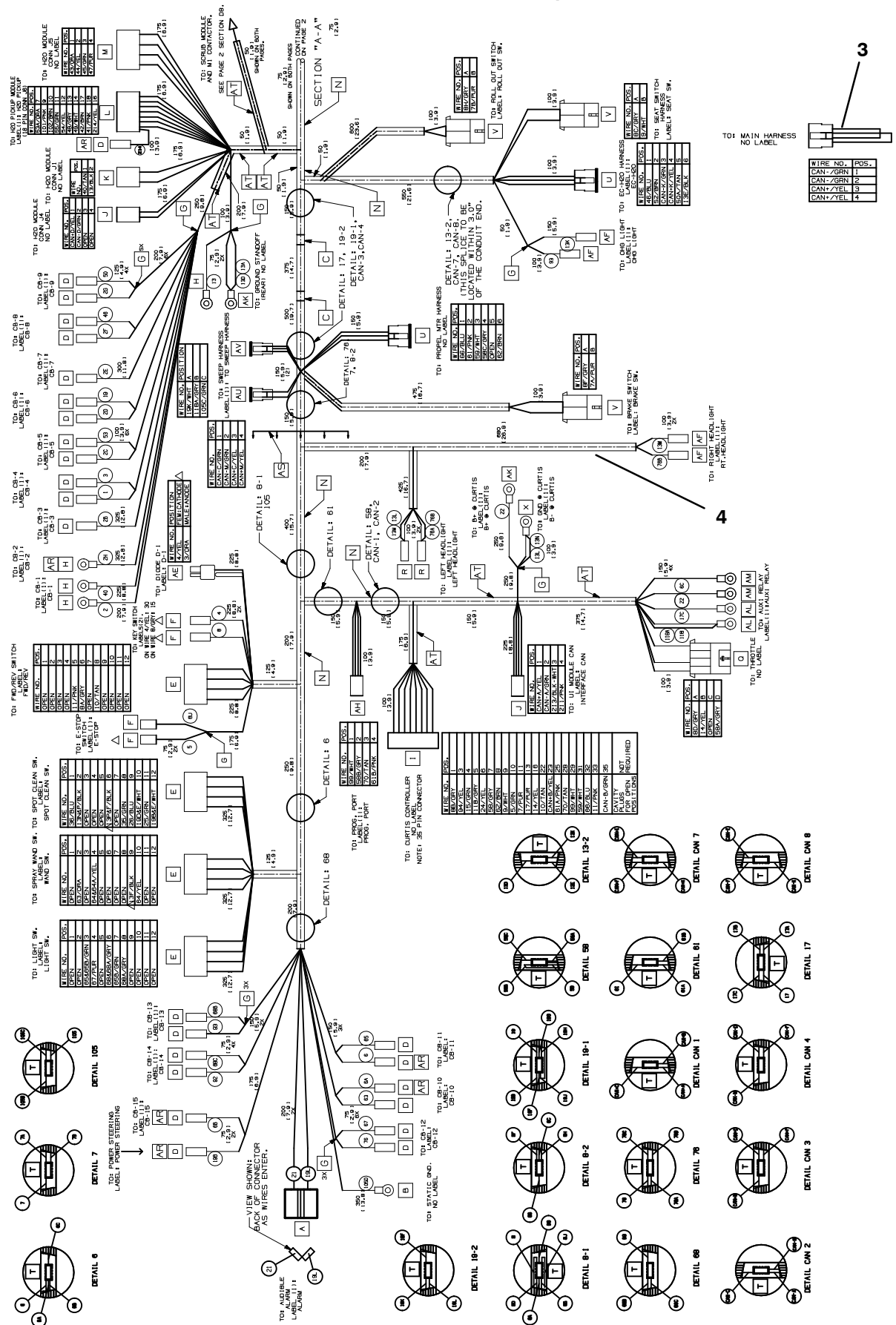
Fig. 38 - Wire Harnesses Group
