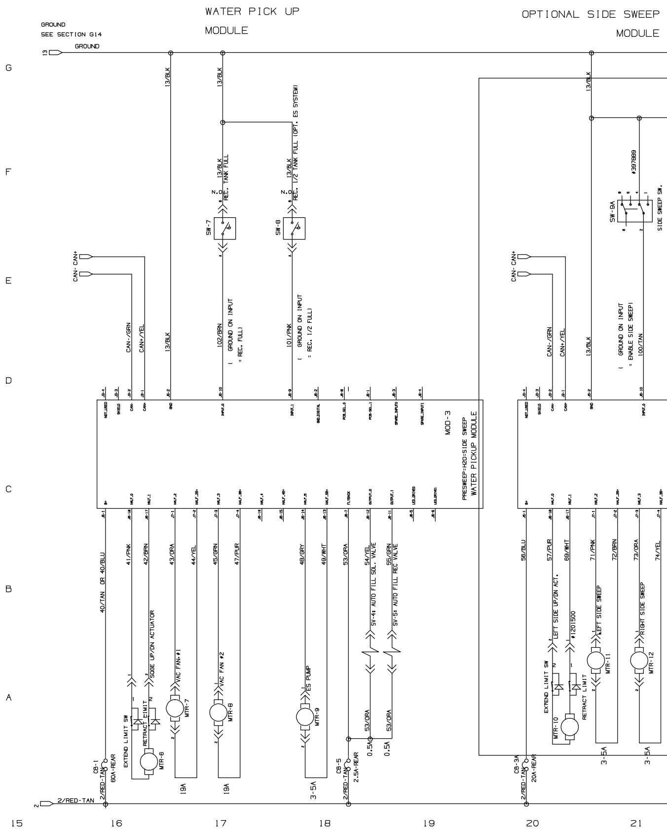
Fig. 35 – Electrical Schematic (0400-1199)
