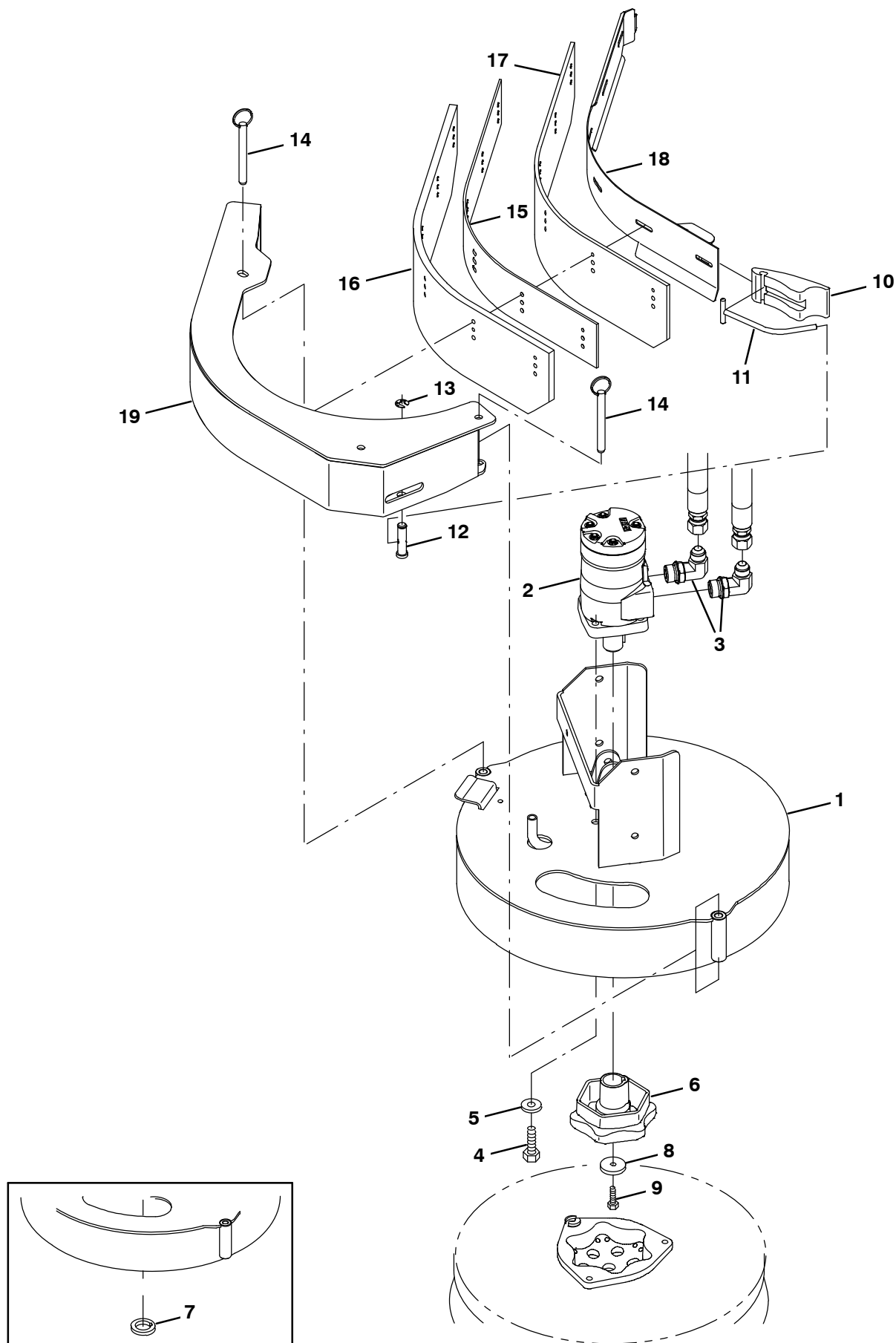
Fig. 4 – Side Brush Motor Group (0181– )
