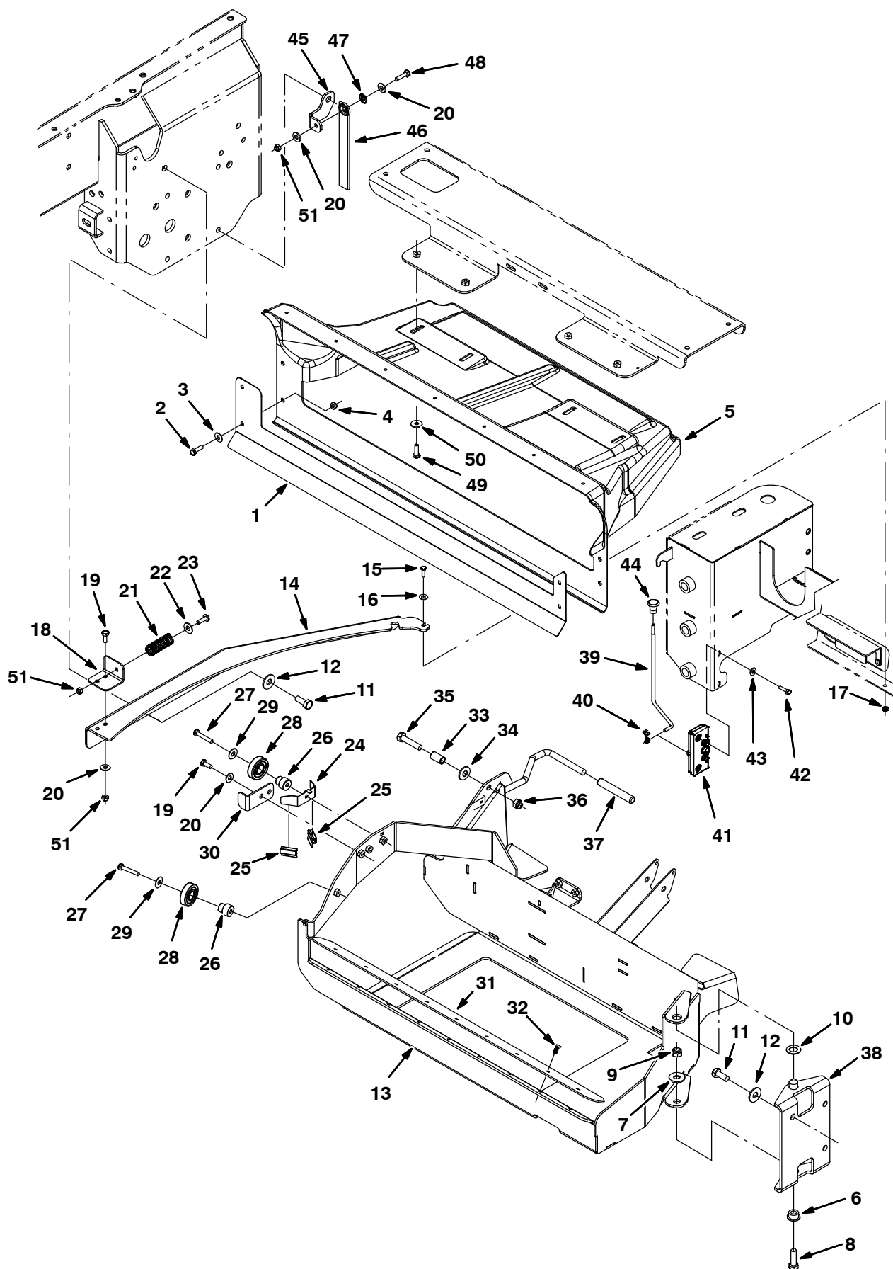
Fig. 34 – Cylindrical Scrub Head Debris Tray Mount Group
