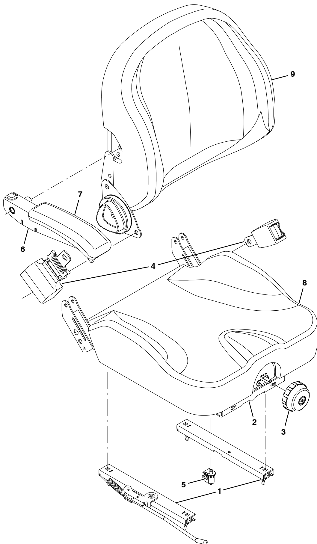
Fig. 17 – Seat Breakdown, 1072456
