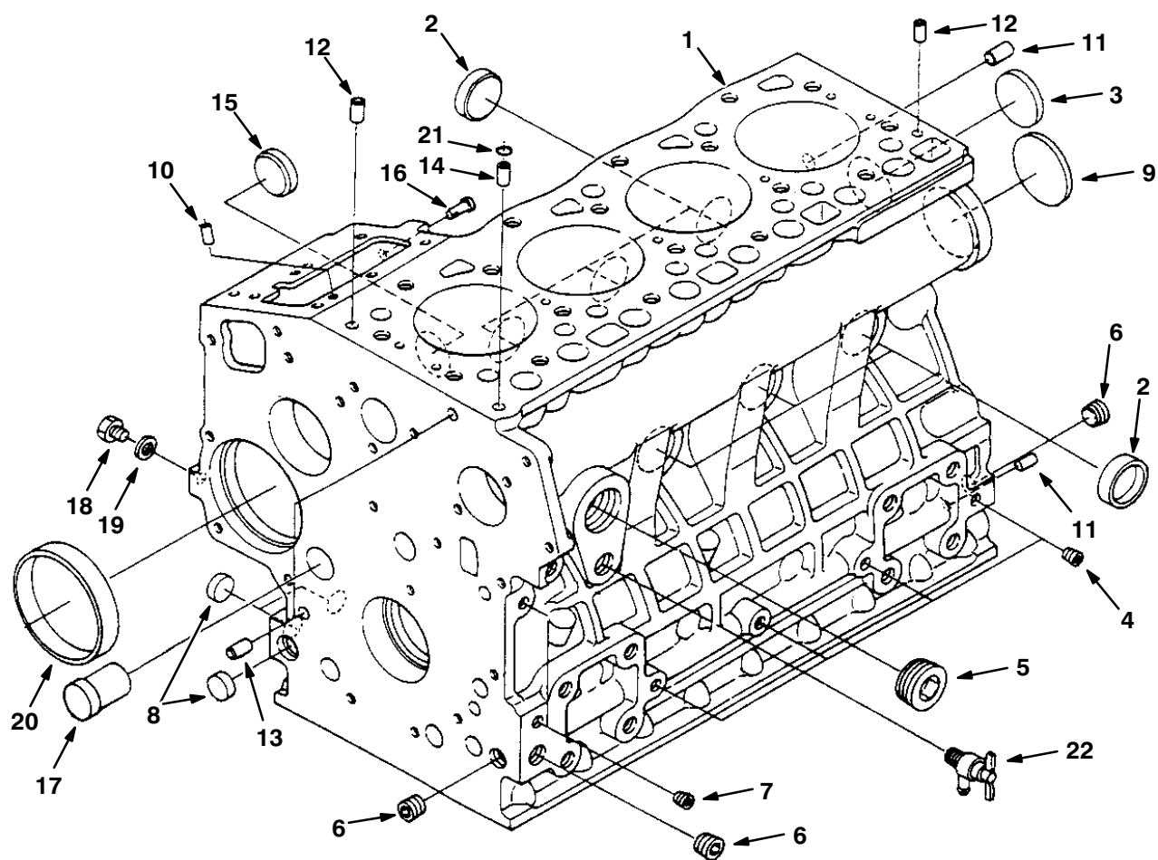
Fig. 1 - Crankcase Group
