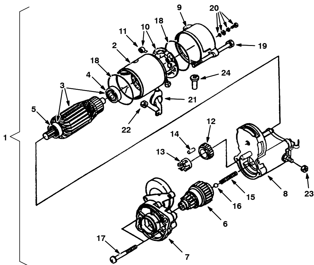
Fig. 14 – Starter Breakdown, 74405
