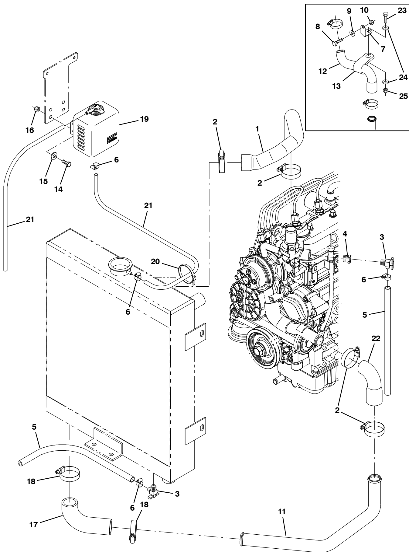
Fig. 21 – Engine Radiator Hose Group, Diesel (0189– )
