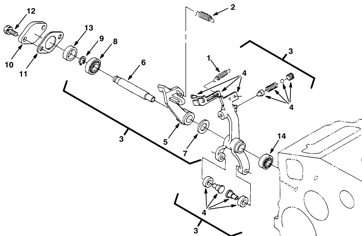
Fig. 20 – Governor Group
