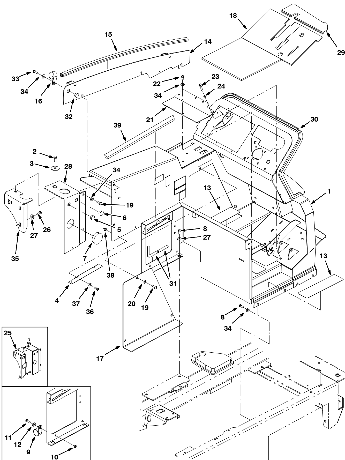
Fig. 4 – Operator Station
