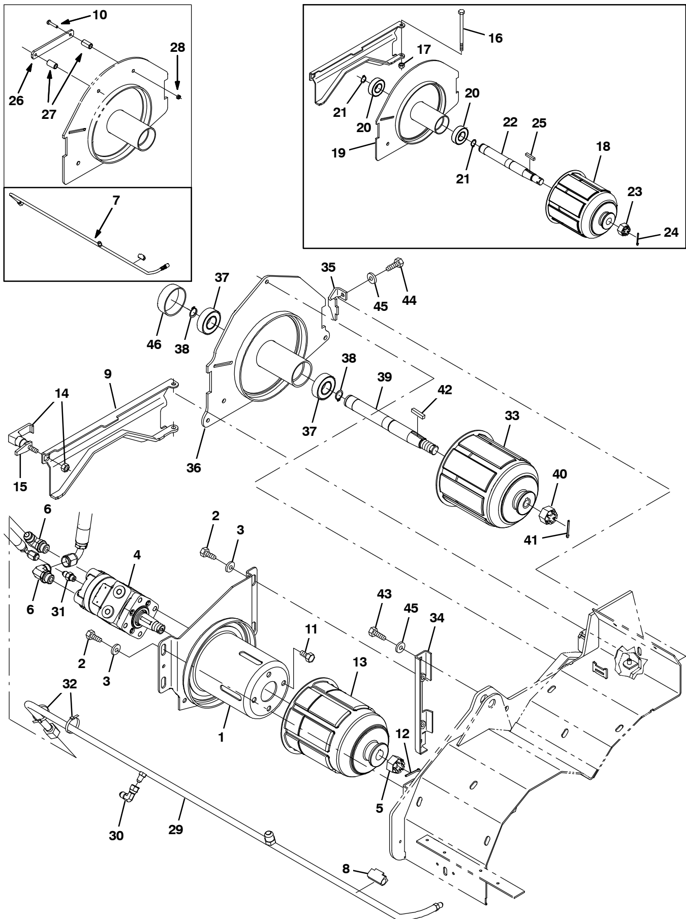
Fig. 28 – Cylindrical Scrub Brush Drive Group, Right Side
