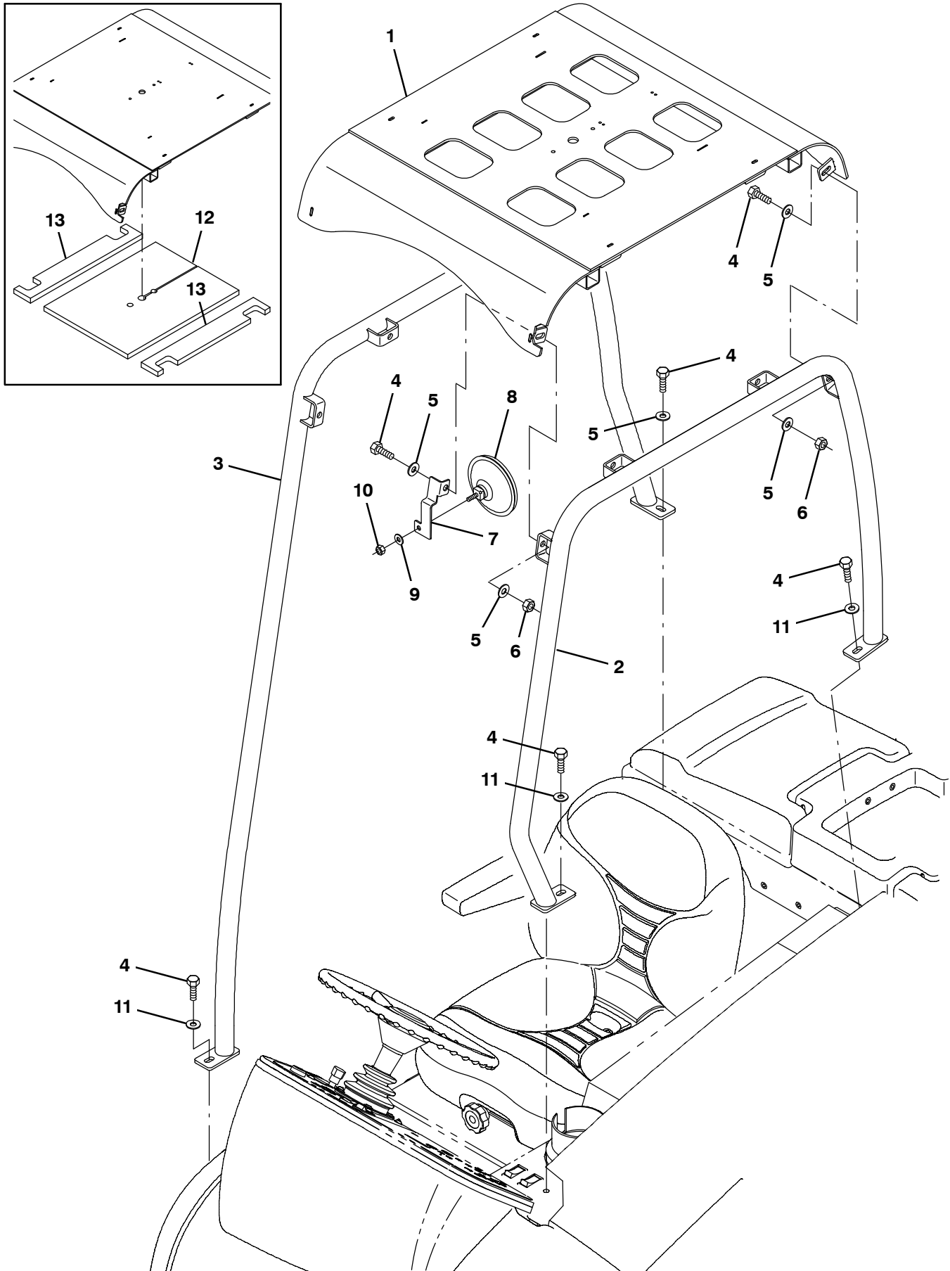
Fig. 31 – Overhead Guard Kit
