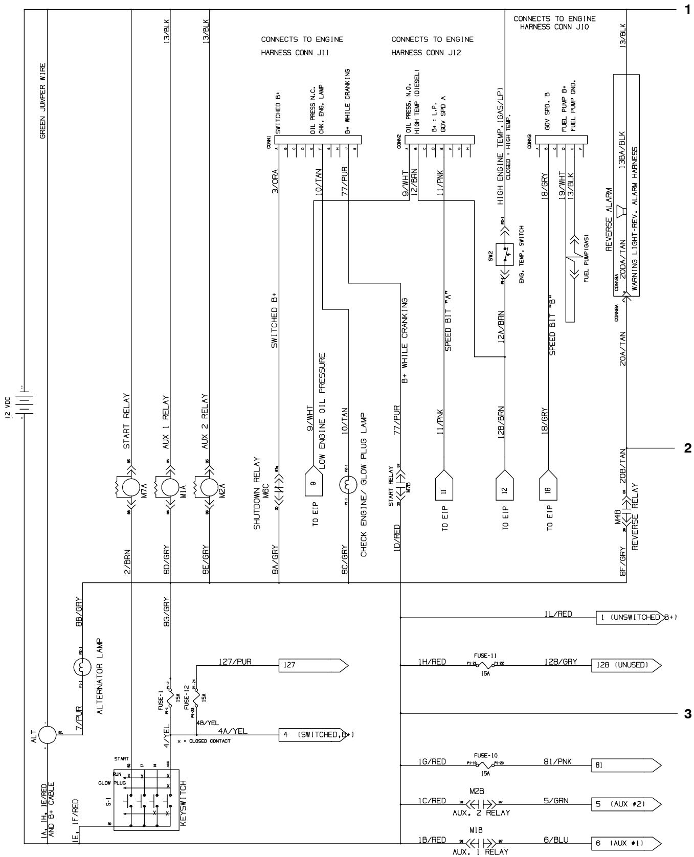
Fig. 62 – Electrical Schematic
