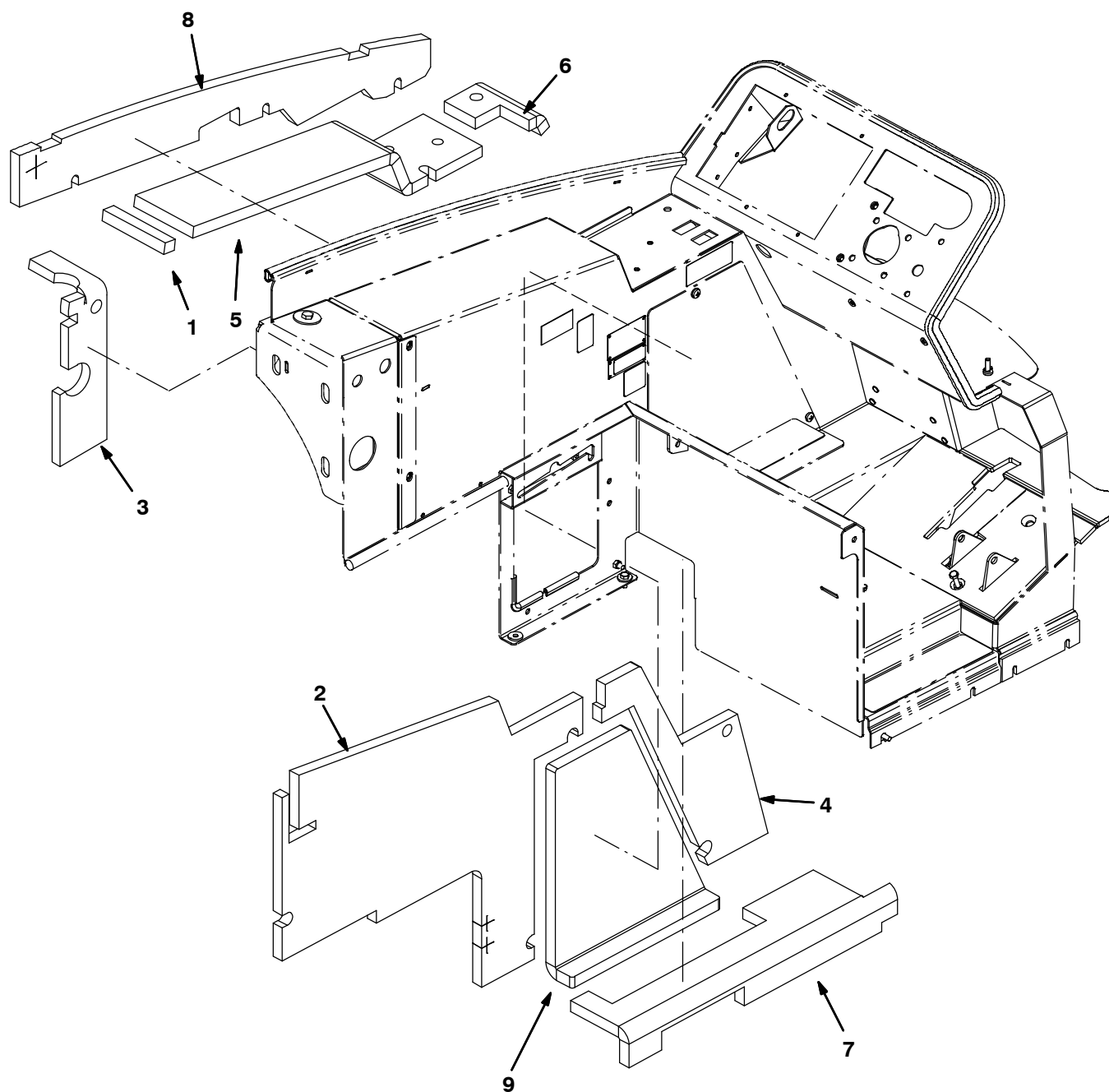
Fig. 5 – Operator Station Insulation Group
