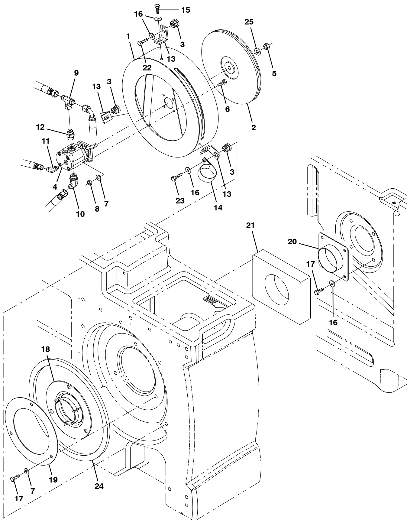
Fig. 49 – Vacuum Fan Group, Scrubbing (0779– )
