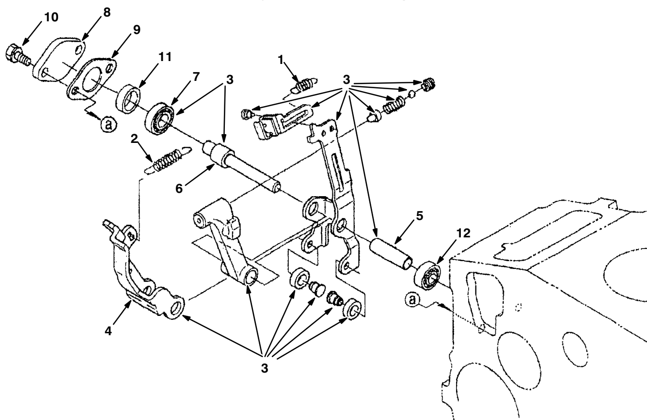
Fig. 21 – Governor Group
