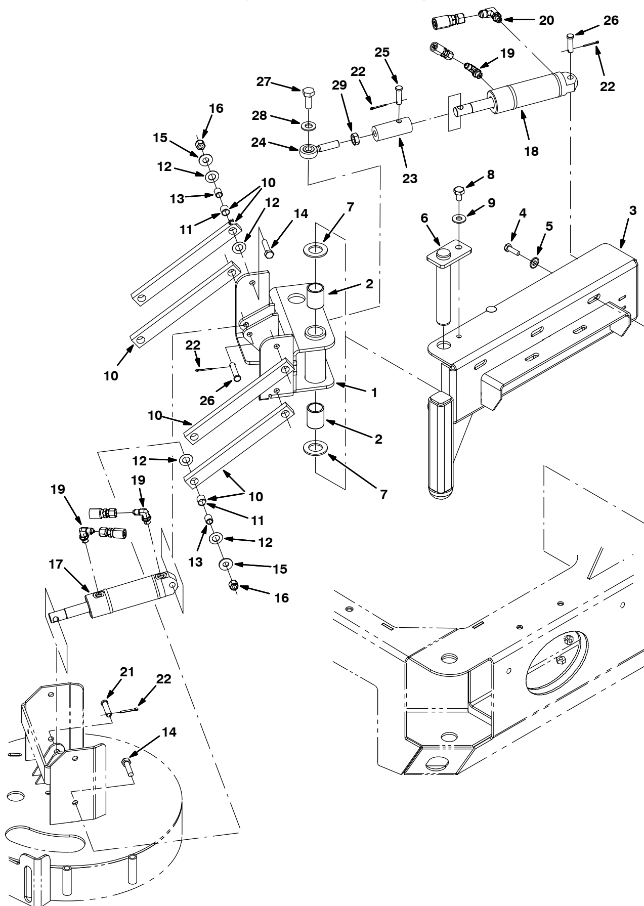
Fig. 5 – Side Brush Lift Group
