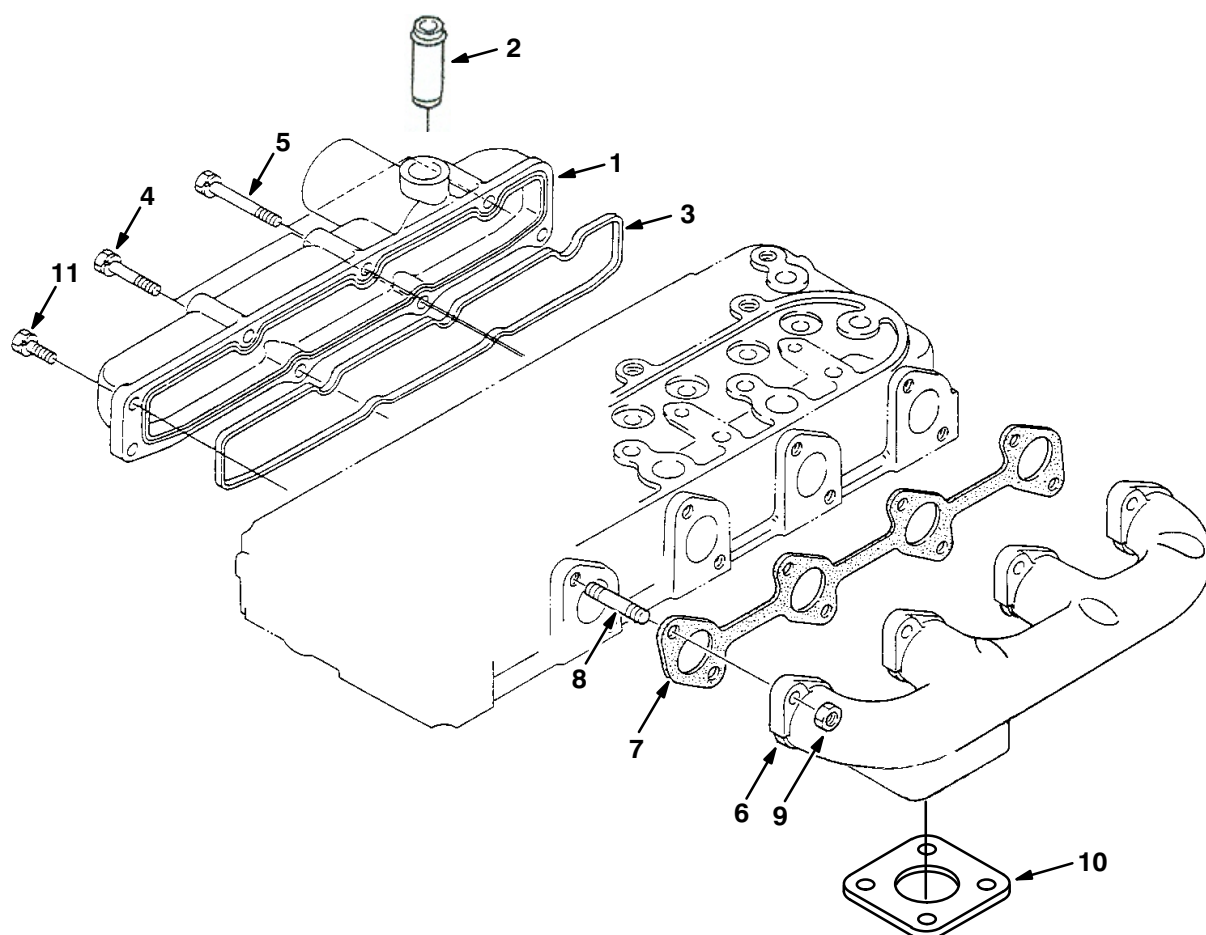
Fig. 8 – Manifold Group
