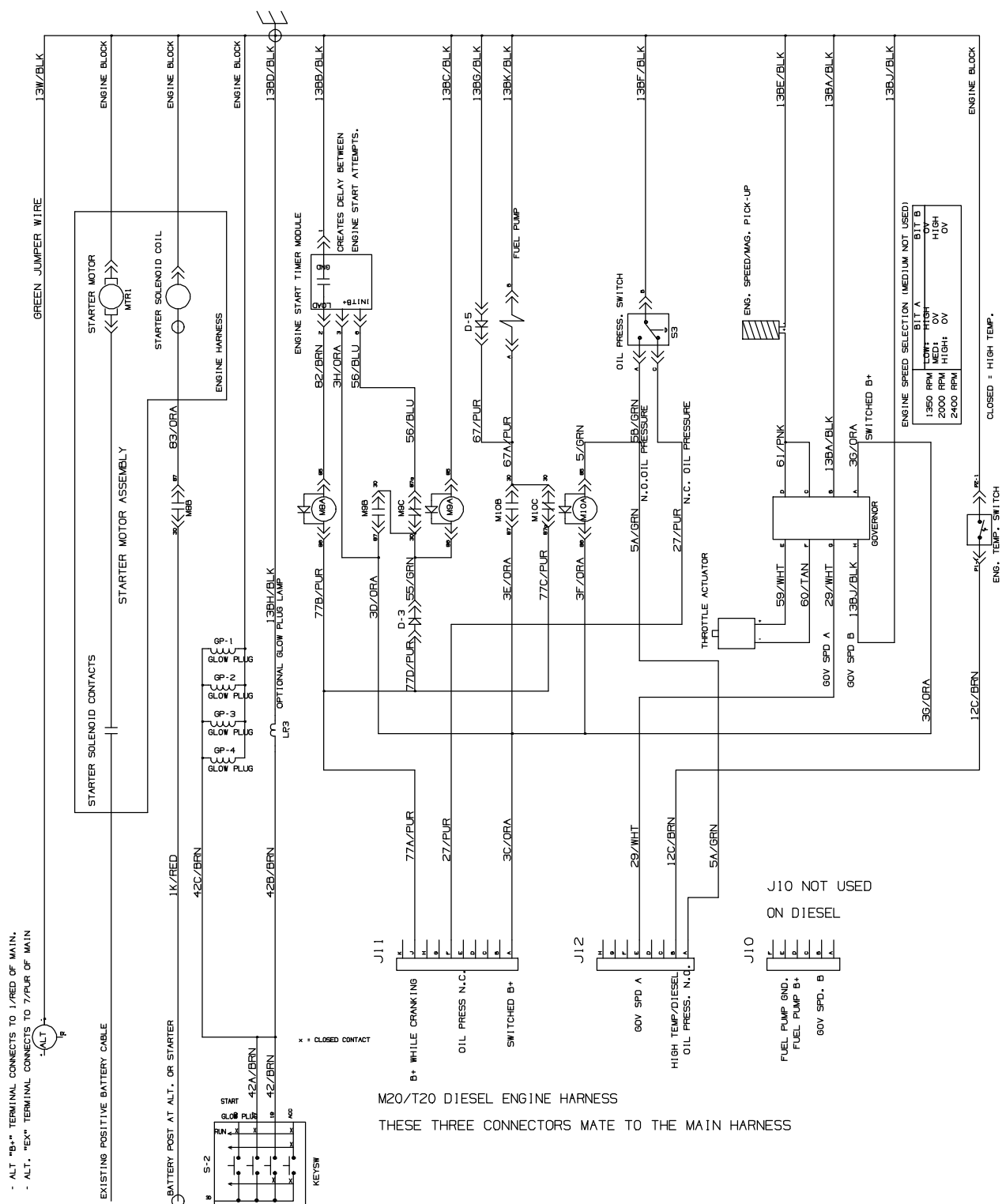
Fig. 63 – Electrical Schematic, Diesel Engine Harness
