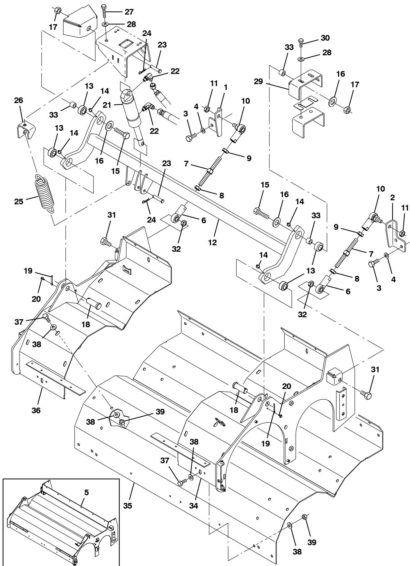
Fig. 29 – Cylindrical Scrub Brush Head Lift Group
