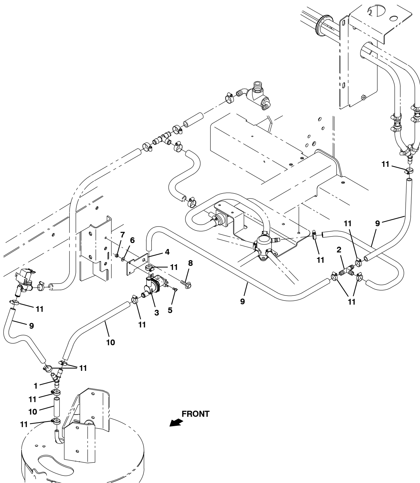
Fig. 20 – FaST Solution Supply Group with Side Brush, Disk Scrub Head (0130- )
