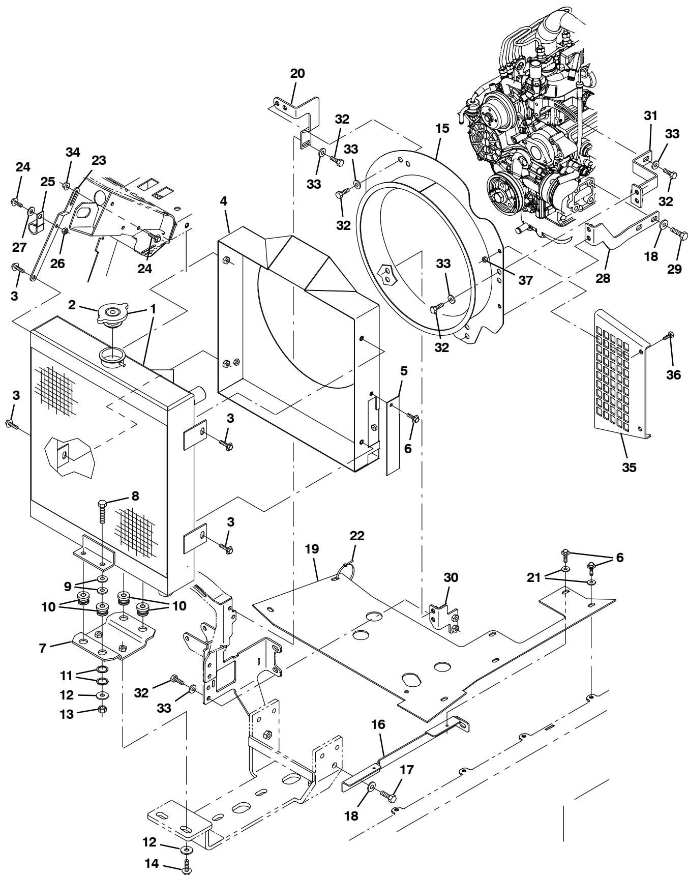
Fig. 19 – Engine Radiator Group, Diesel (0189–0499)
