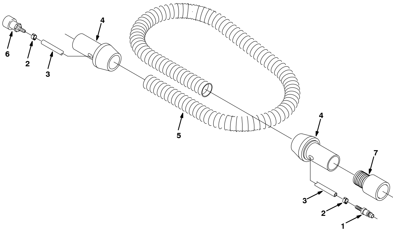
Fig. 33 – Power Wand Hose Assembly
