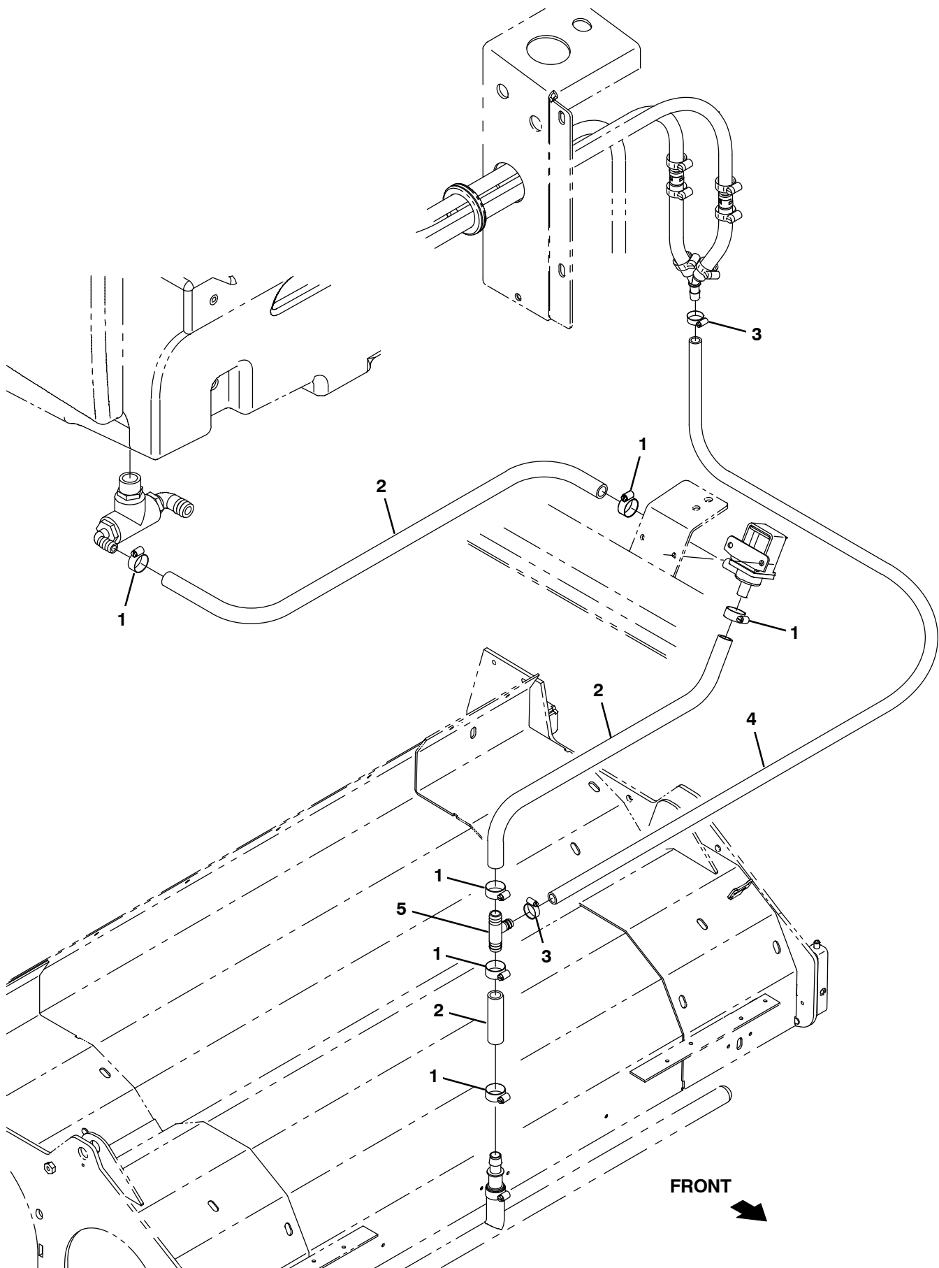
Fig. 17 – FaST Solution Supply Group, Cylindrical Scrub Head (0130– )
