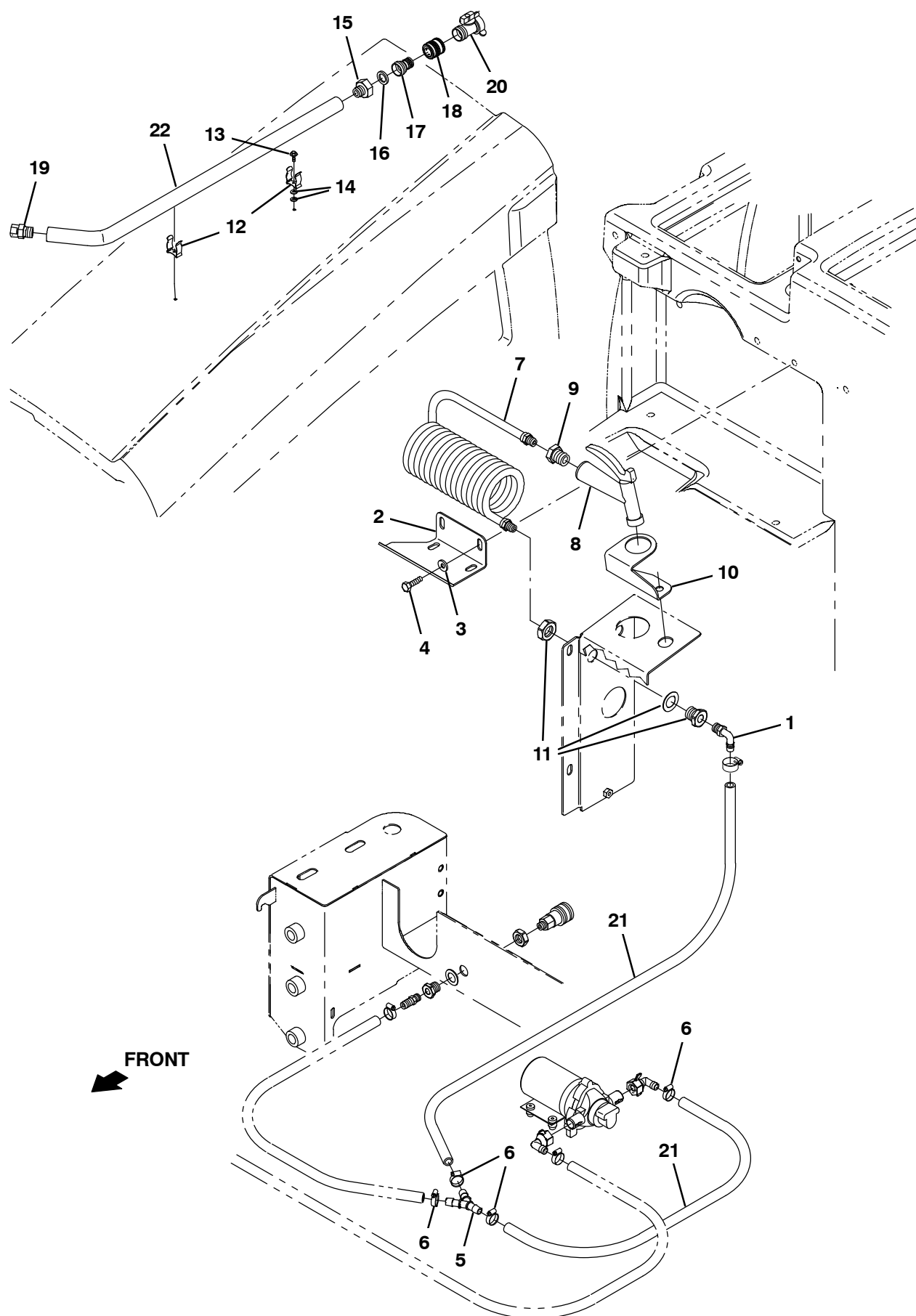
Fig. 38 – Spray Nozzle Kit with Power Wand
