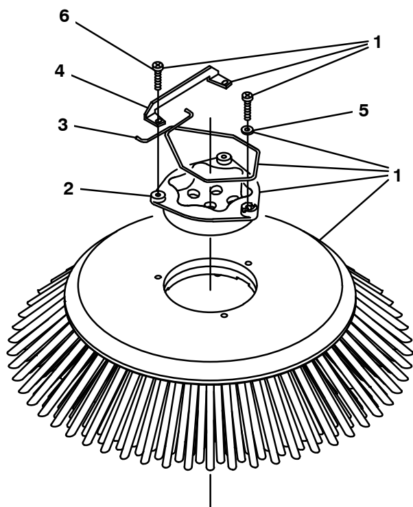
Fig. 2 – Brushes, Replacement, Side Brush
