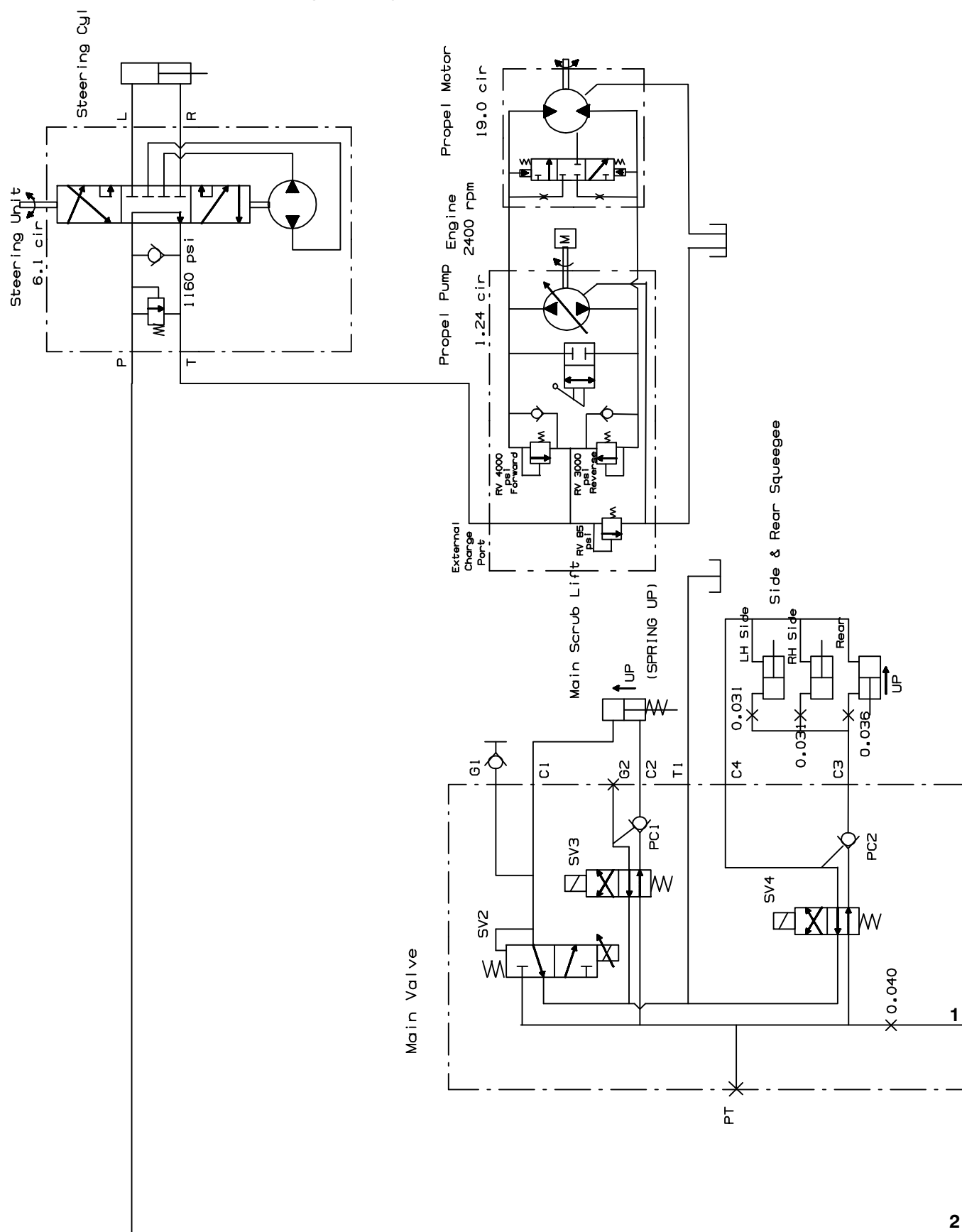
Fig. 51 – Hydraulic Schematic (0043–0244)
