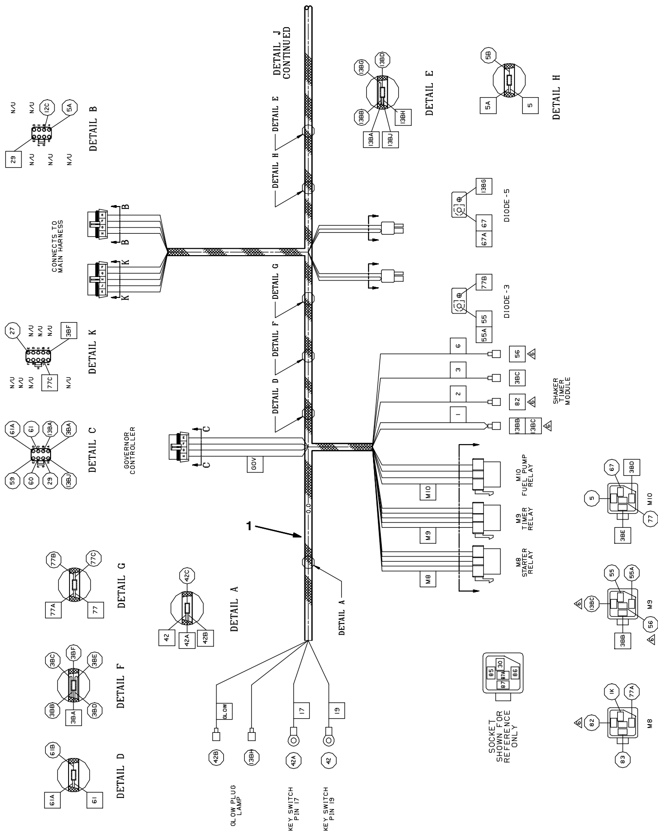
Fig. 66 – Electrical Wire Harness Group, Diesel Engine
