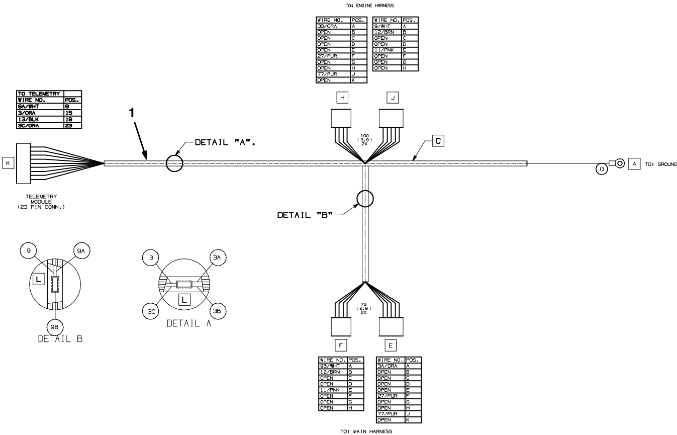
Fig. 41 – Telemetry Wire Harness Group
