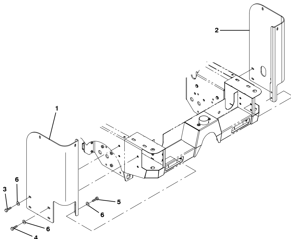
Fig. 42 – Heavy Duty Bumper Kit
