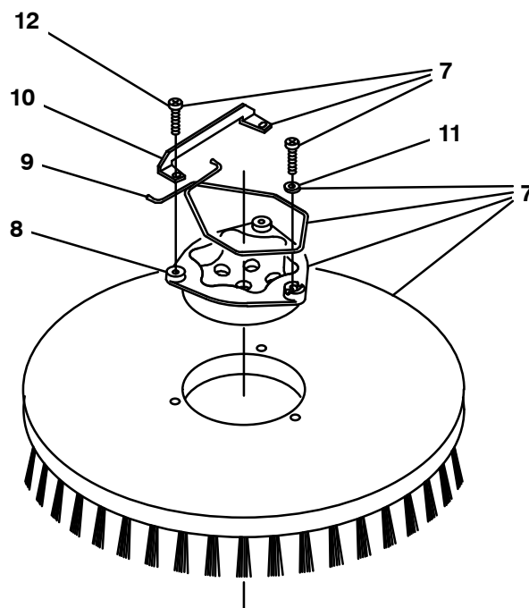
Fig. 2 – Brushes, Replacement, Side Brush
