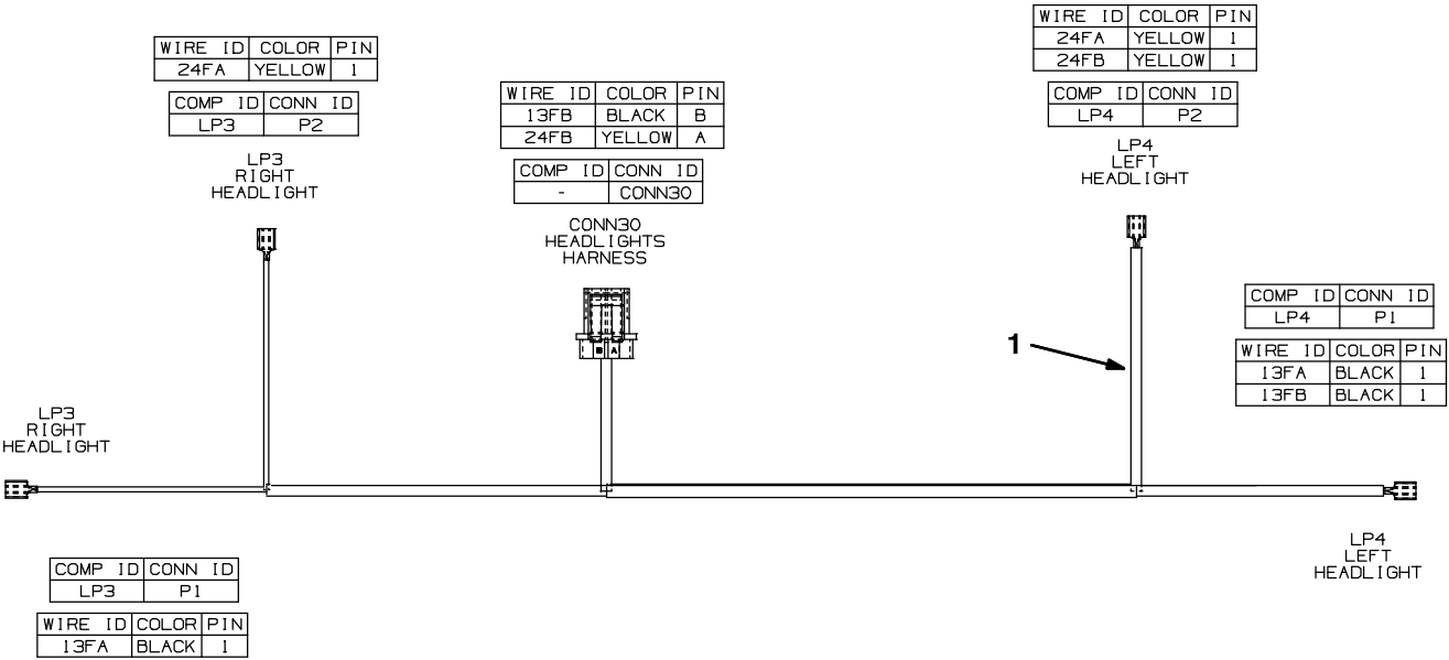
Fig. 67 – Electrical Wire Harness Group, Headlight
