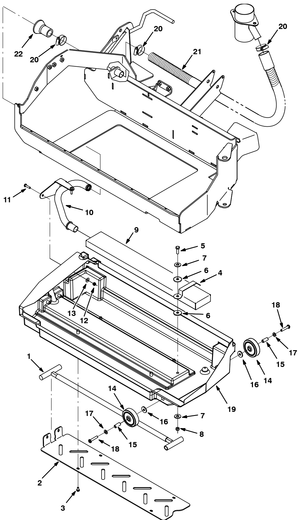
Fig. 35 – Cylindrical Scrub Head Debris Tray Group
