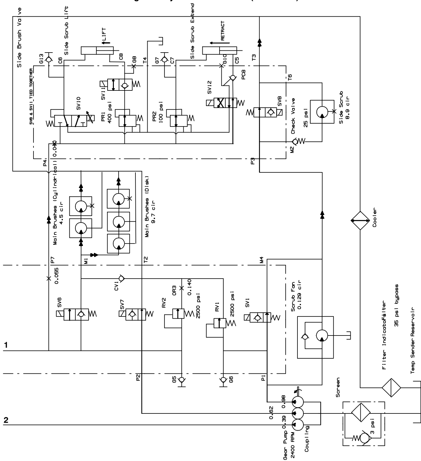
Fig. 51 – Hydraulic Schematic (0043-0244)
