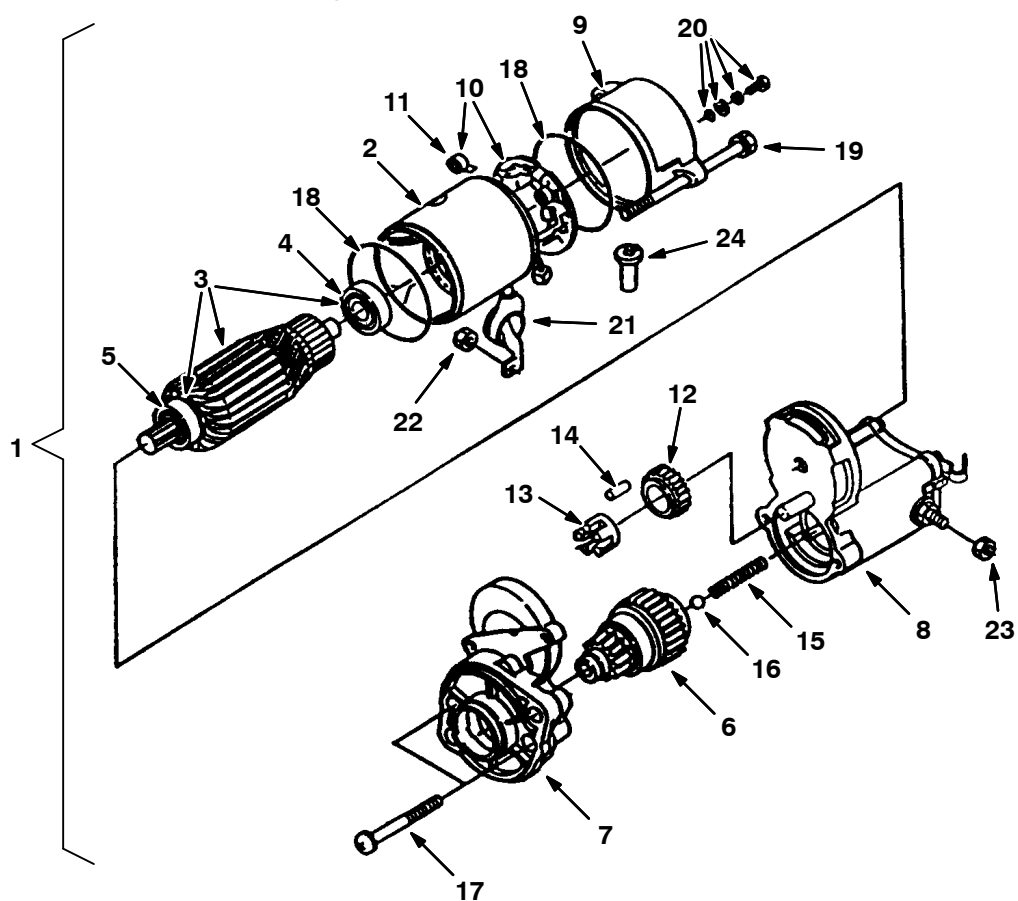
Fig. 14 – Starter Breakdown, 74405
