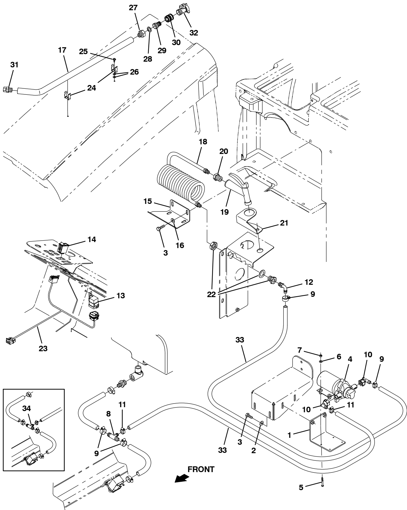
Fig. 37 – Spray Nozzle Kit
