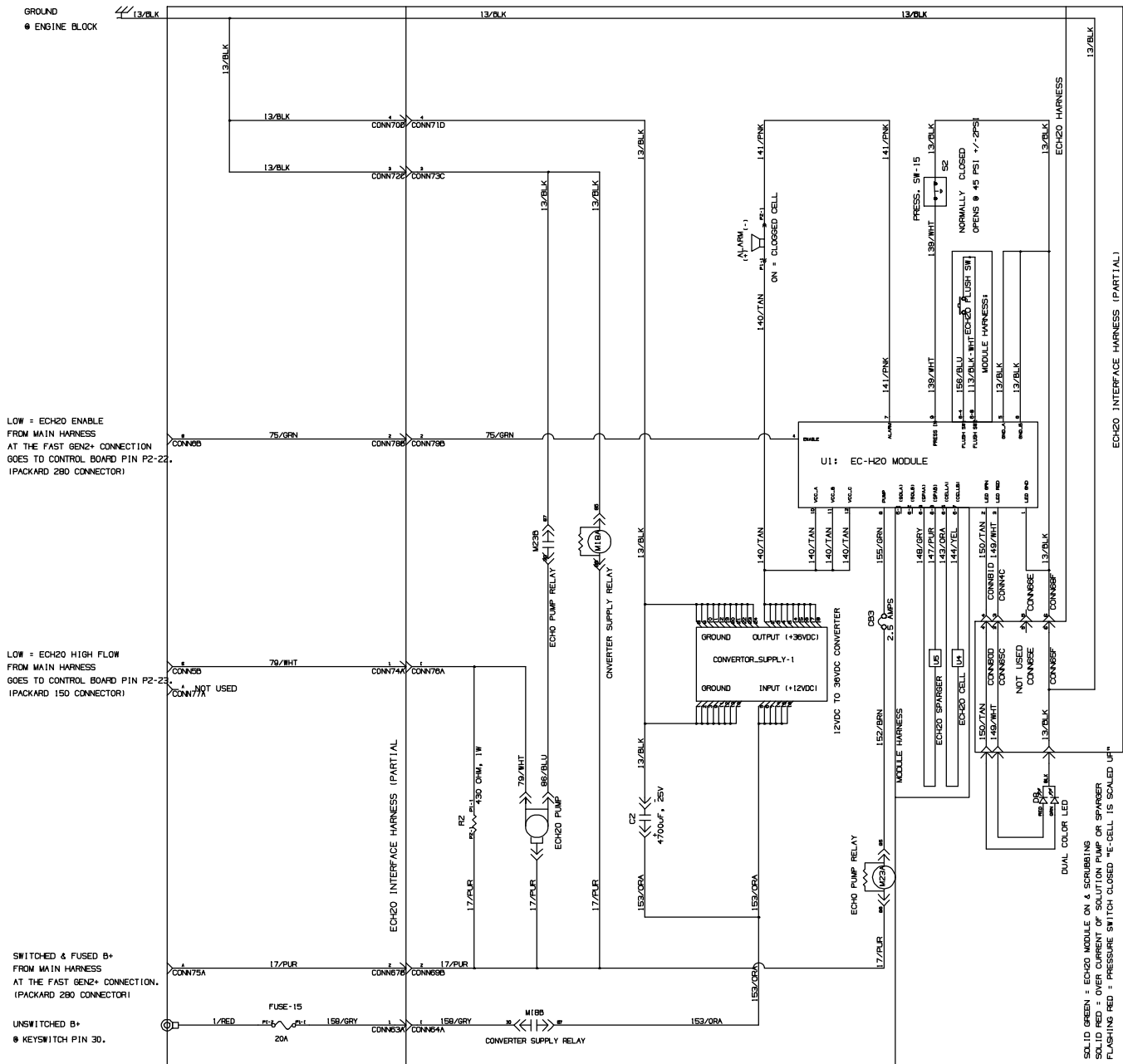
Fig. 62 – Electrical Schematic
