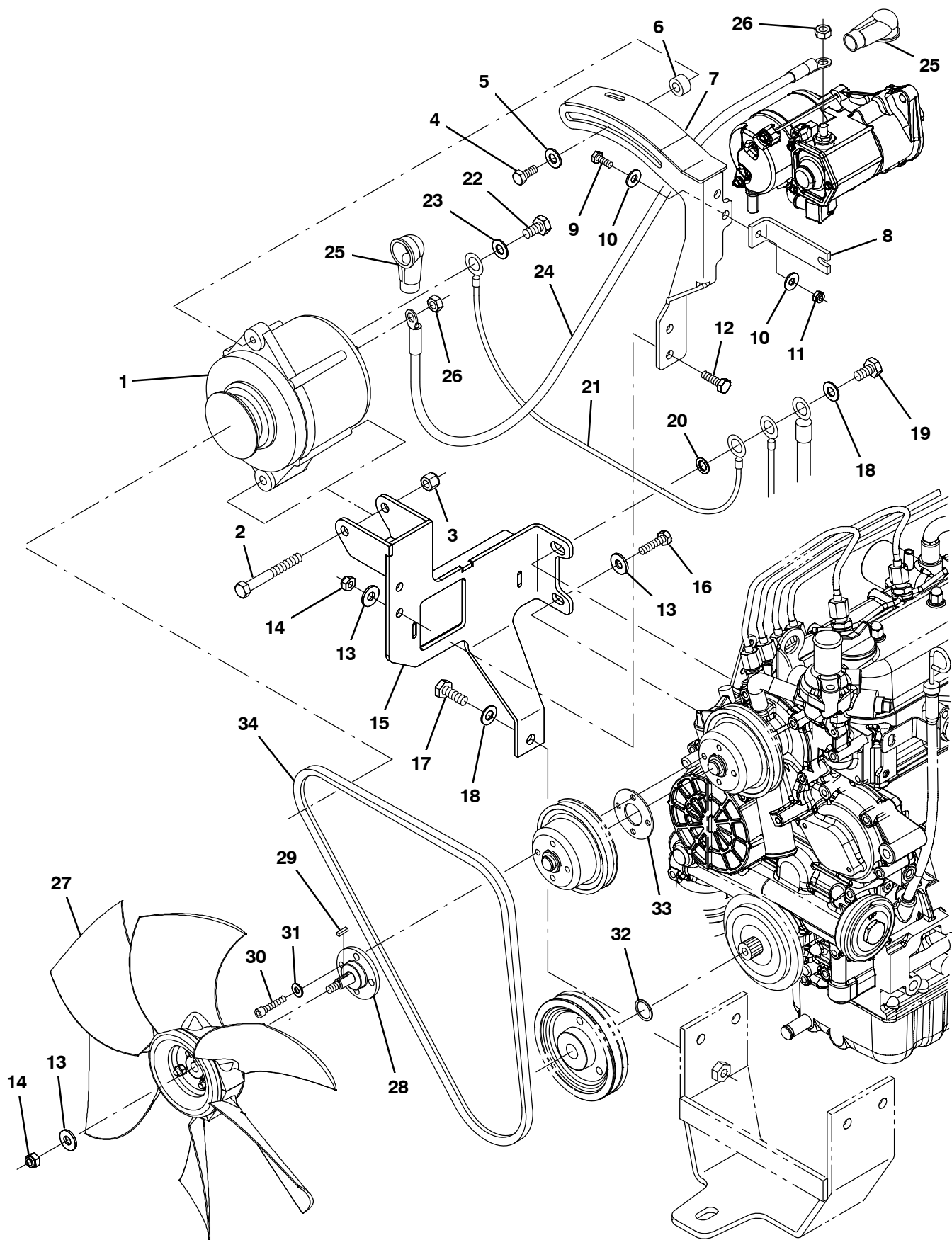
Fig. 16 – Engine Alternator Group, Diesel (0193– )
