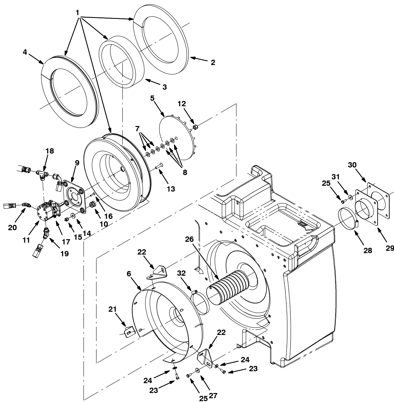
Fig. 48 – Vacuum Fan Group, Scrubbing (0000-0778)
