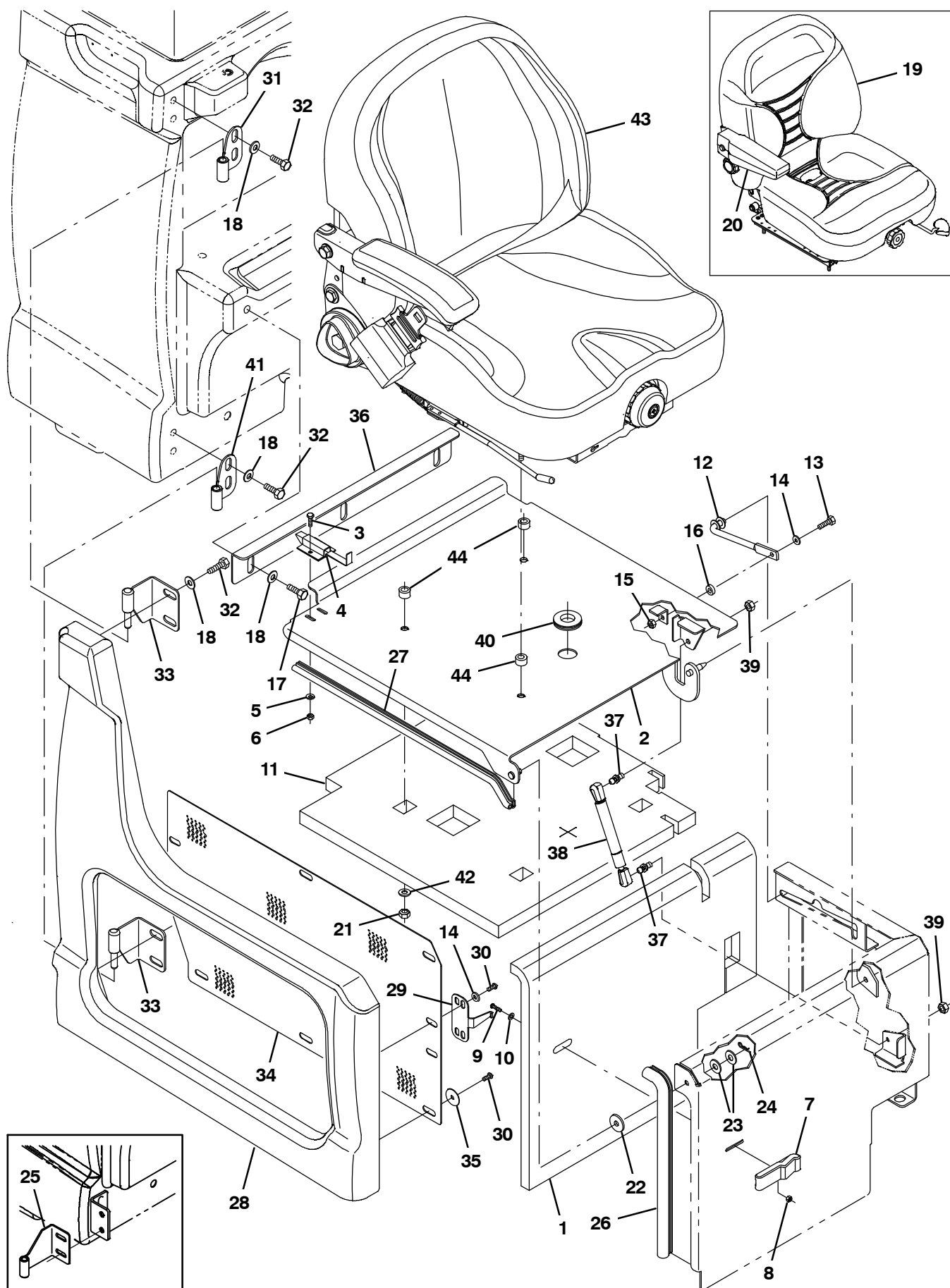
Fig. 7 – Seat Group
