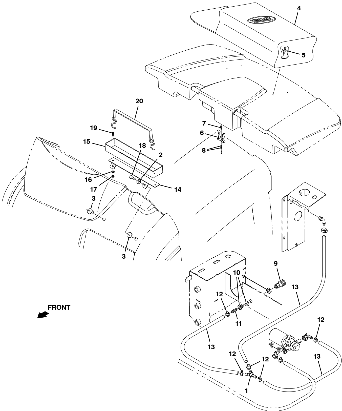
Fig. 36 – Power Wand Pump and Mount Group with Spray Nozzle
