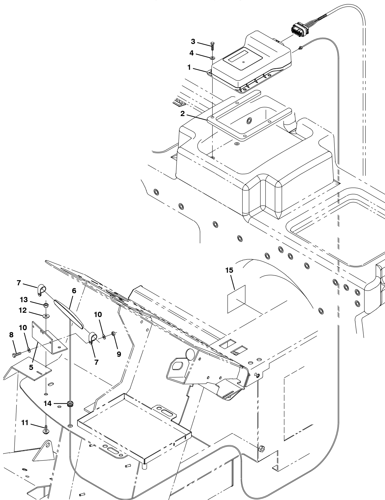
Fig. 40 – Telemetry Group
