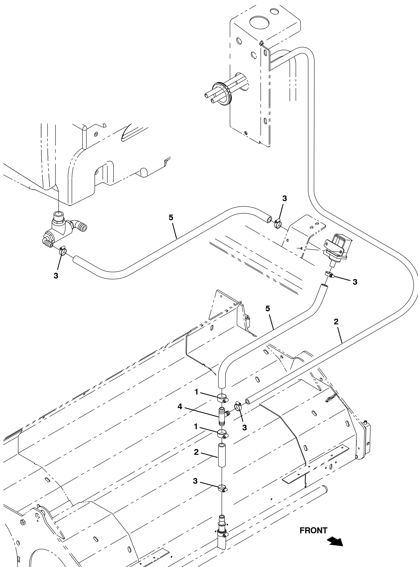
Fig. 24 – ec-H2O Solution Supply Group, Cylindrical Scrub Head
