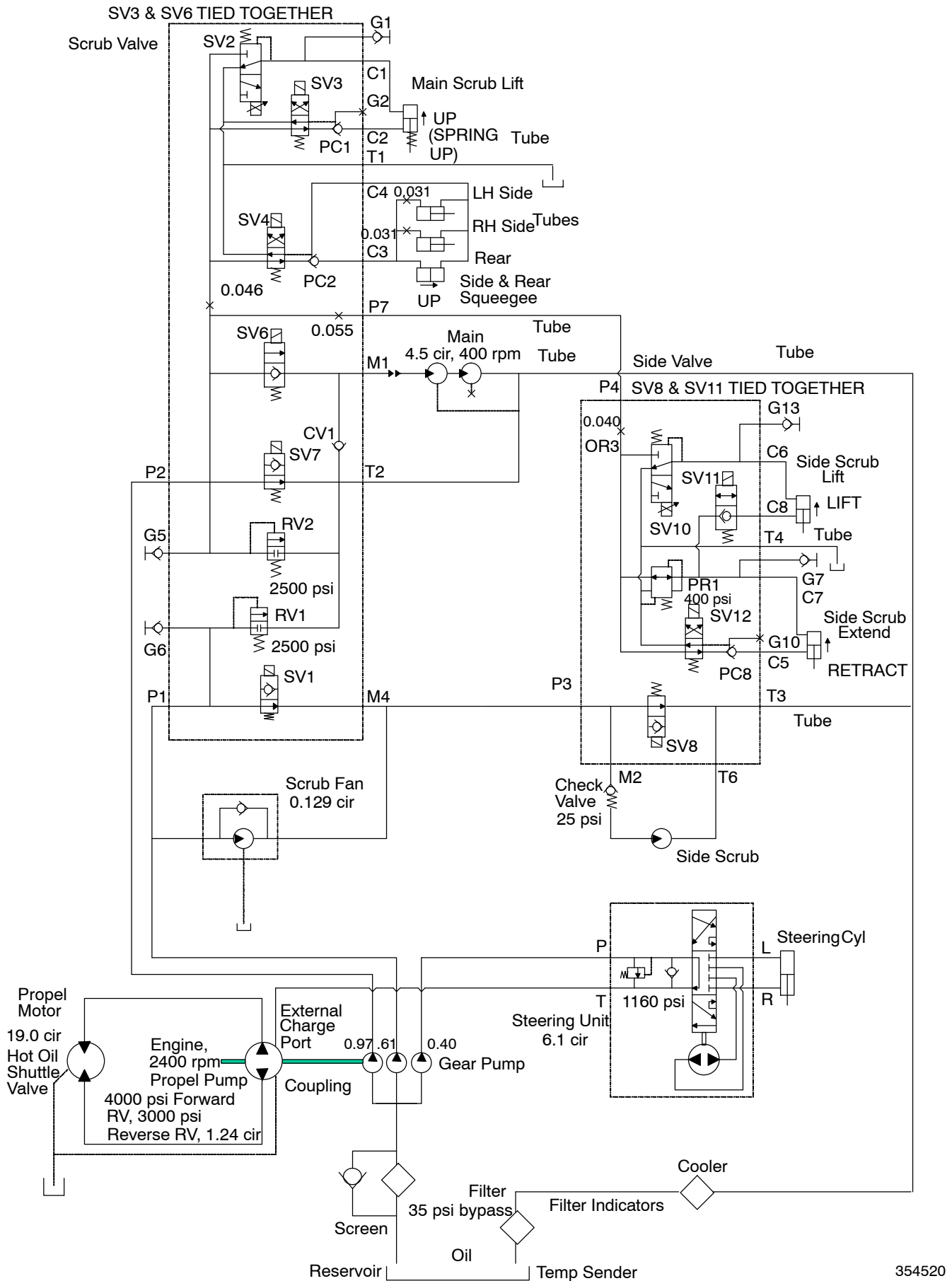
Fig. 50 – Hydraulic Schematic (0000–0042)
