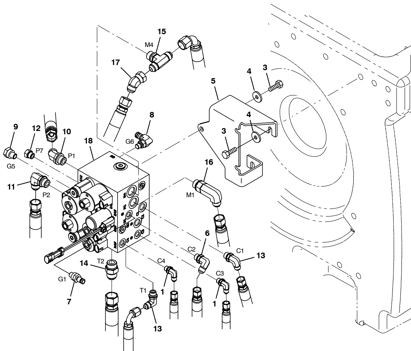
Fig. 61 – Hydraulic Valve Group
