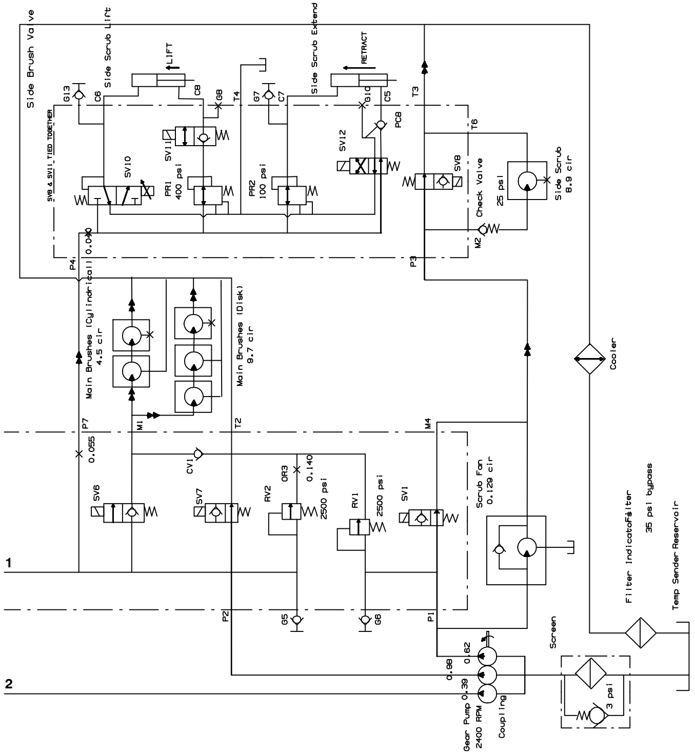
Fig. 52 – Hydraulic Schematic (0245- )
