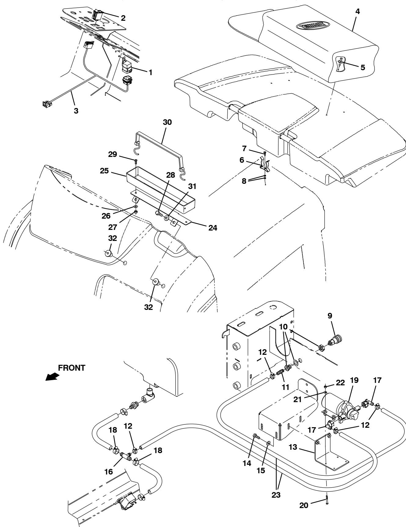
Fig. 35 – Power Wand Pump and Mount Group
