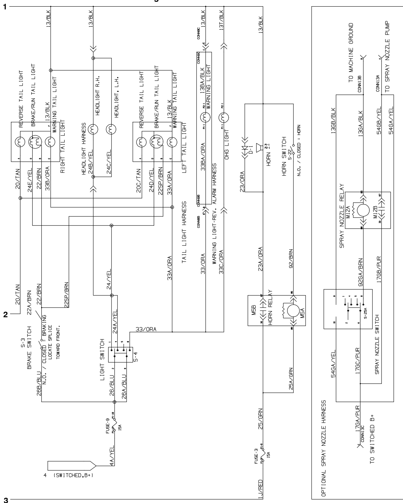
Fig. 62 – Electrical Schematic
