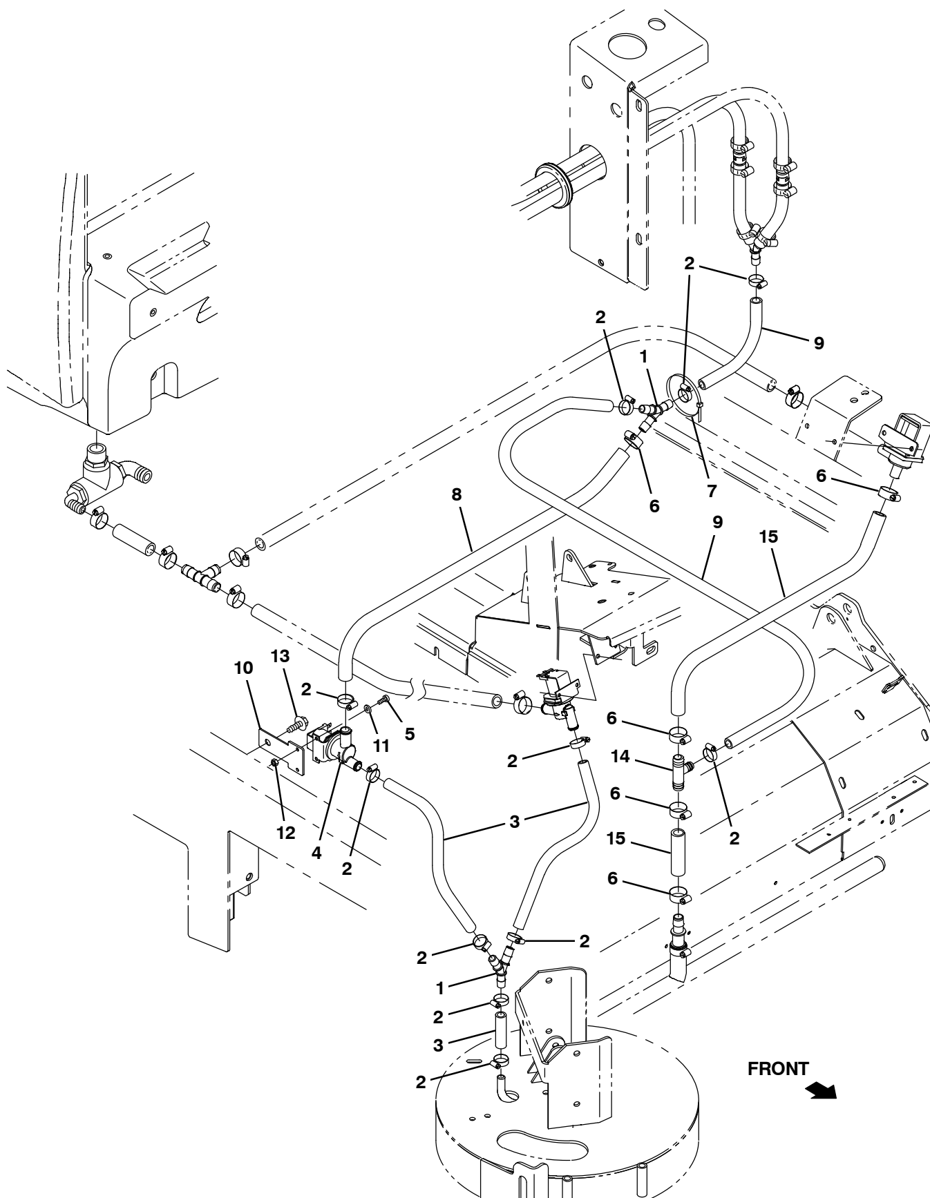
Fig. 18 – FaST Solution Supply Group with Side Brush, Cylindrical Scrub Head (0130- )
