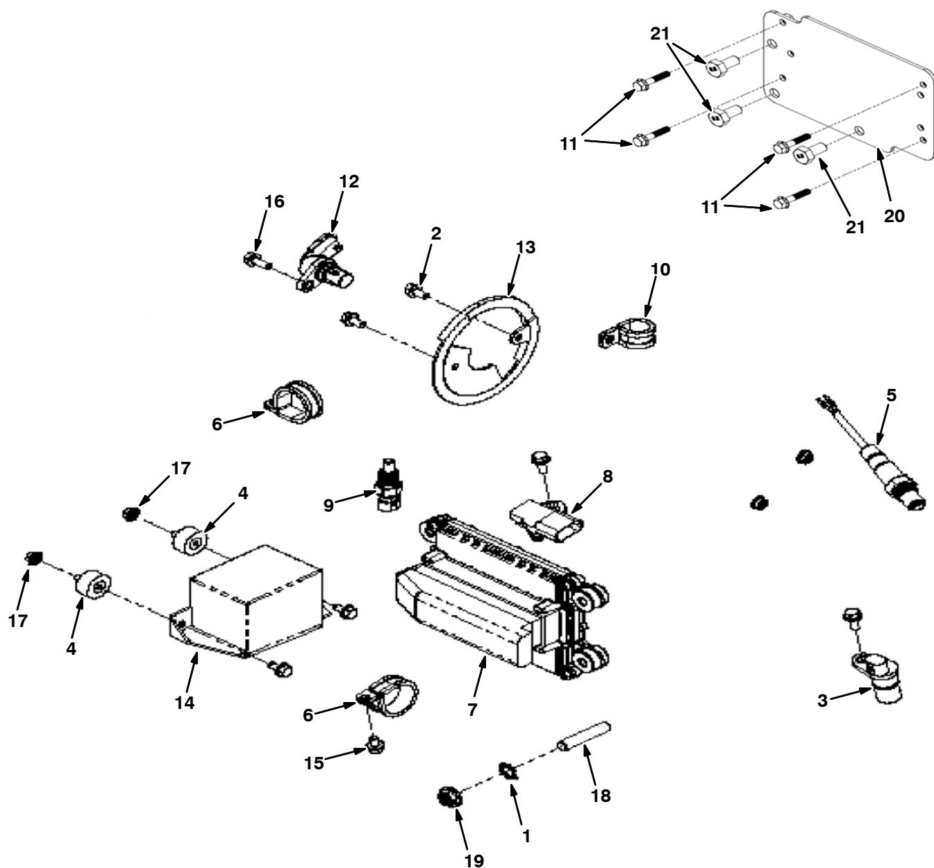
Fig. 19 – Electrical Group
