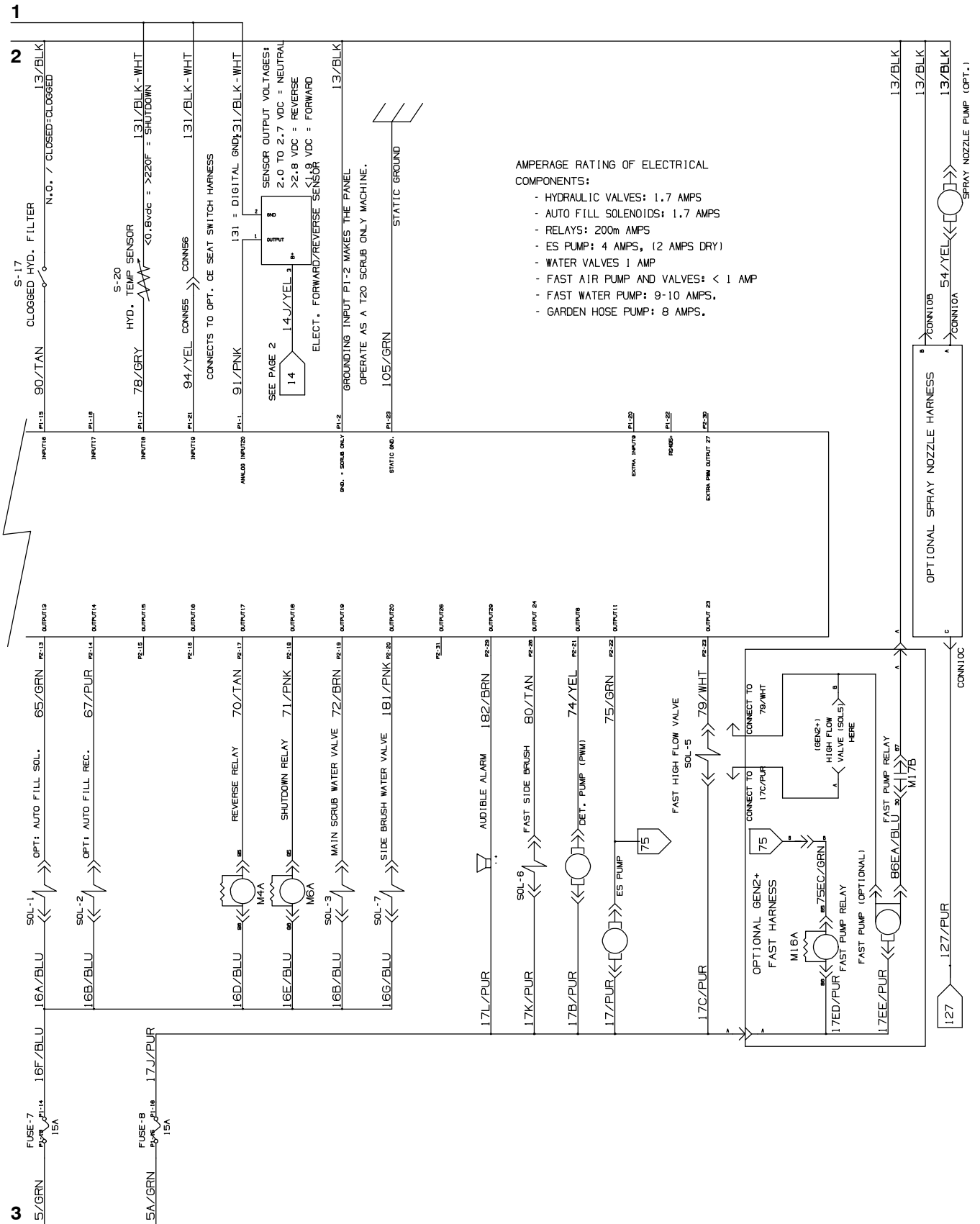
Fig. 91 – Mitsubishi Electrical Schematic (0500- )
