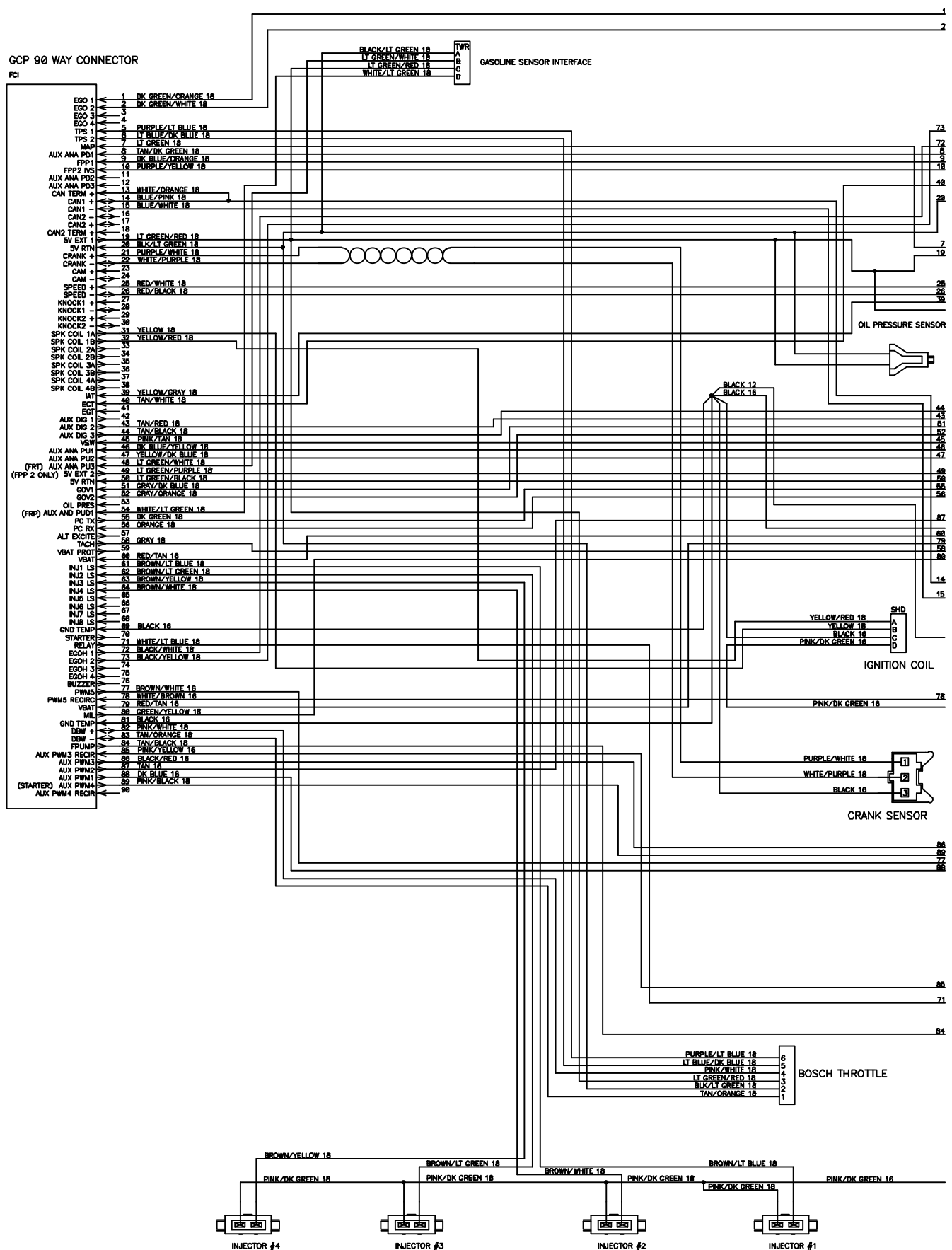
Fig. 88 – GM Electrical Schematic, Gas Engine Harness (0203-0499)
