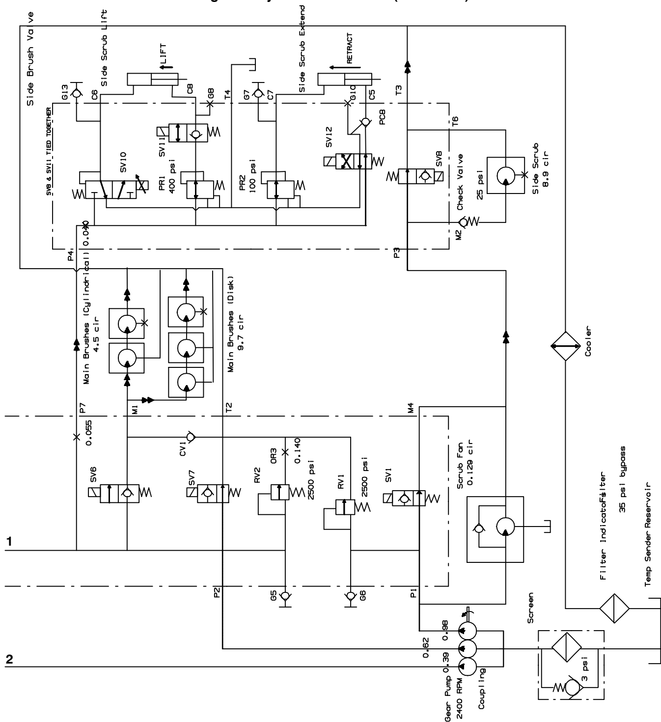
Fig. 72 – Hydraulic Schematic (0043-0244)
