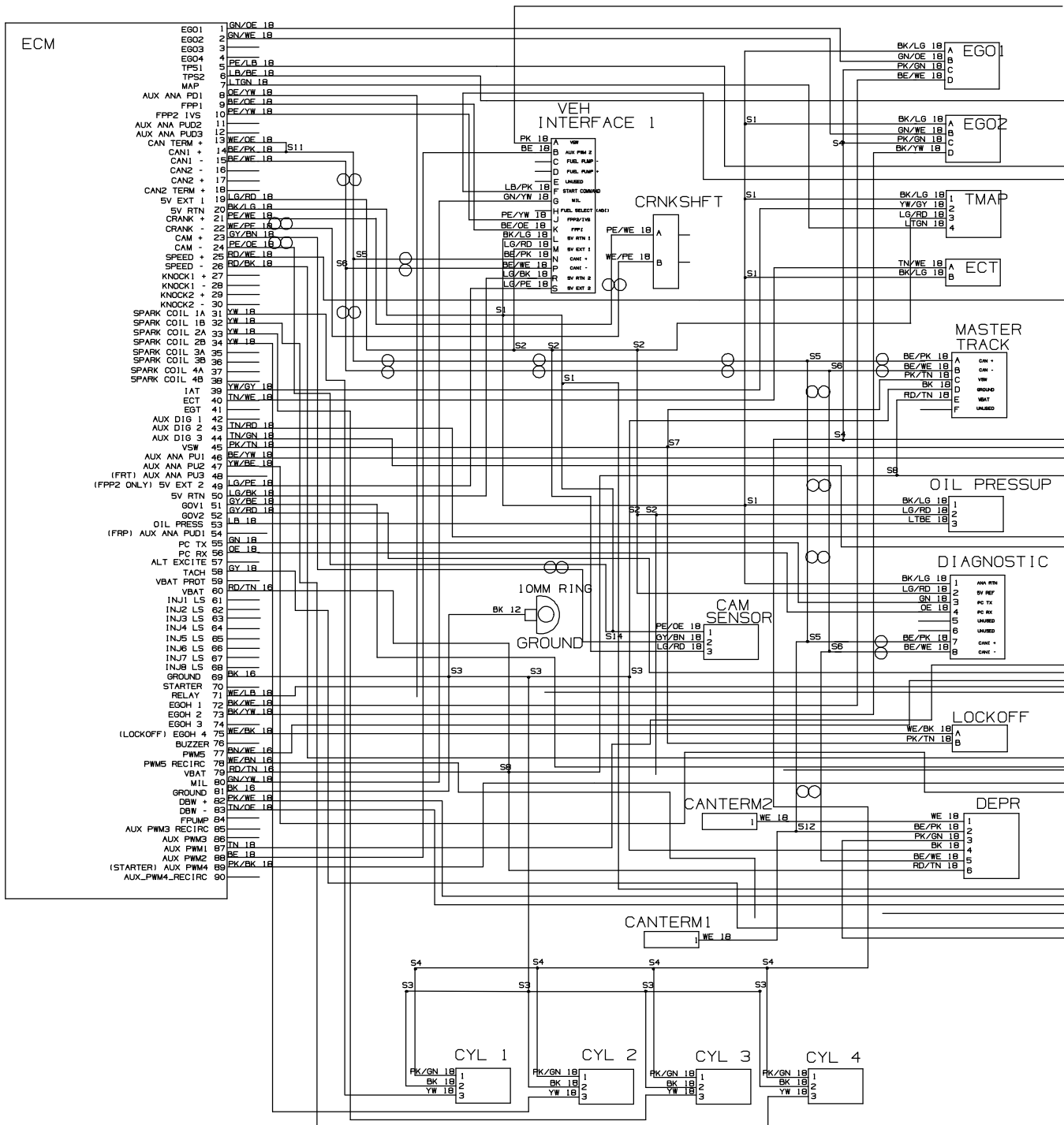
Fig. 93 – Mitsubishi Electrical Schematic, LPG Engine Harness (0500– )
