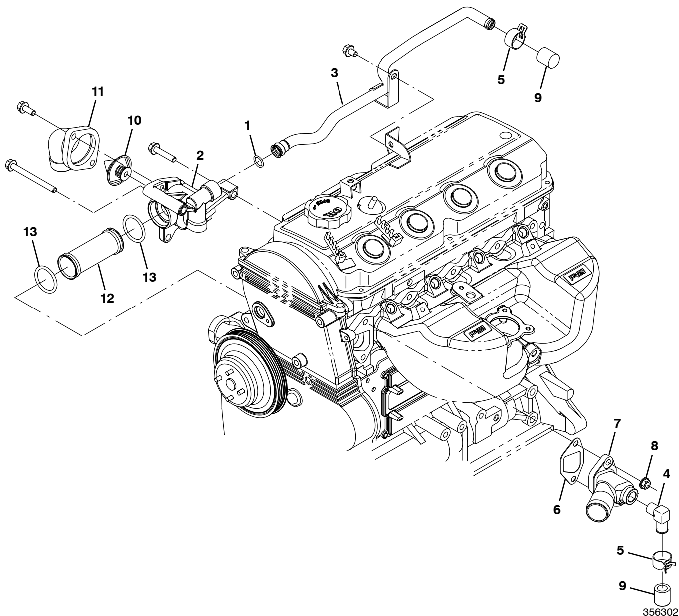
Fig. 17 – Coolant Group
