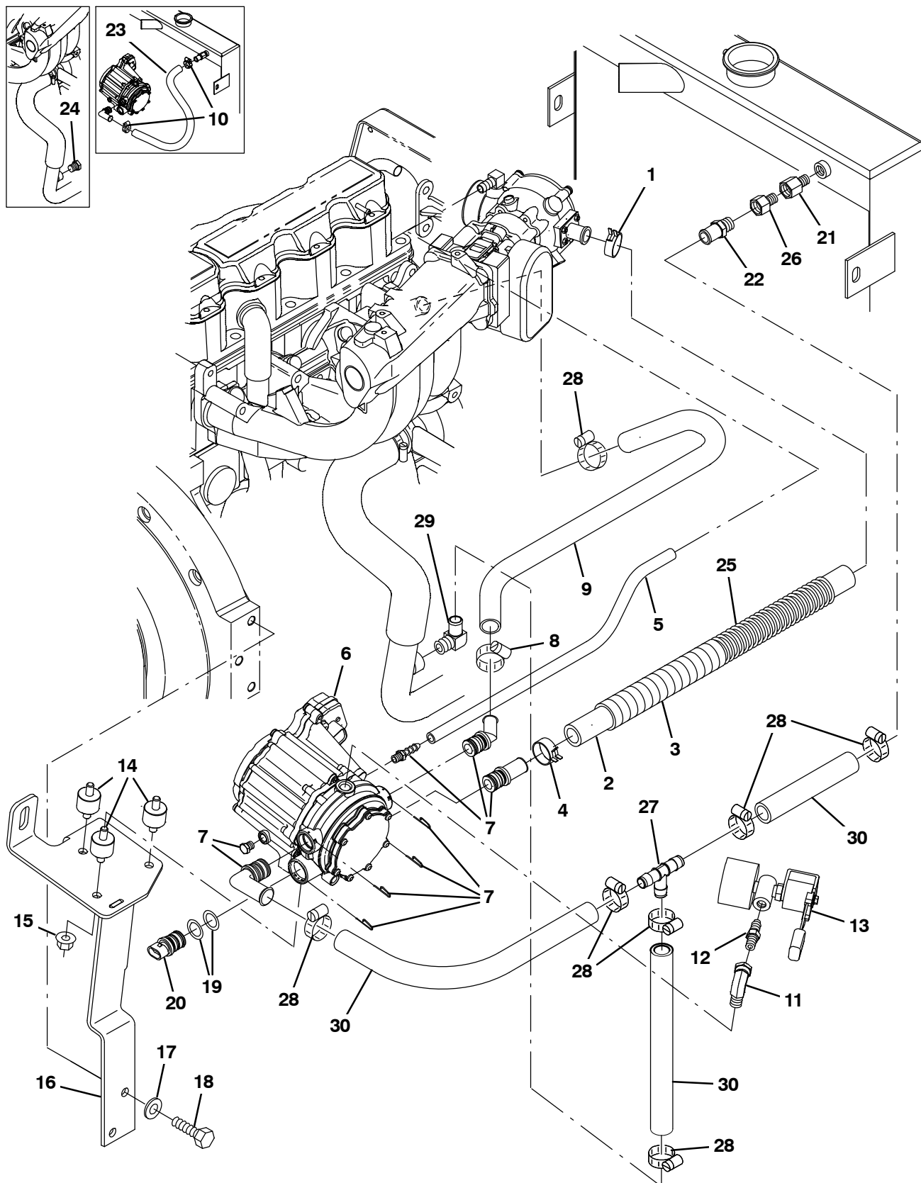
Fig. 18 – GM Engine Vaporizer Group, LPG (0203-0499)
