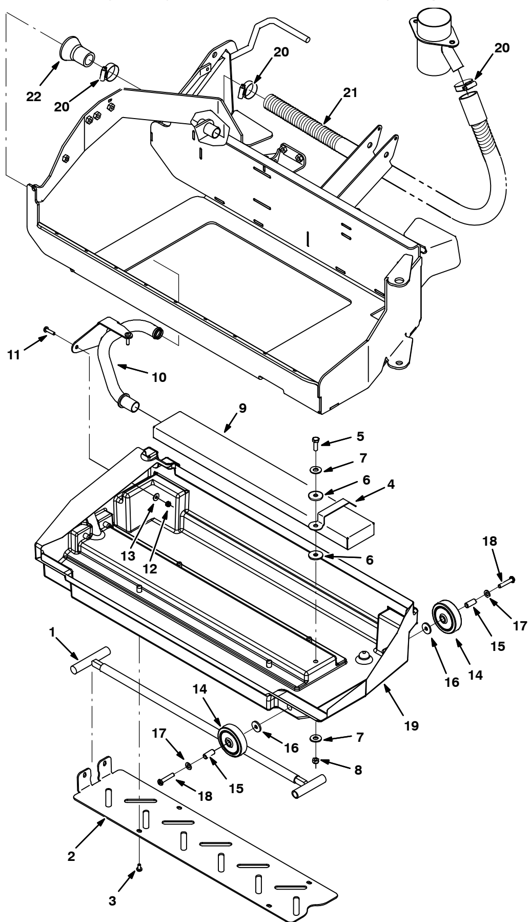
Fig. 55 – Cylindrical Scrub Head Debris Tray Group
