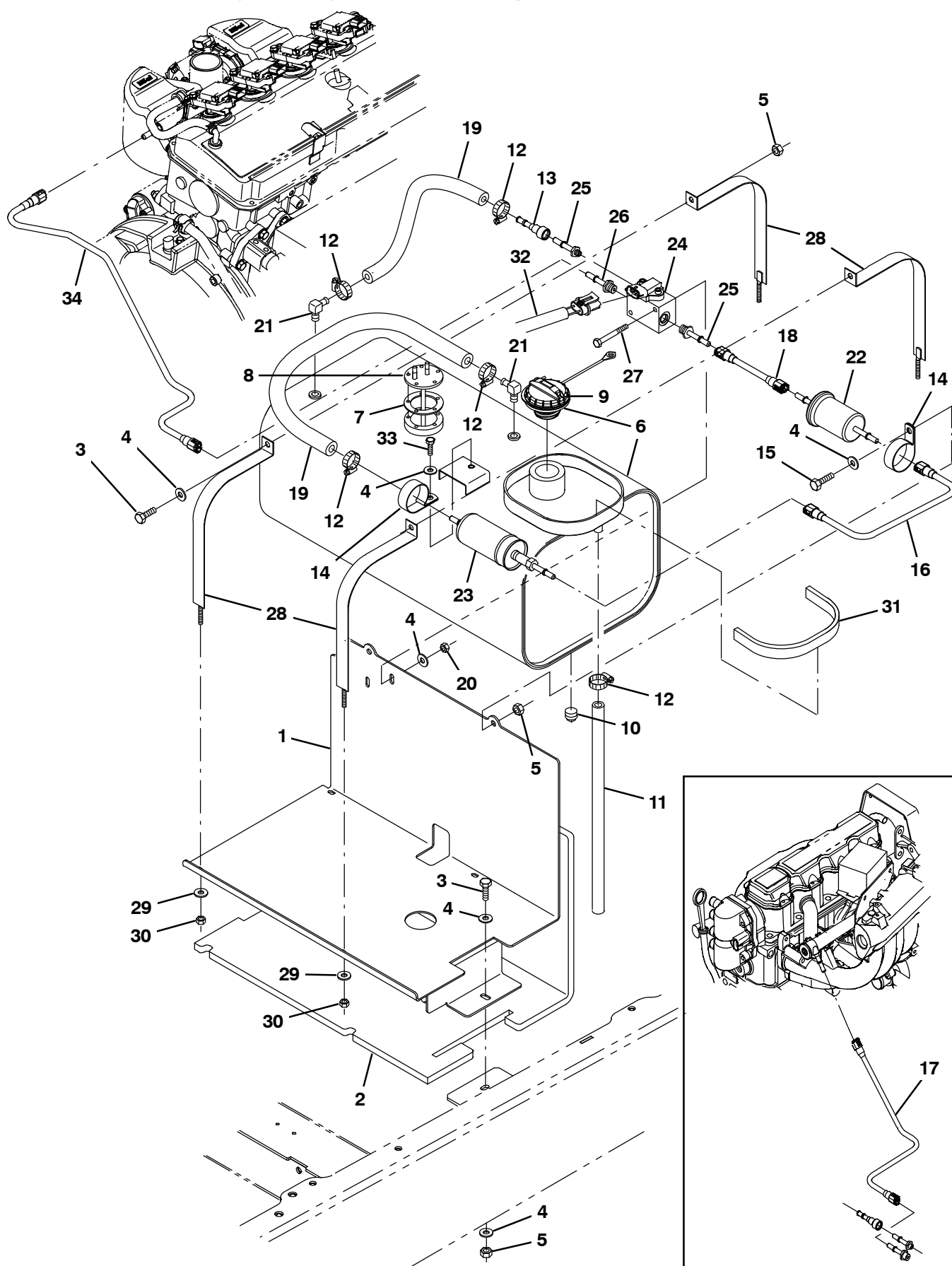
Fig. 40 – Engine Fuel Tank Group, Gasoline (0044– )
