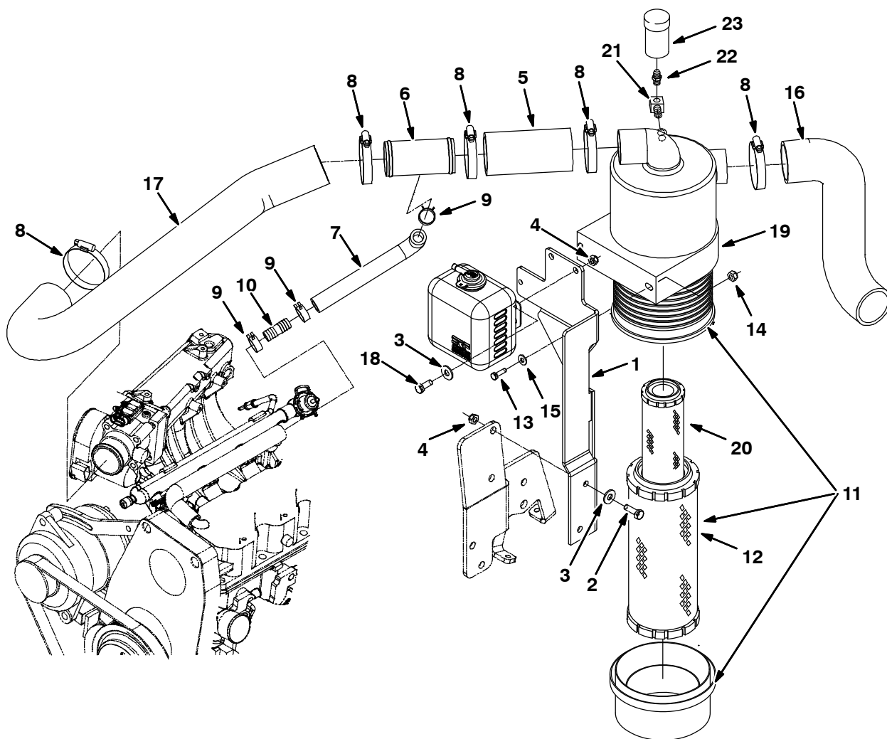
Fig. 20 – GM Engine Air Cleaner Group, Gasoline (0000–0043)
