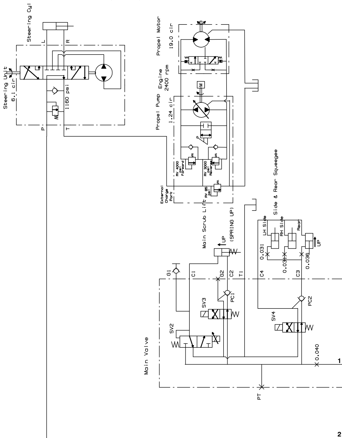
Fig. 72 – Hydraulic Schematic (0043–0244)
