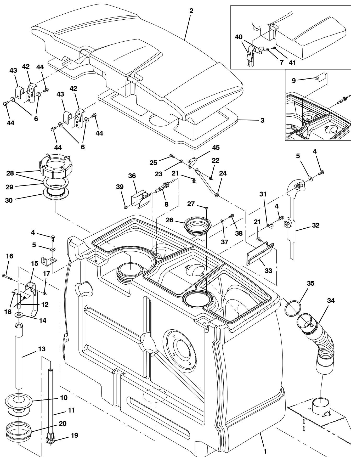
Fig. 67 – Recovery Tank Group
