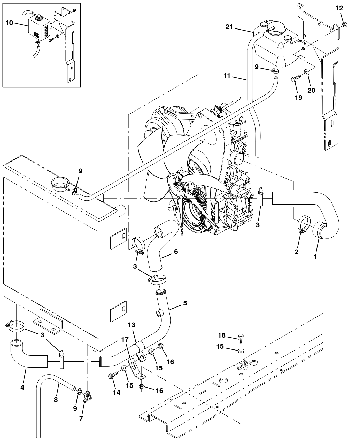
Fig. 29 – GM Engine Radiator Hose Group (0189–0499)
