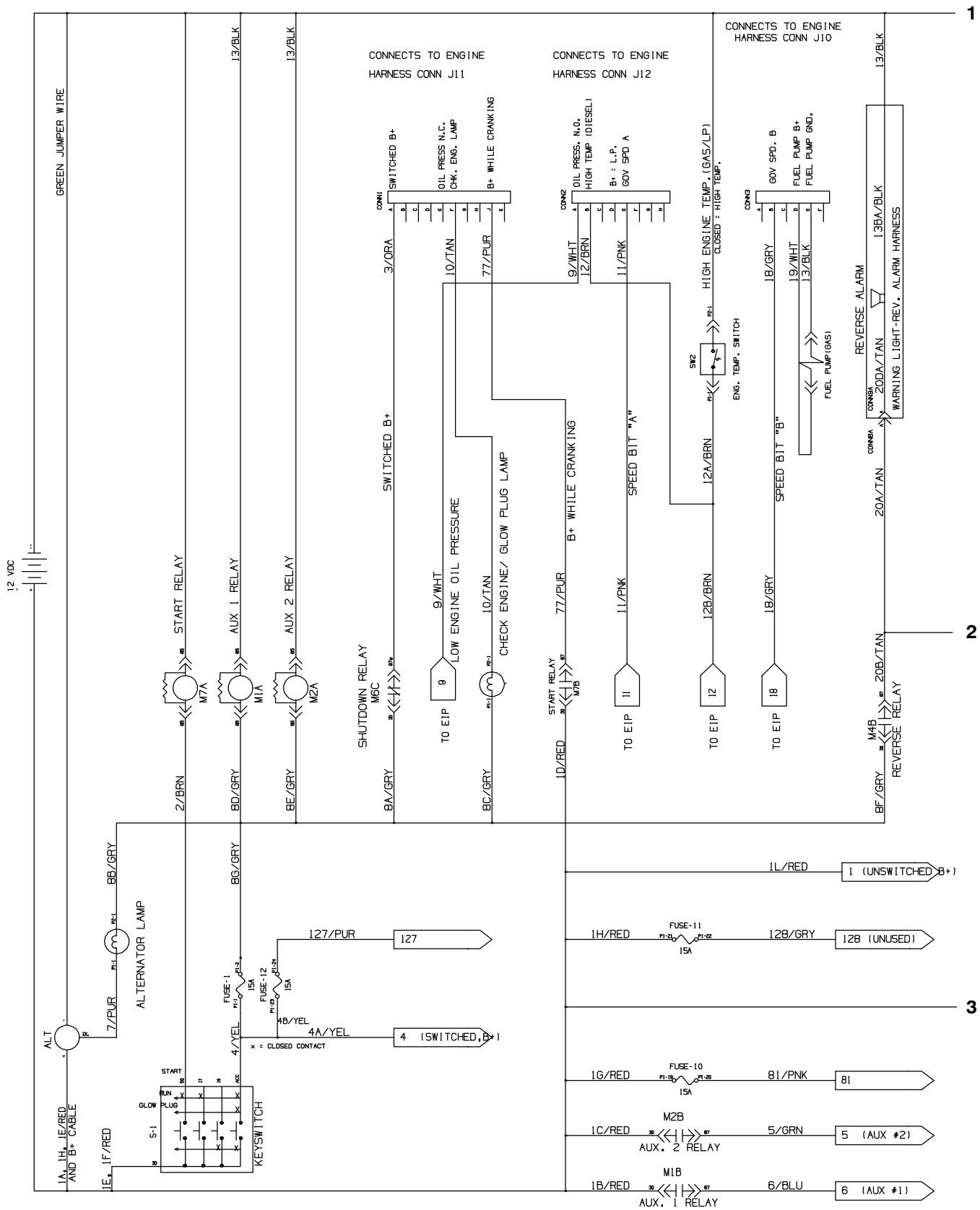
Fig. 83 – GM Electrical Schematic (0000–0043)
