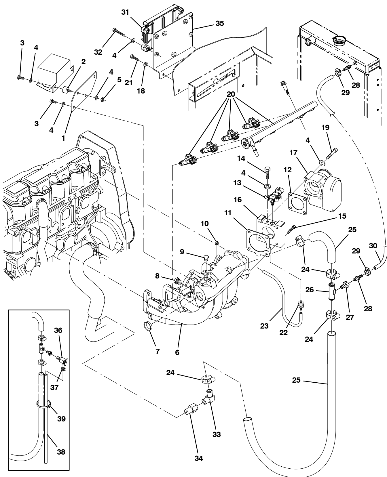
Fig. 13 – GM Engine EFI Group, Gasoline (0044-0202)
