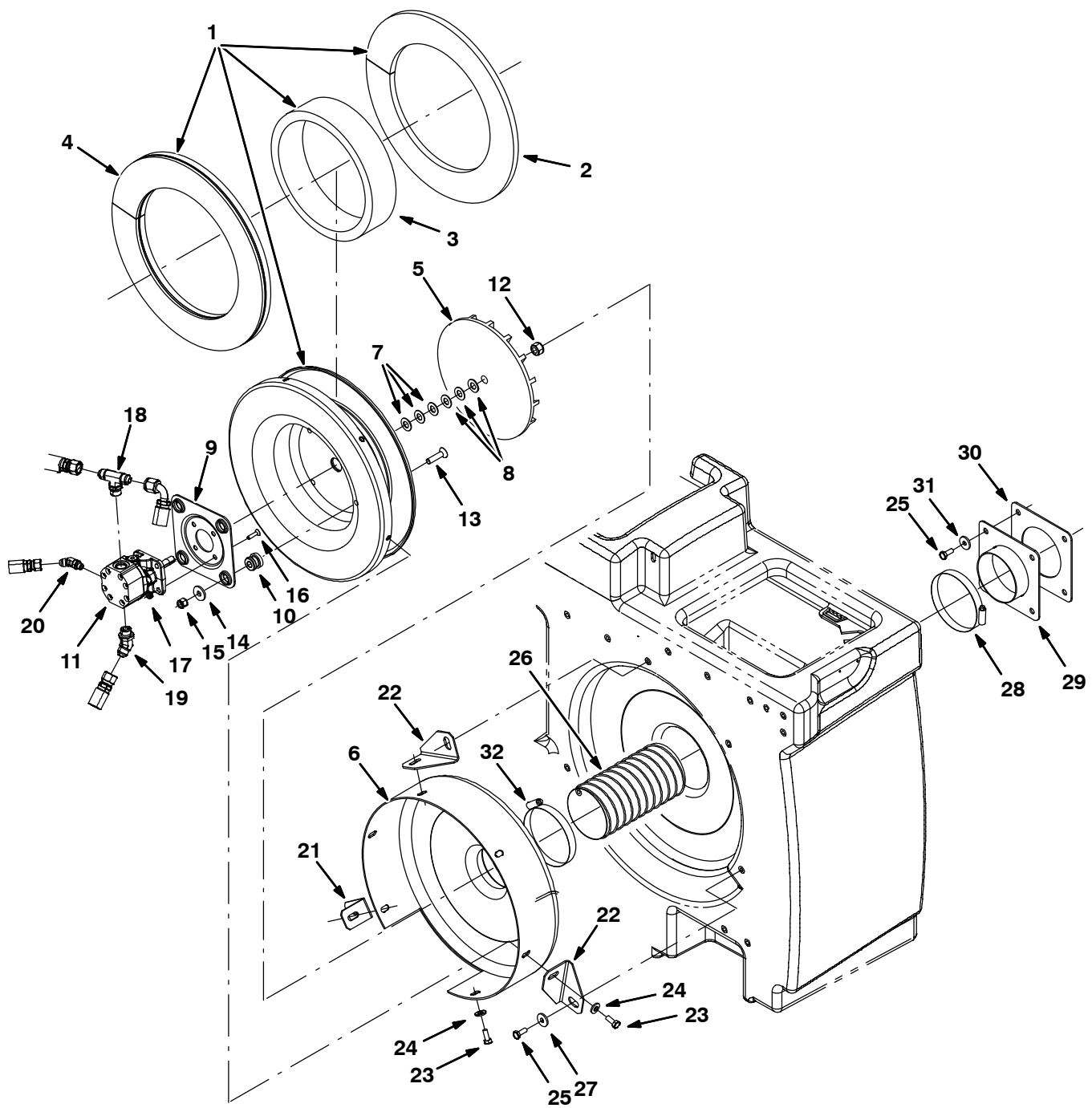
Fig. 69 – Vacuum Fan Group, Scrubbing (0000–0778)
