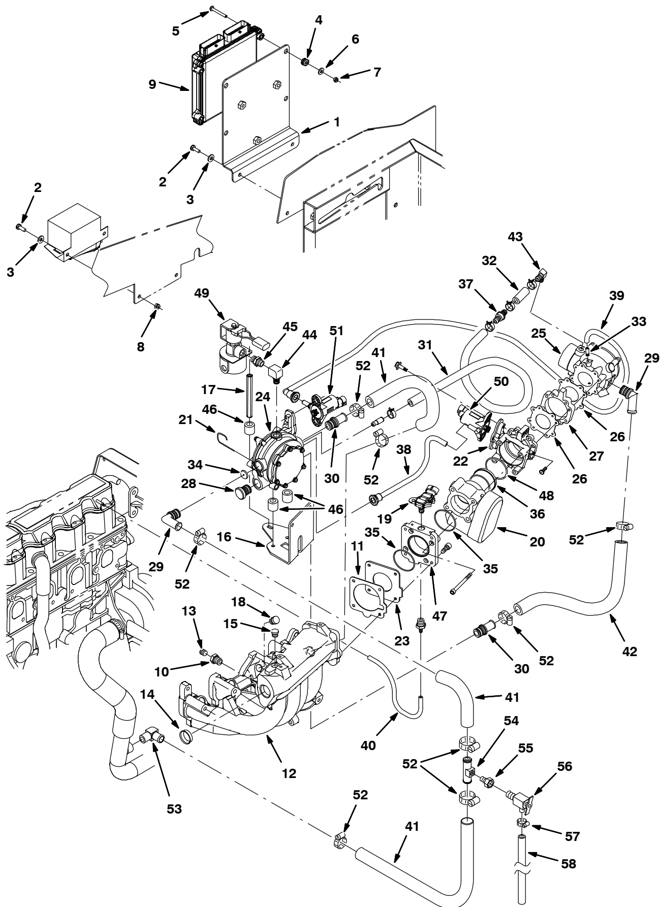
Fig. 15 – GM Engine EFI Group, LPG (0000-0043)
