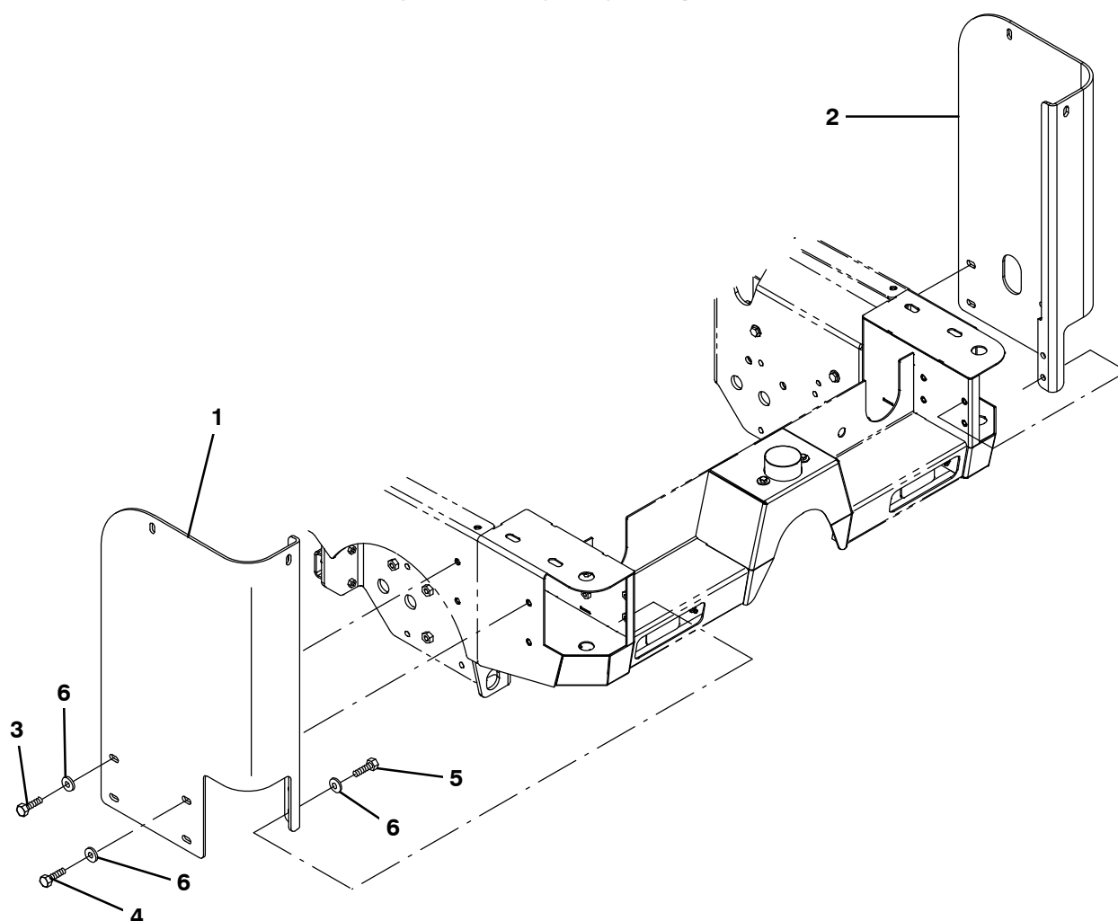
Fig. 43 – Heavy Duty Bumper Kit
