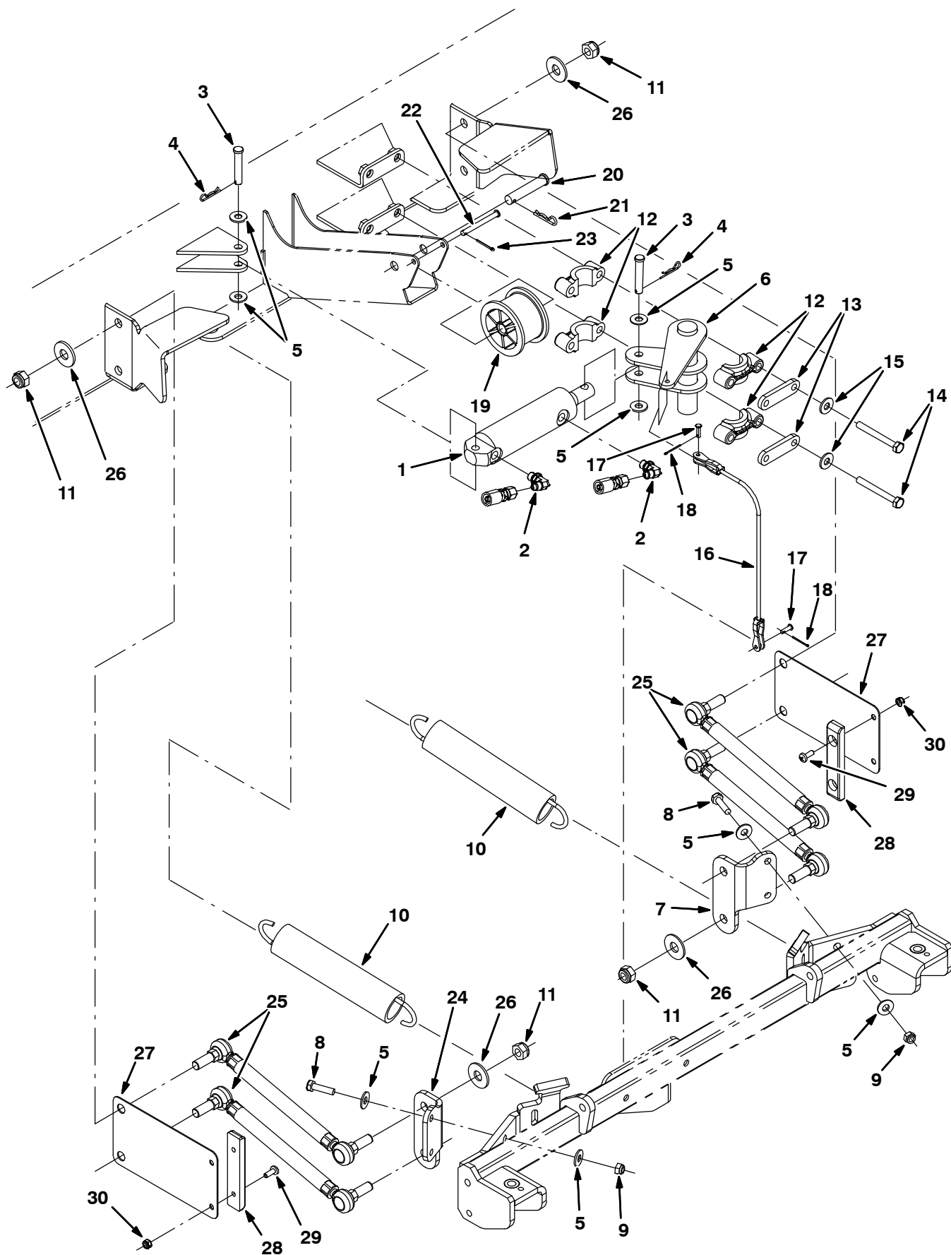
Fig. 56 – Rear Squeegee Lift Group
