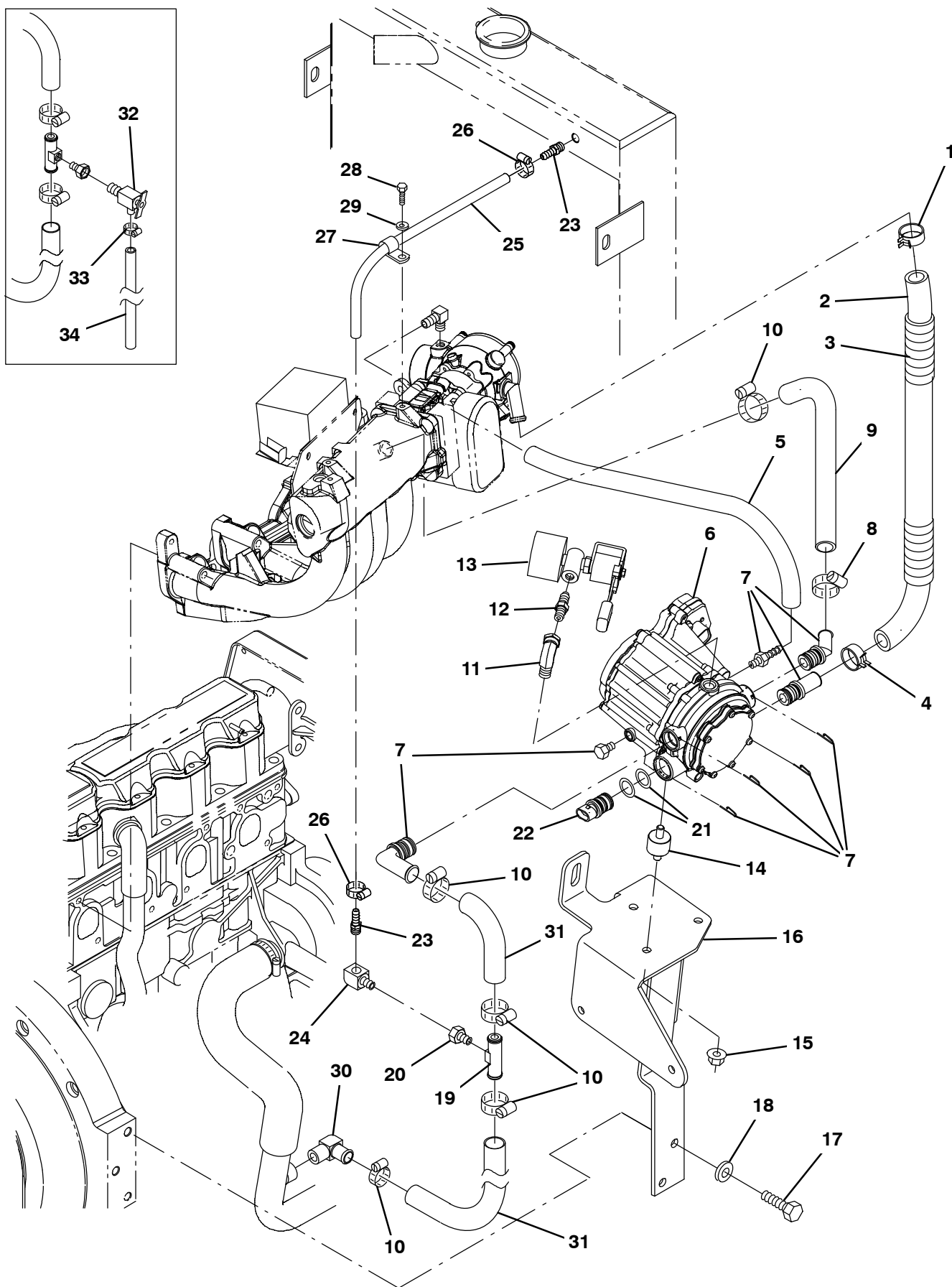
Fig. 17 – GM Engine Vaporizer Group, LPG (0044-0202)
