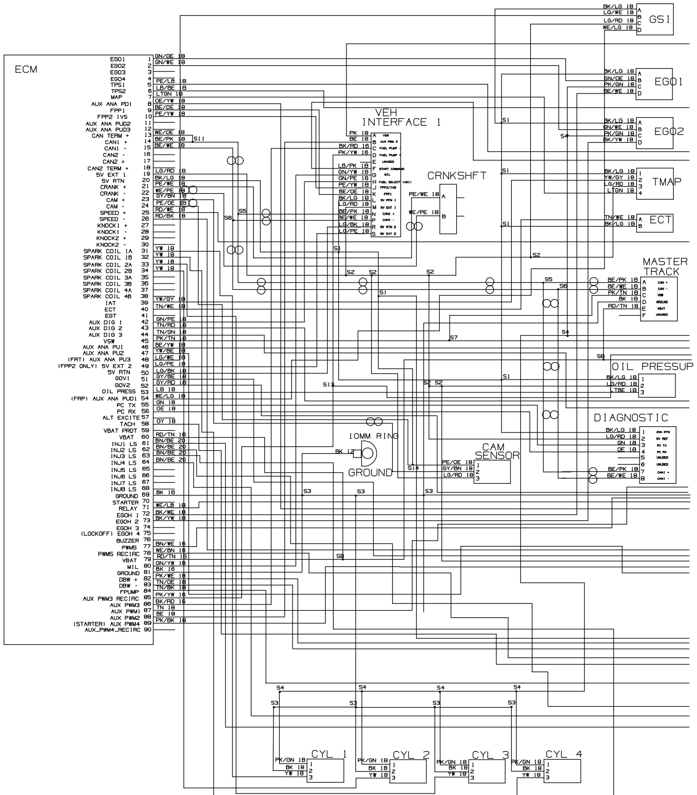
Fig. 92 – Mitsubishi Electrical Schematic, Gas Engine Harness (0500– )
