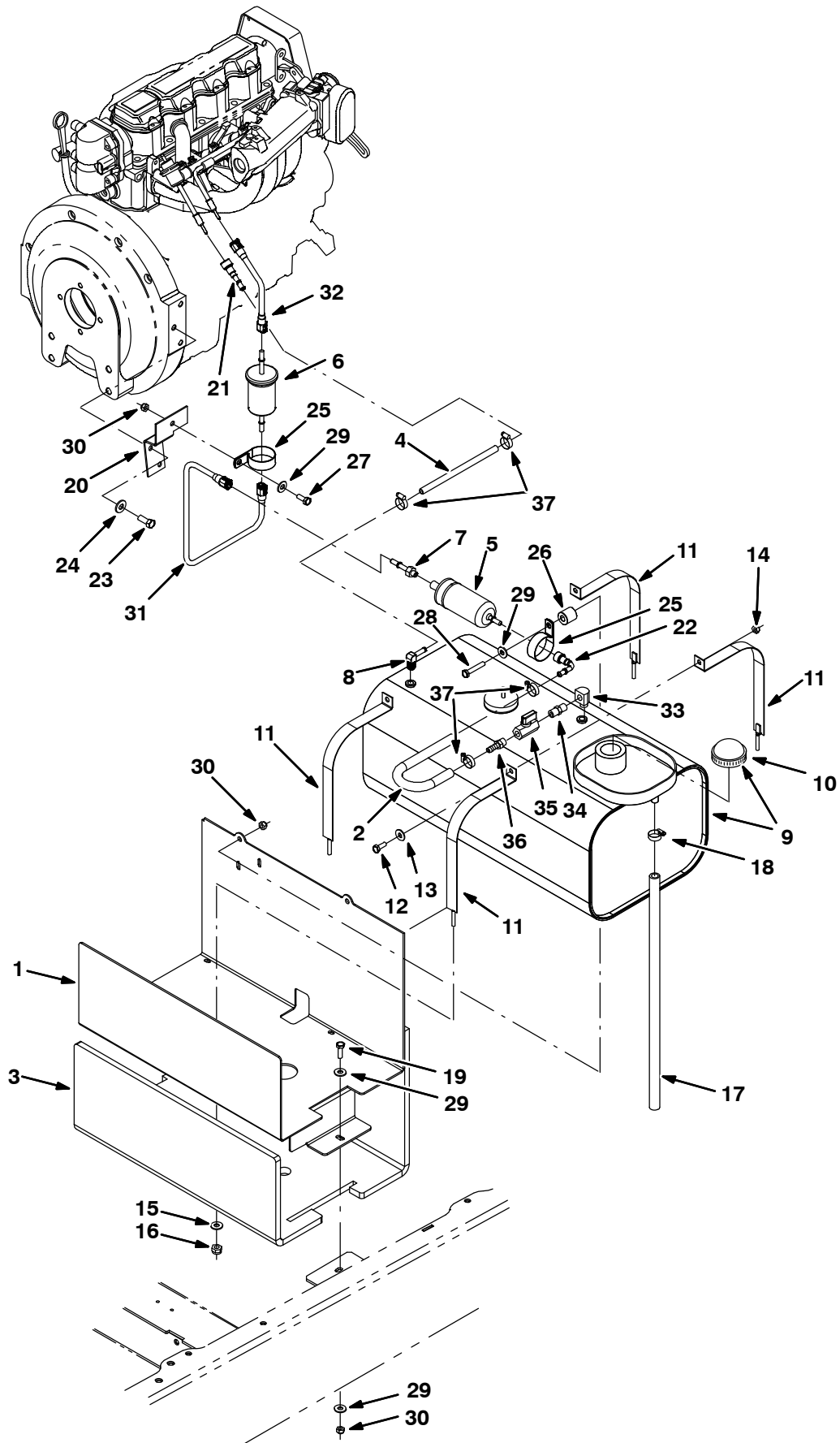
Fig. 19 – GM Engine Fuel Tank Group, Gasoline (0000–0043)
