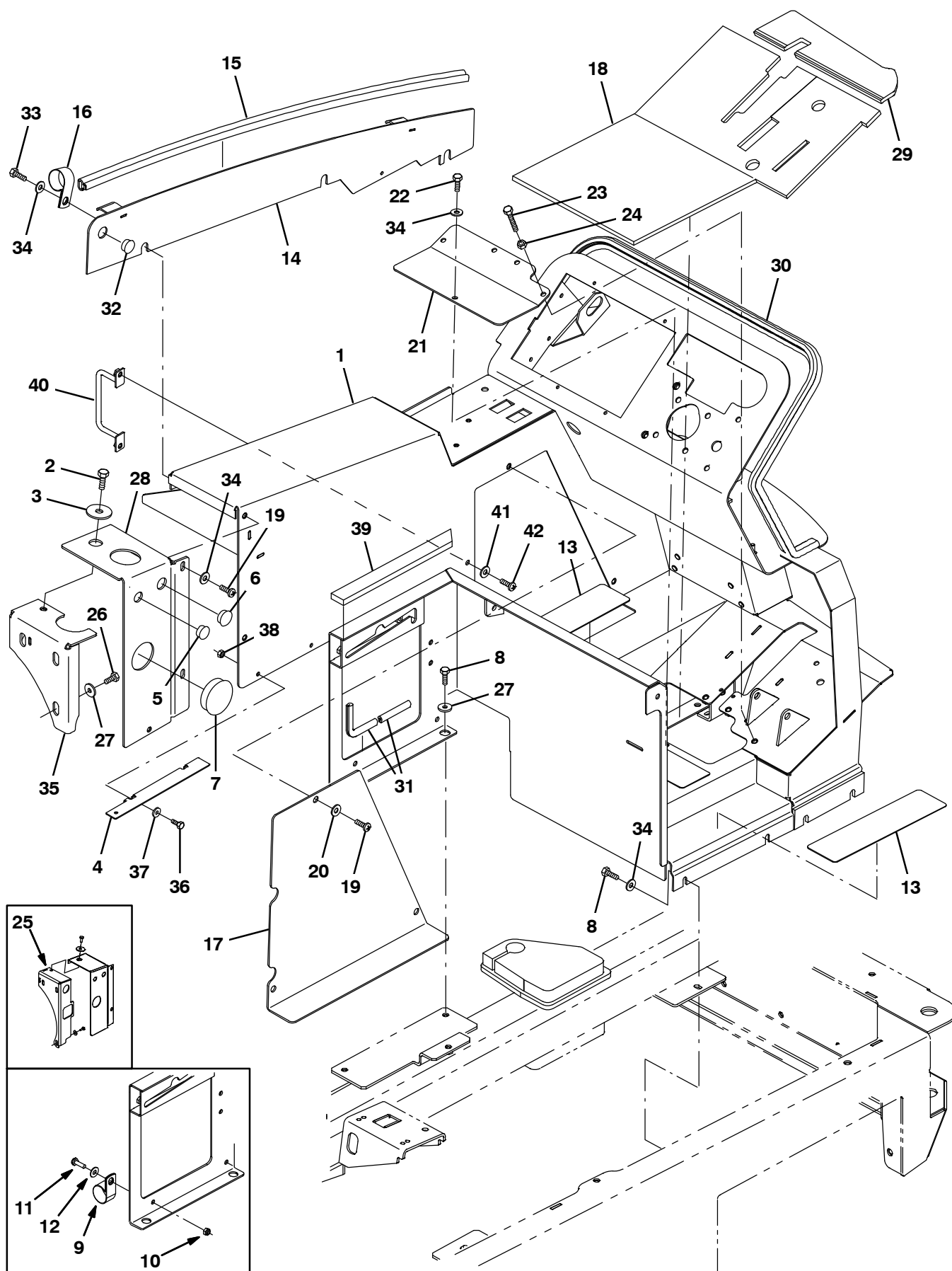
Fig. 4 – Operator Station
