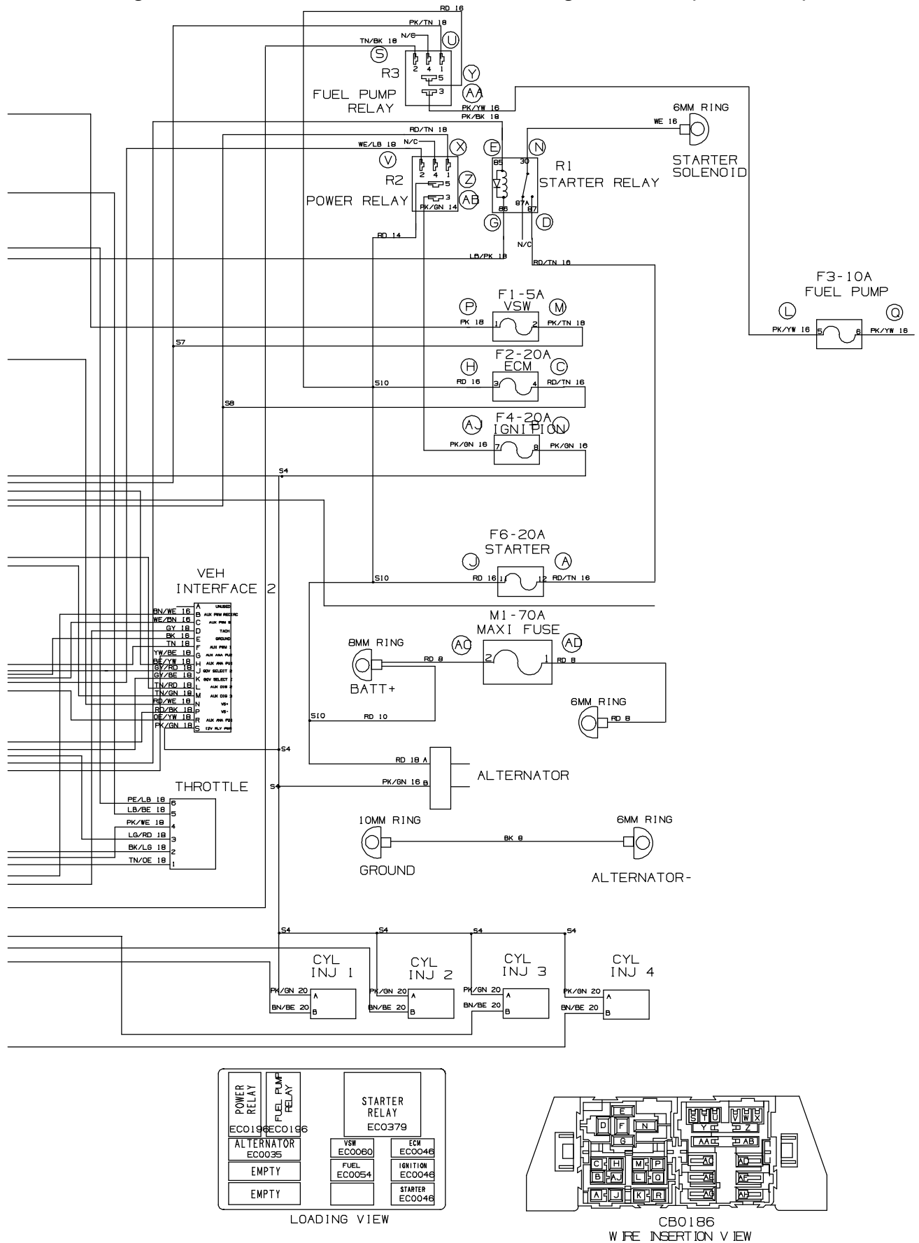
Fig. 92 – Mitsubishi Electrical Schematic, Gas Engine Harness (0500– )
