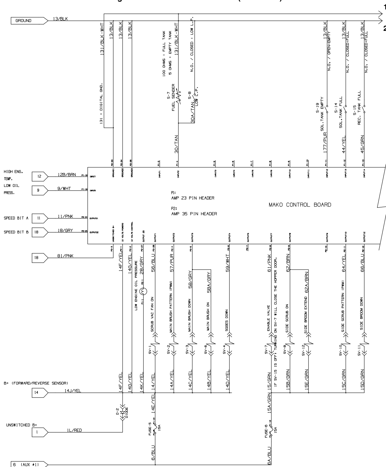
Fig. 85 – GM Electrical Schematic (0203-0499)
