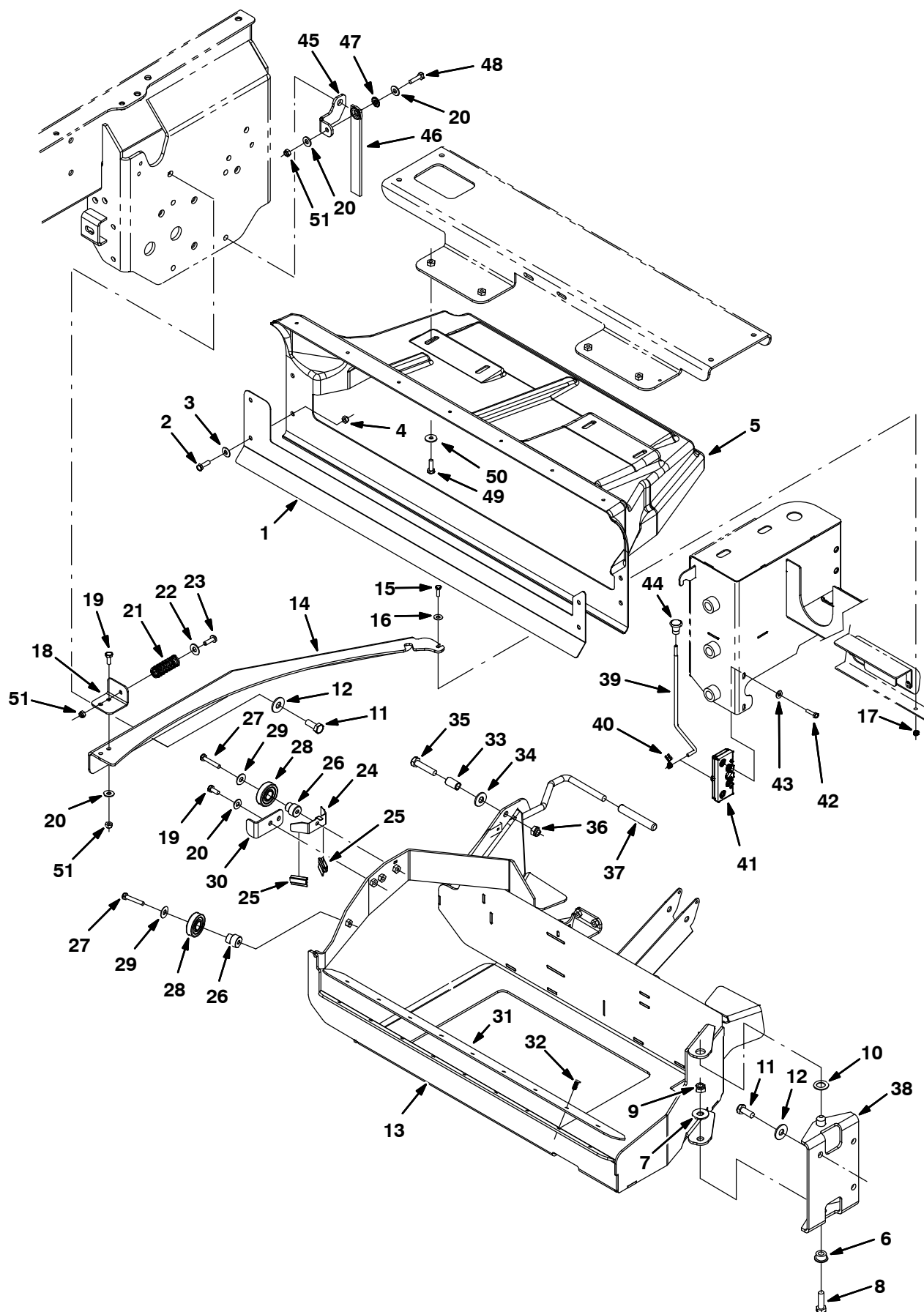
Fig. 54 – Cylindrical Scrub Head Debris Tray Mount Group
