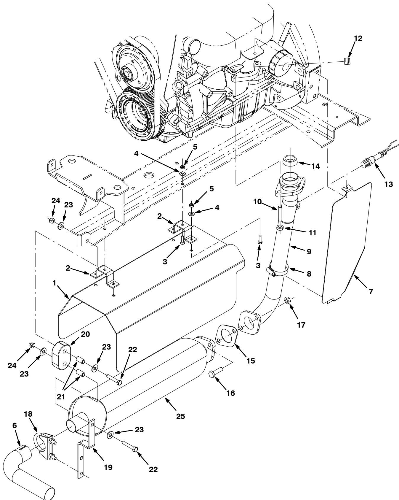
Fig. 25 – GM Engine Muffler Group (0000–0043)
