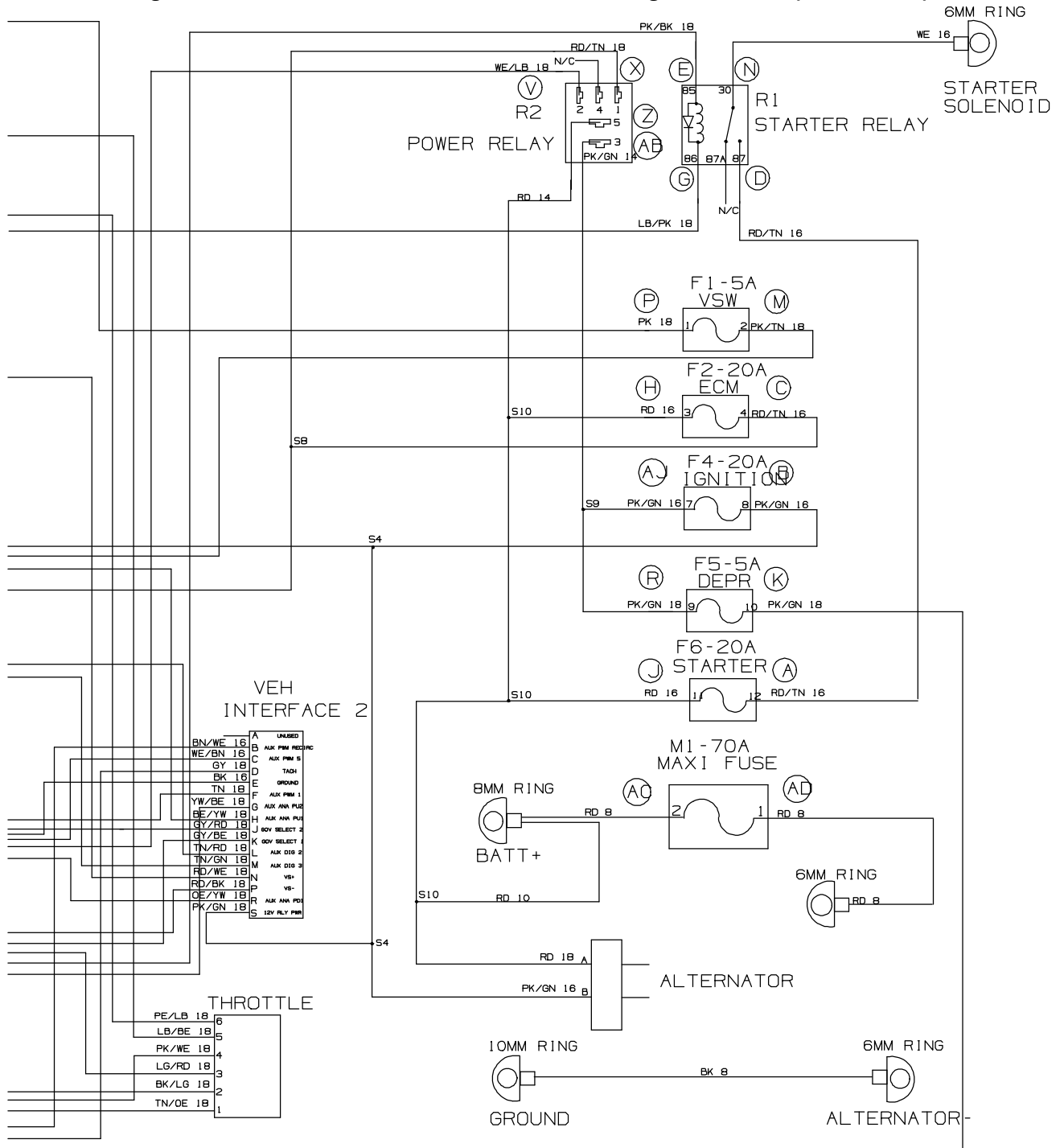
Fig. 93 – Mitsubishi Electrical Schematic, LPG Engine Harness (0500– )
