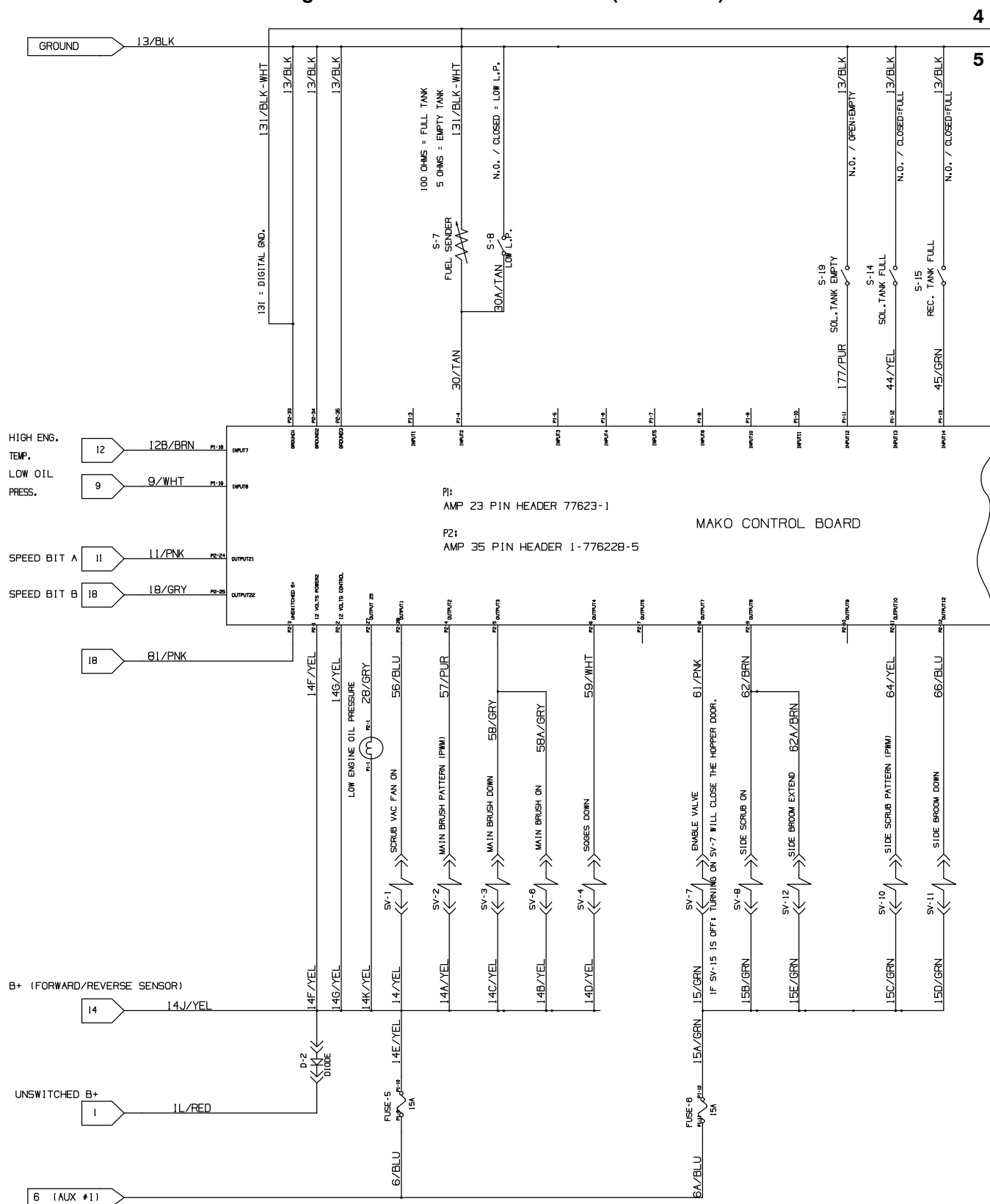
Fig. 84 – GM Electrical Schematic (0044-0202)
