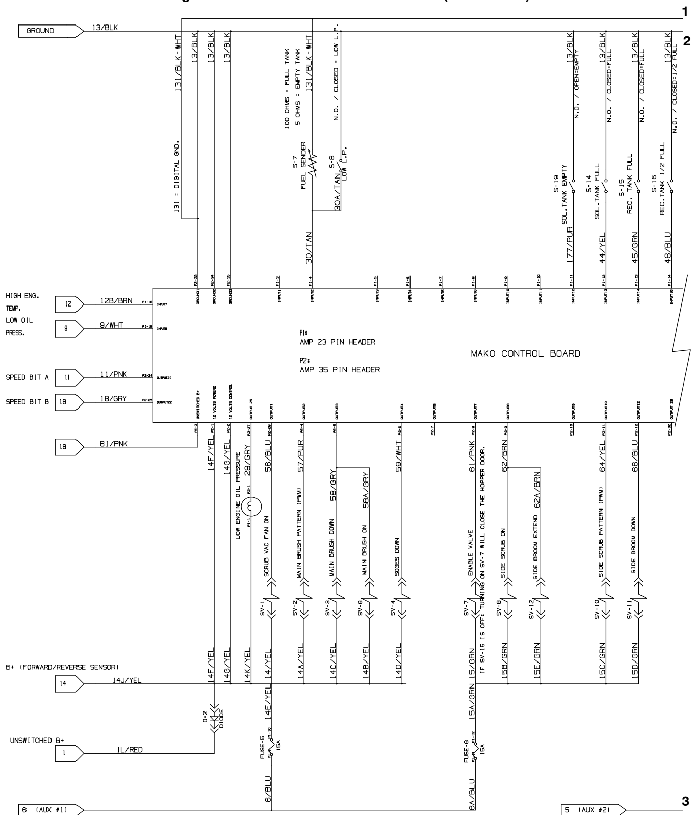
Fig. 91 – Mitsubishi Electrical Schematic (0500– )
