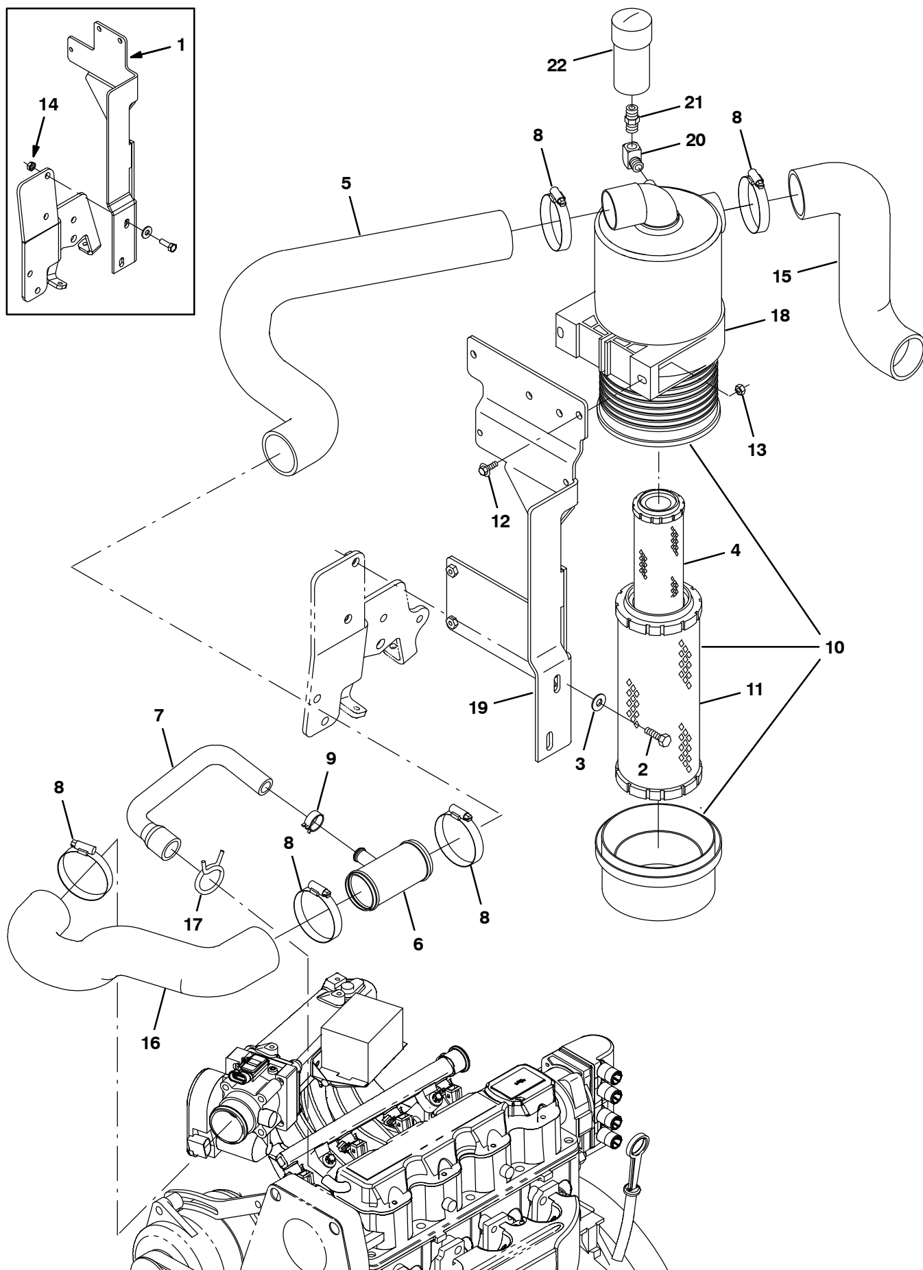
Fig. 21 – GM Engine Air Cleaner Group, Gasoline (0044–0499)
