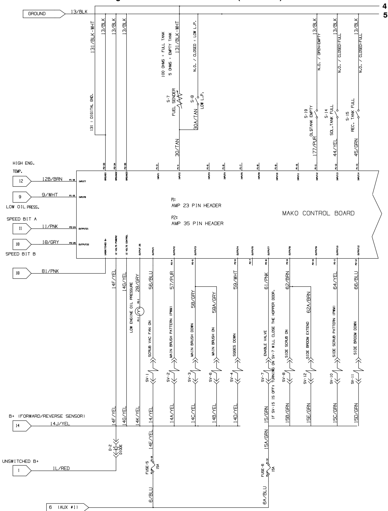
Fig. 83 – GM Electrical Schematic (0000–0043)
