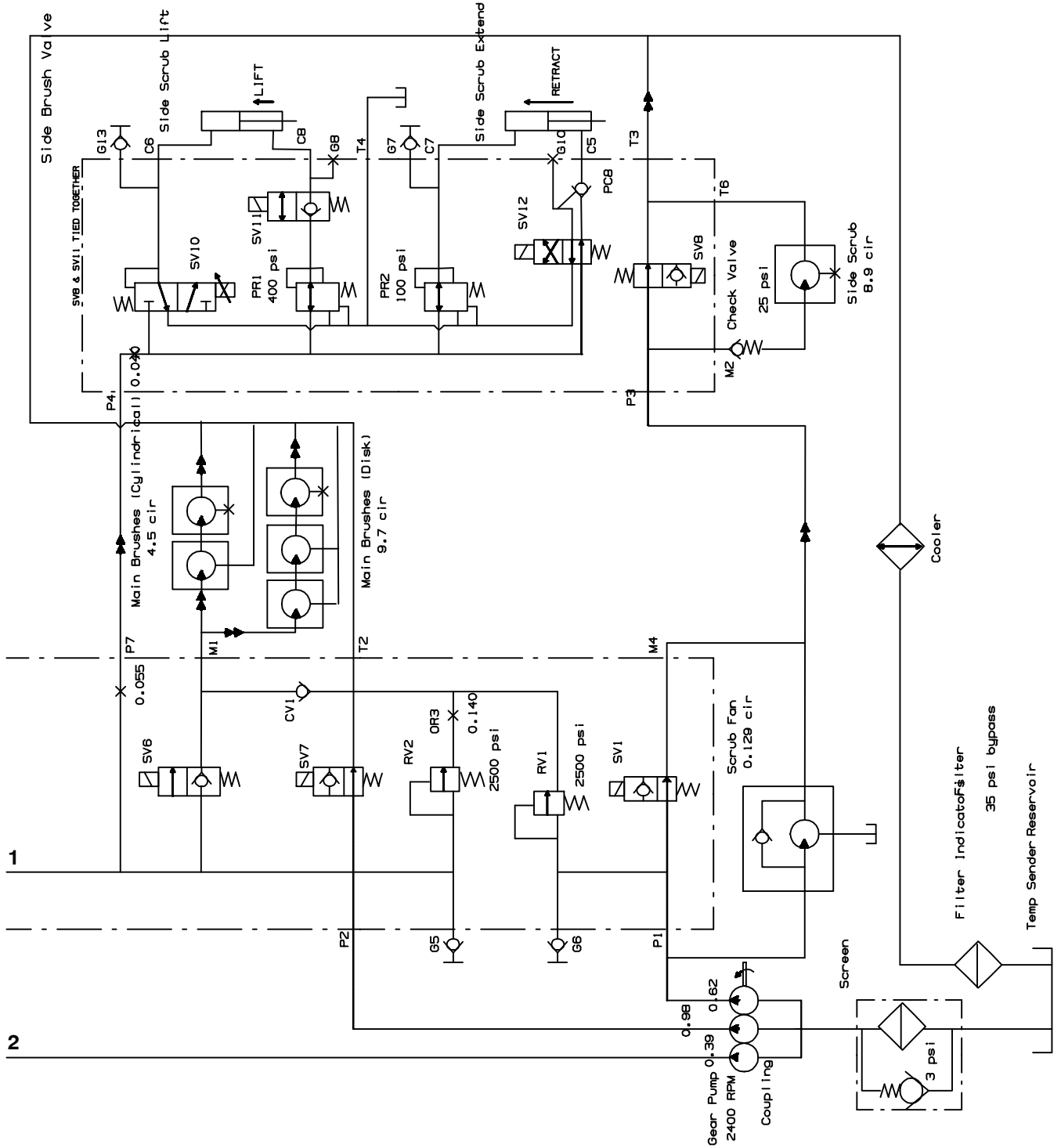
Fig. 73 – Hydraulic Schematic (0245- )
