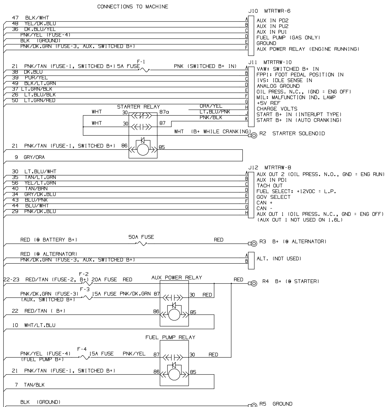
Fig. 86 – GM Electrical Schematic, Gasoline/LPG Engine Harness (0000–0043)
