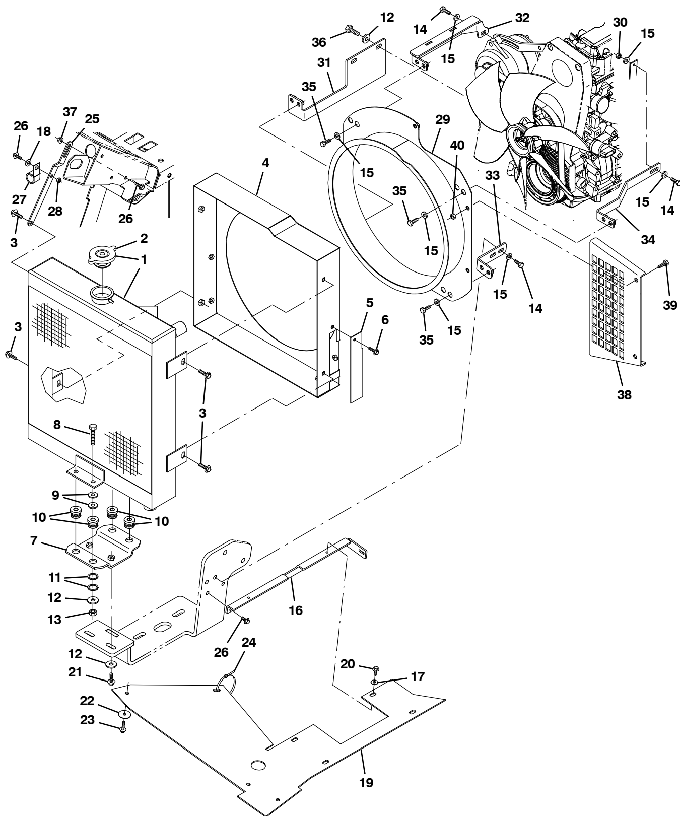
Fig. 28 – GM Engine Radiator and Mount Group (0189-0499)
