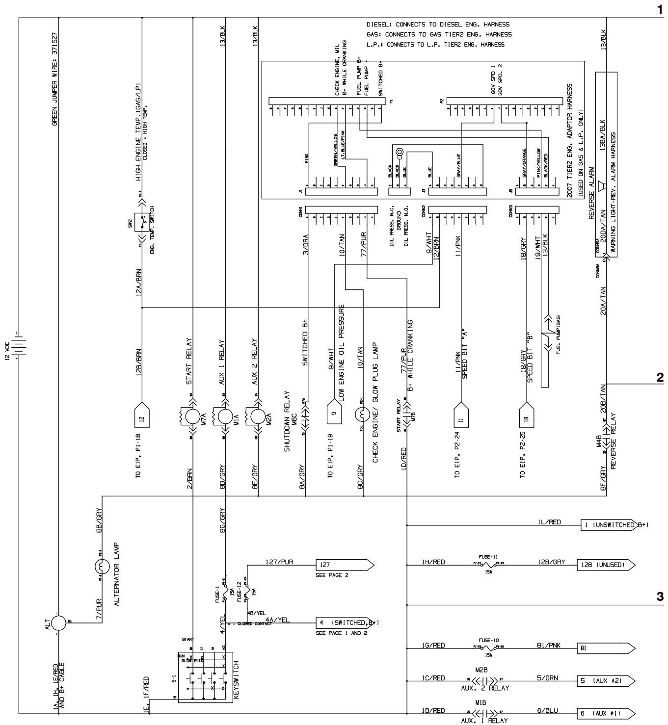
Fig. 84 – GM Electrical Schematic (0044-0202)
