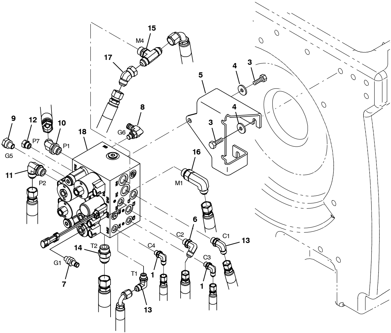
Fig. 82 – Hydraulic Valves Group
