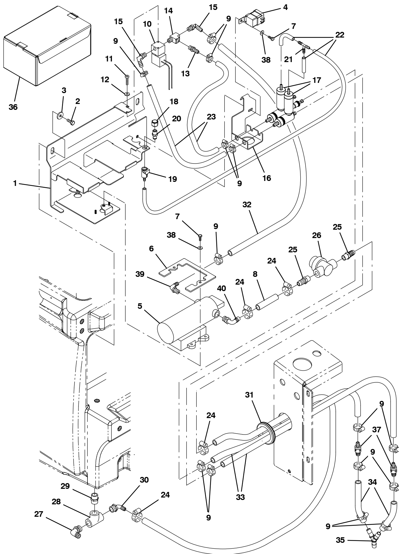
Fig. 16 – FaST Pumps and Detergent Group (0130– )
