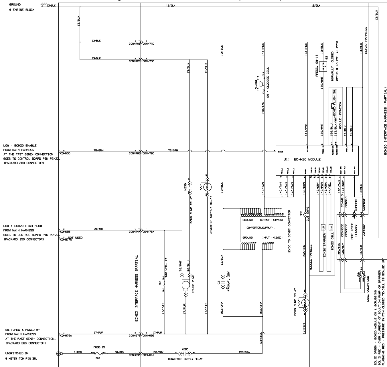
Fig. 85 – GM Electrical Schematic (0203-0499)
