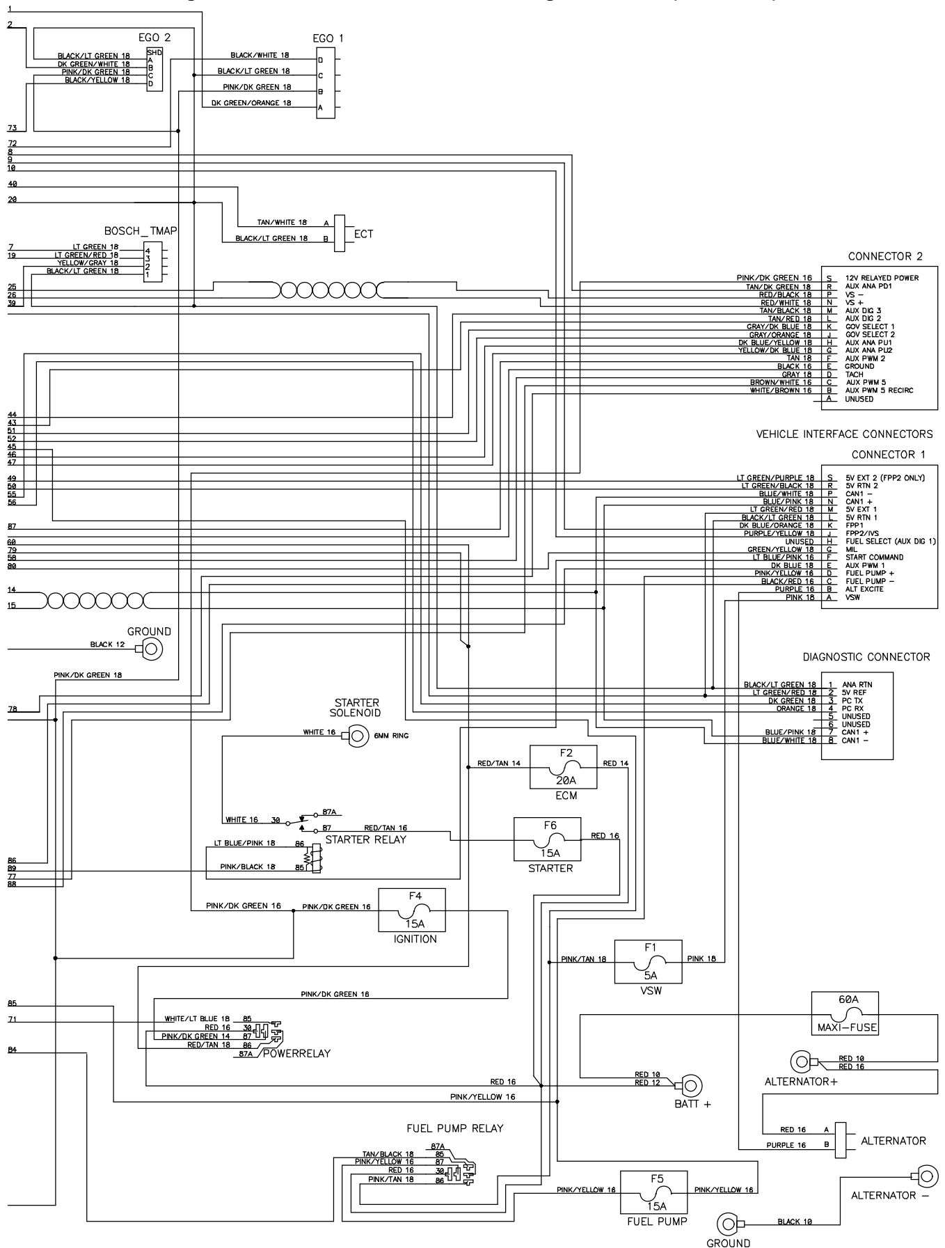
Fig. 87– GM Electrical Schematic, Gas Engine Harness (0044–0202)
