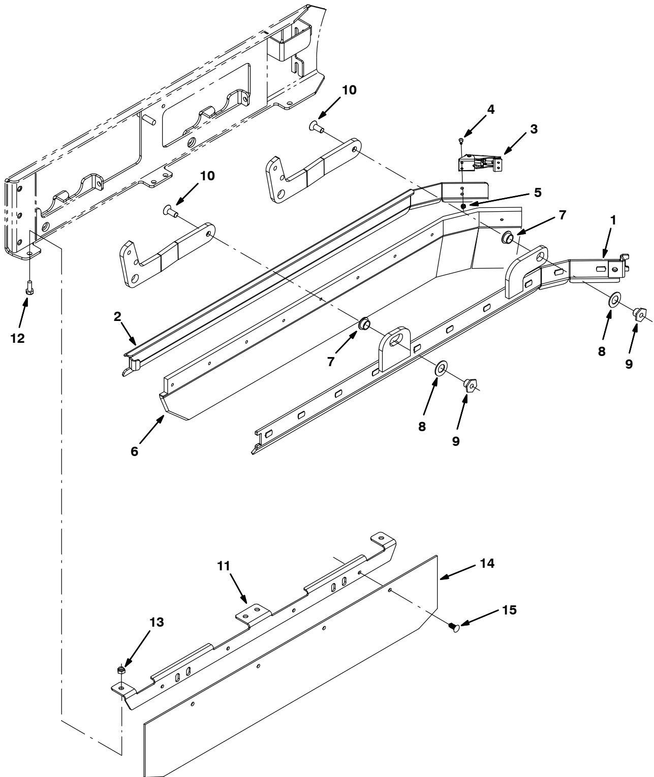
Fig. 59 – Cylindrical Scrub Head Squeegee Group, Right Side
