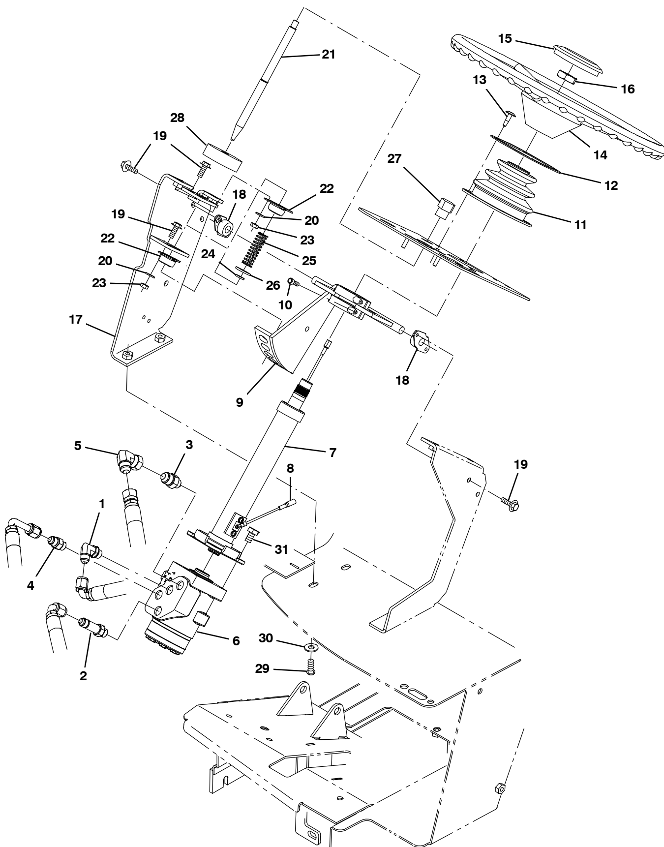
Fig. 8 – Steering Group
