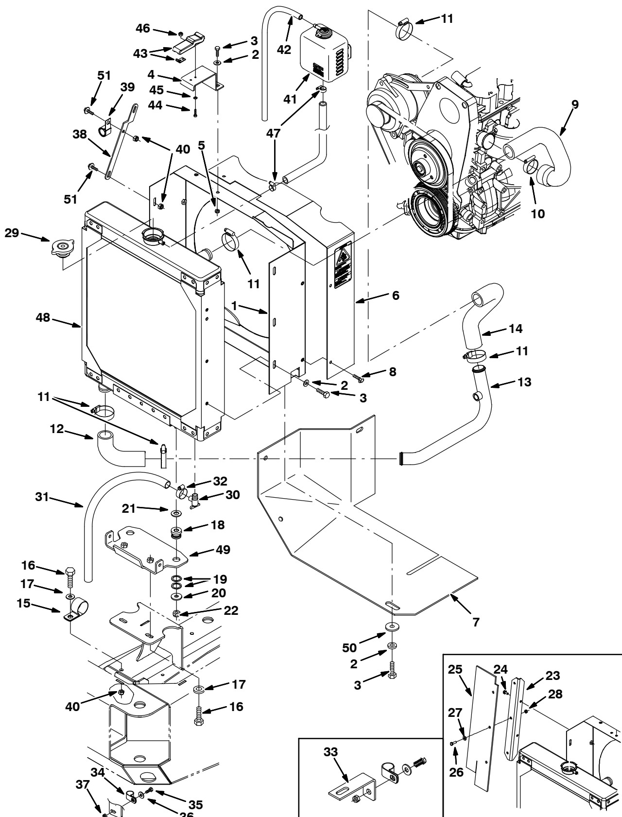
Fig. 27 – GM Engine Radiator Group (0000-0188)
