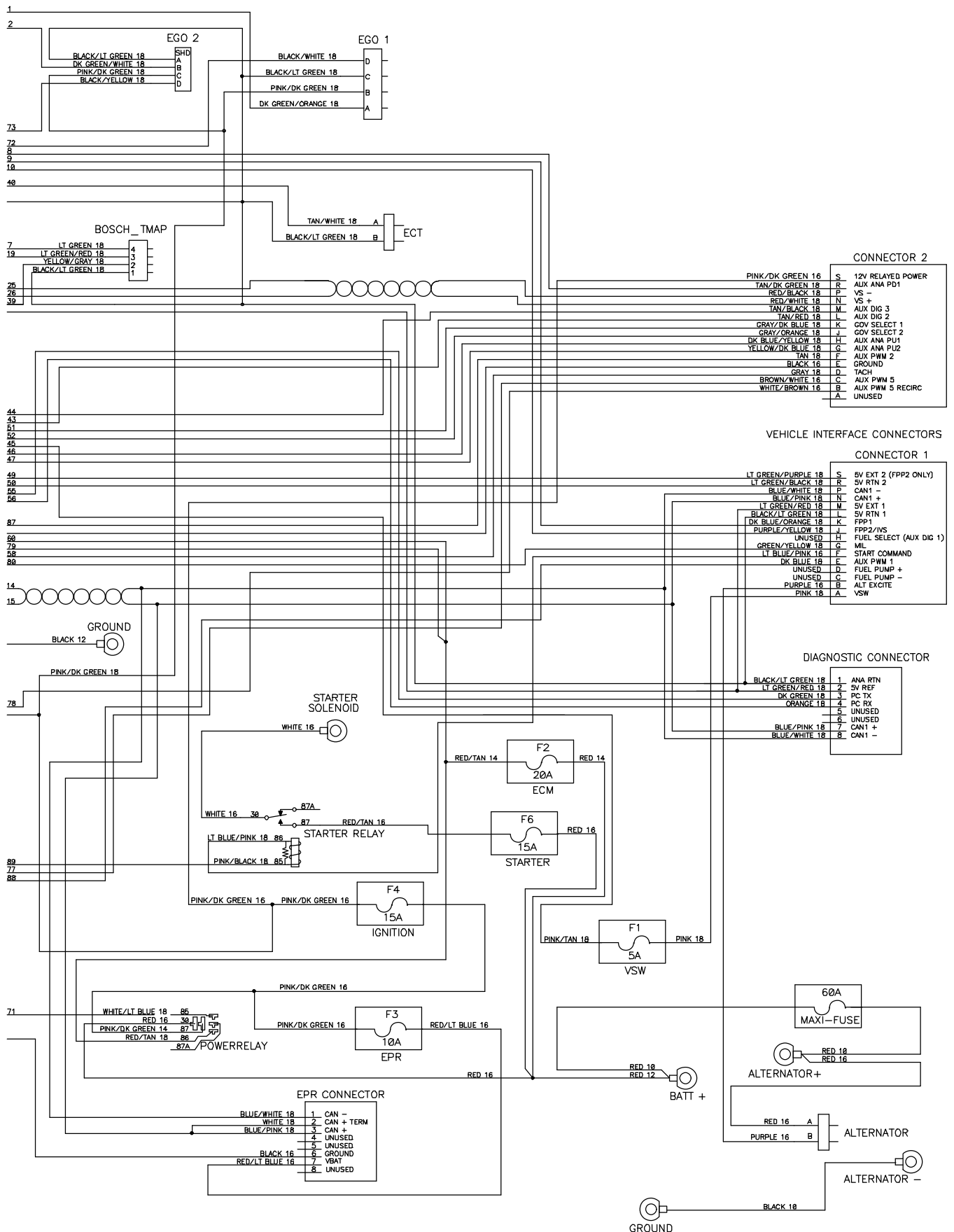
Fig. 89 – GM Electrical Schematic, LPG Engine Harness (0044–0202)
