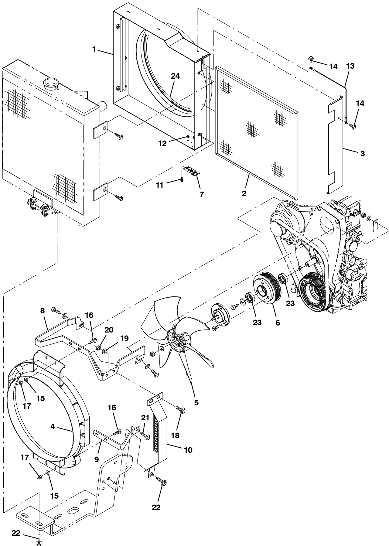
Fig. 40 – Engine Radiator Screen Kit (0203–0499)
