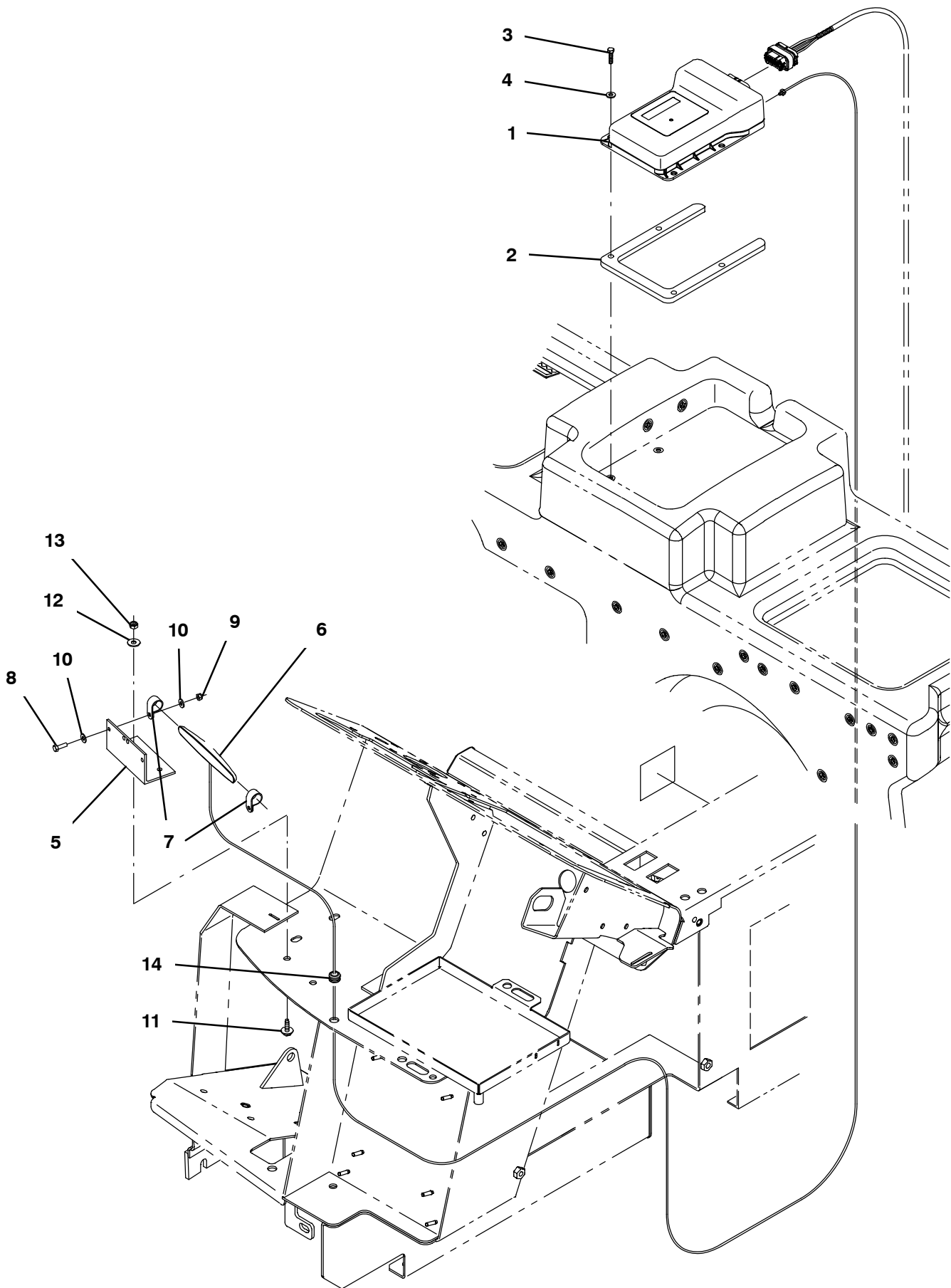
Fig. 41 – Telemetry Group
