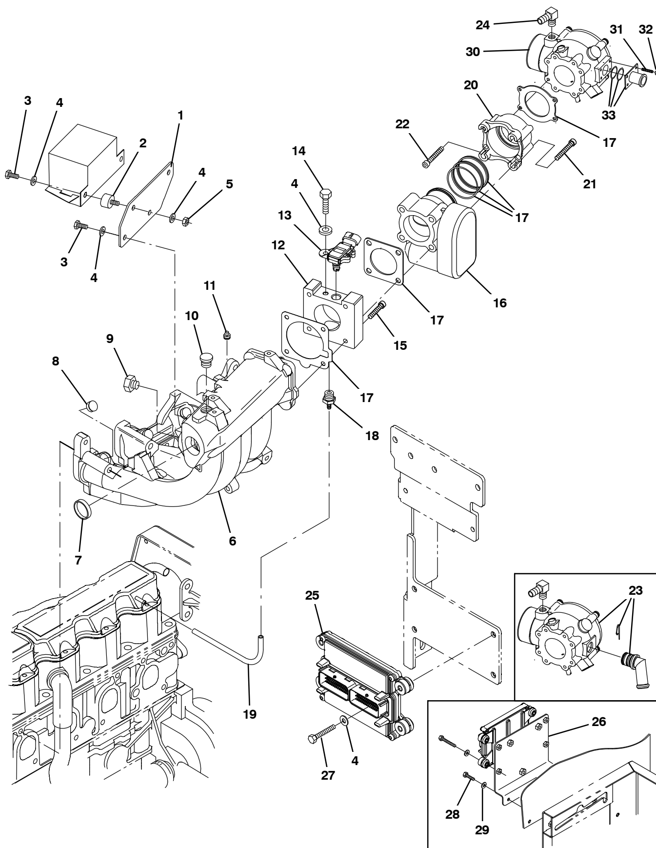
Fig. 16 – GM Engine EFI Group, LPG (0044–0499)
