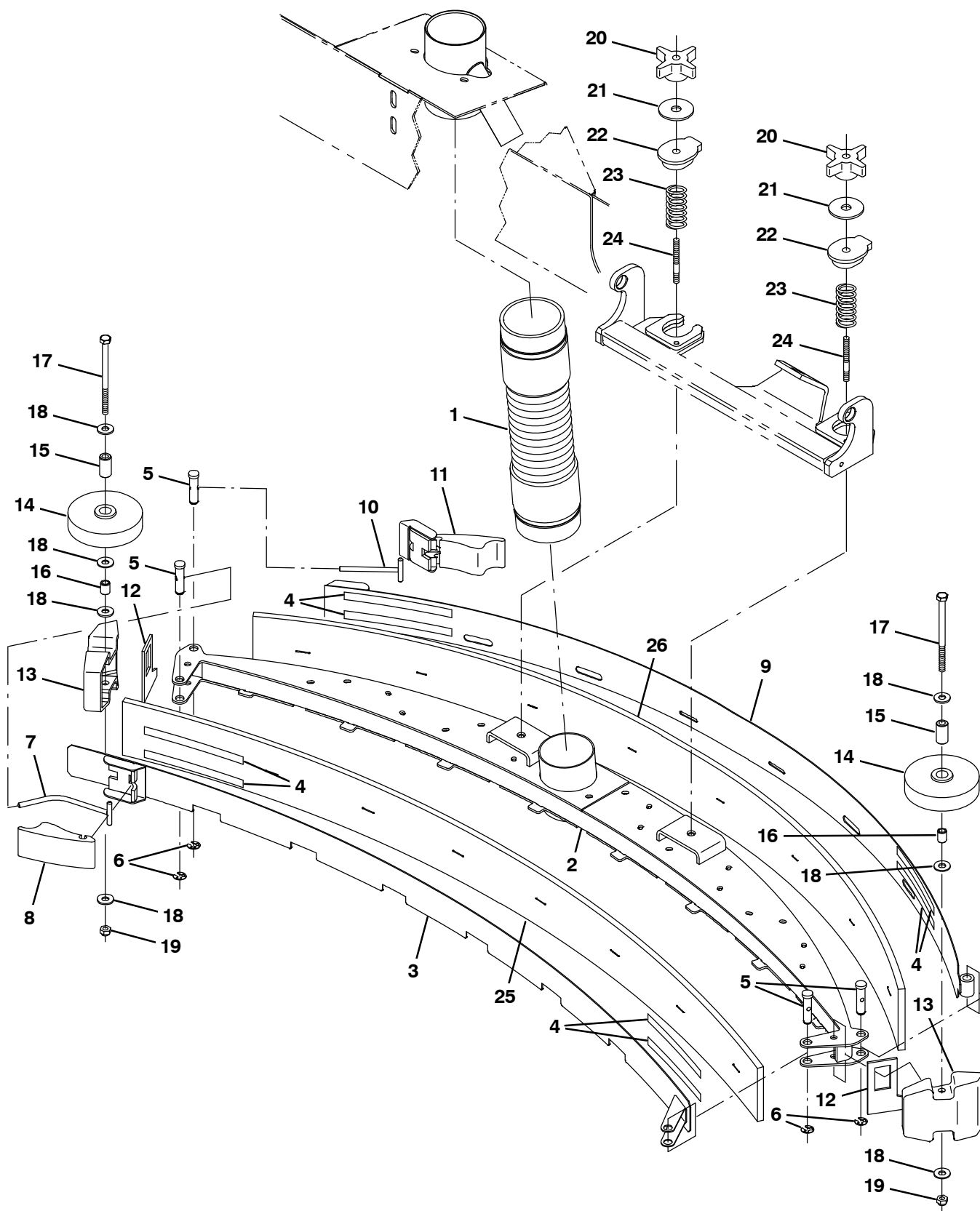
Fig. 57 – Squeegee Group, Rear
