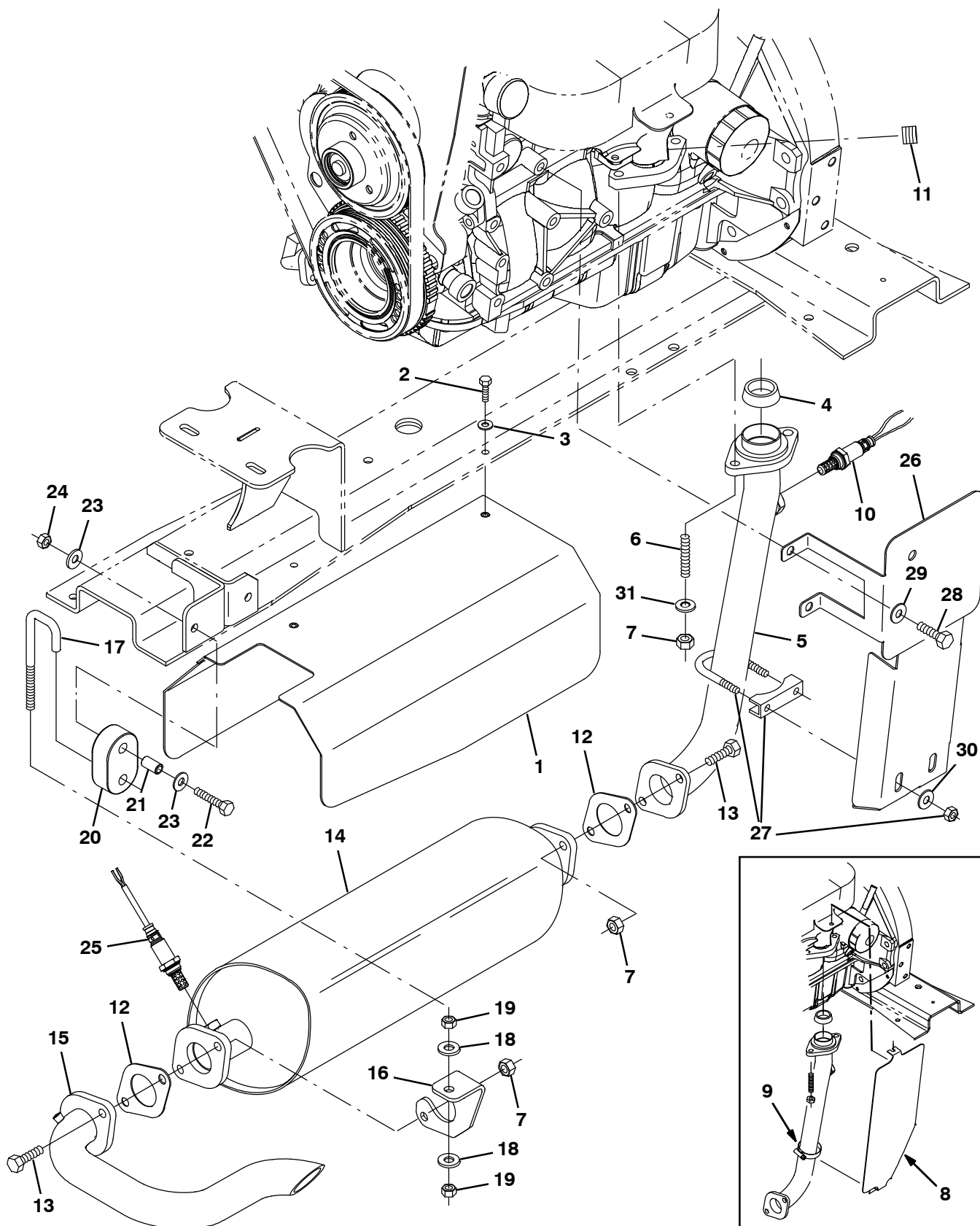
Fig. 26 – GM Engine Muffler Group (0044–0499)
