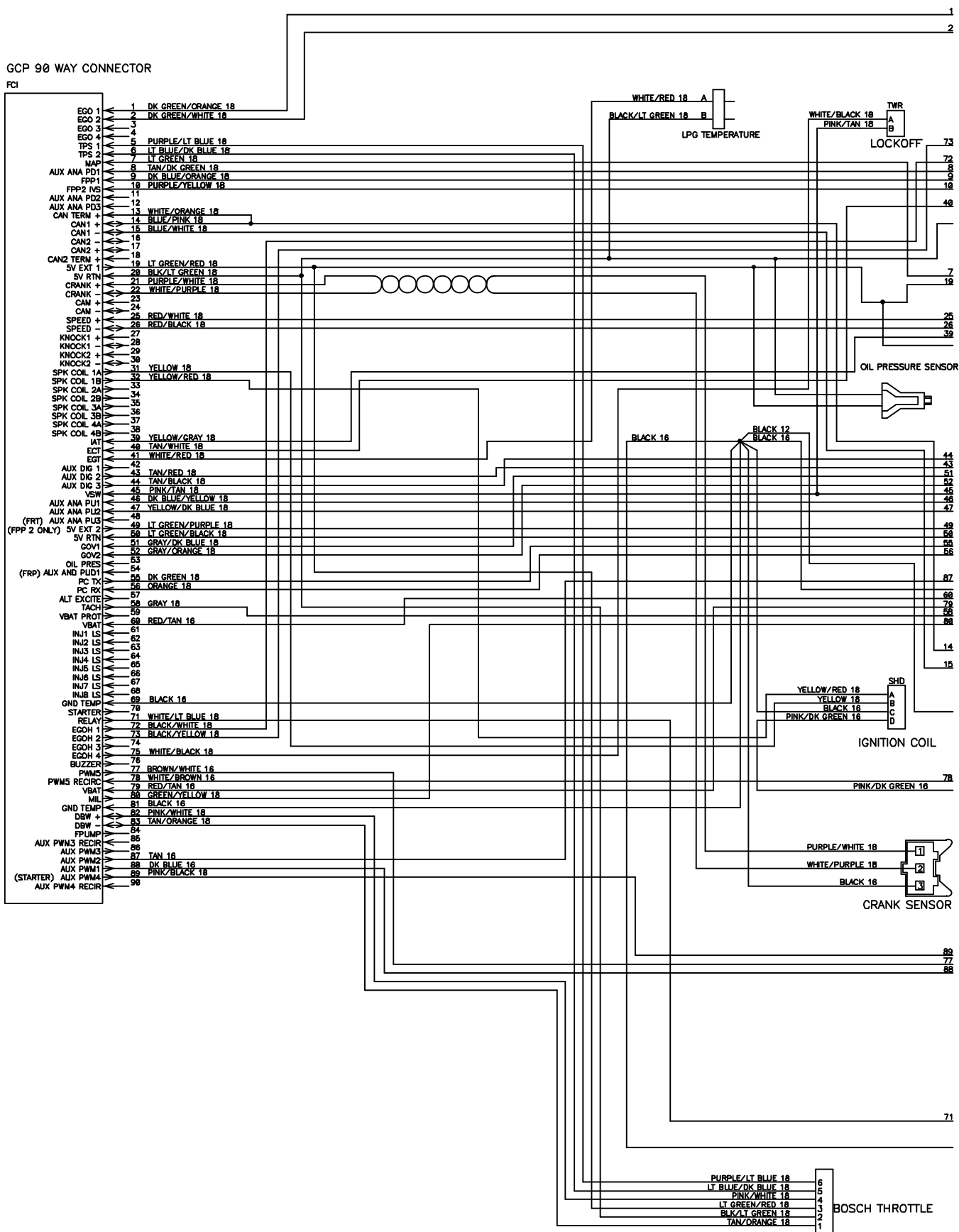
Fig. 90 – GM Electrical Schematic, LPG Engine Harness (0203–0499)
