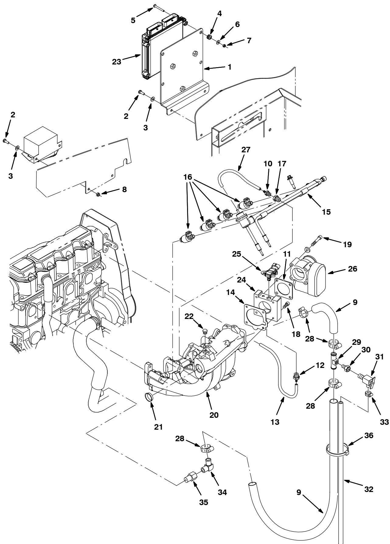
Fig. 12 – GM Engine EFI Group, Gasoline (0000–0043)
