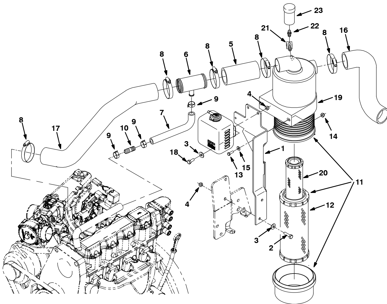
Fig. 22 – GM Engine Air Cleaner Group, LPG (0000–0043)
