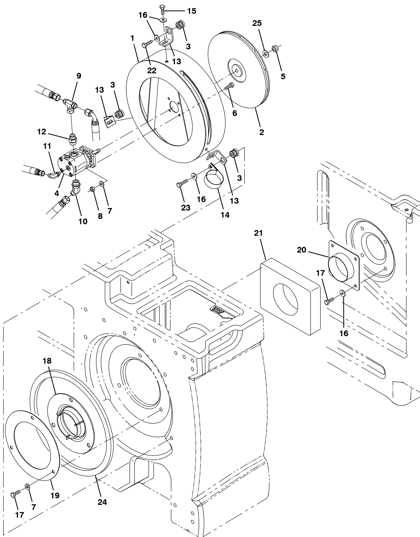
Fig. 70 – Vacuum Fan Group, Scrubbing (0779– )
