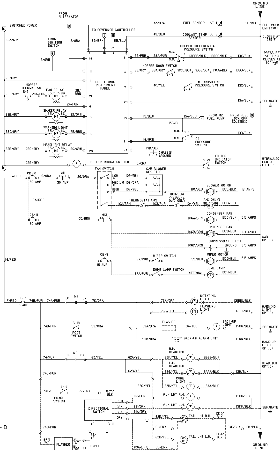
Fig. 60 - Electrical Schematic (004303-006008)
