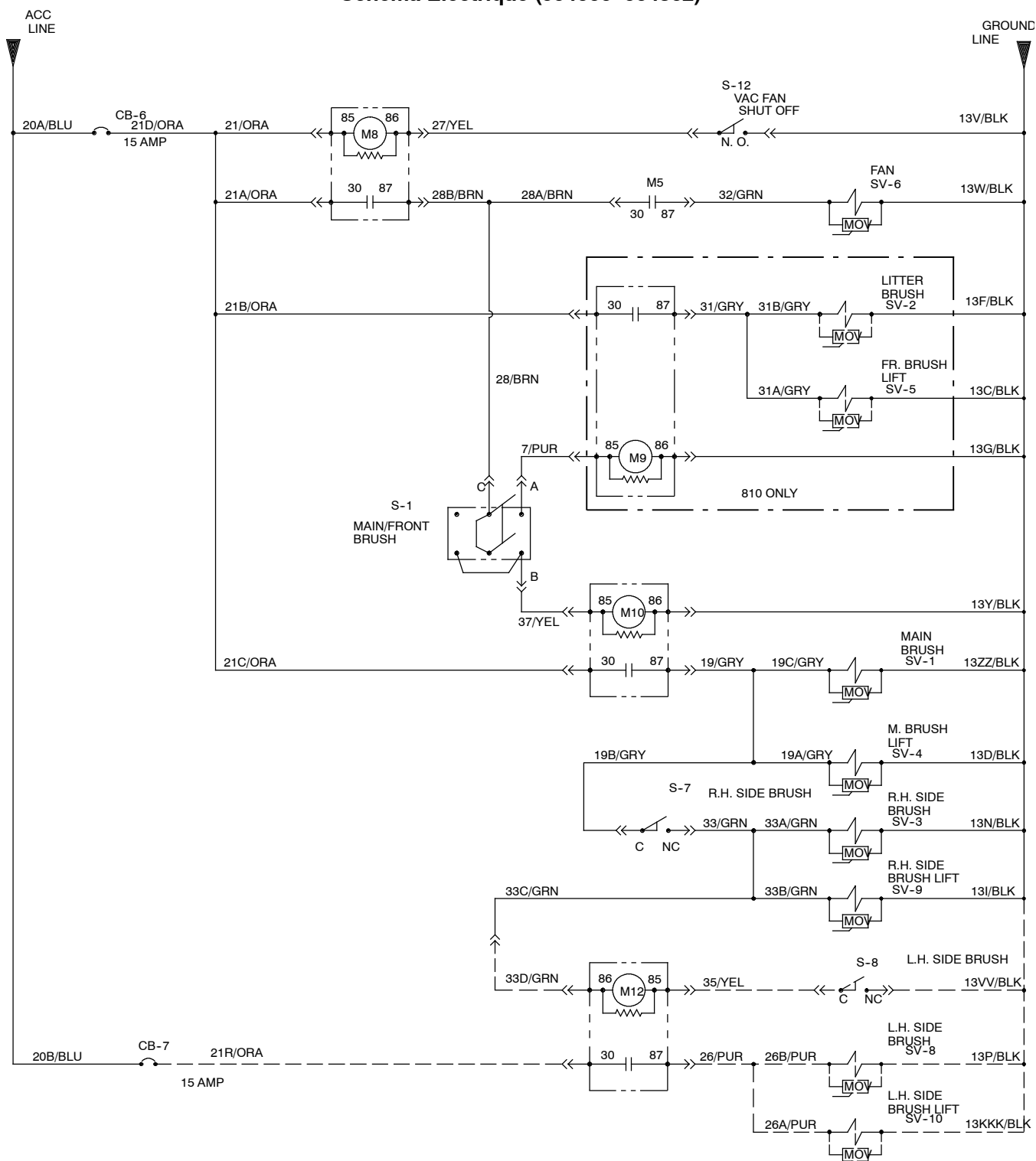
Fig. 59 - Electrical Schematic (004000-004302)
