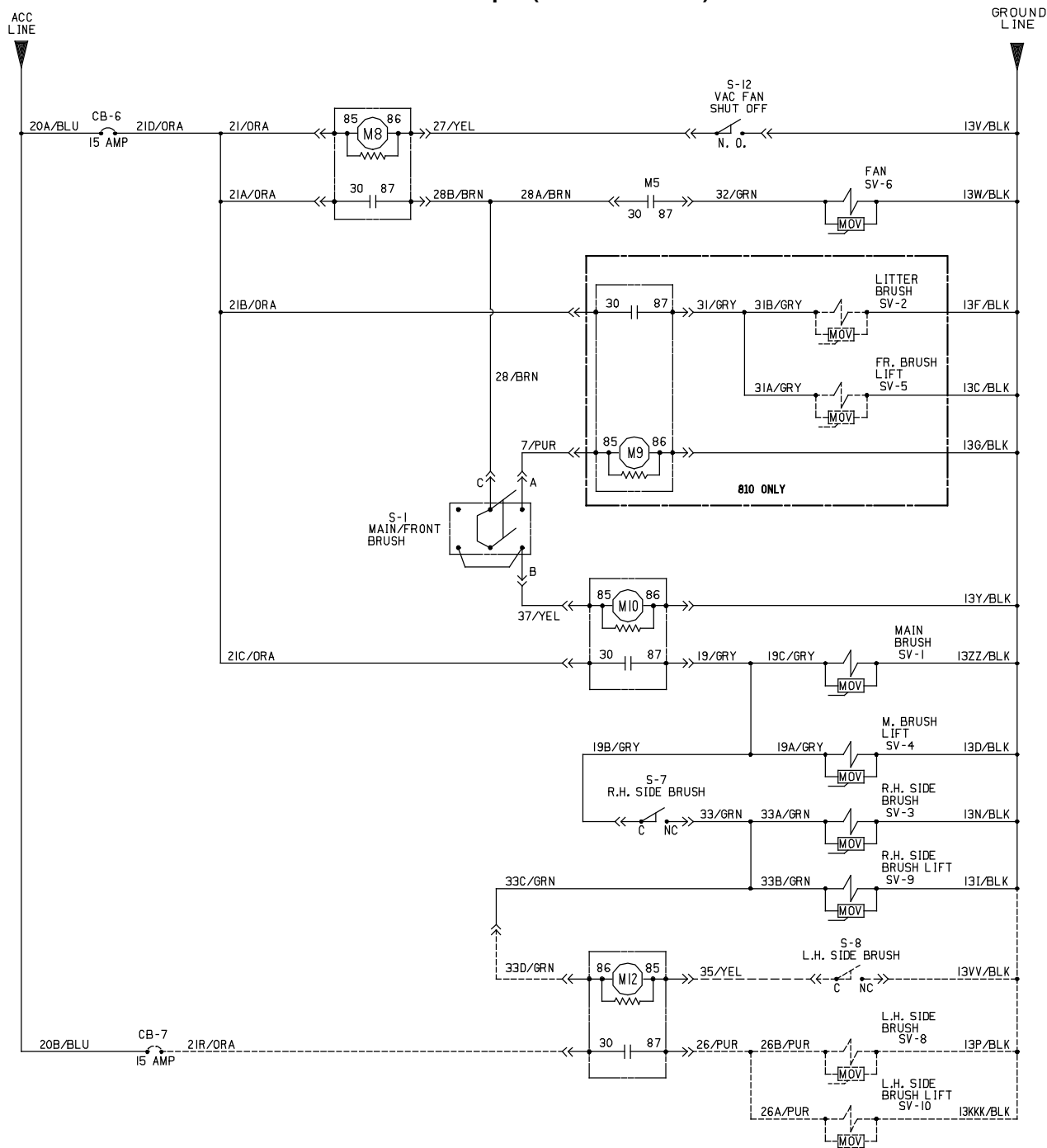
Fig. 60 - Electrical Schematic (004303-006008)
