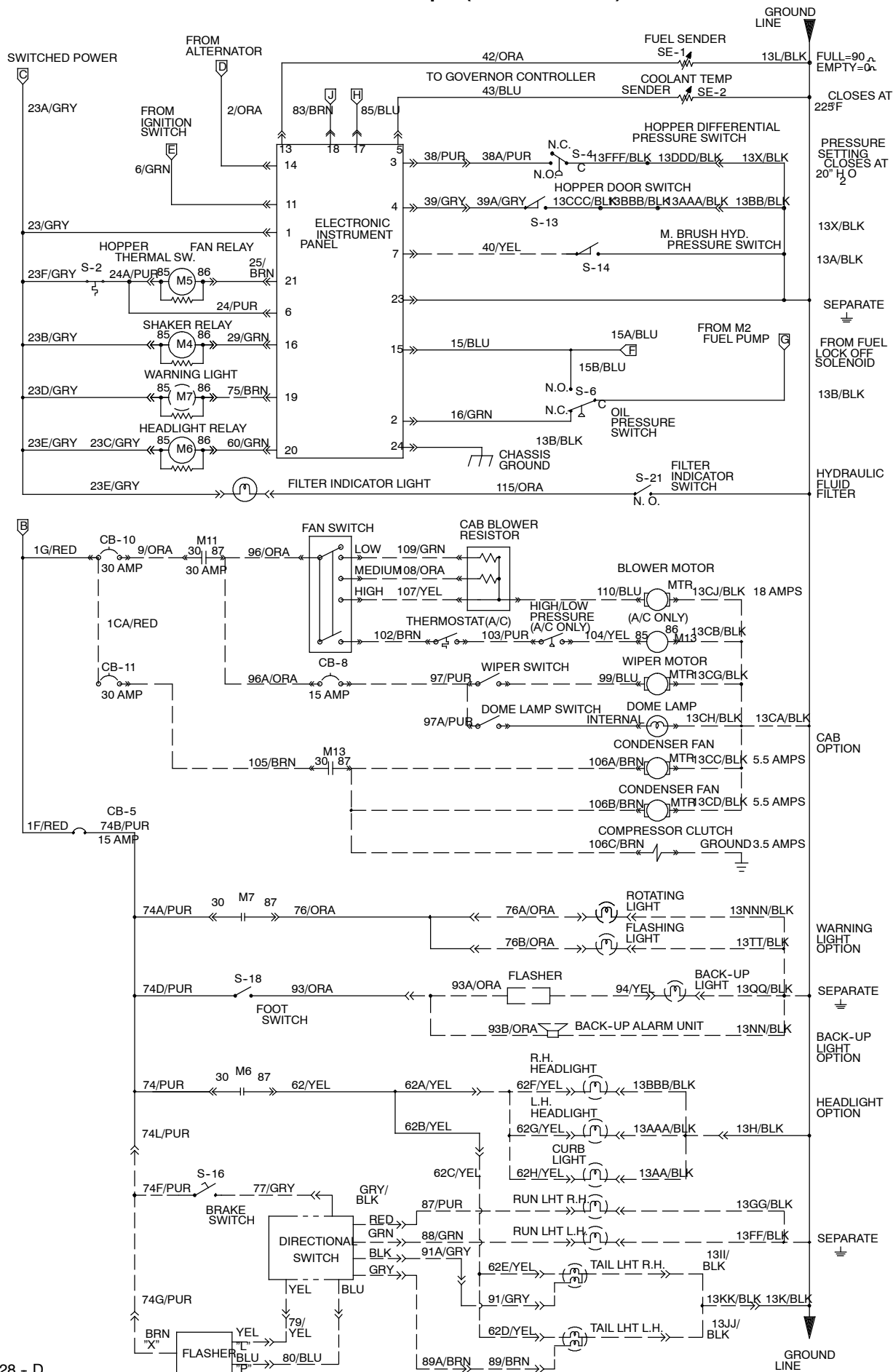
Fig. 59 - Electrical Schematic (004000-004302)
