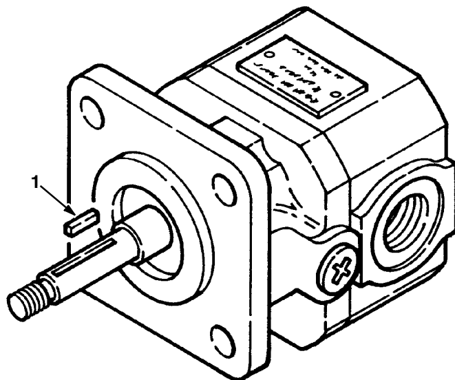
Fig. 18 - Hydraulic Motor Breakdown, 19117 — Hydraulik-Motor-Komponente — Composantes moteur hydraulique
