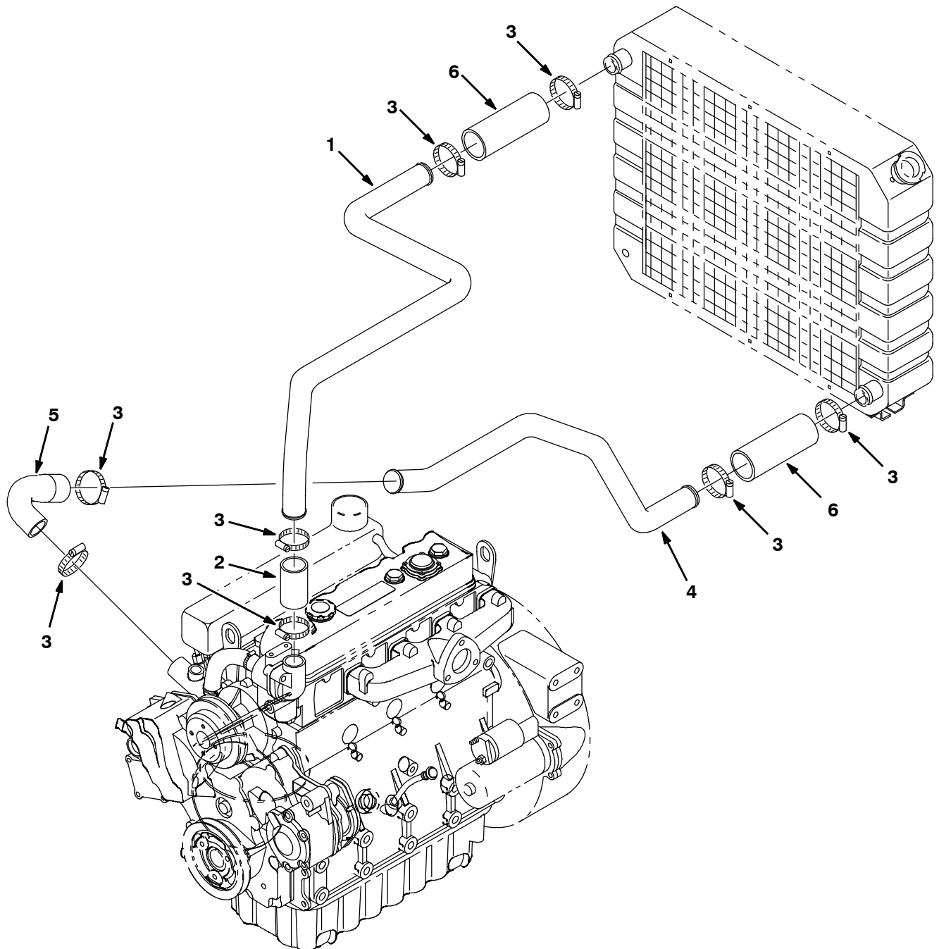
Fig. 30 - Radiator Hose Group (004000-006008) Kühler-Schlauch-gruppe (004000-006008) Groupe Durite radiateur (004000-006008)
