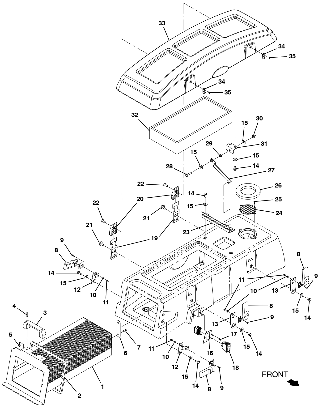
Fig. 50 – Dry Vacuum Debris Tray and Filter Group (0562– )
