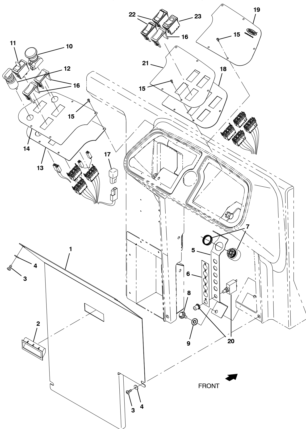
Fig. 9 – Instrument Panel Group
