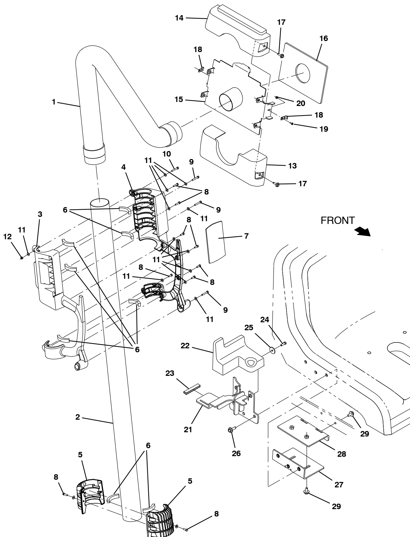
Fig. 47 – Dry Vacuum Wand Group (0562– )
