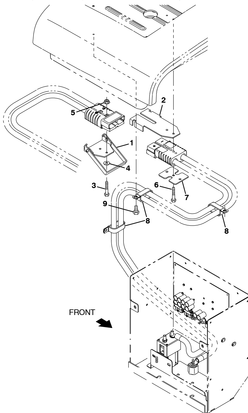
Fig. 54 – Battery Quick Disconnect Group (0500– )
