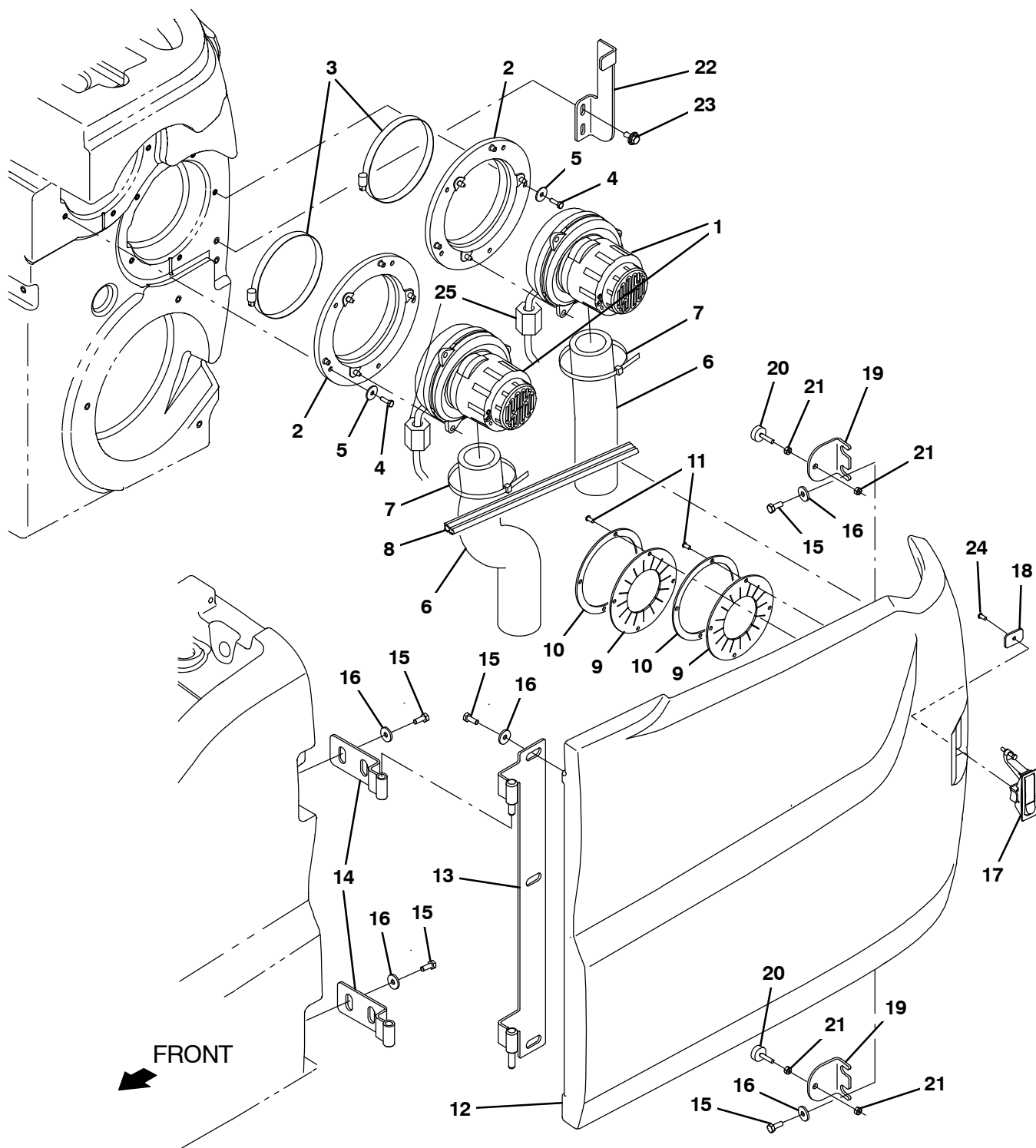
Fig. 45 – Vacuum Fans and Rear Side Door Group
