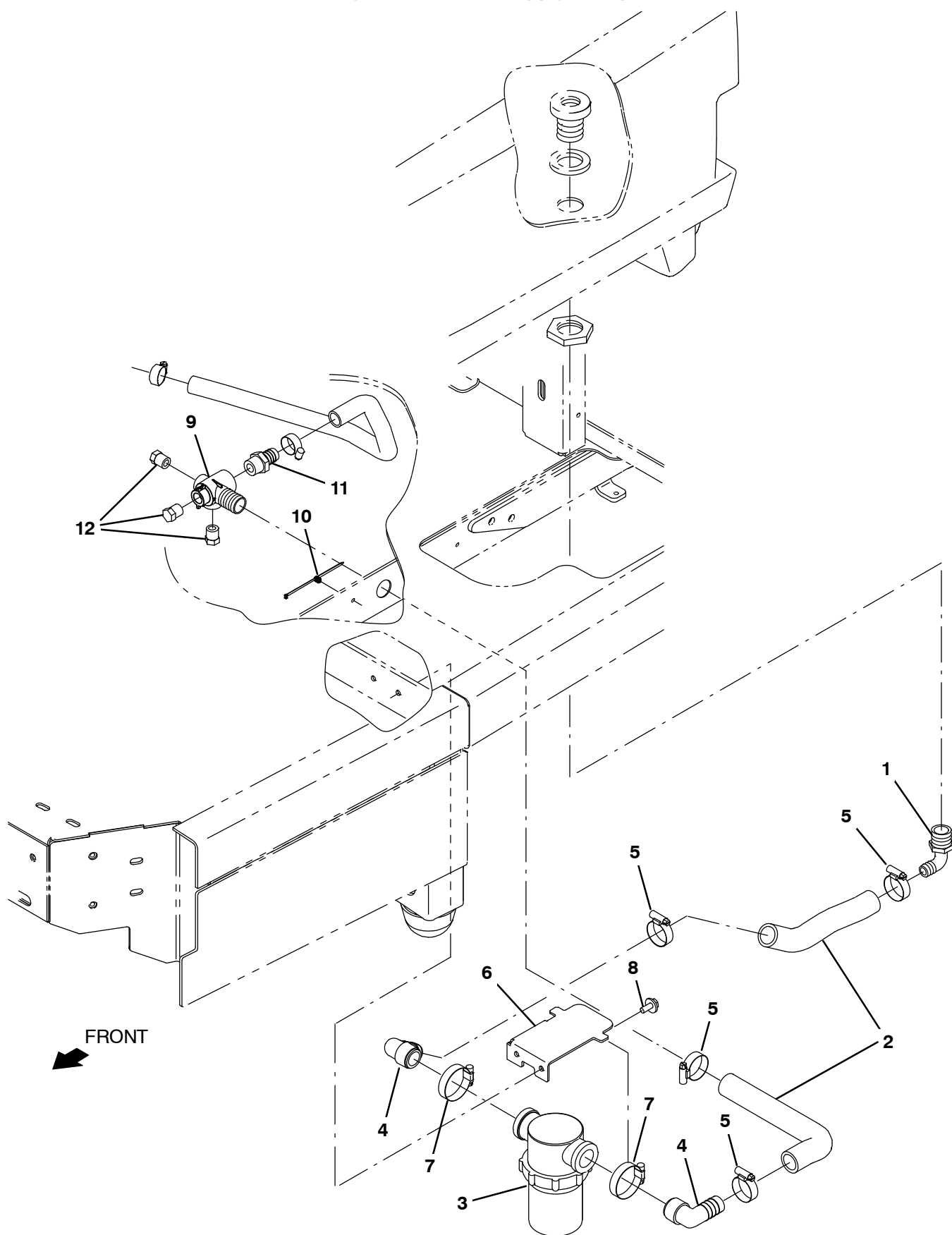
Fig. 42 – Solution Supply Group
