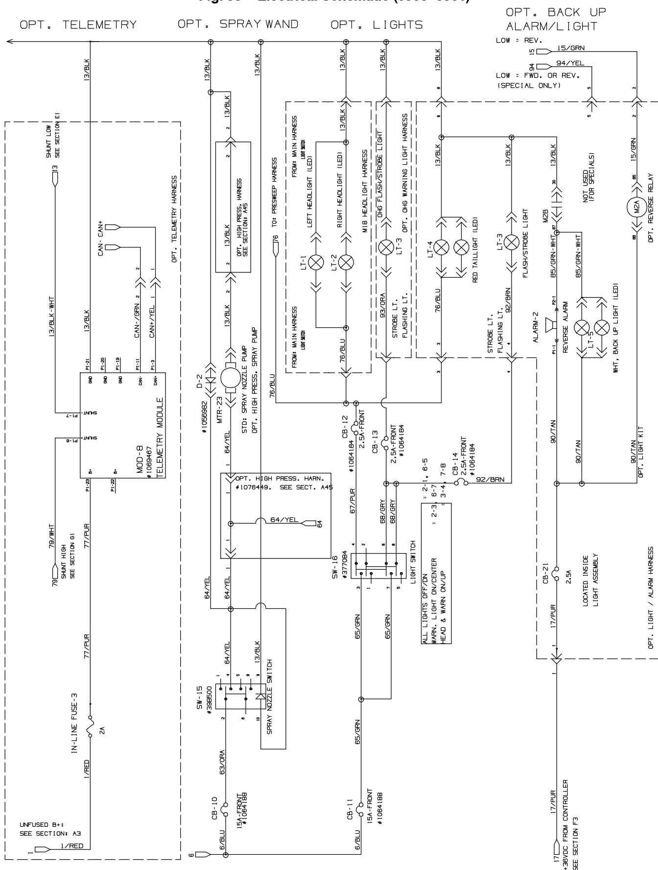
Fig. 55 – Electrical Schematic (0500–0561)
