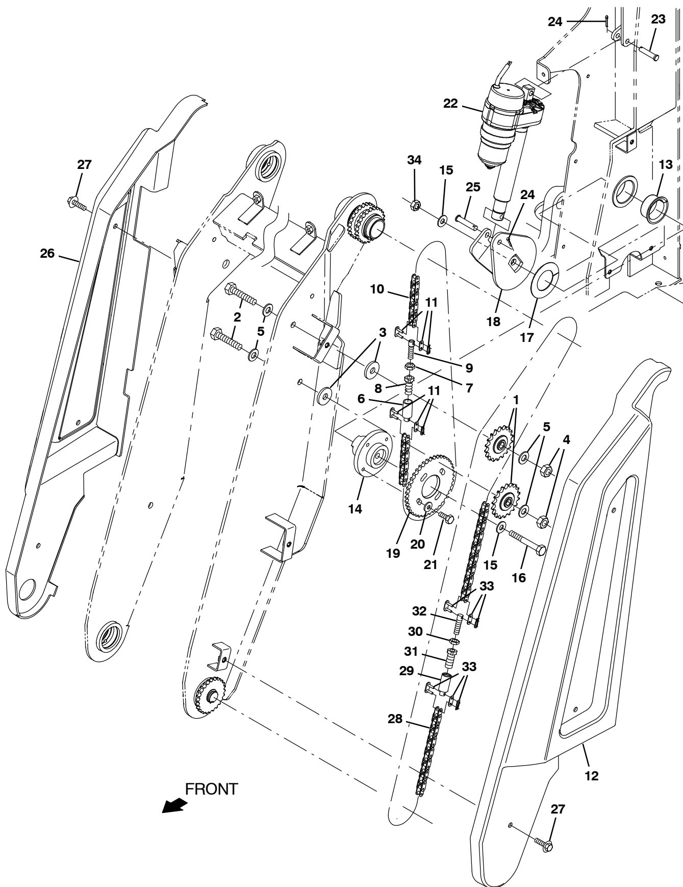
Fig. 36 – Hopper Chain Roller and Cover Group
