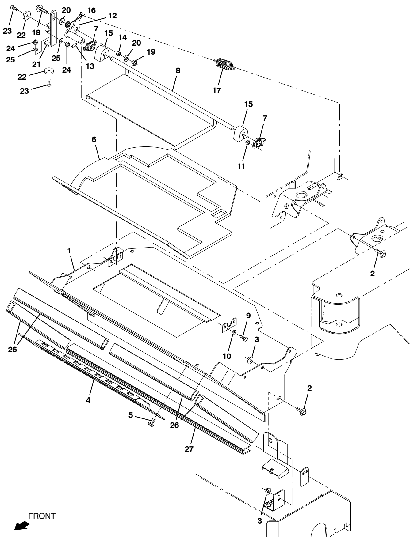
Fig. 40 – Steel Hopper Pre-Filter and Dump Door Group (0500– )
