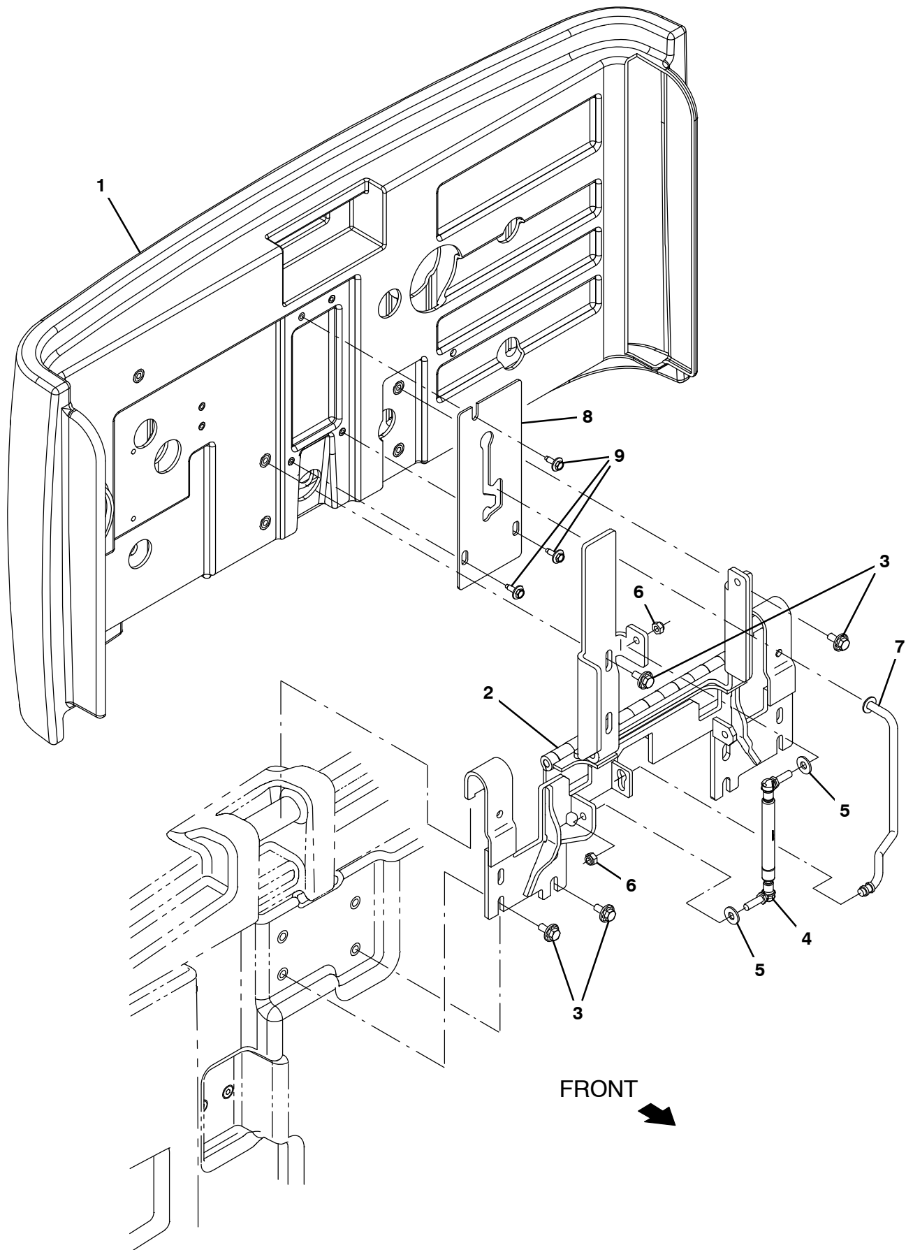
Fig. 48 – Dry Vacuum Rear Cover and Hinge Group (0562– )
