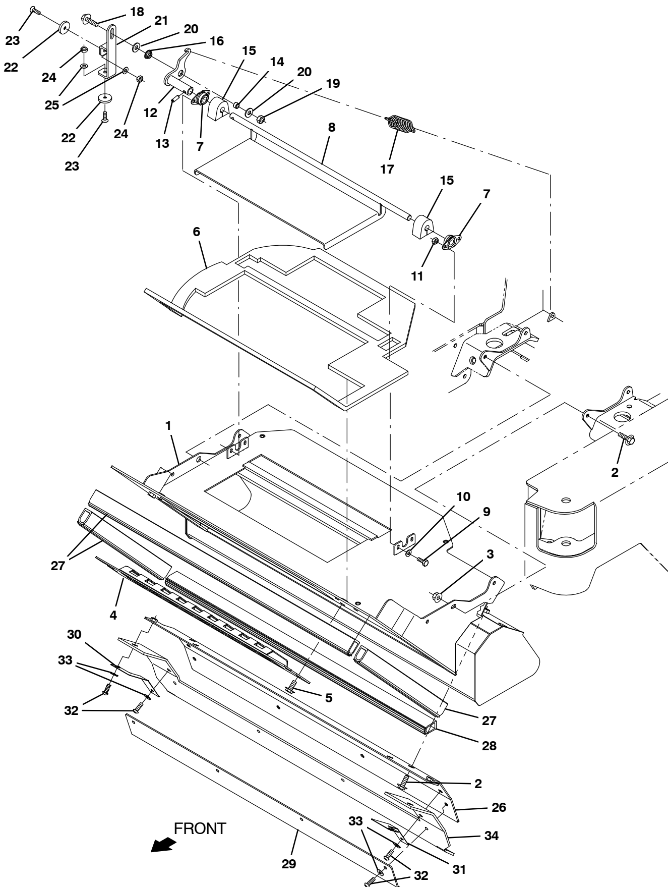
Fig. 40 – Plastic Hopper Pre-Filter and Dump Door Group
