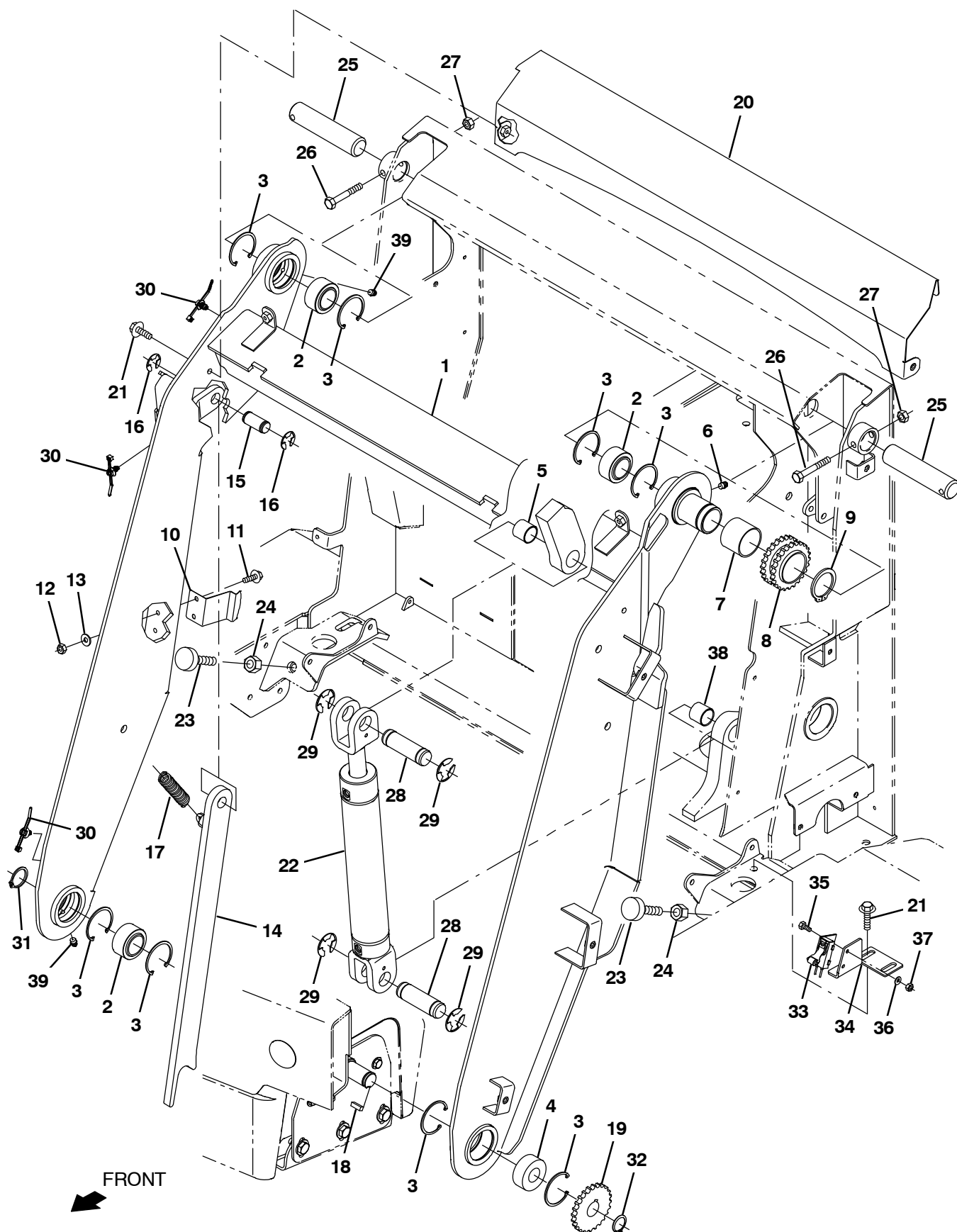
Fig. 35 – Hopper Lift Arm Group
