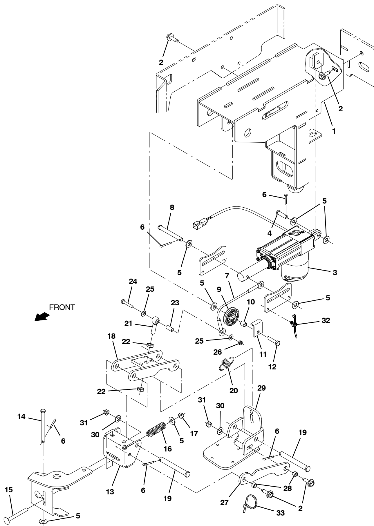
Fig. 23 – Sweeping Side Brush Lift Group, Left Side
