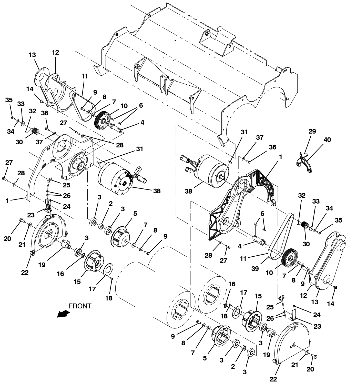
Fig. 28 – Scrub Head Drive Motors Group, Cylindrical
