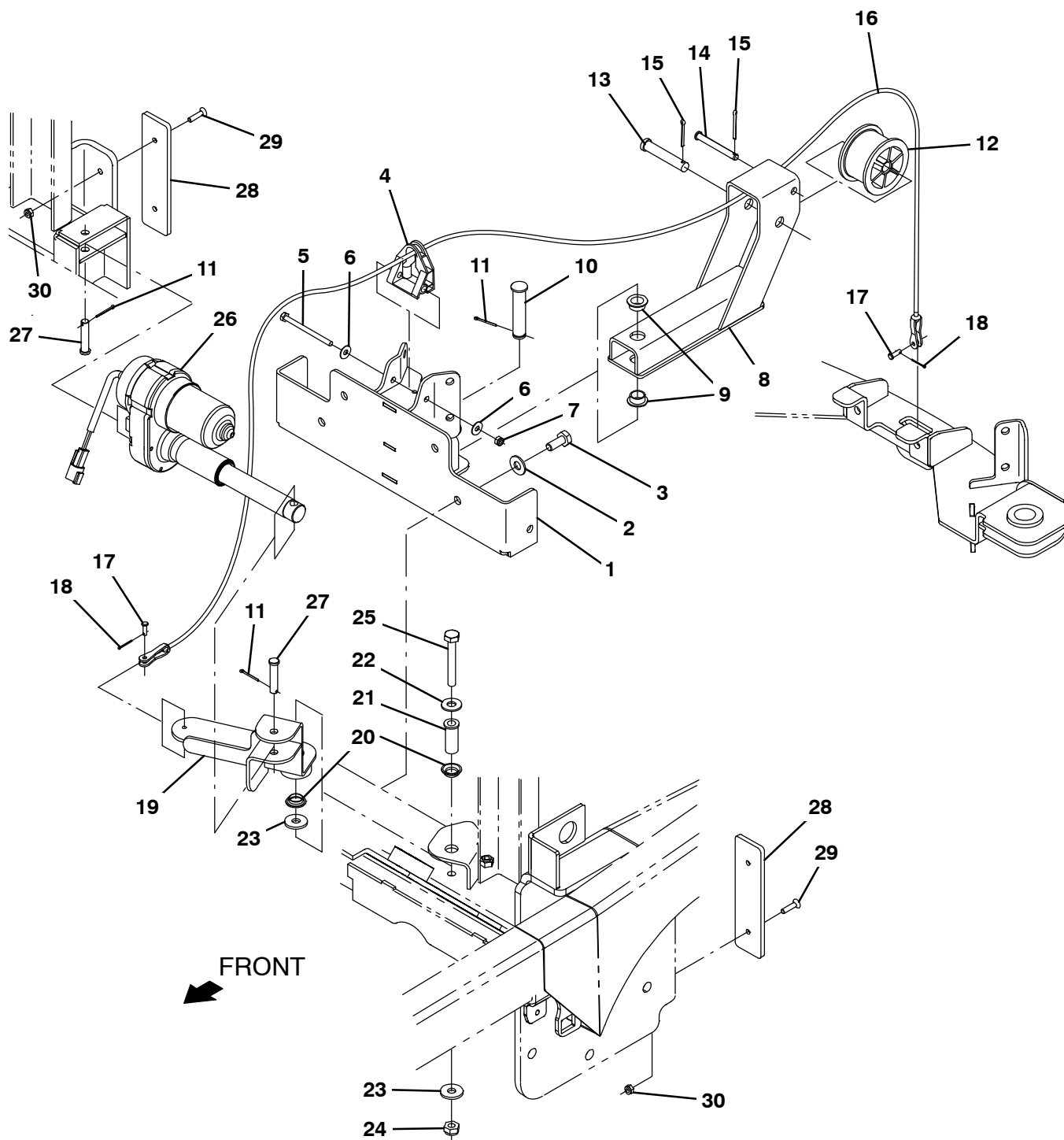
Fig. 46 – Rear Squeegee Lift Group
