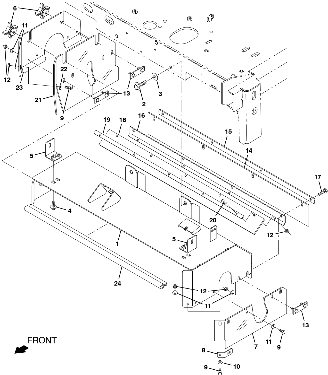
Fig. 41 – Direct Throw Main Brush Frame Group (0500– )
