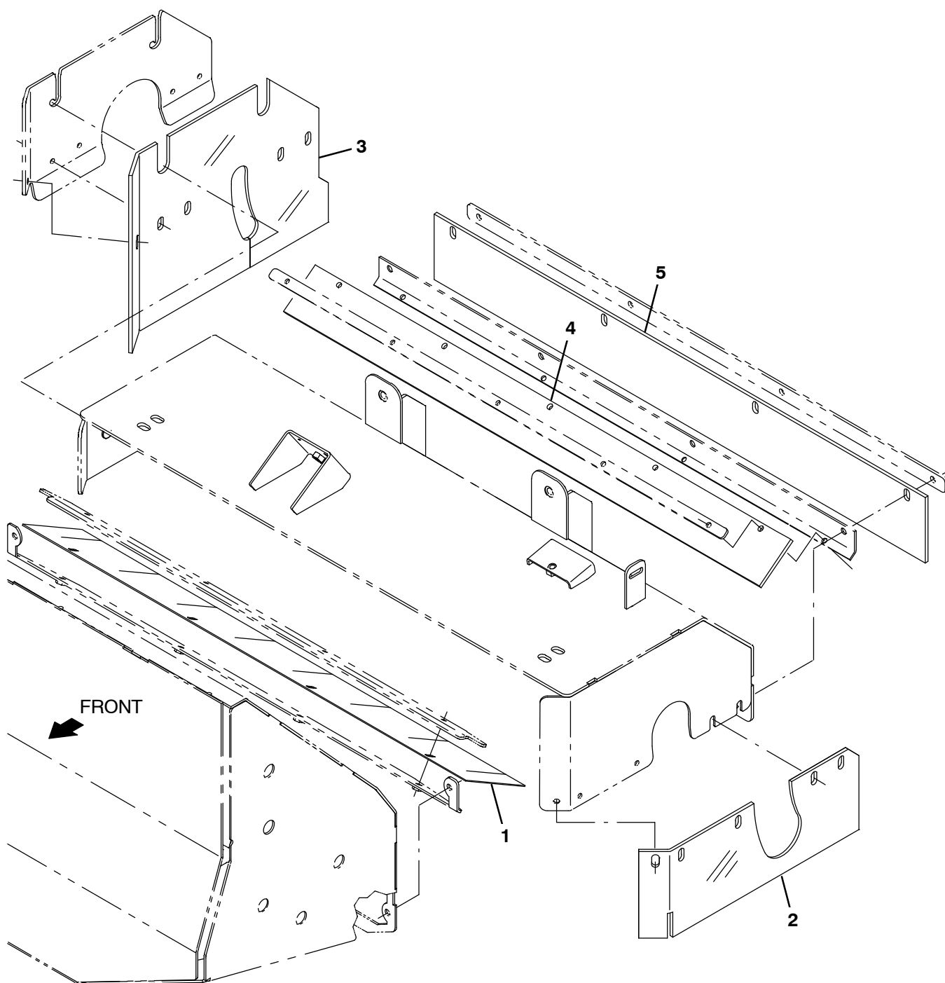
Fig. 45 – Direct Throw Main Brush Skirt Kit (0500– )
