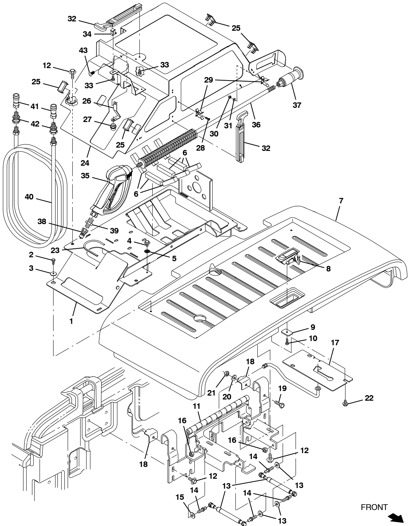
Fig. 34 – Pressure Washer Wand and Cover Group (0500– )
