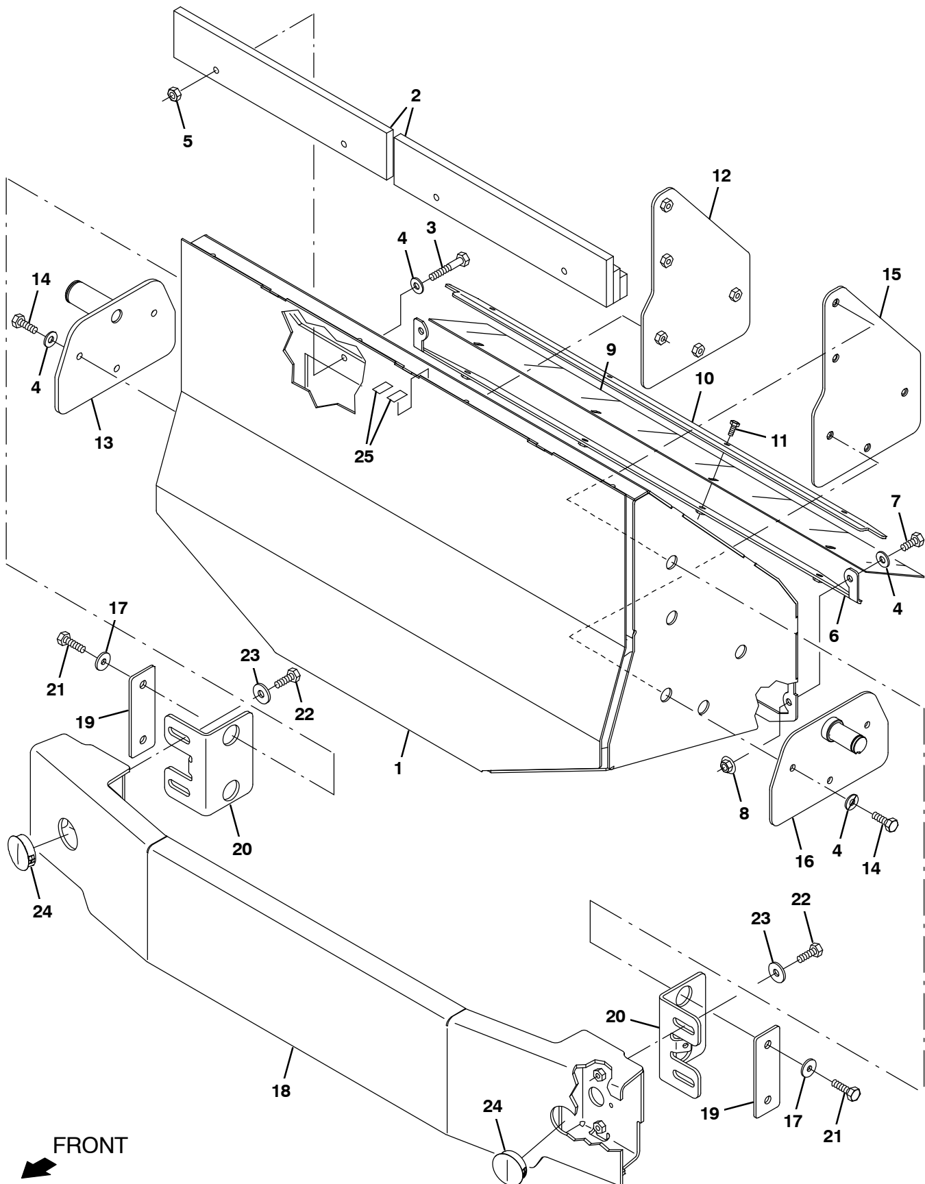
Fig. 39 – Steel Hopper and Bumper Group (0500– )
