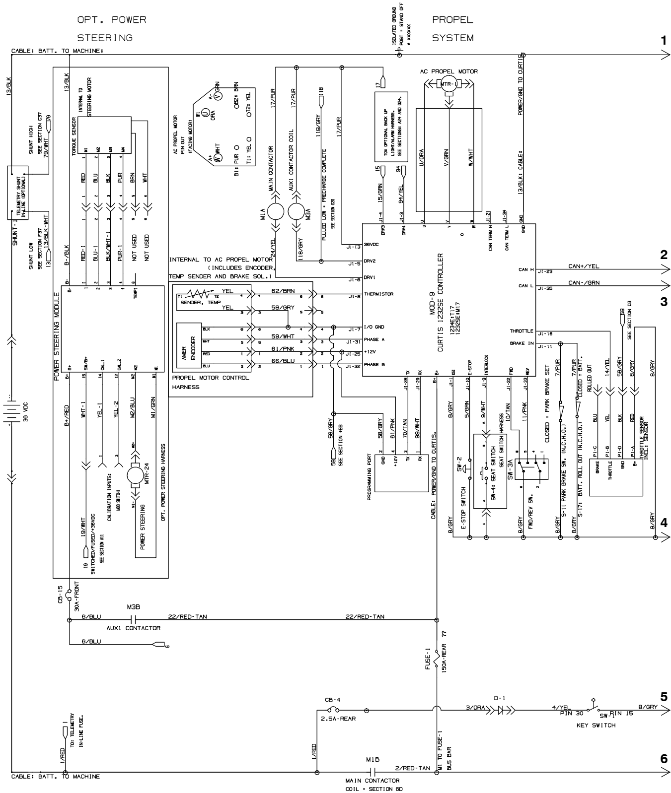
Fig. 54 – Electrical Schematic (0000-0499)
