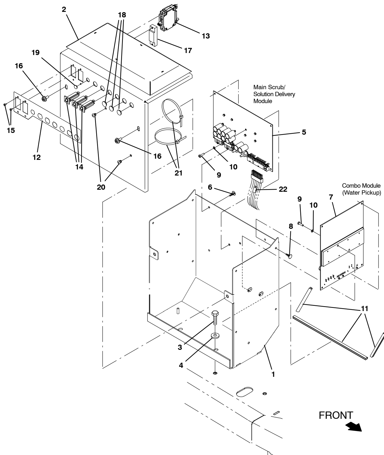
Fig. 50 – Electrical Box Group
