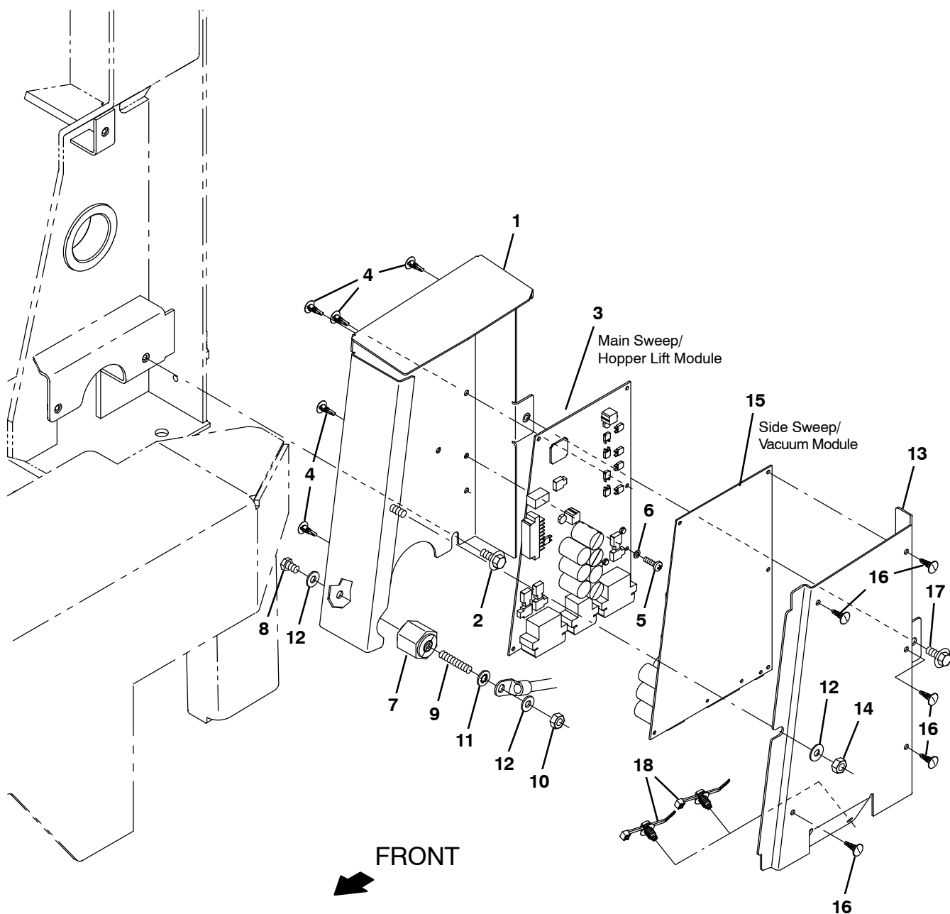
Fig. 53 – Electrical Box Group, Sweeping
