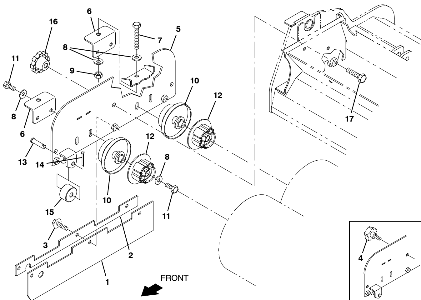
Fig. 16 – Sweeping Main Brush Idler Group
