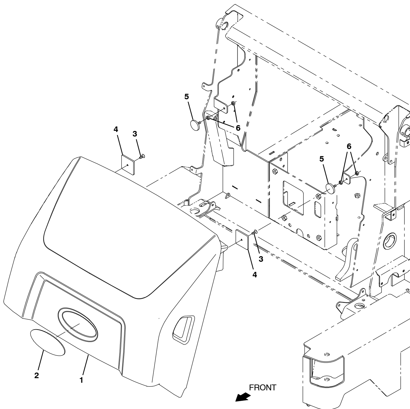
Fig. 34 – Hopper Cover Group
