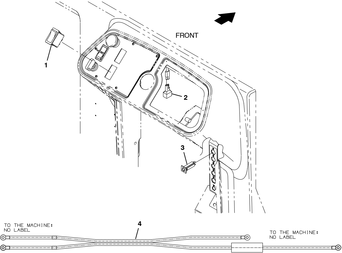
Fig. 37 – Pressure Washer Electrical Group (0500– )
