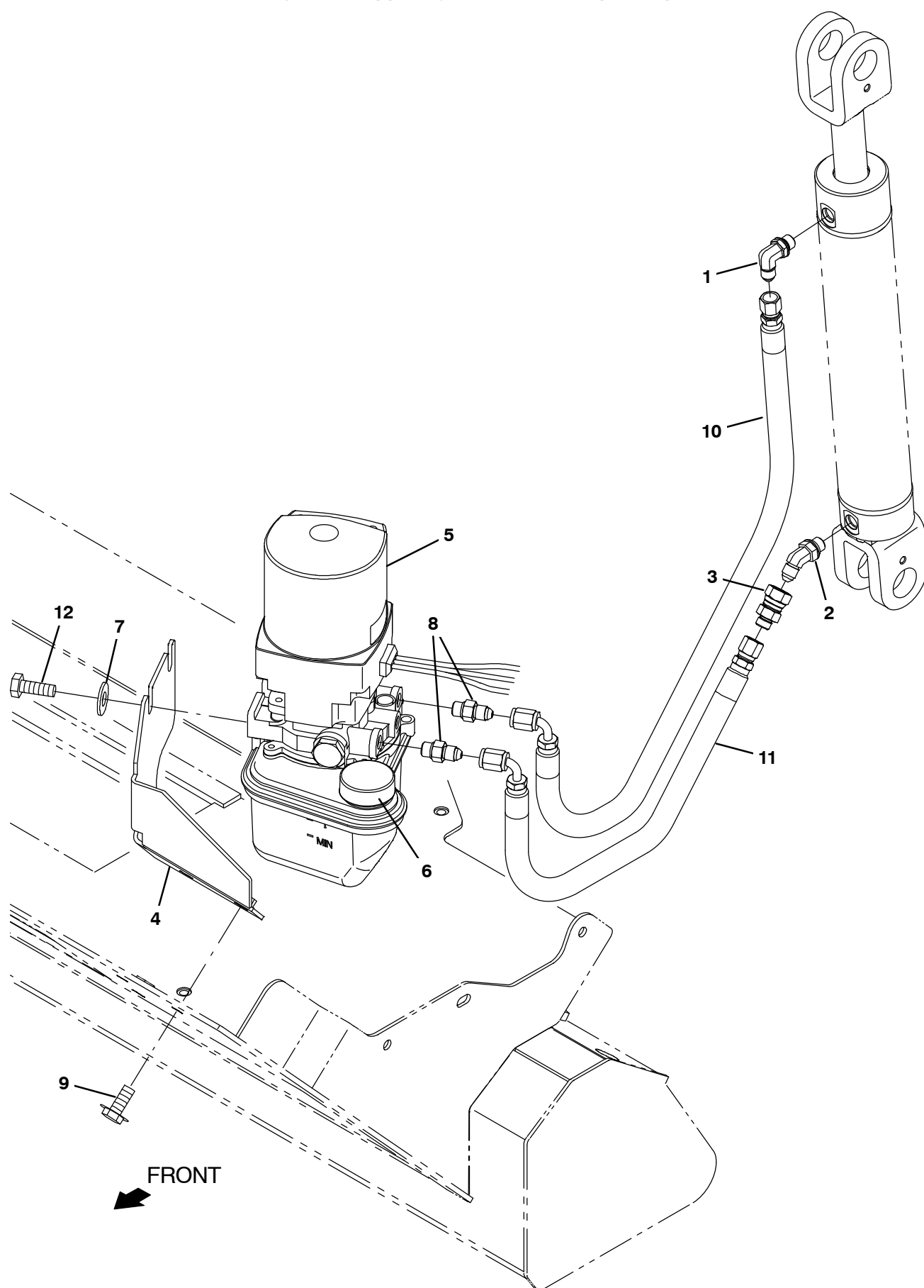
Fig. 37 – Hopper Hydraulic Lift Pump Group
