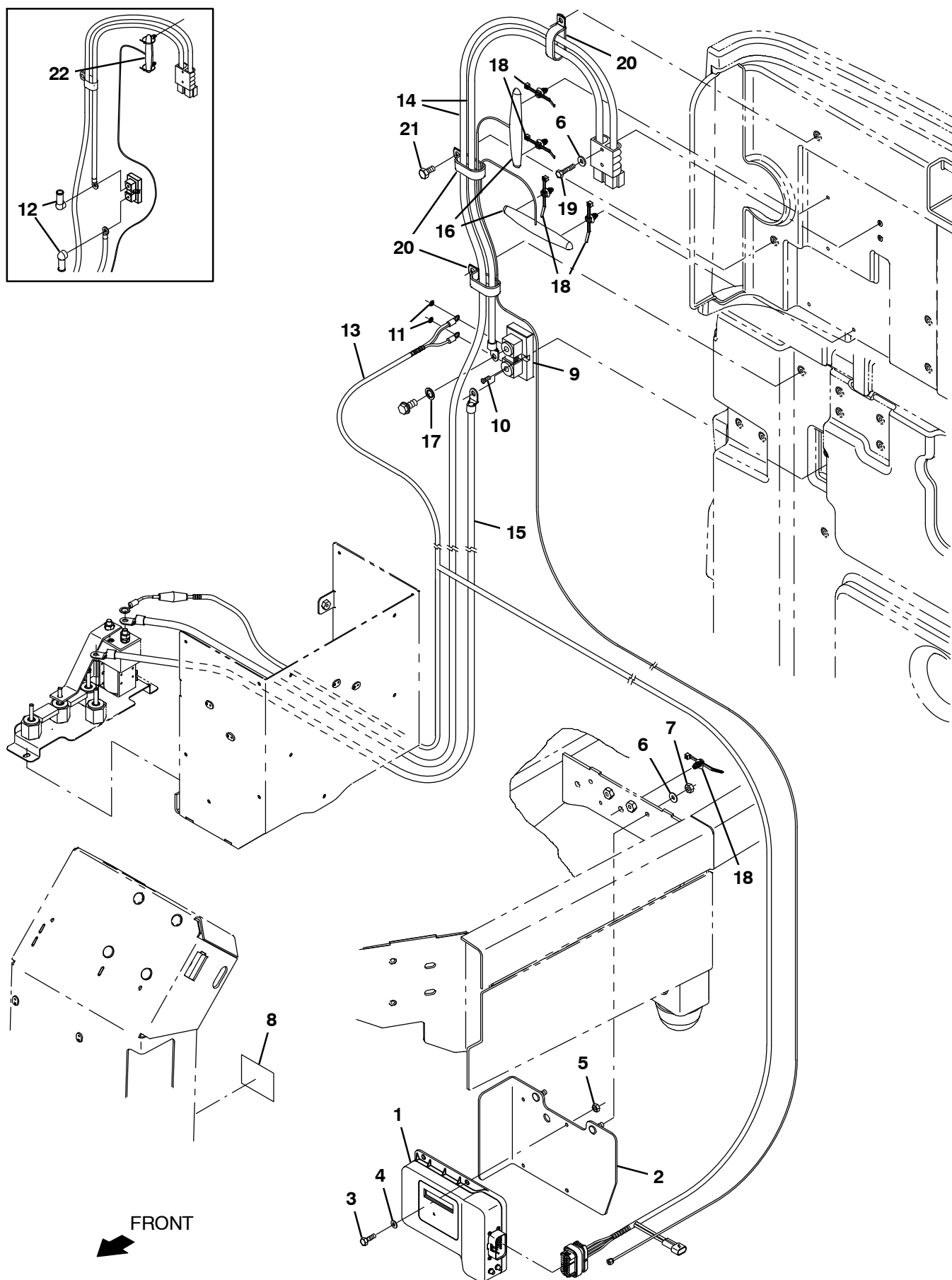
Fig. 23 - Telemetry Group
