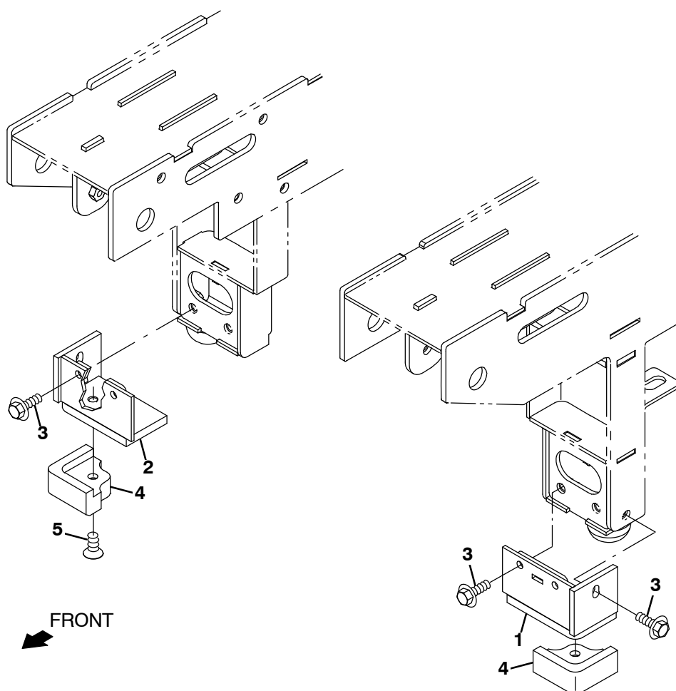
Fig. 46 – Direct Throw Main Brush Leg Pads Group (0500– )
