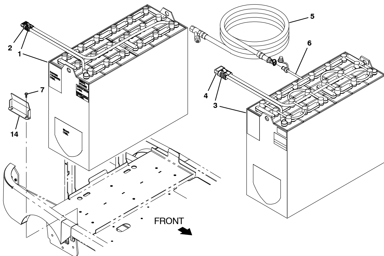
Fig. 32 – Battery and Charger Group, 930AH (APAC)
