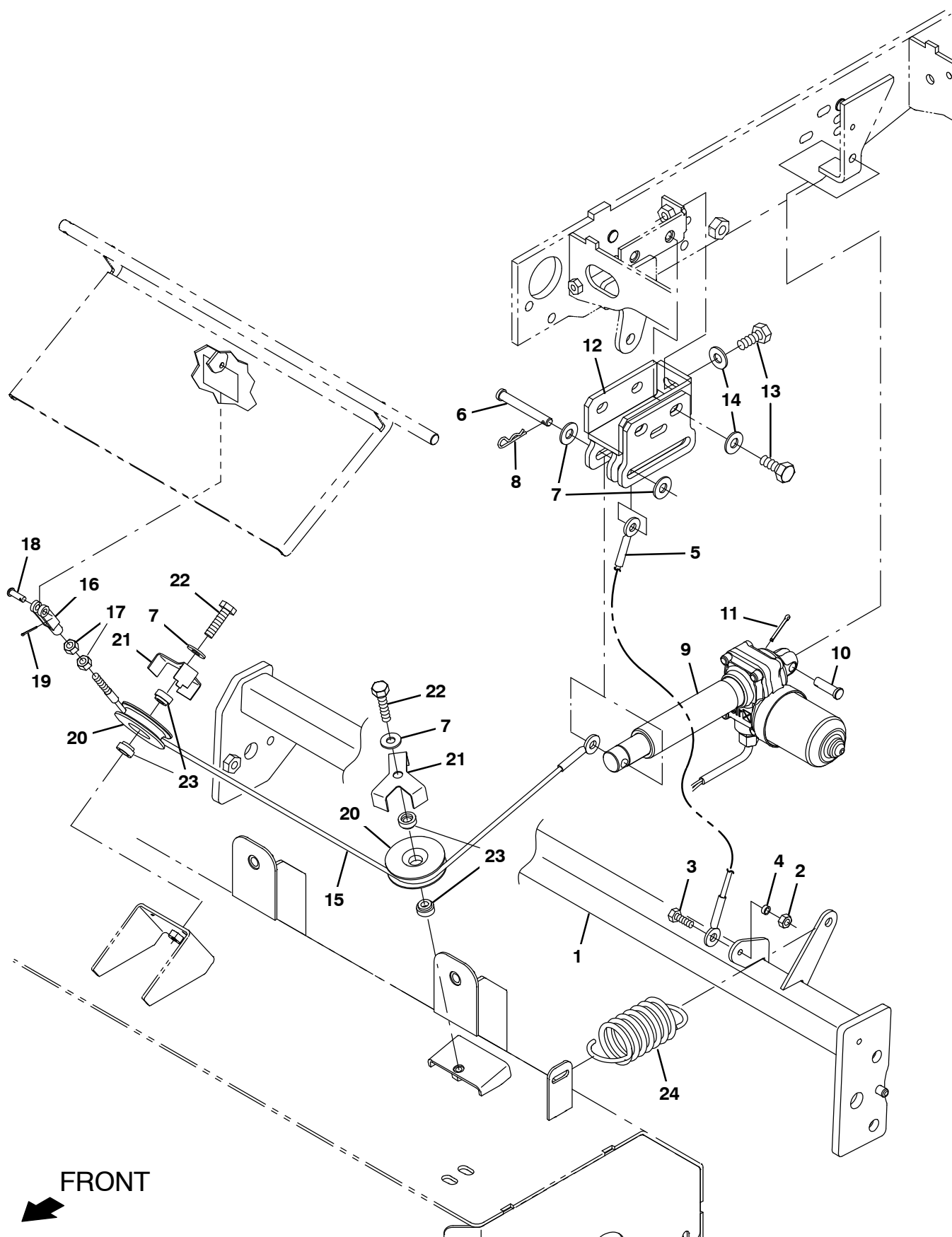
Fig. 43 – Direct Throw Main Brush Lift Group (0500– )
