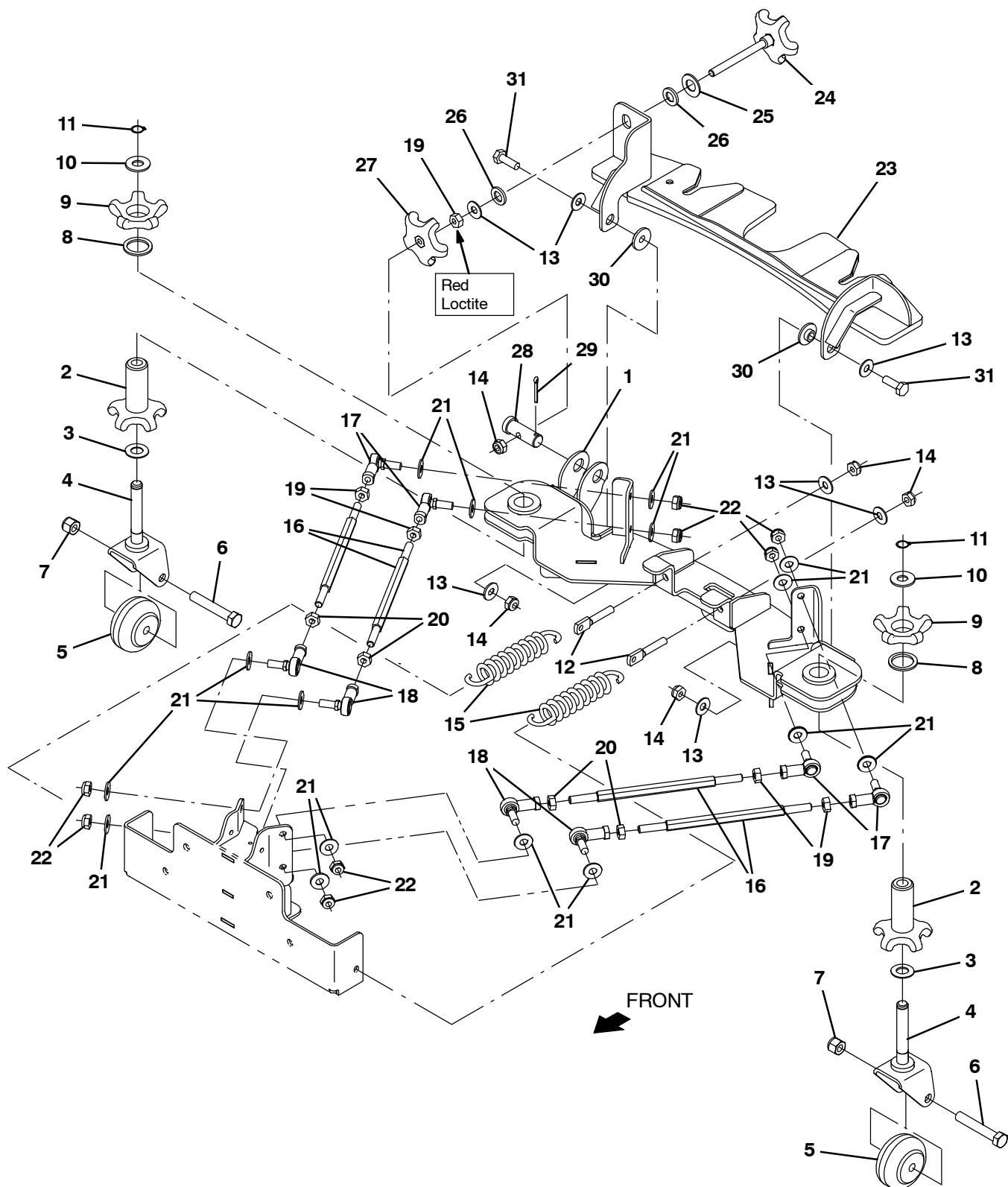
Fig. 47 – Rear Squeegee Linkage Group
