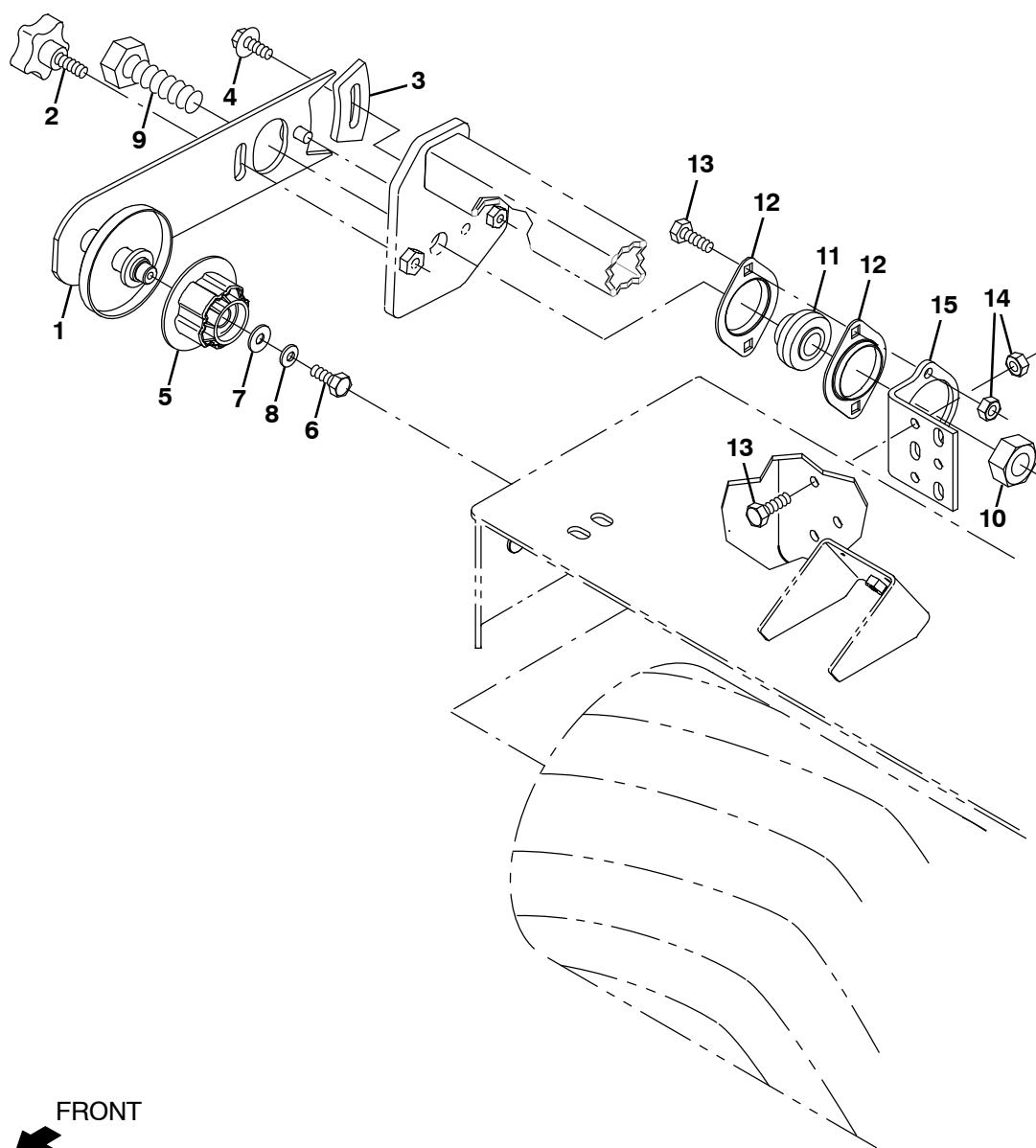
Fig. 44 – Direct Throw Main Brush Idler Group (0500– )
