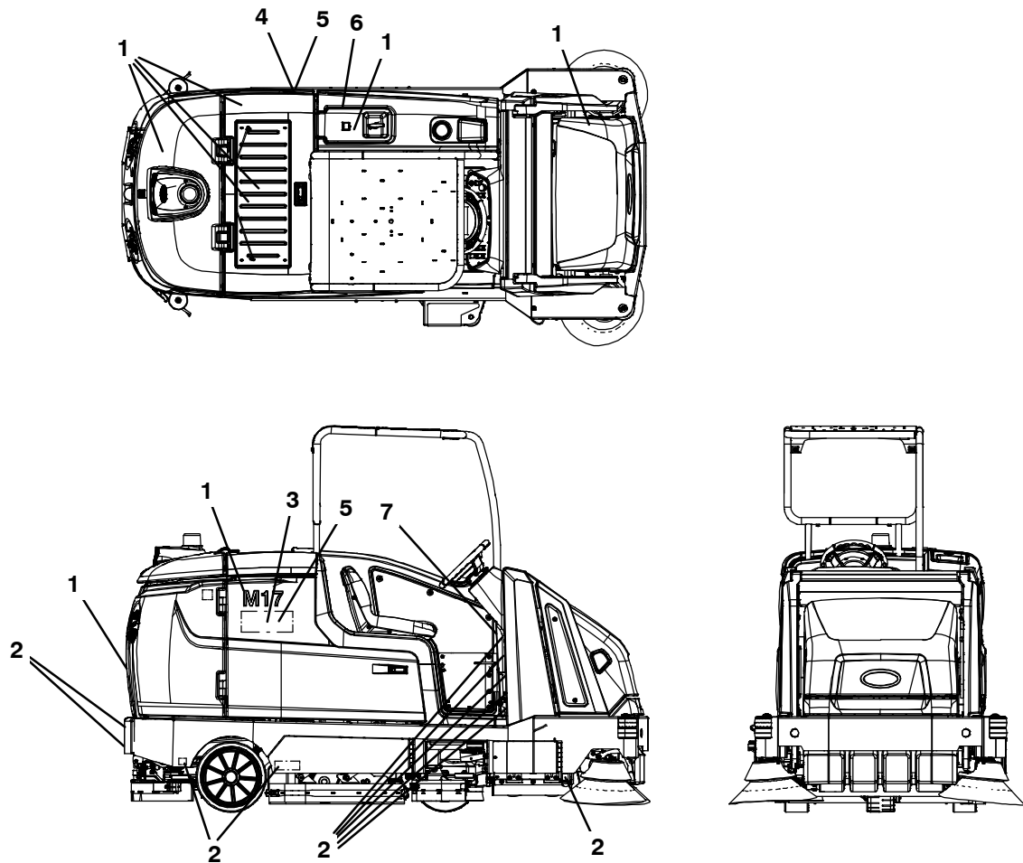
Fig. 58 – Label Group
