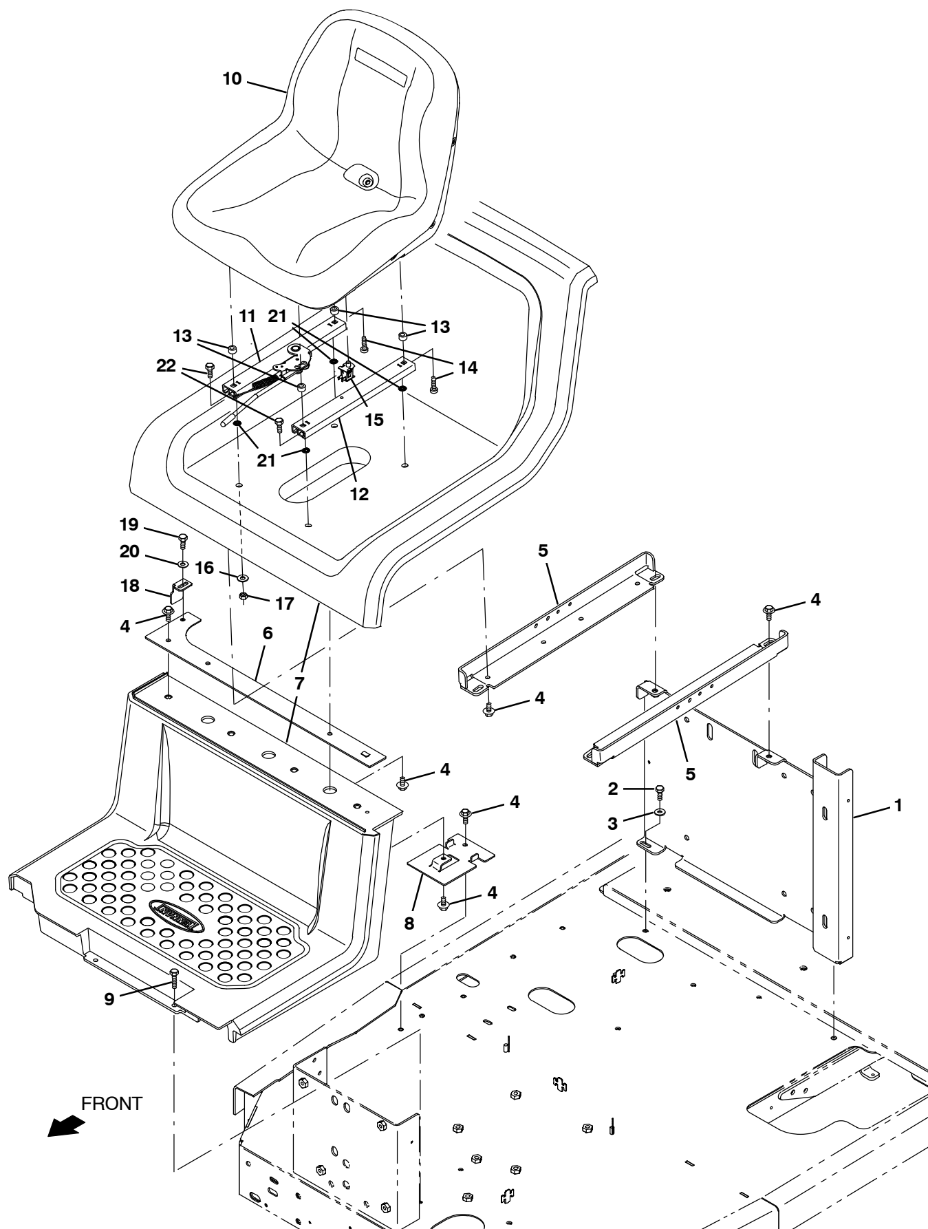
Fig. 10 – Seat Group
