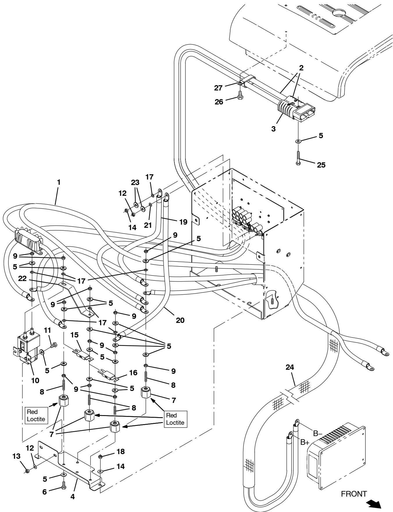
Fig. 51 – Electrical Box Wires Group
