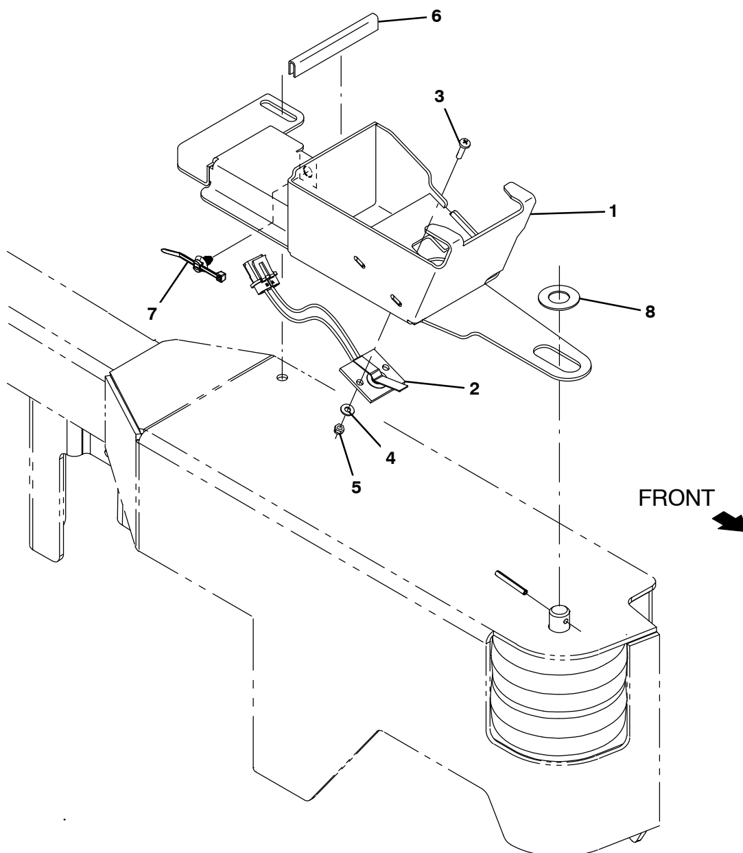
Fig. 51 – Dry Vacuum Nozzle Holder Group (0562– )
