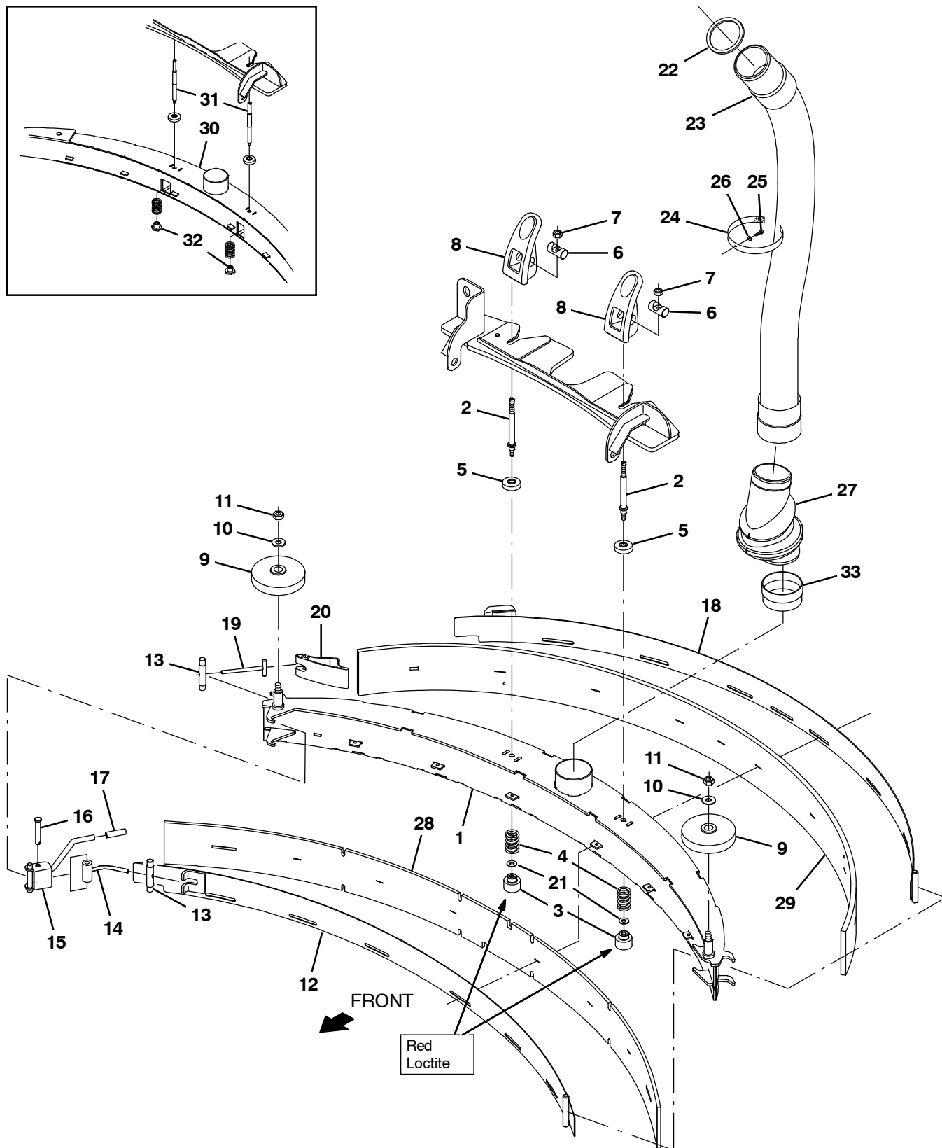
Fig. 48 – Rear Squeegee Group
