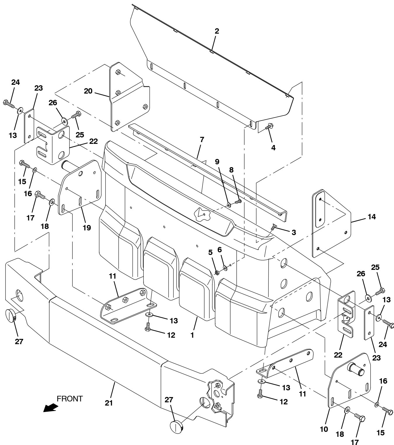
Fig. 33 – Plastic Hopper and Bumper Group
