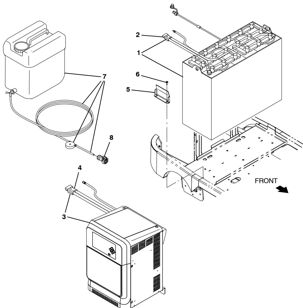
Fig. 28 – Battery and Charger Group, 775AH, Opportunity Charging (EMEA)
