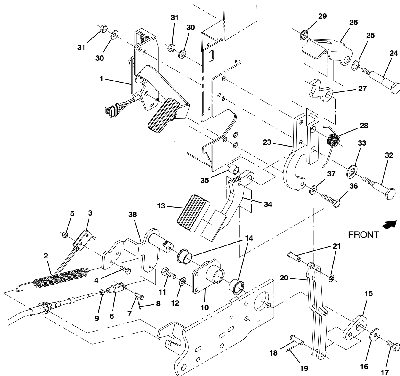
Fig. 8 – Brake Pedal Group
