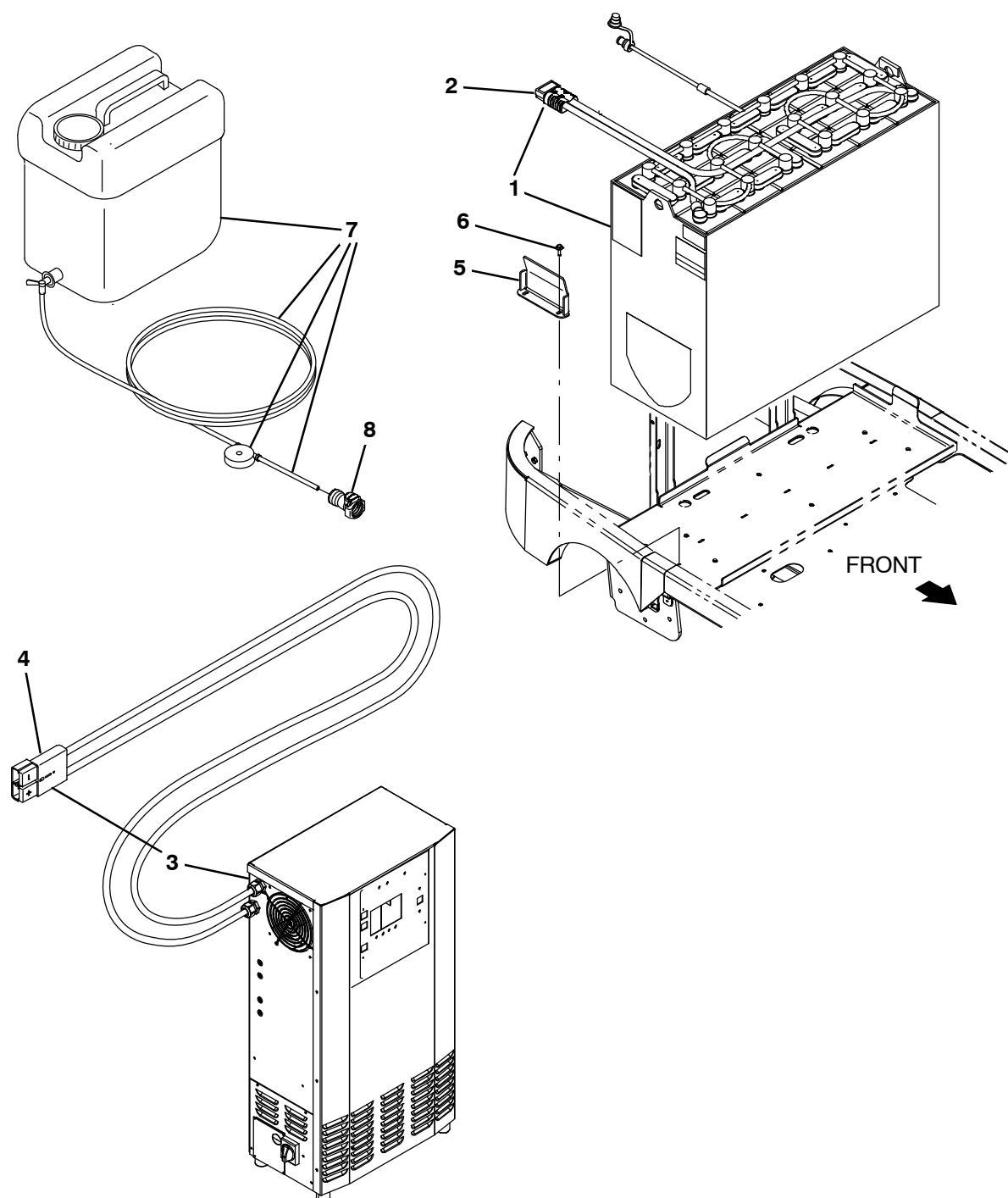
Fig. 27 – Battery and Charger Group, 775AH (EMEA)
