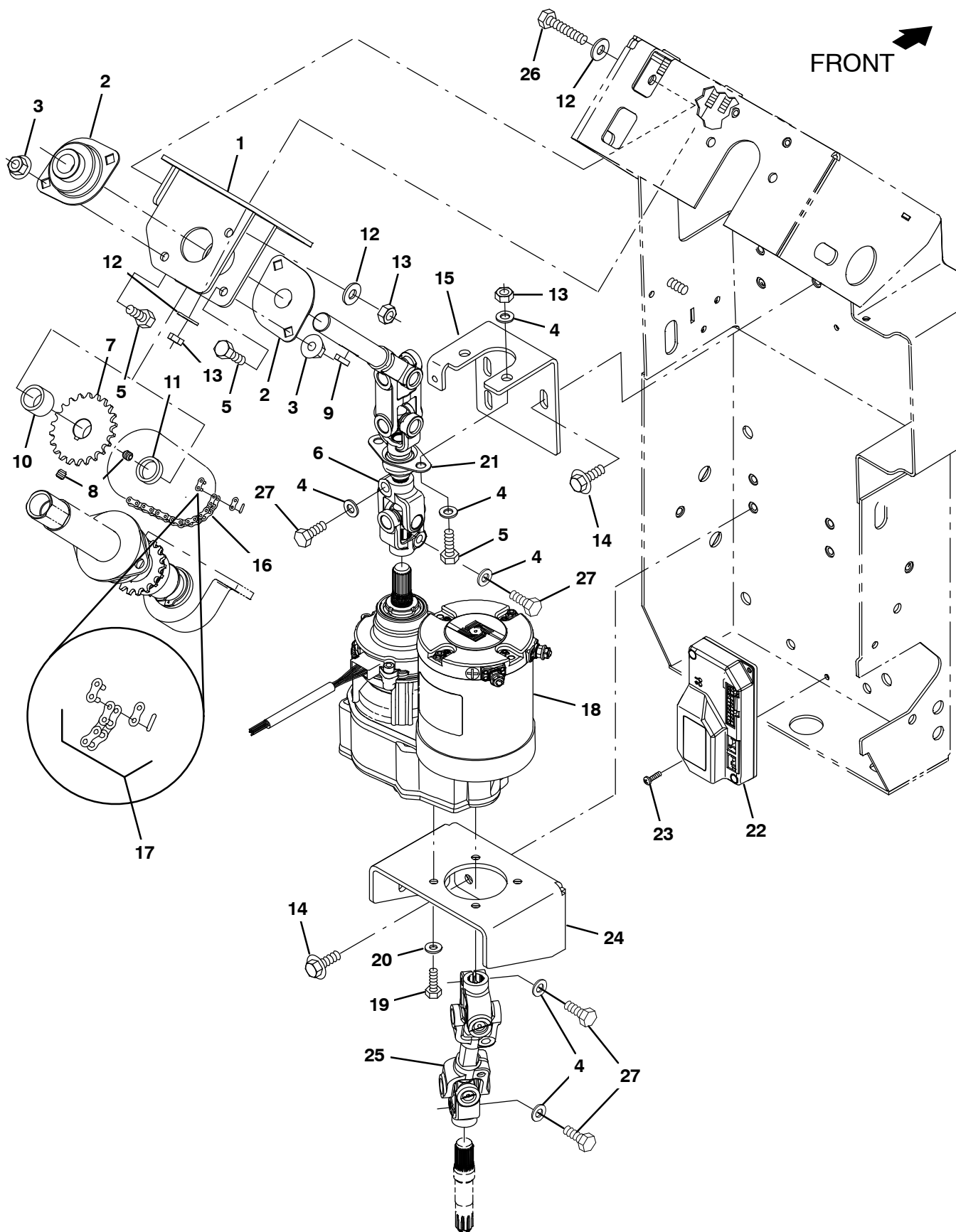
Fig. 7 – Power Steering Group (0726– )
