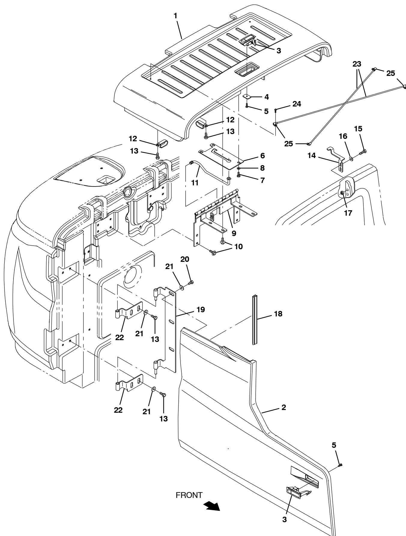
Fig. 49 – Right Hand Door and Battery Cover Group
