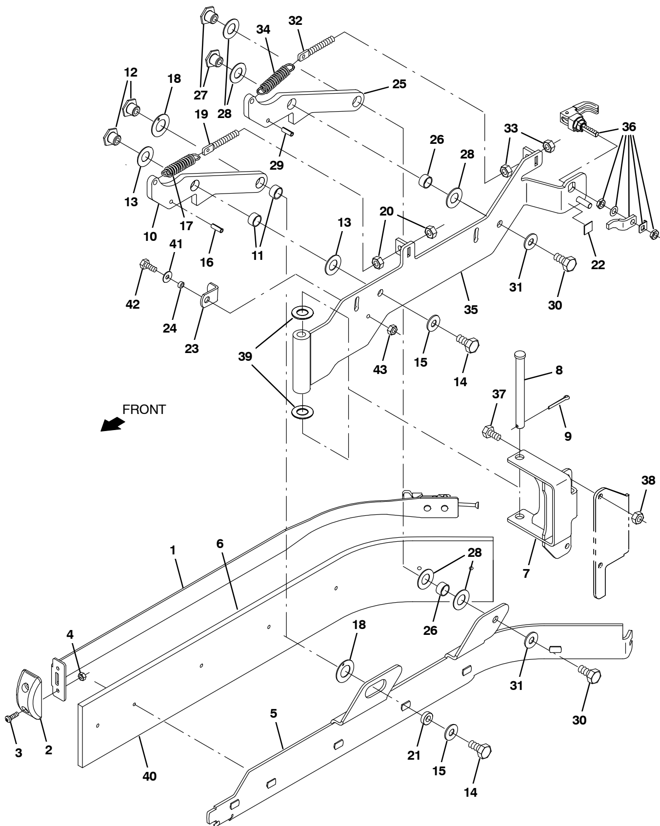
Fig. 30 – Scrub Head Side Squeegee Group, Right Hand (U00838- )
