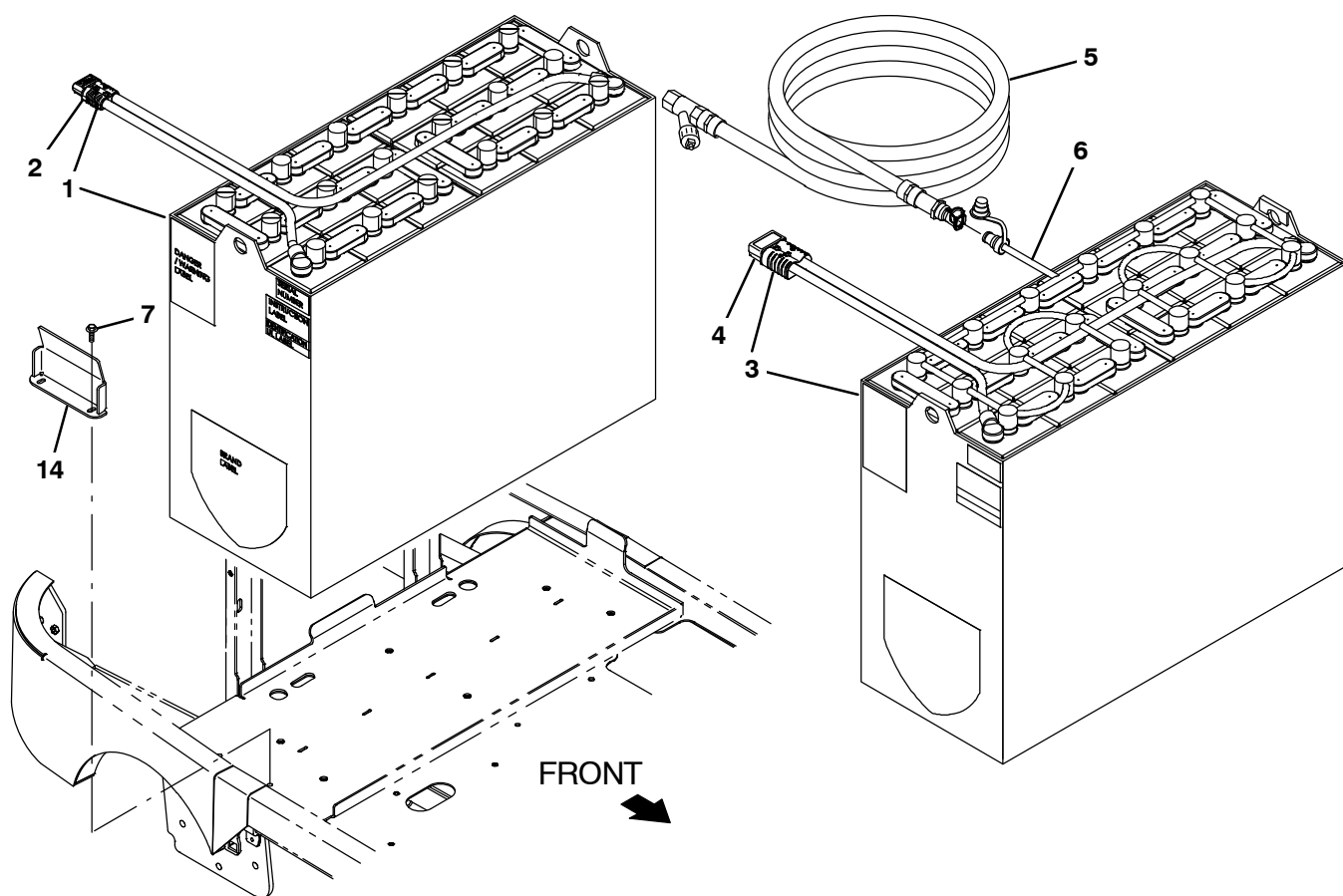
Fig. 30 – Battery and Charger Group, 510AH / 625AH (APAC)
