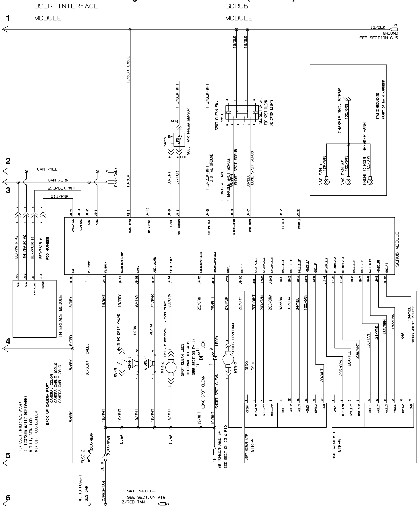
Fig. 54 – Electrical Schematic (0000–0499)
