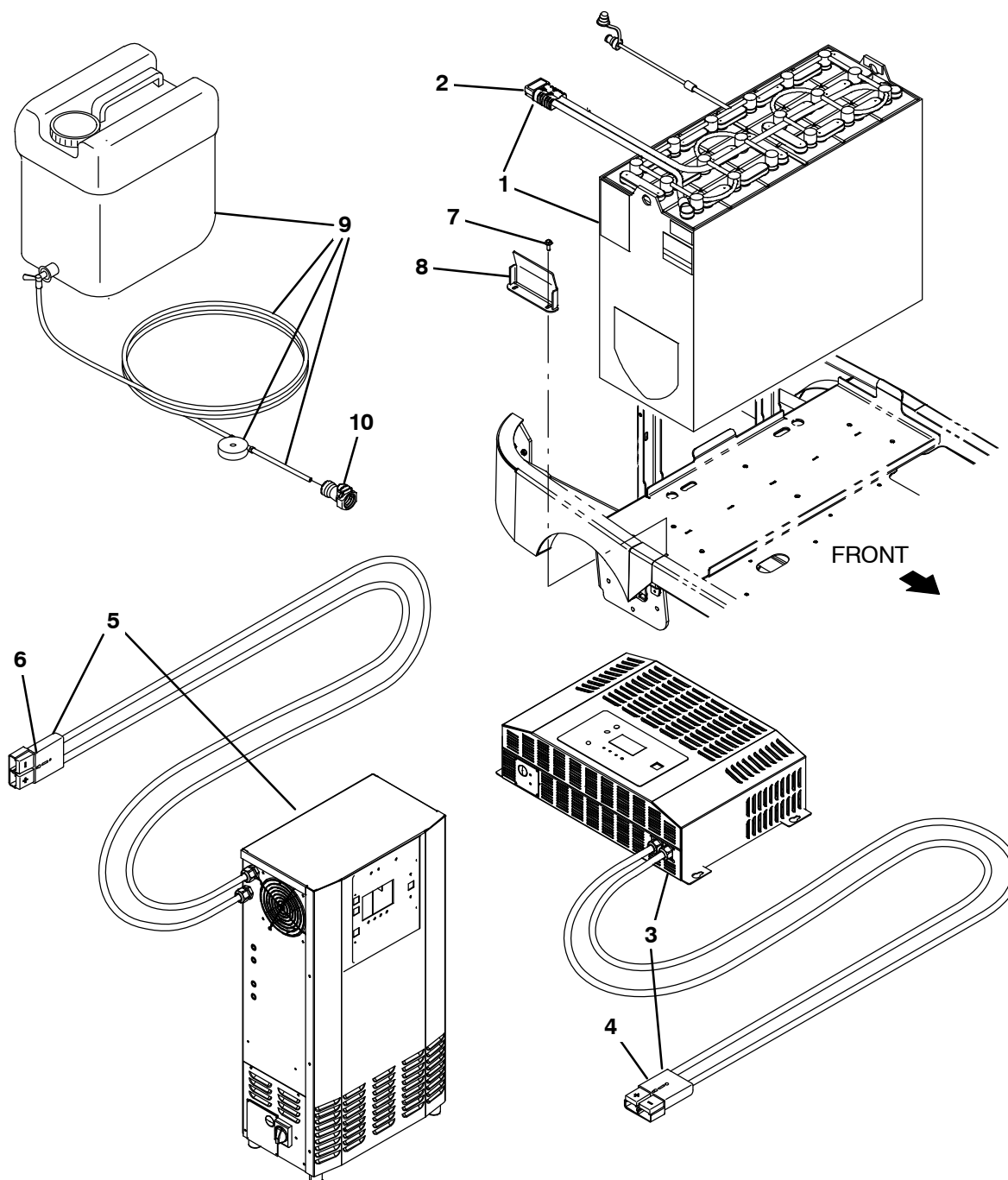
Fig. 26 – Battery and Charger Group, 625AH (EMEA)
