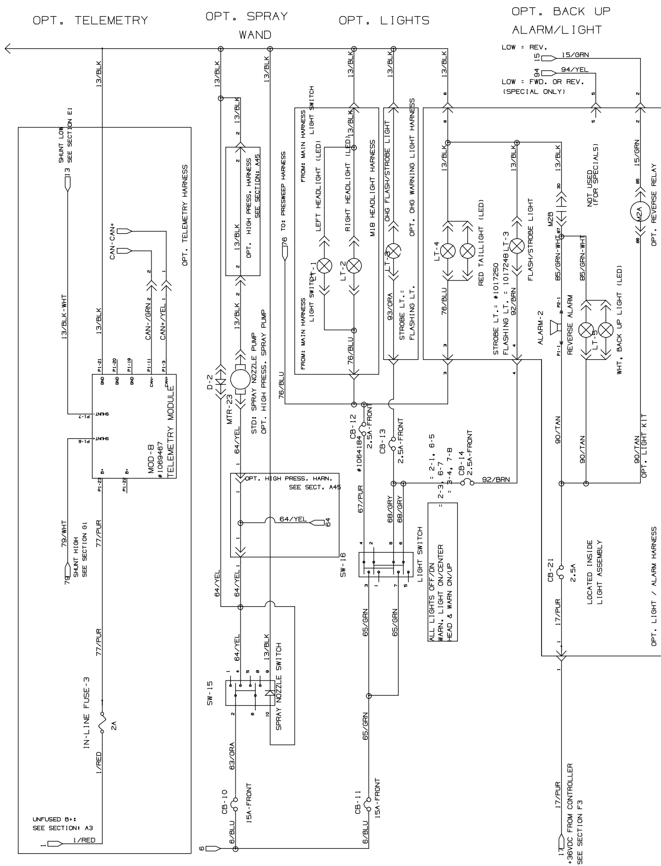
Fig. 56 – Electrical Schematic (0562– )
