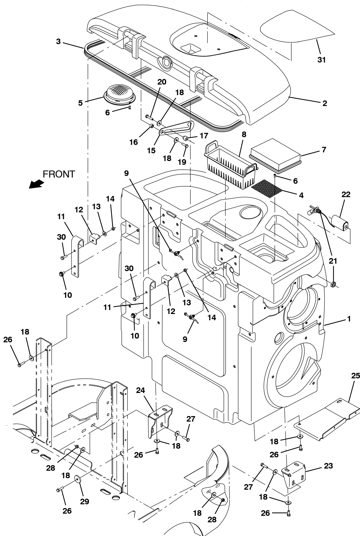
Fig. 43 – Recovery Tank Group
