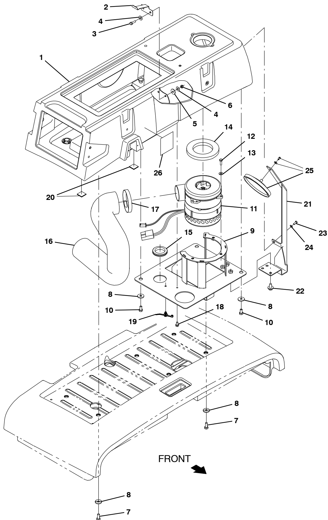
Fig. 49 – Dry Vacuum Fan and Housing Group (0562– )
