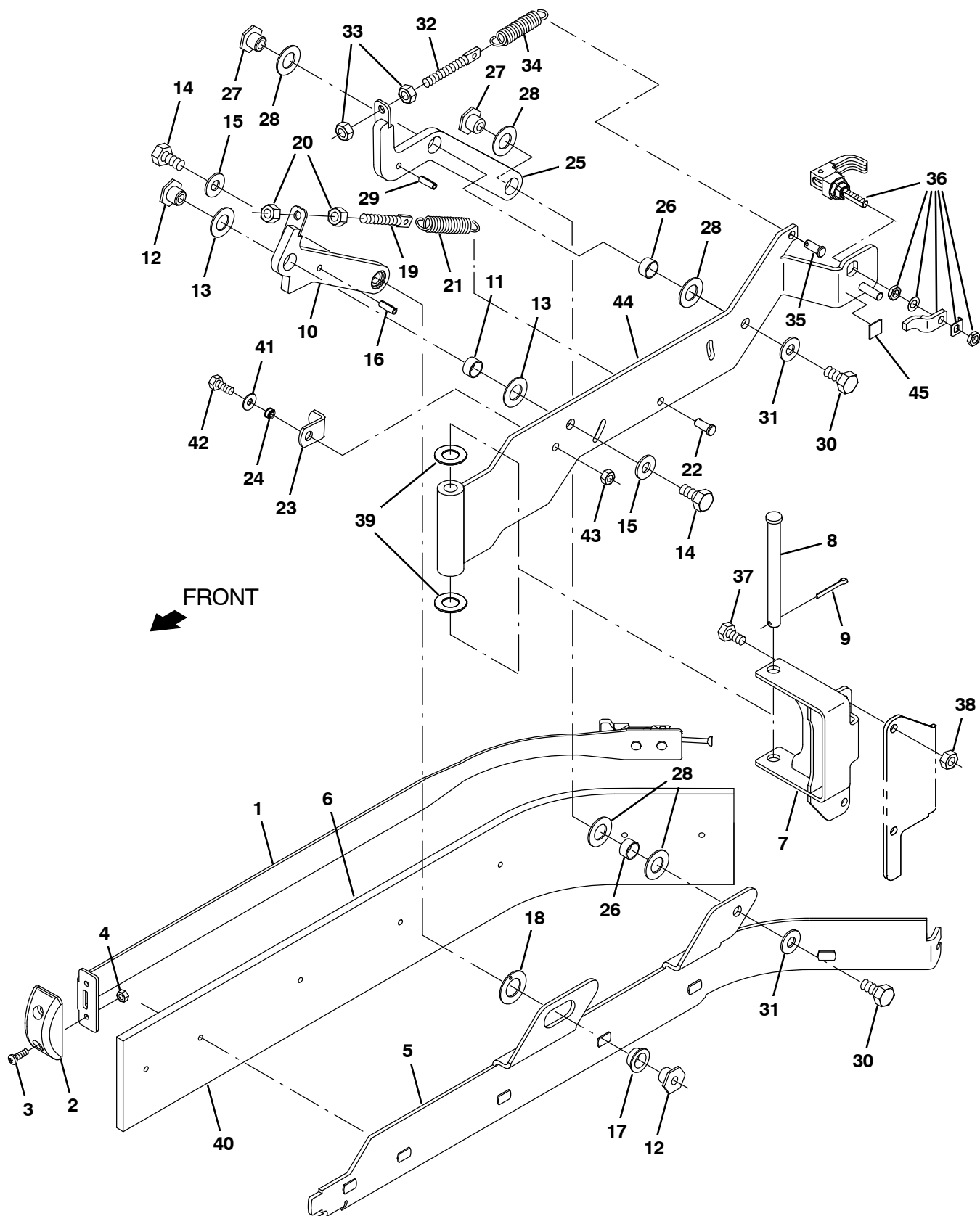
Fig. 29 – Scrub Head Side Squeegee Group, Right Hand (0000-U00837)
