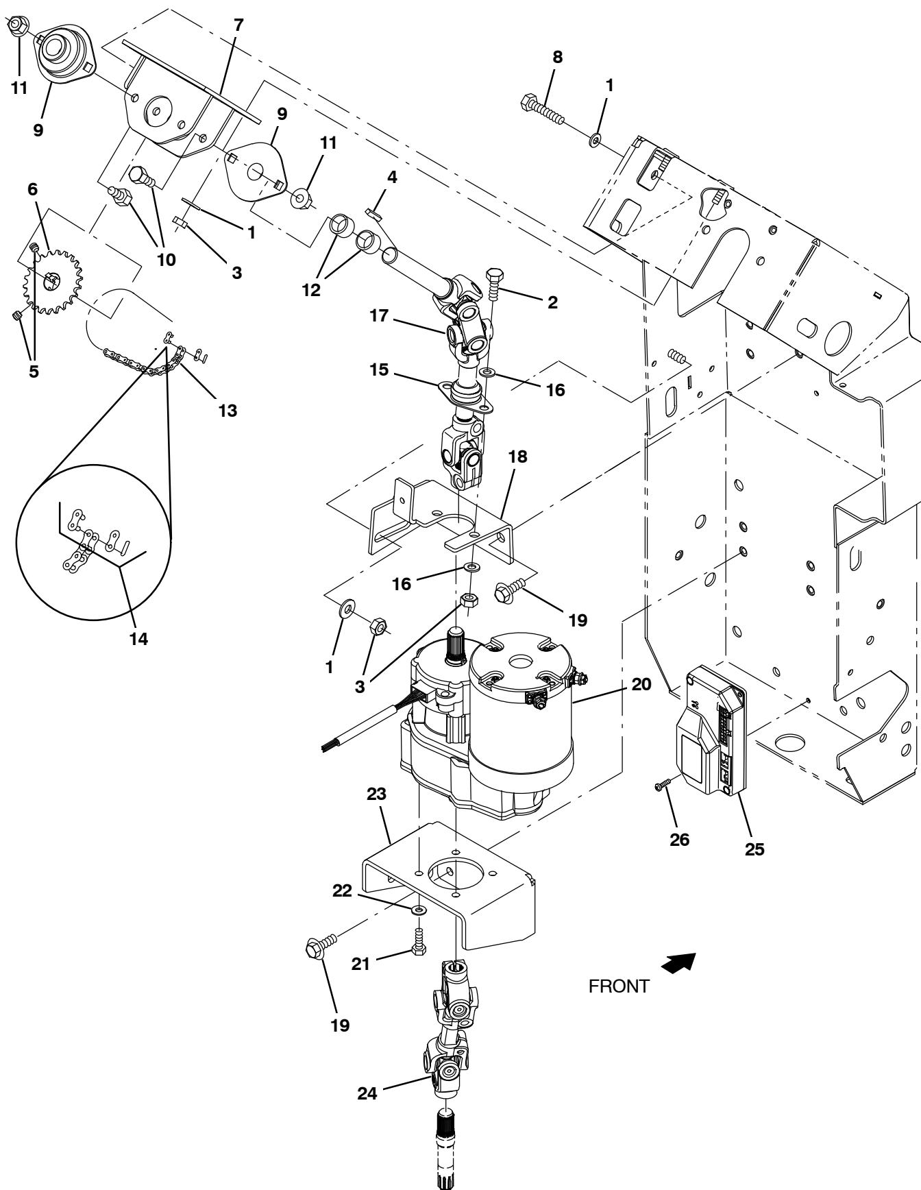
Fig. 6 – Power Steering Group (0000–0725)
