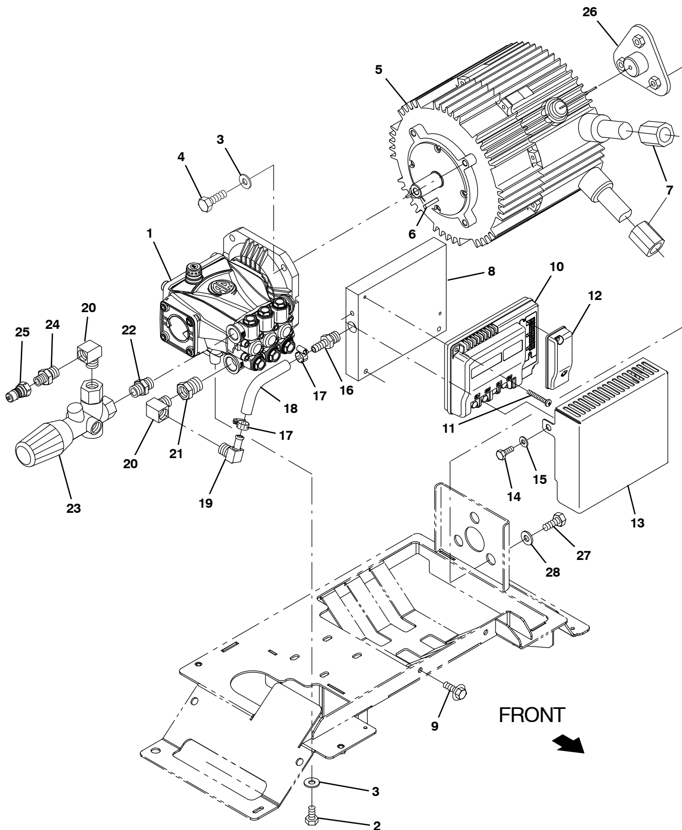
Fig. 36 – Pressure Washer Motor and Pump Group (0500– )
