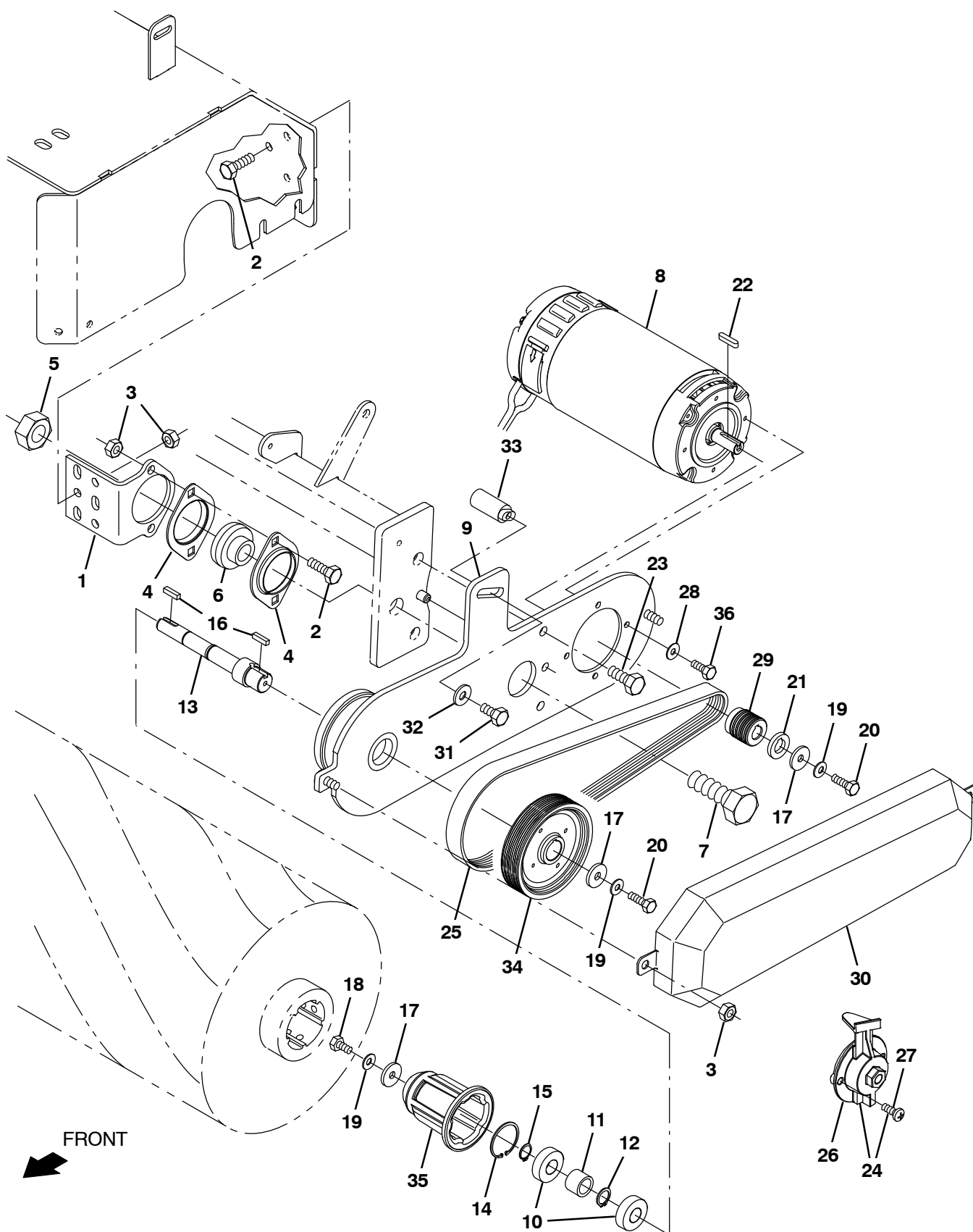
Fig. 42 – Direct Throw Main Brush Drive Motor Group (0500– )
