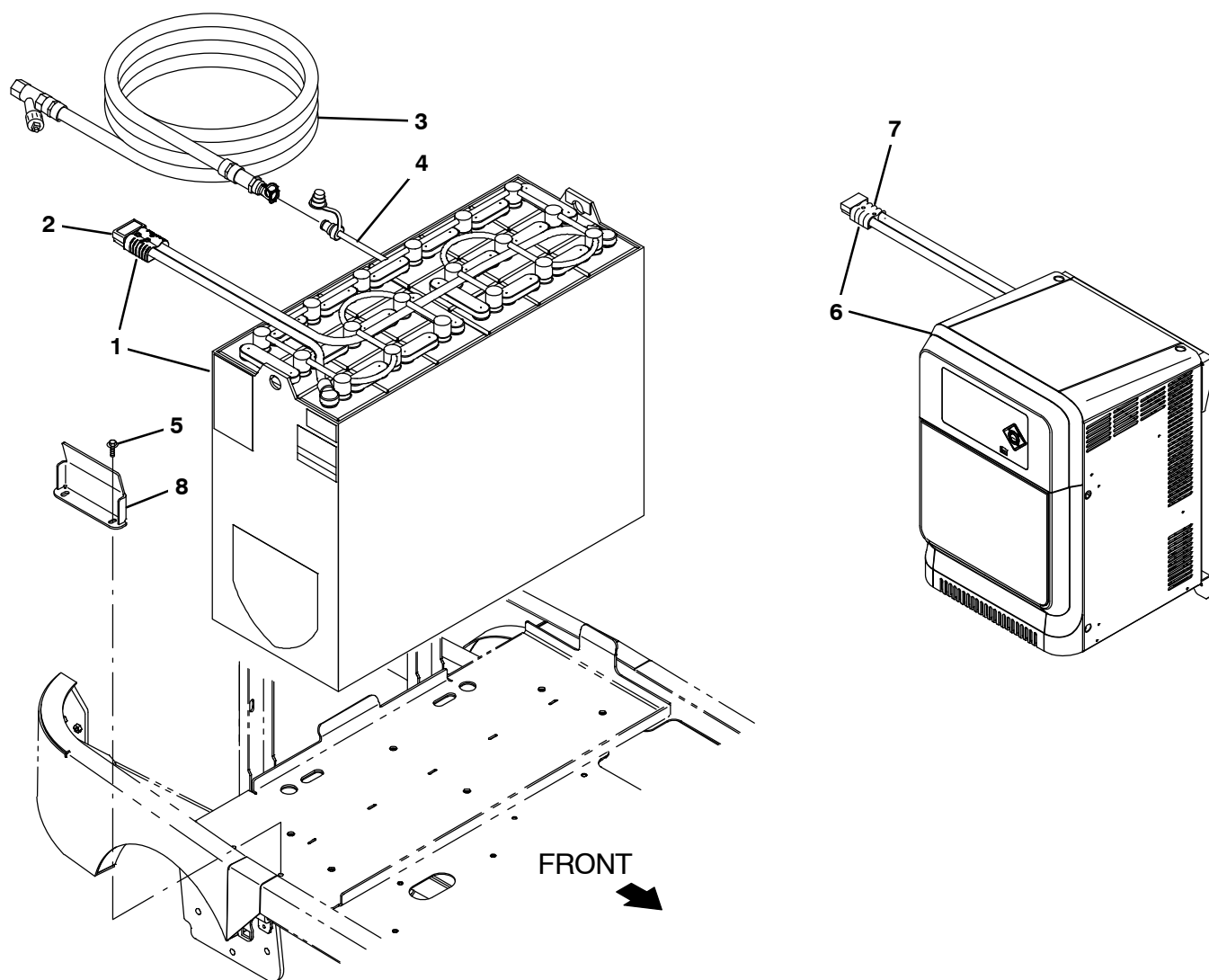
Fig. 33 – Battery and Charger Group, 930AH, Opportunity Charging (APAC)
