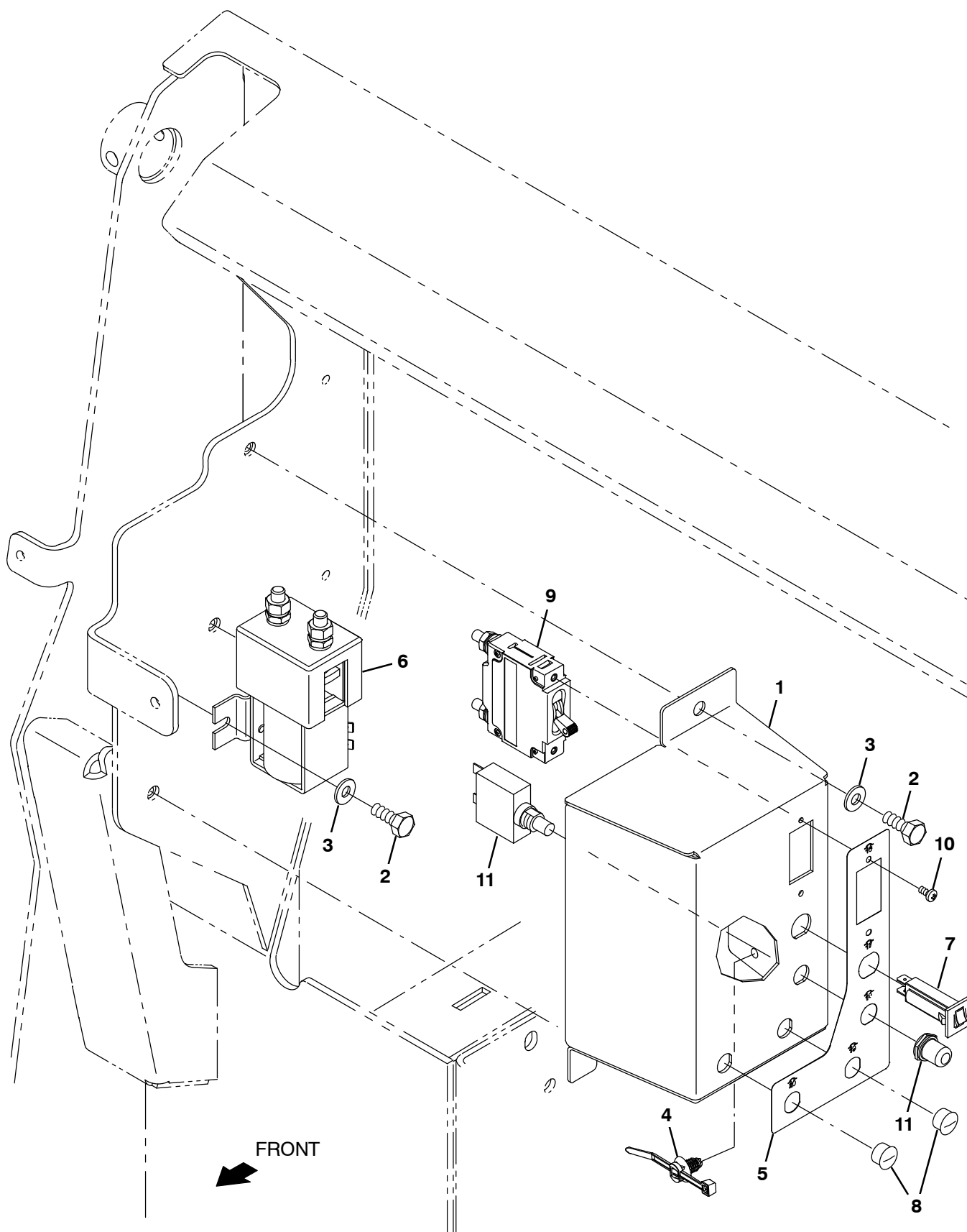
Fig. 52 – Electrical Circuit Breaker Box Group, Sweeping
