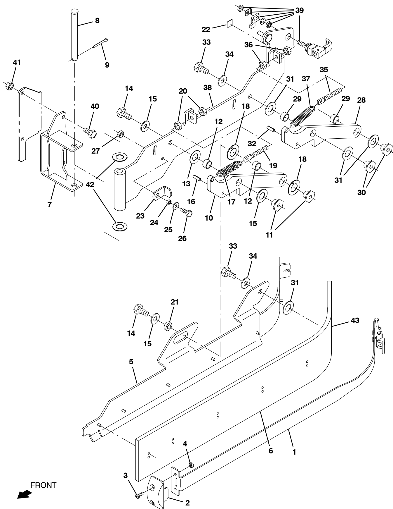
Fig. 32 – Scrub Head Side Squeegee Group, Left Hand (U00838– )
