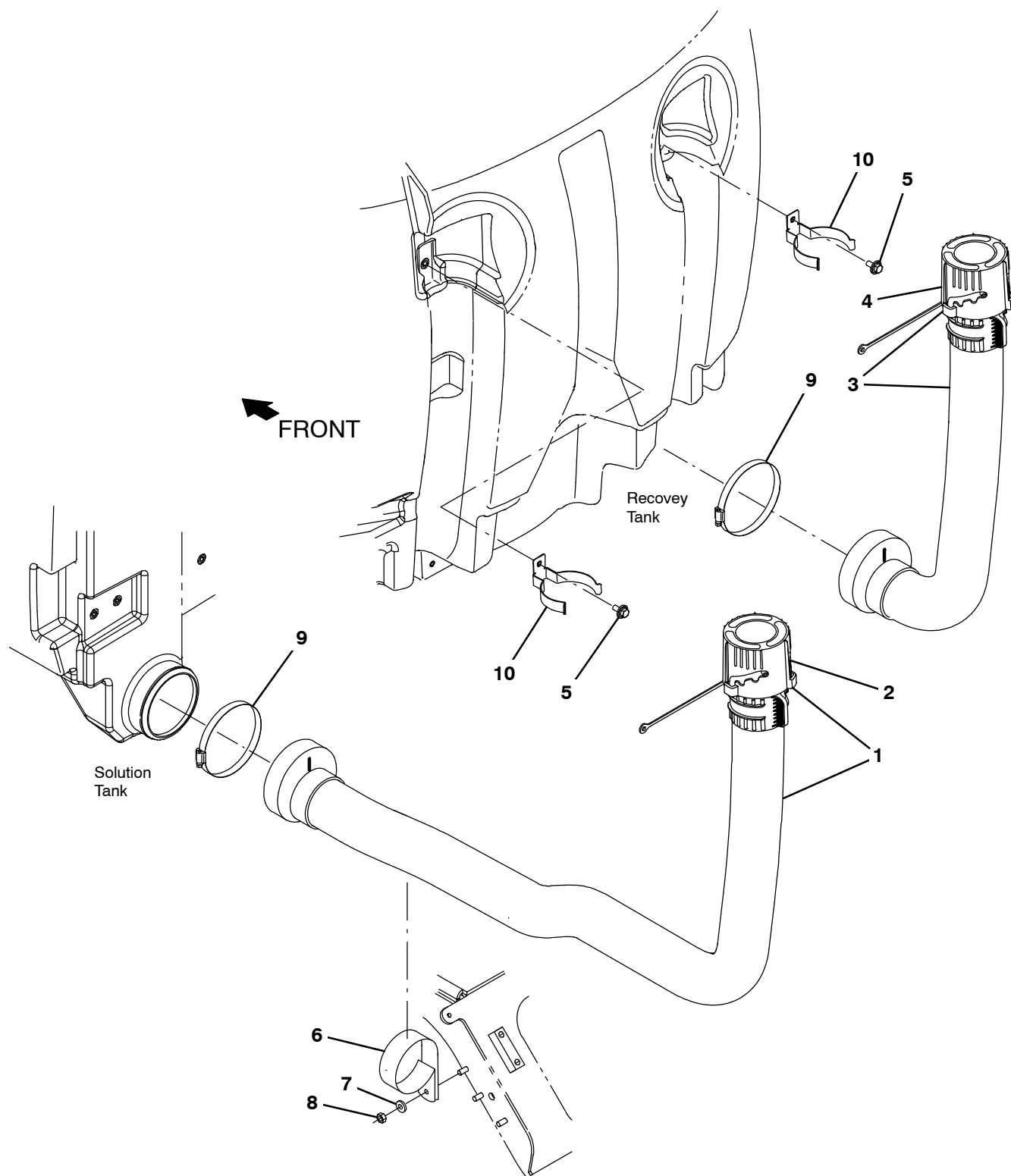
Fig. 44 – Tank Drains Group
