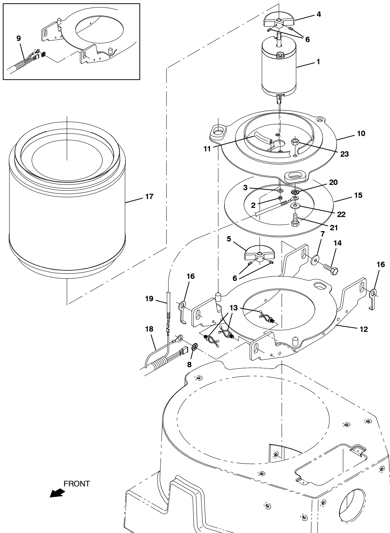
Fig. 39 – Hopper Filter Shaker Group
