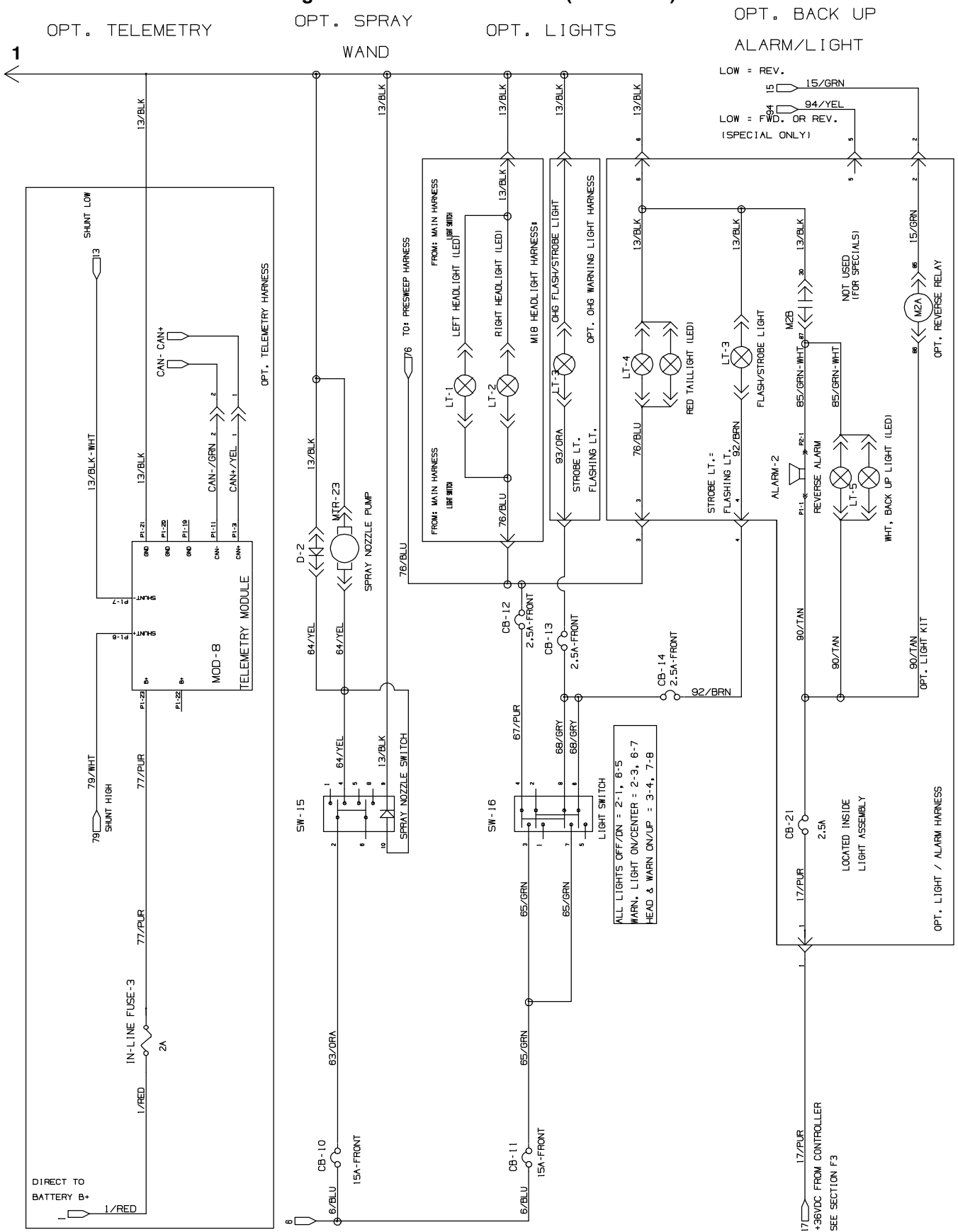
Fig. 54 – Electrical Schematic (0000–0499)
