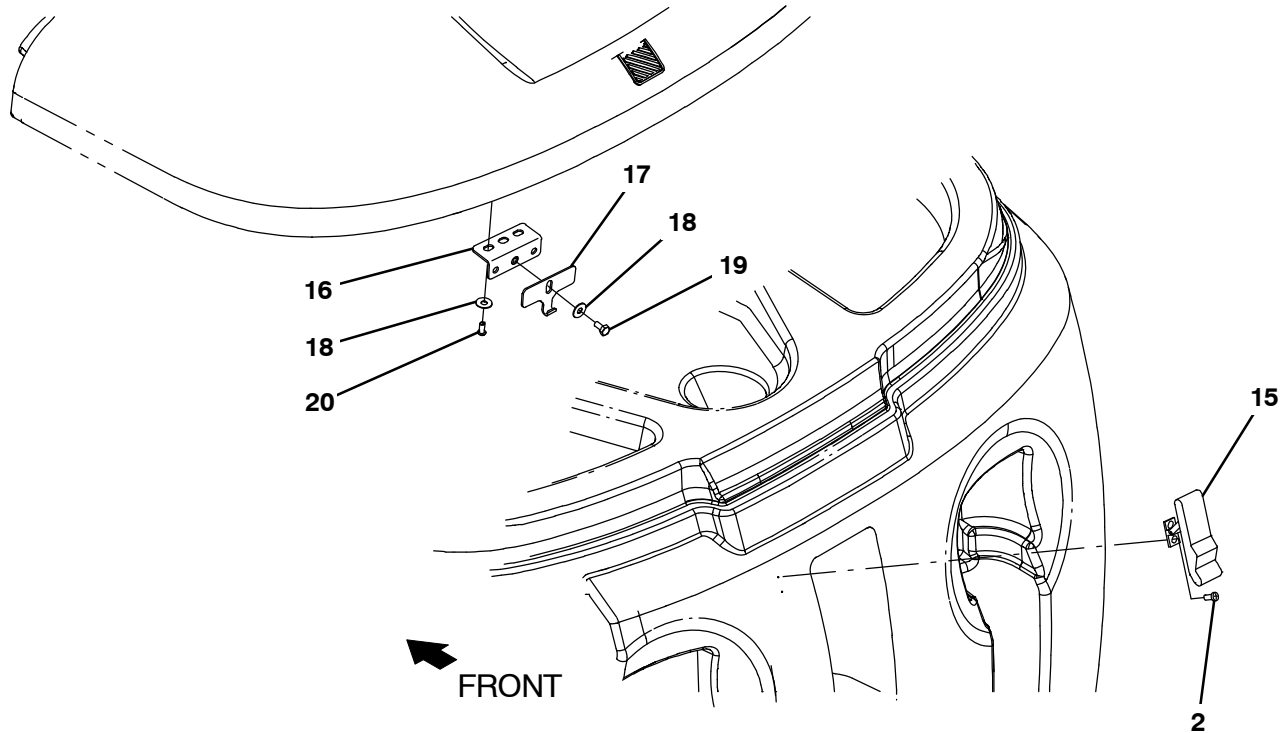
Fig. 24 – Transport Group
