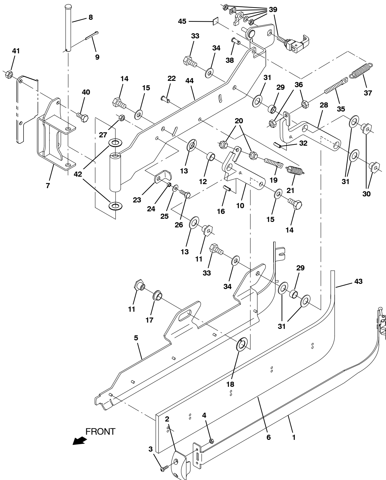
Fig. 31 – Scrub Head Side Squeegee Group, Left Hand (0000–U00837)
