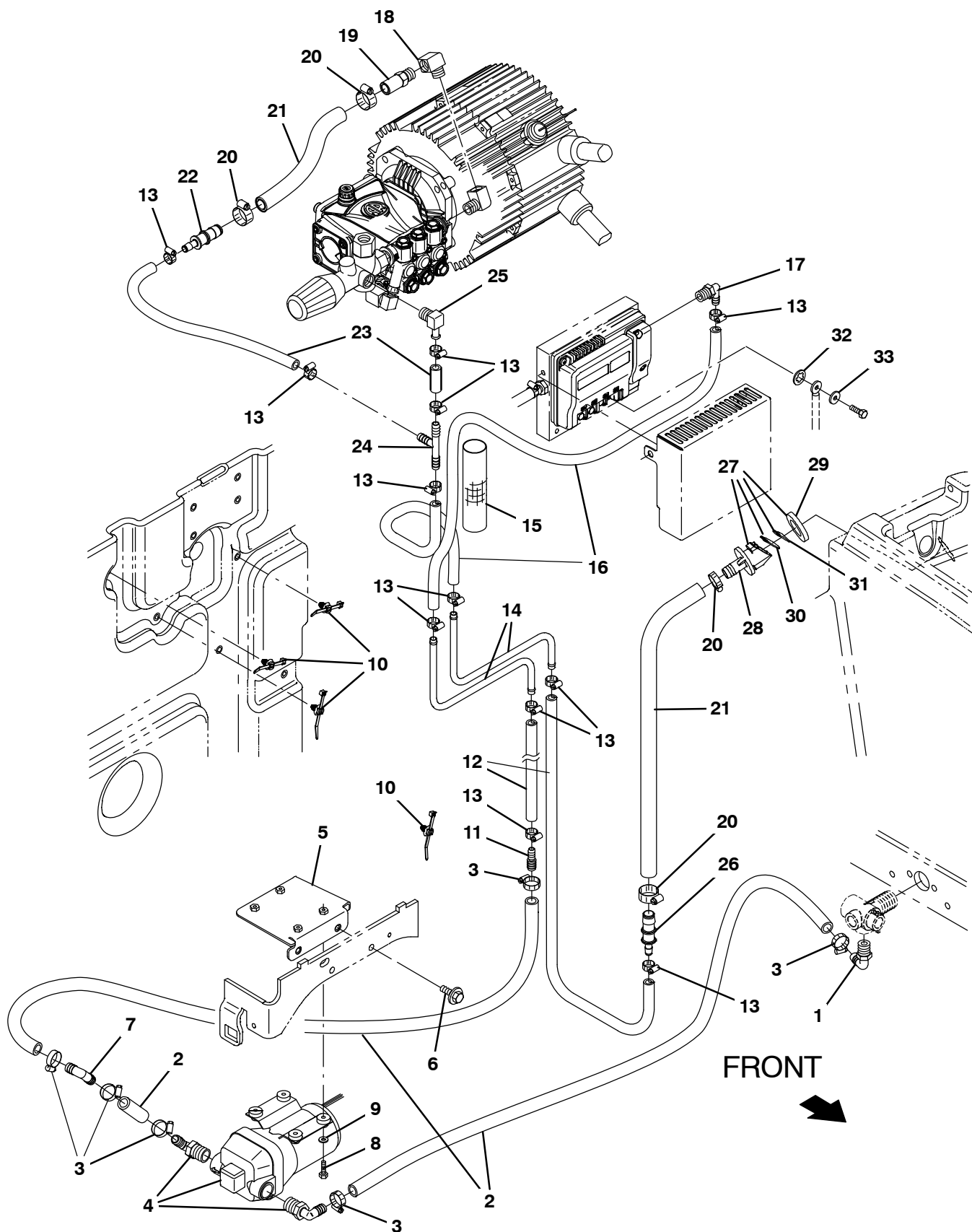
Fig. 35 – Pressure Washer Solution Supply Group (0500– )
