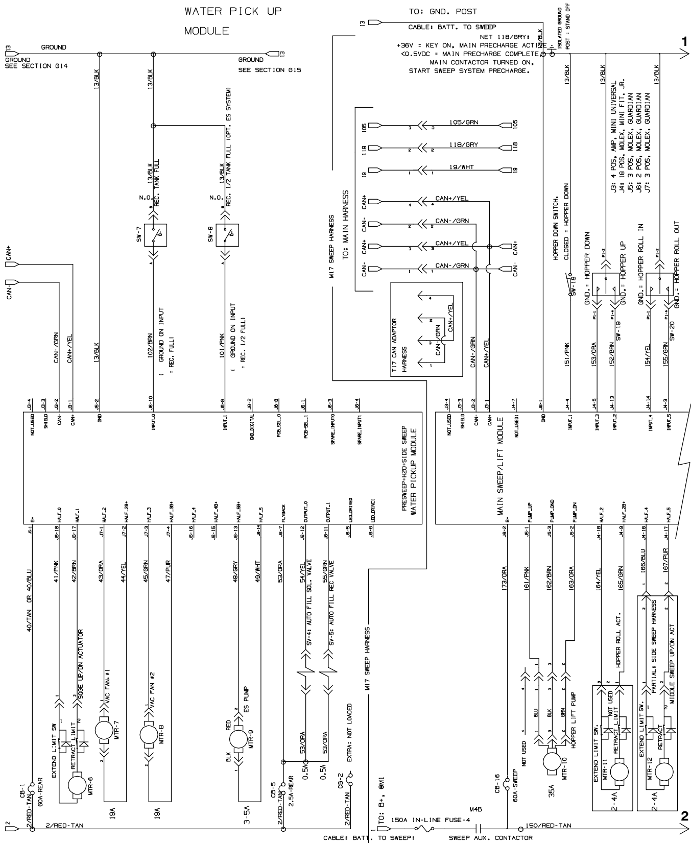
Fig. 54 – Electrical Schematic (0000–0499)
