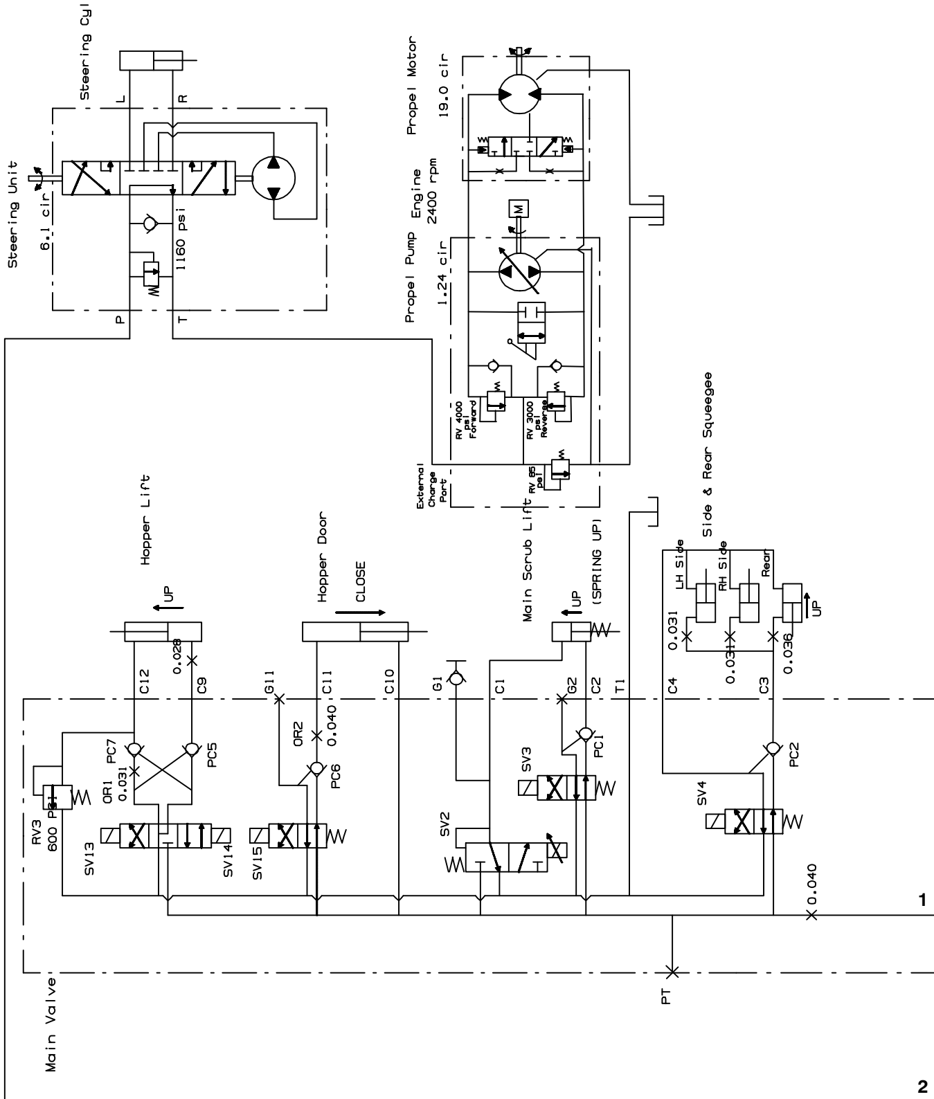
Fig. 53 – Hydraulic Schematic (0132–0270)
