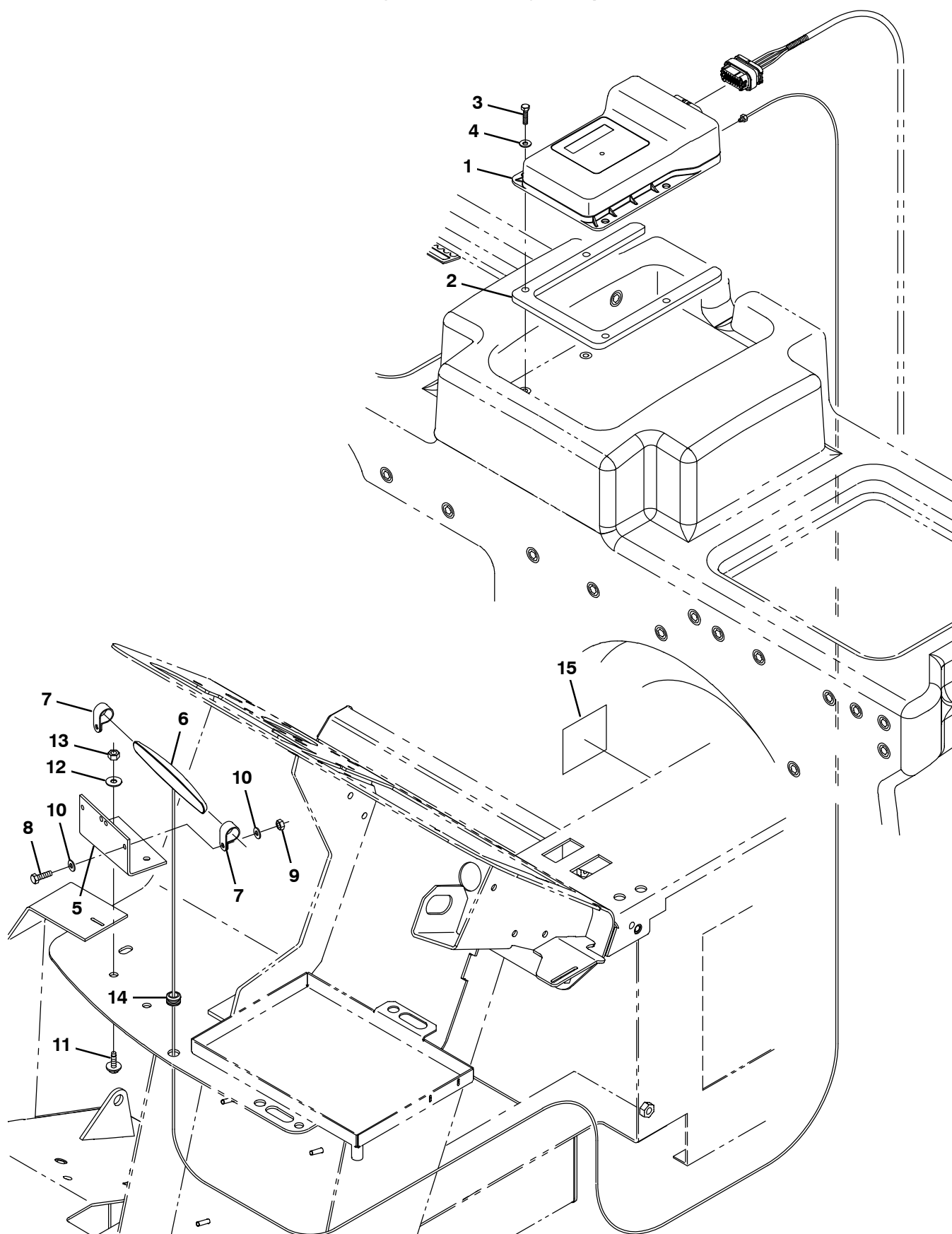
Fig. 30 – Telemetry Group
