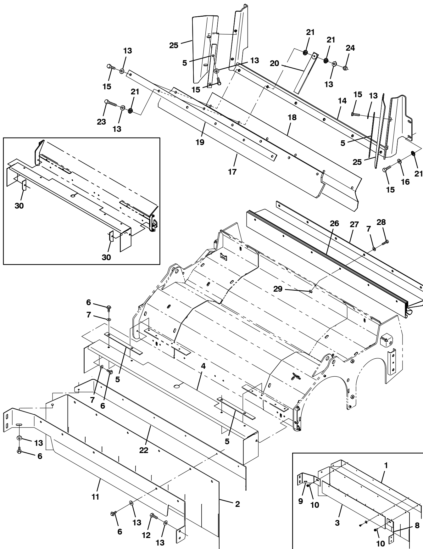
Fig. 36 – Brush Head Skirt Group
