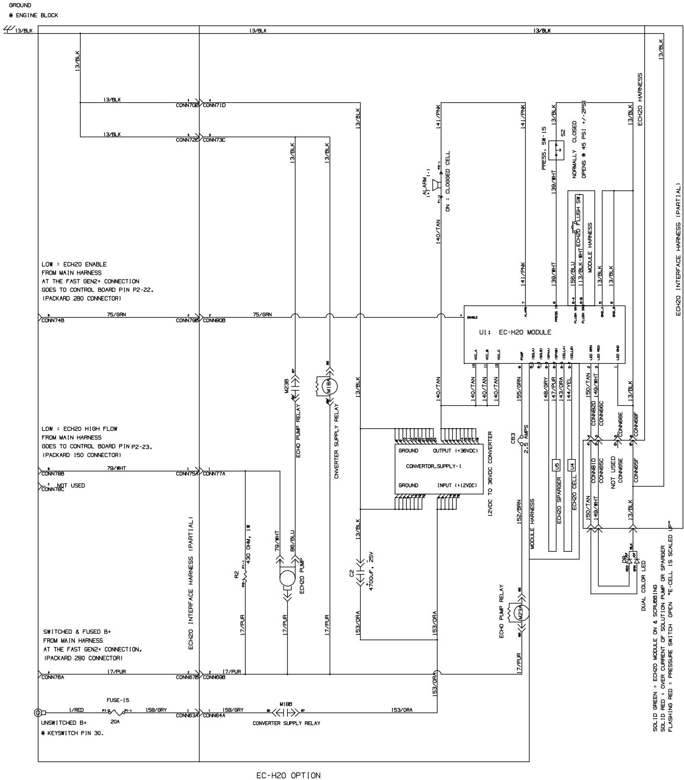
Fig. 65 – Electrical Schematic
