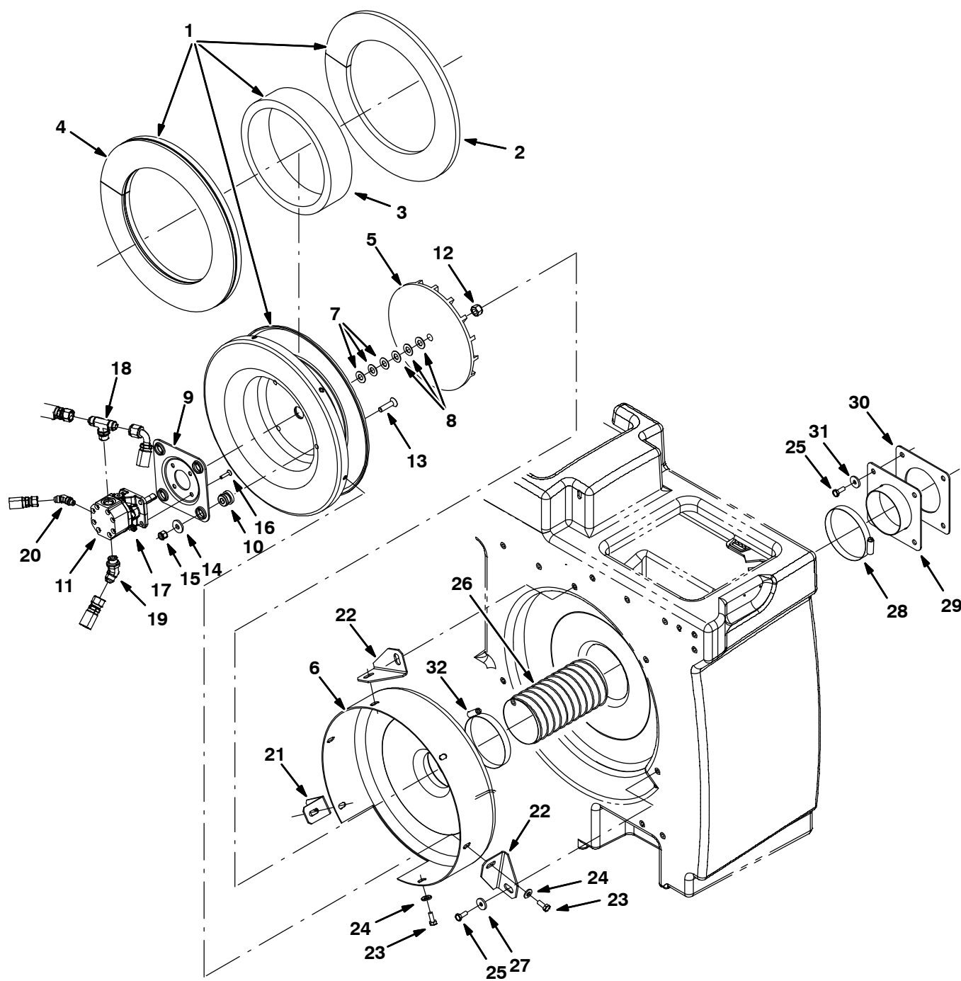
Fig. 49 – Vacuum Fan Group, Scrubbing (0000-0781)
