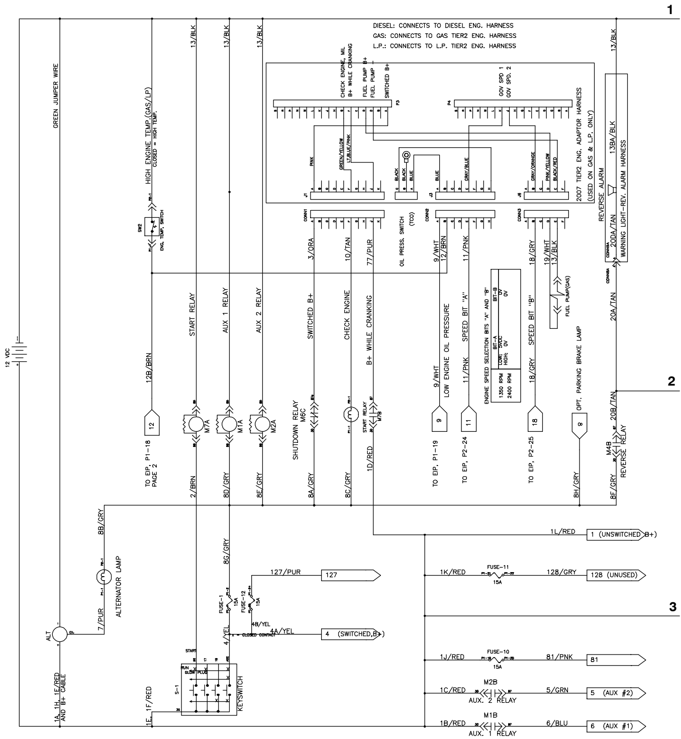
Fig. 65 – Electrical Schematic
