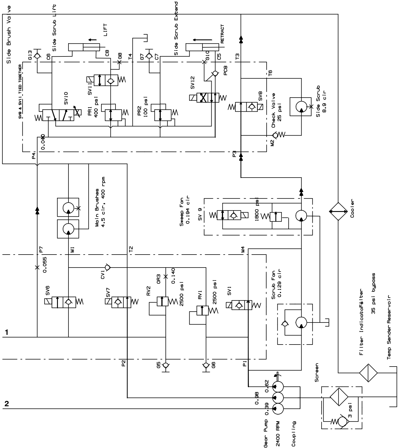
Fig. 54 – Hydraulic Schematic (0271– )
