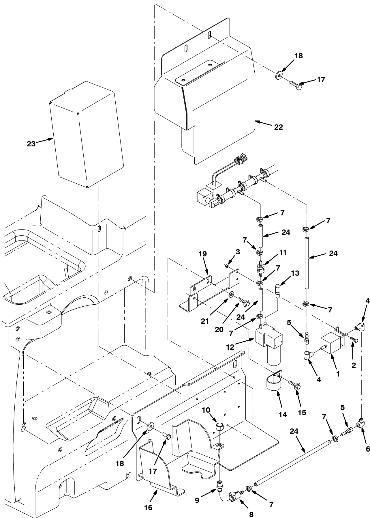
Fig. 10 – FaST Air Pump and Detergent Group (0000-0145)
