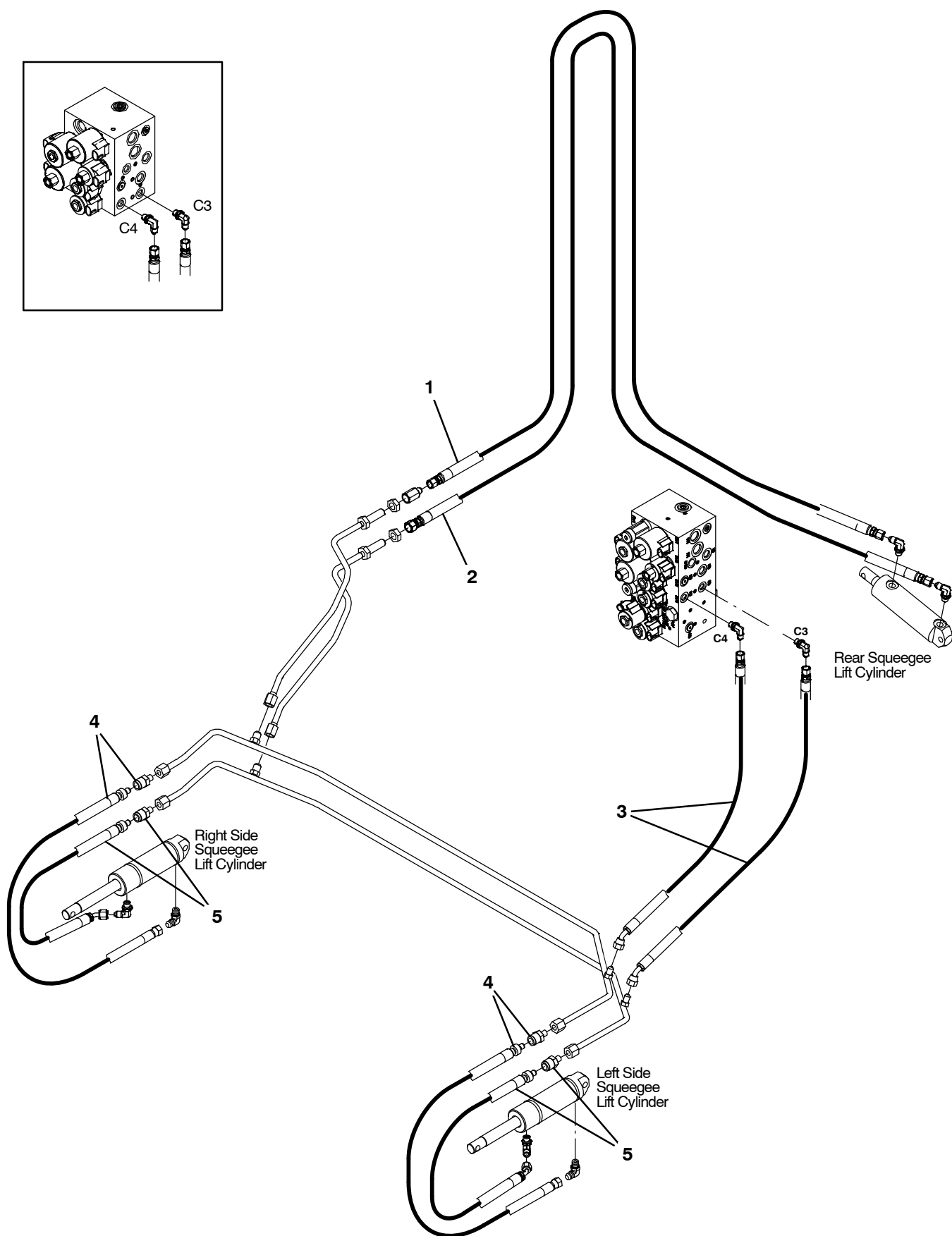
Fig. 59 – Hydraulic Hose Group, Squeegee Lift
