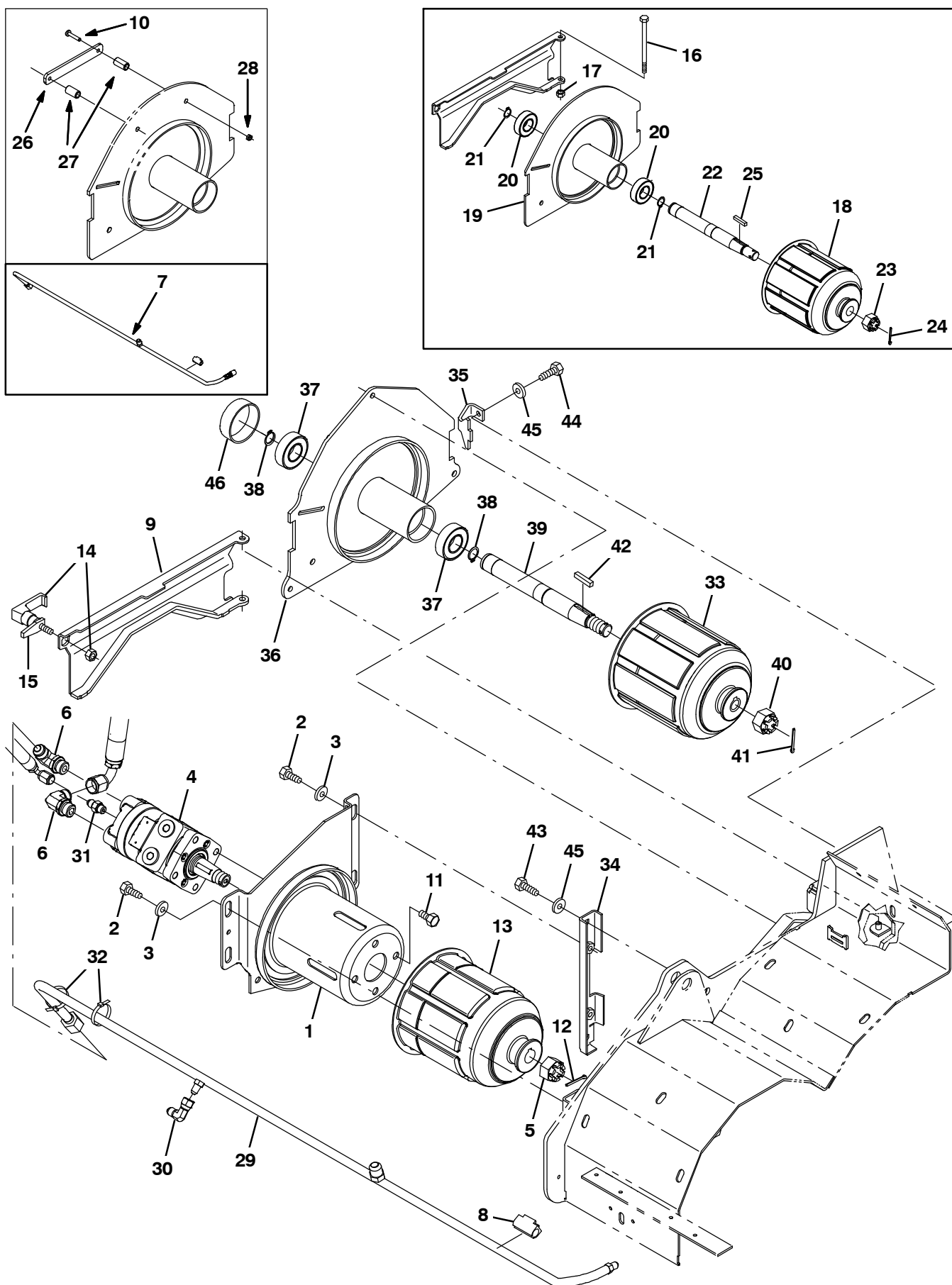
Fig. 34 – Brush Drive Group, Right Side
