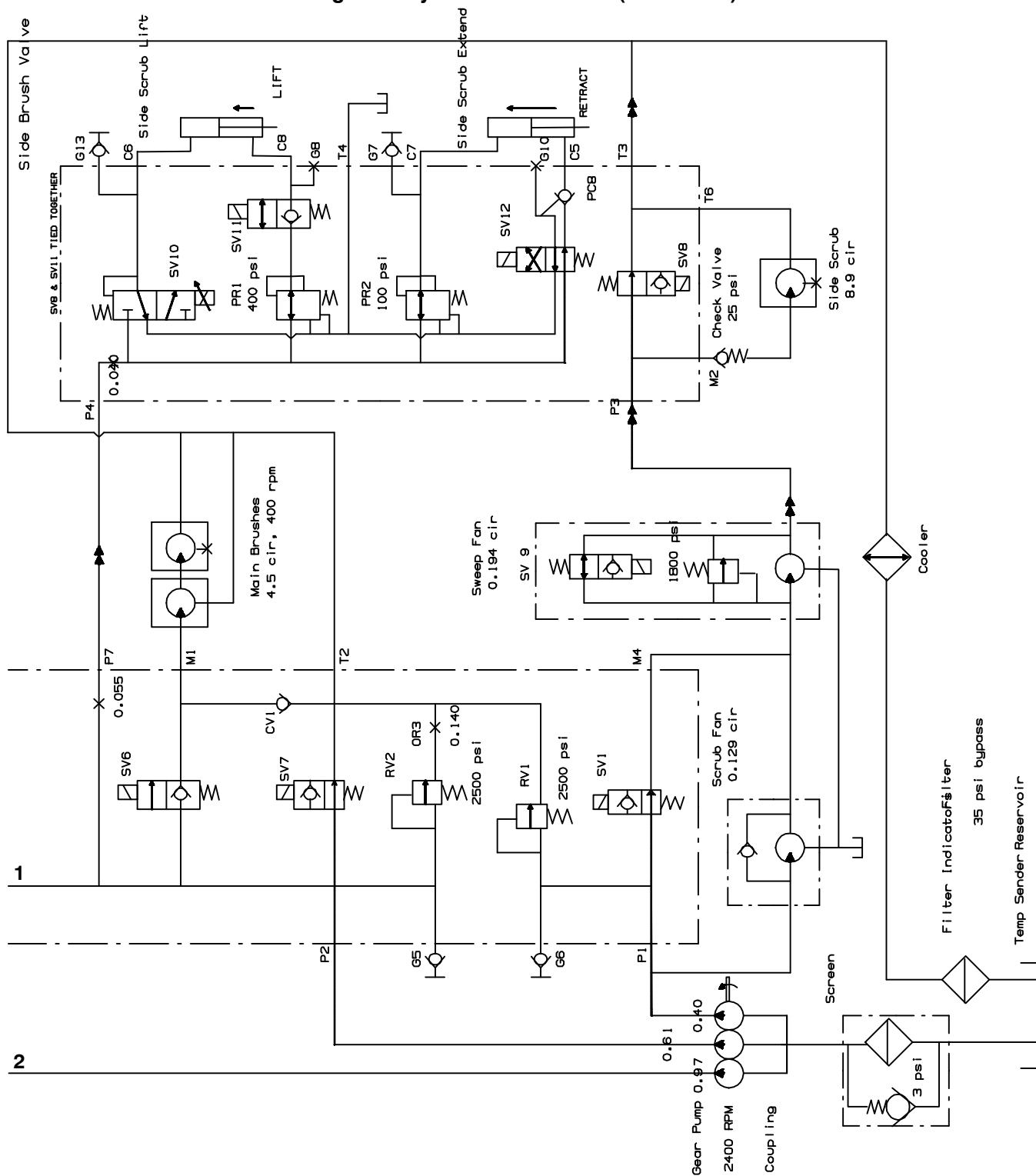
Fig. 53 – Hydraulic Schematic (0132-0270)
