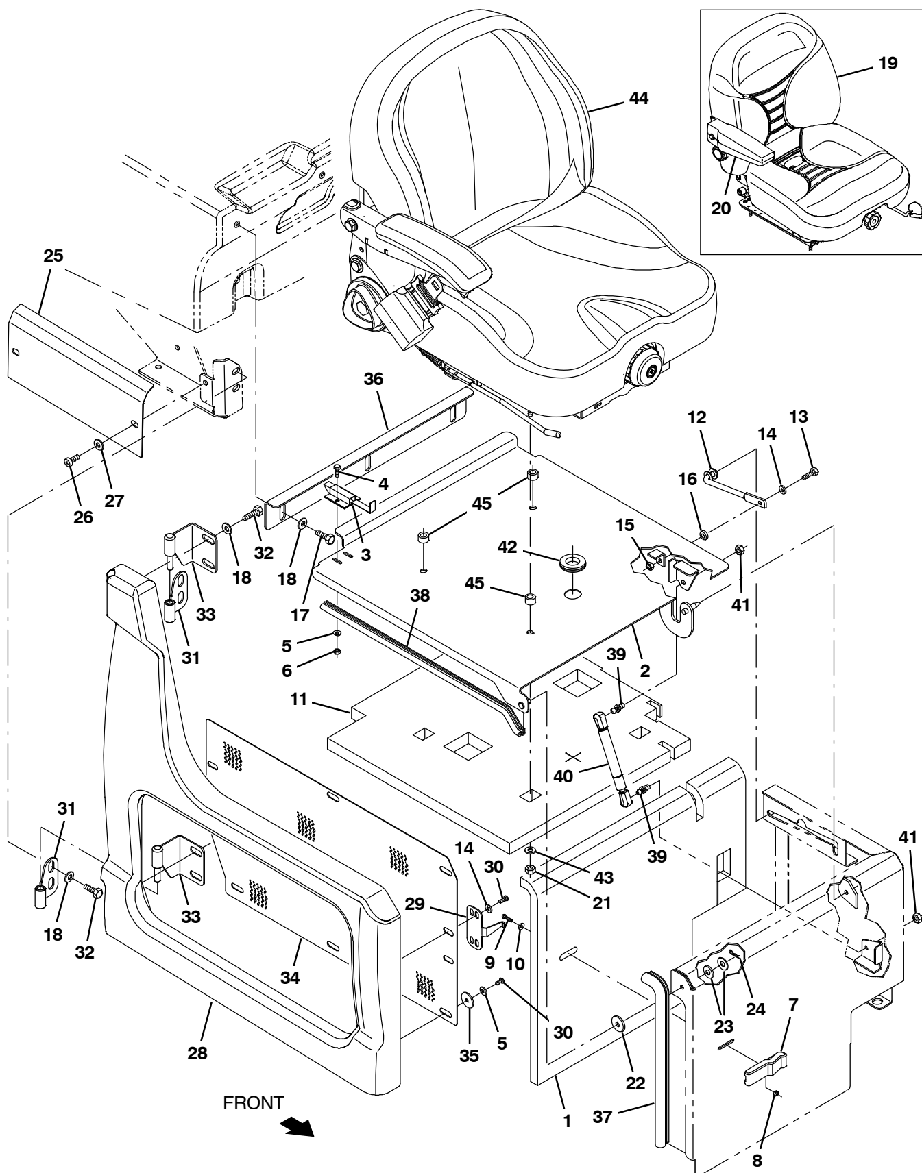
Fig. 7 – Seat Group
