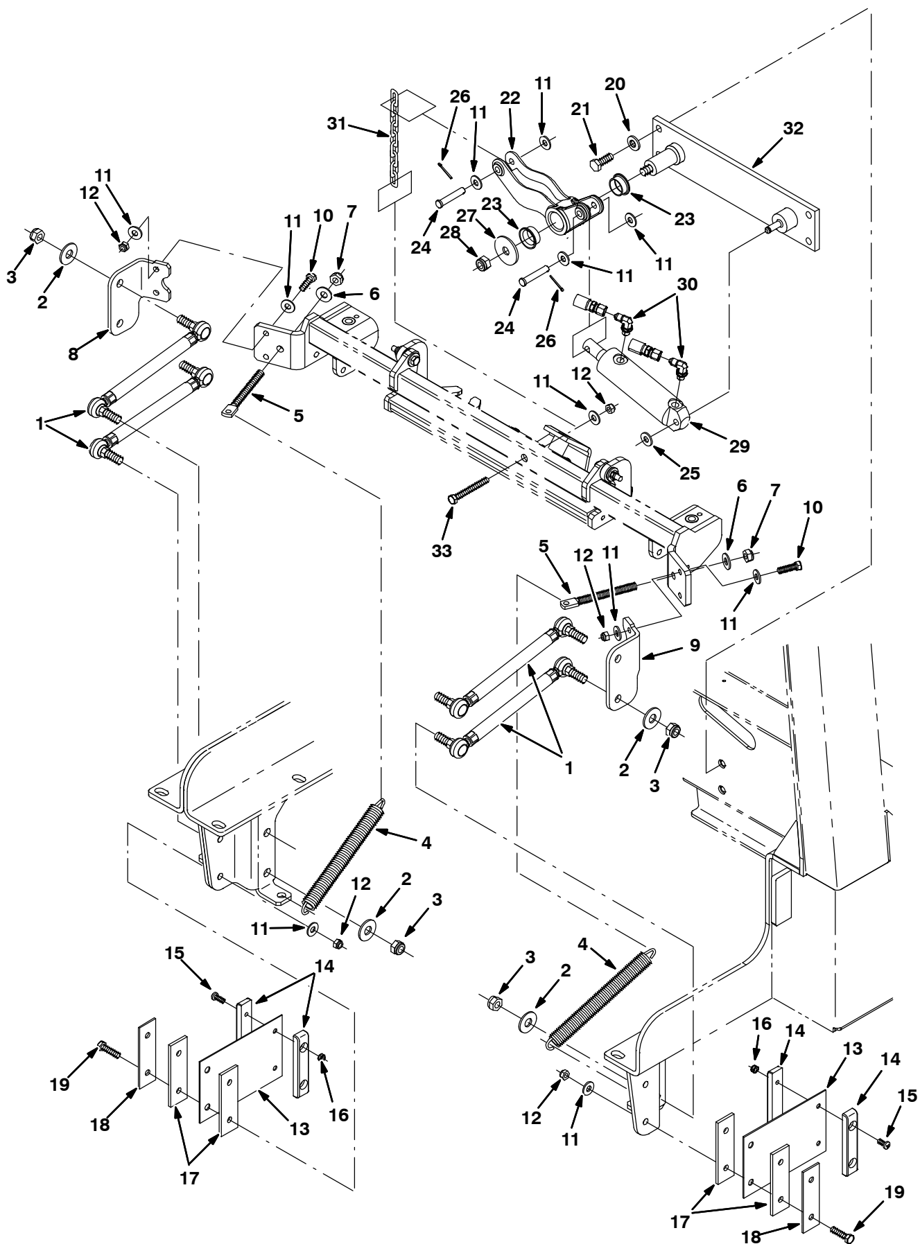
Fig. 37 – Squeegee Lift Group, Rear
