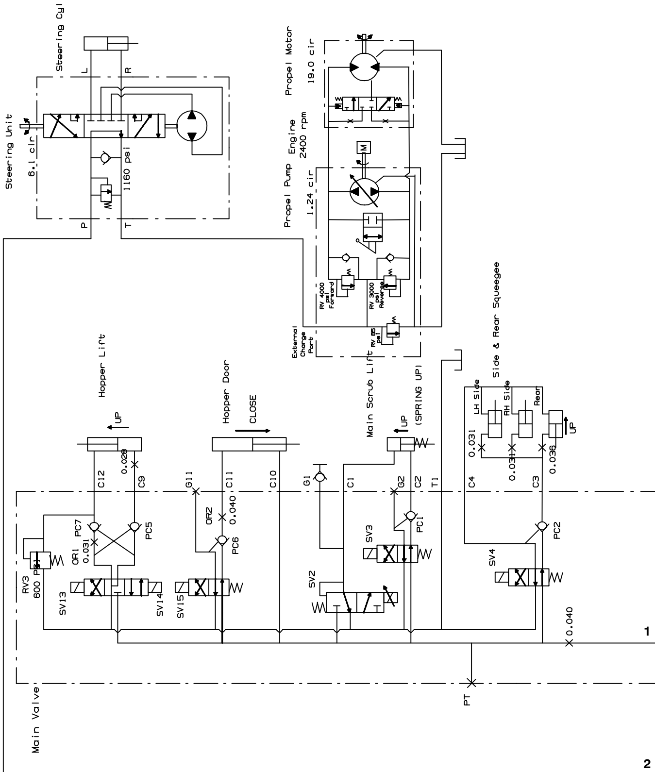
Fig. 75 – Hydraulic Schematic (0271 – )
