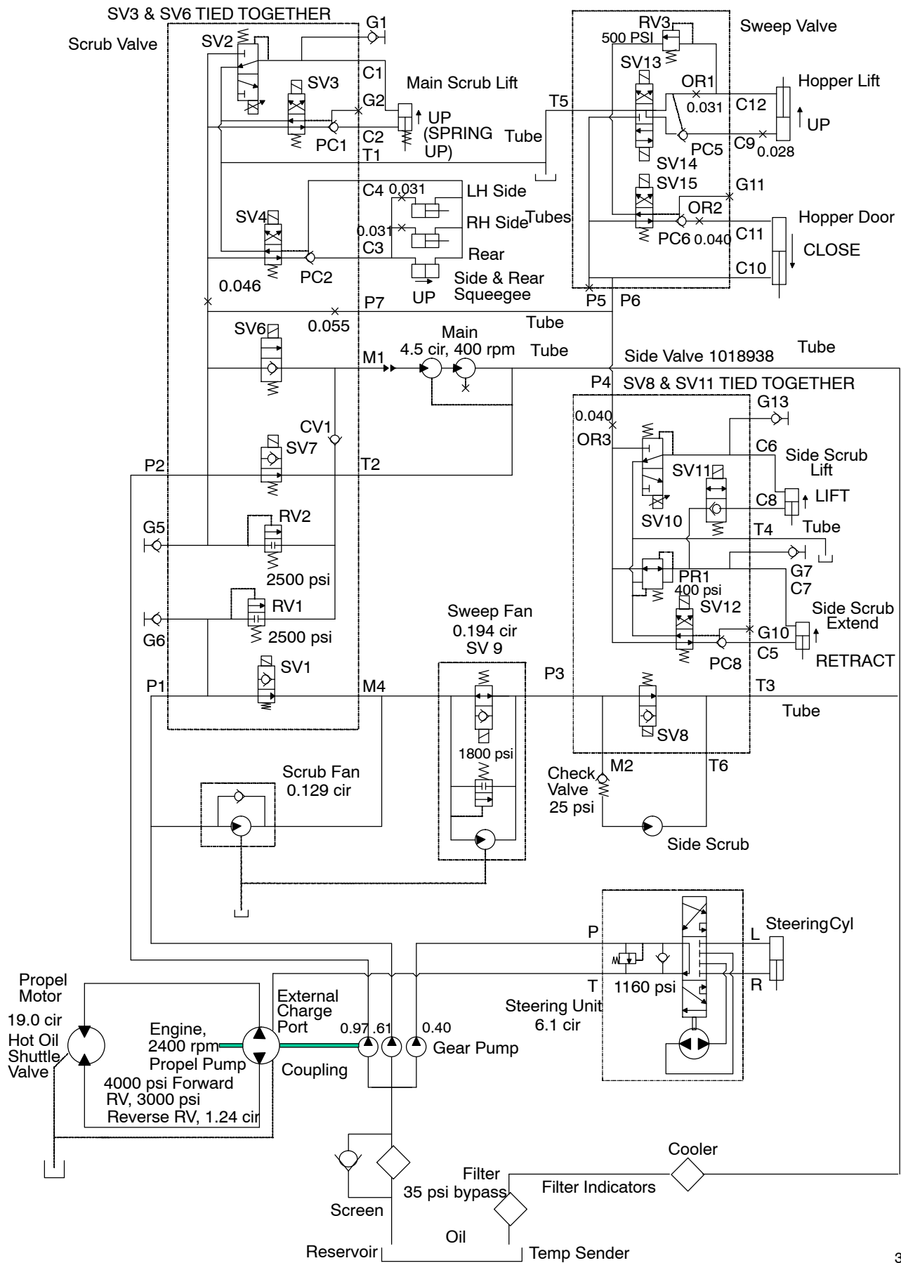
Fig. 73 – Hydraulic Schematic (0000 – 0131)
