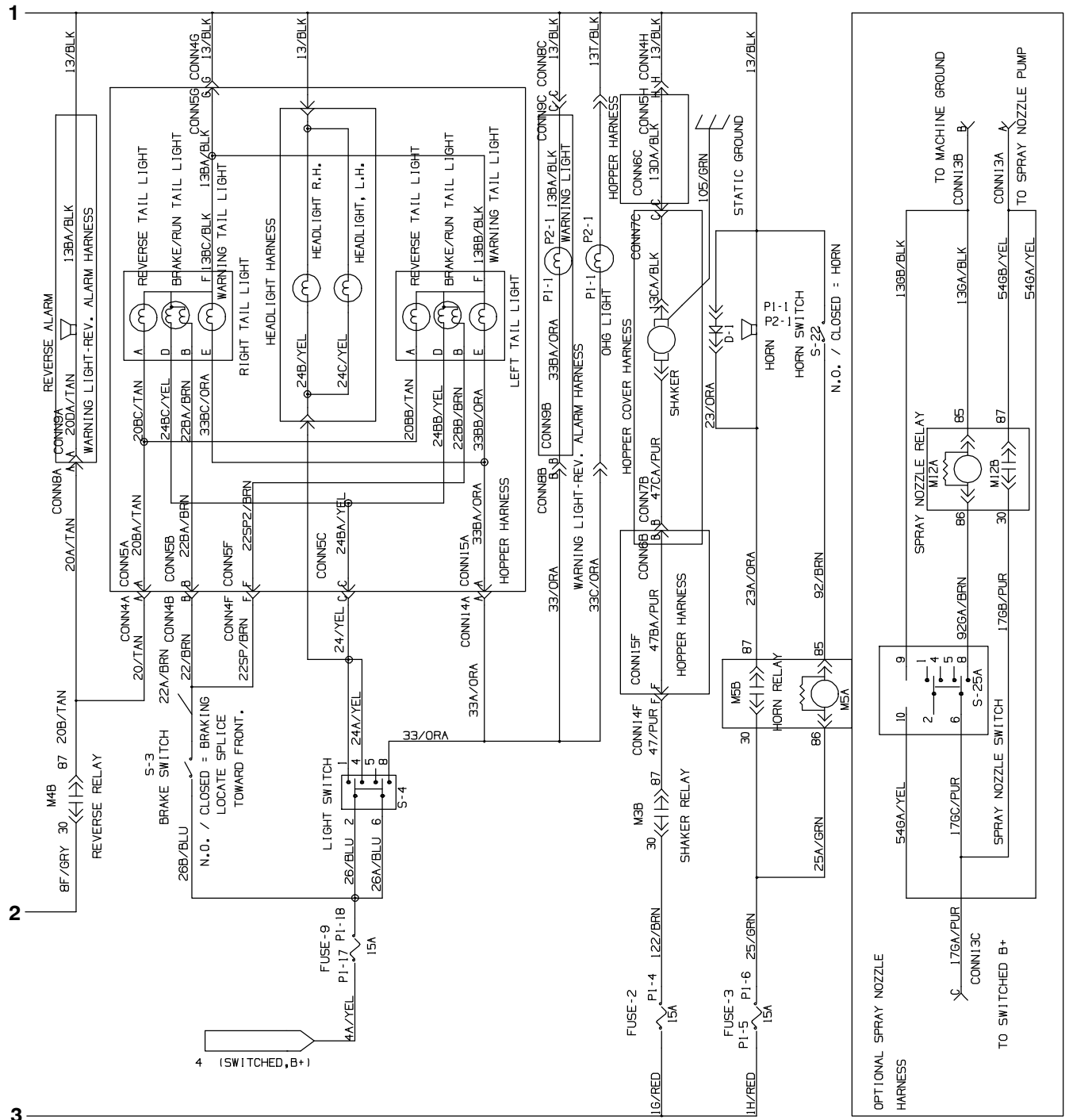
Fig. 86 – GM Electrical Schematic (0000-0046)
