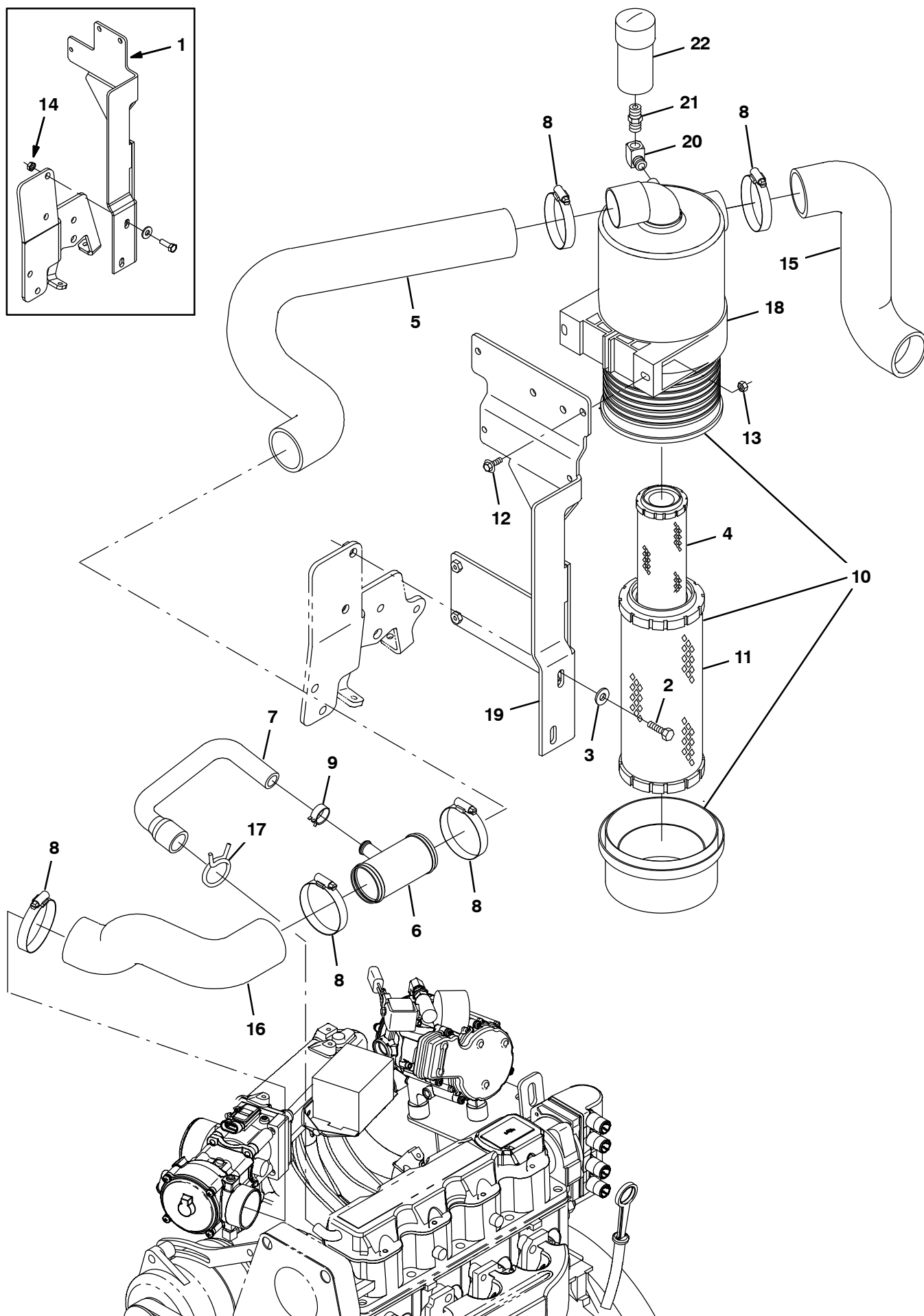
Fig. 23 – GM Engine Air Cleaner Group, LPG (0047–0499)
