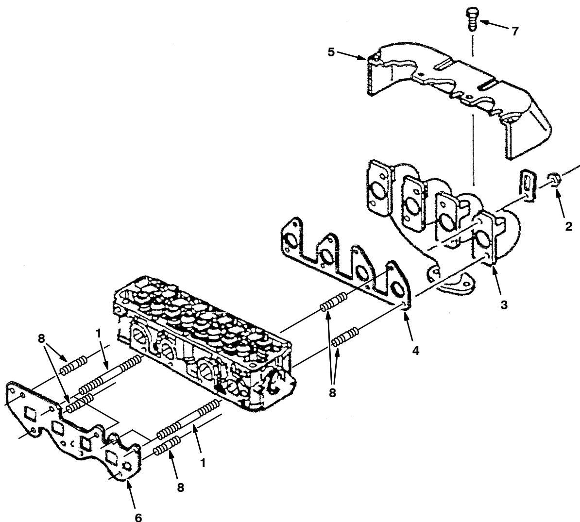
Fig. 5 – Manifold Group
