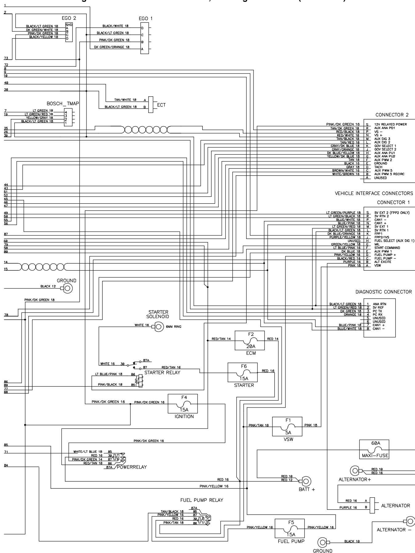
Fig. 91 – GM Electrical Schematic, Gas Engine Harness (0047-0222)
