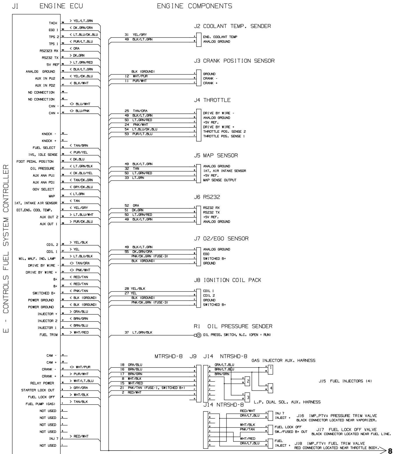
Fig. 90 – GM Electrical Schematic, Gas/LPG Engine Harness (0000–0046)
