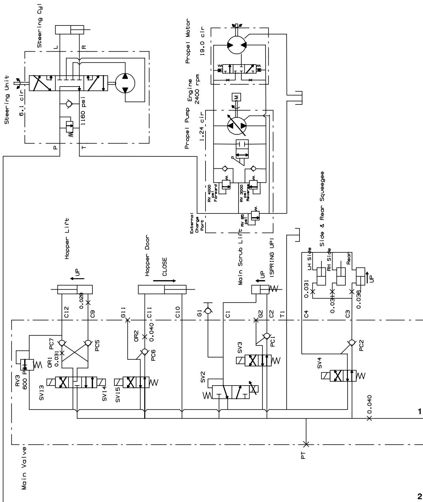
Fig. 74 – Hydraulic Schematic (0132-0270)
