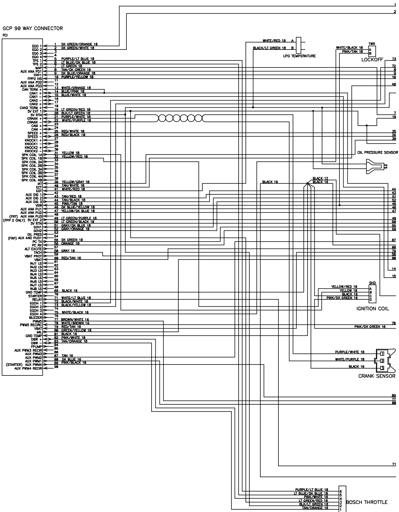
Fig. 94 – GM Electrical Schematic, LPG Engine Harness (0223-0499)
