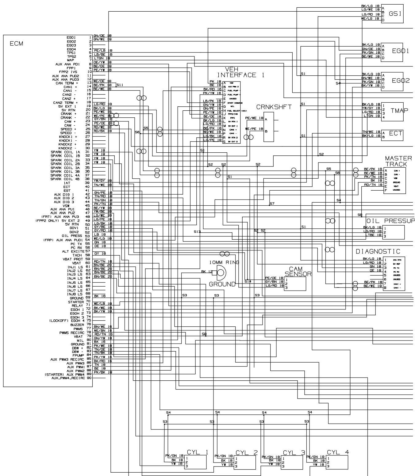
Fig. 96 – Mitsubishi Electrical Schematic, Gas Engine Harness (0500– )
