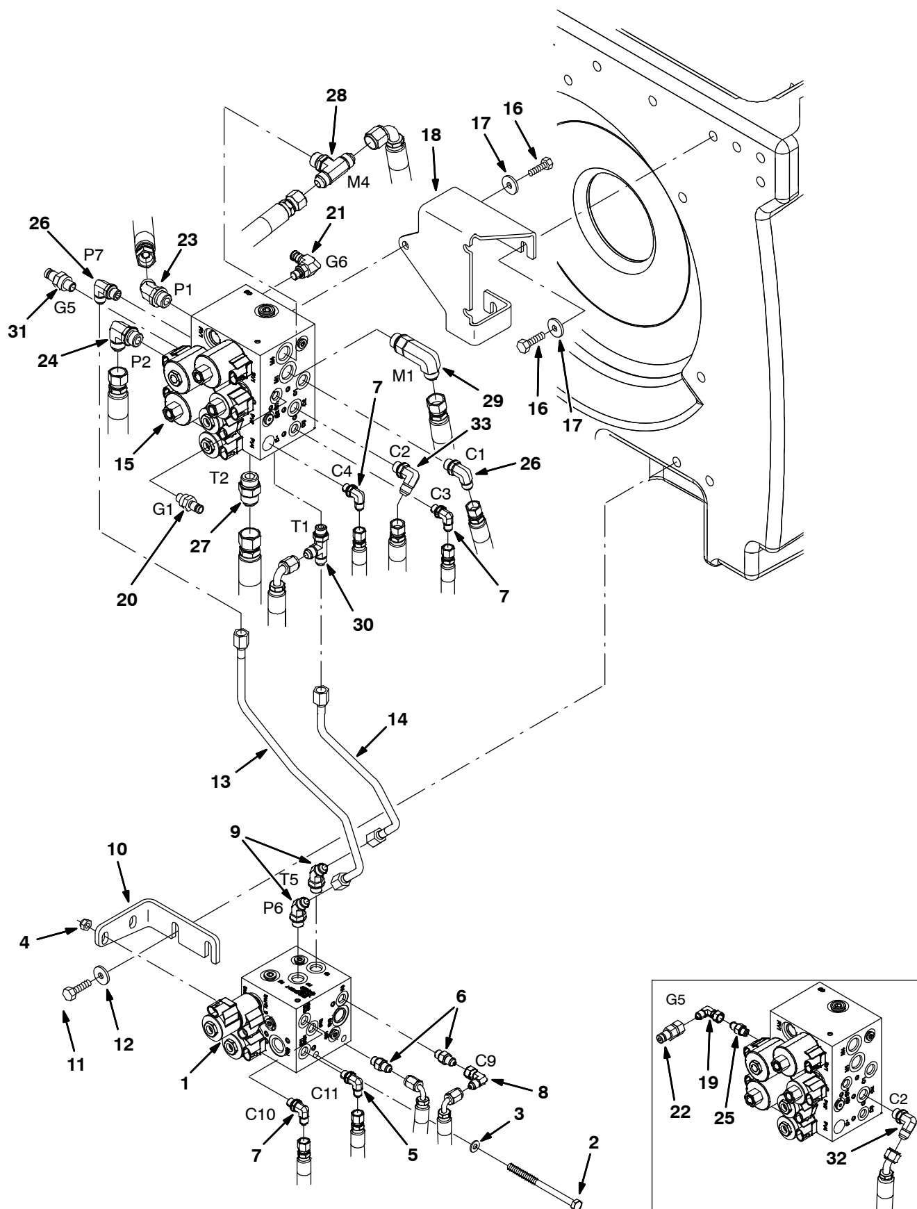
Fig. 84 – Hydraulic Valves Group (0000-0131)
