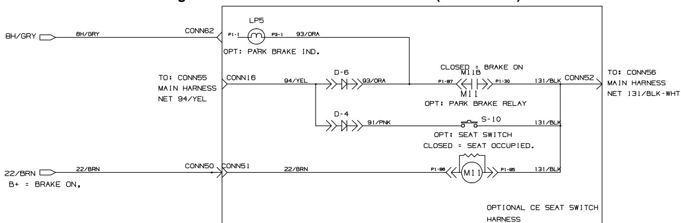
Fig. 95 – Mitsubishi Electrical Schematic (0500– )
