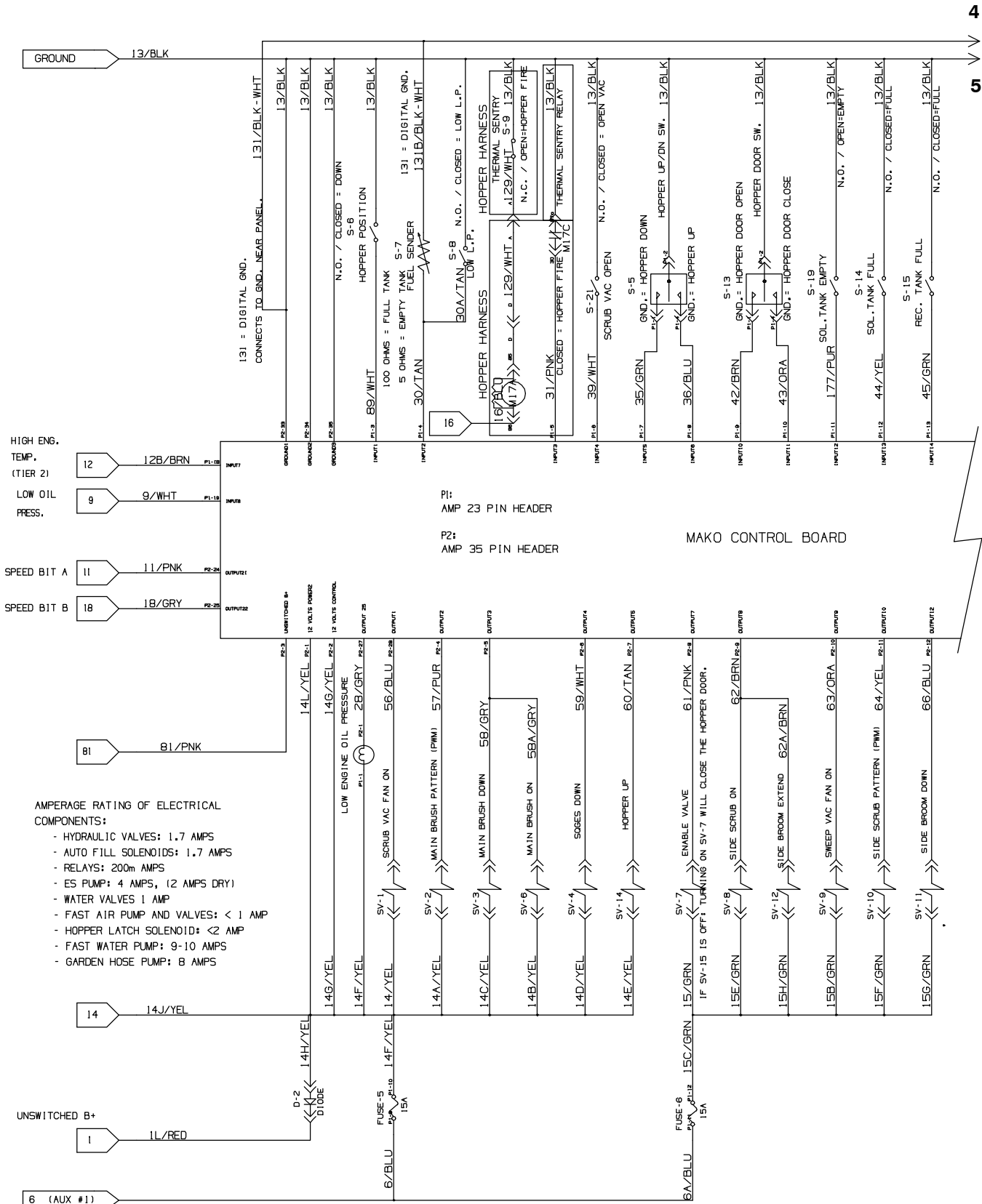
Fig. 89 – GM Electrical Schematic (xxxx-0499)
