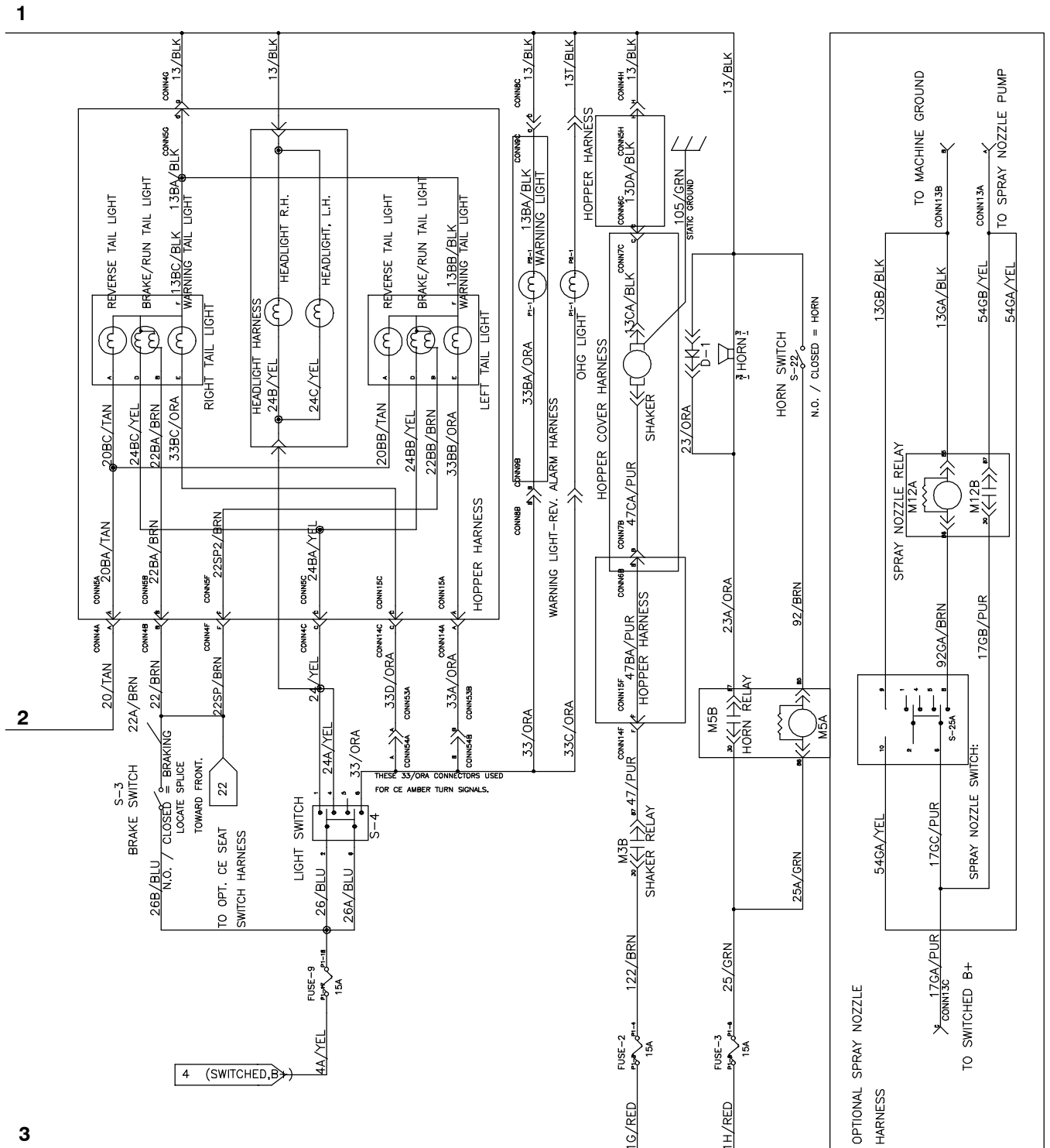
Fig. 88 – GM Electrical Schematic (0145-xxxx)
