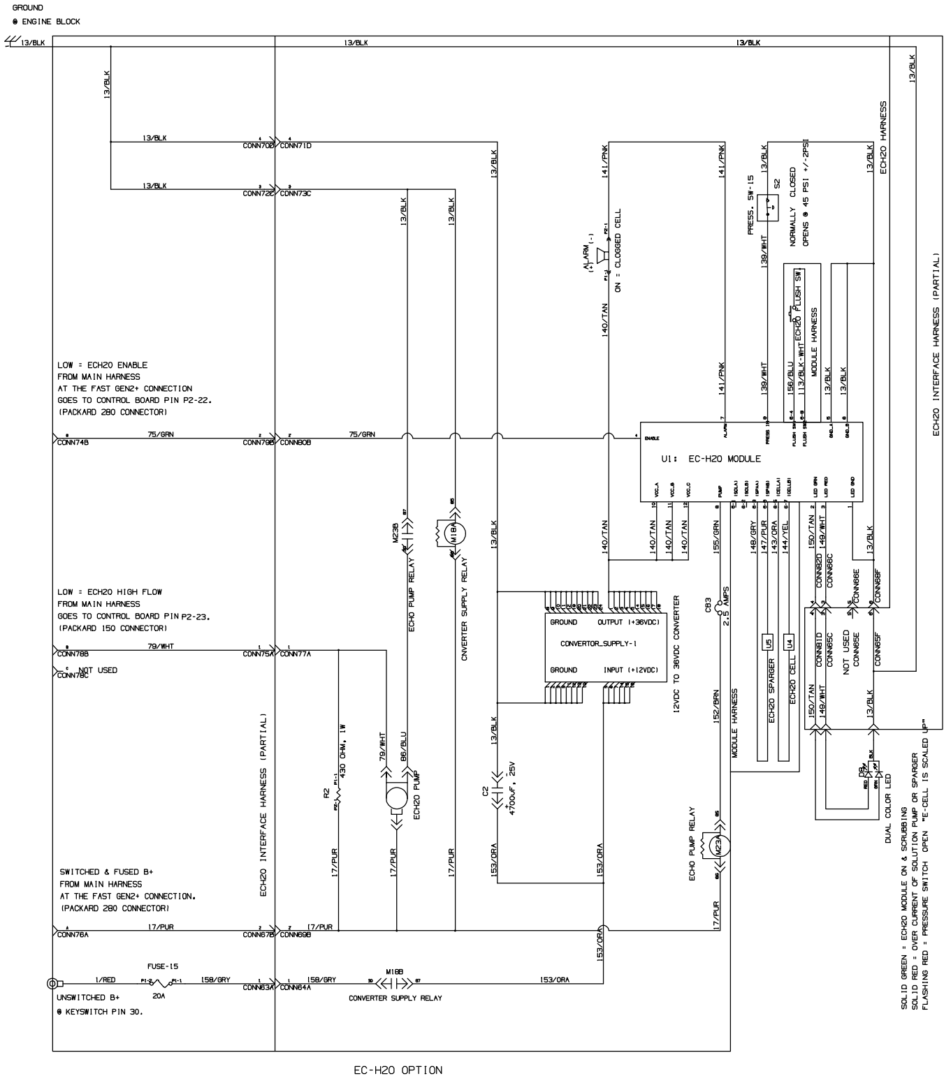
Fig. 89 – GM Electrical Schematic (xxxx-0499)
