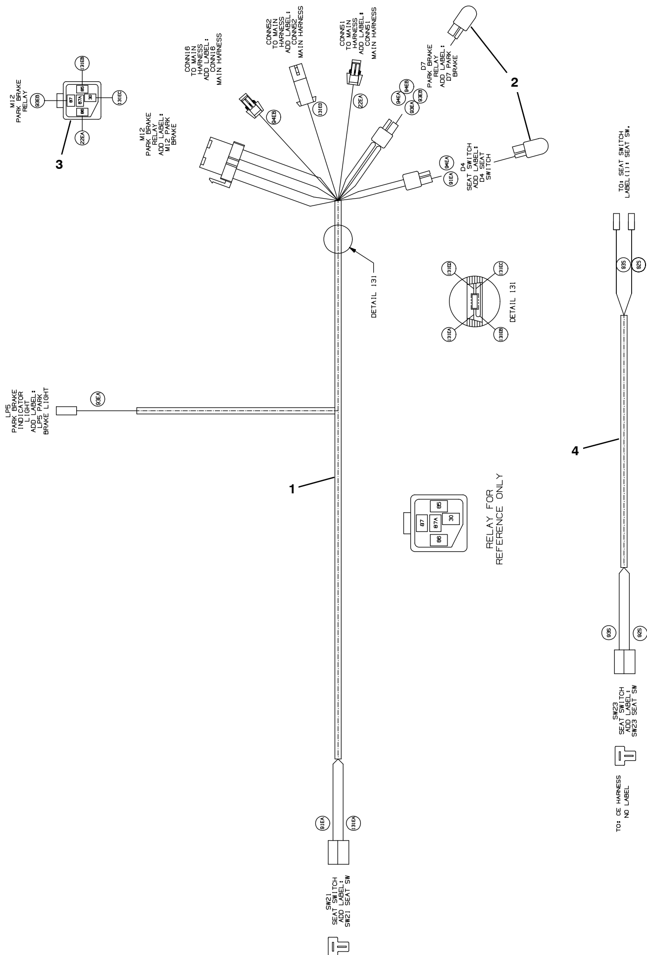
Fig. 104 – Electrical Wire Harness Group, Seat Switch
