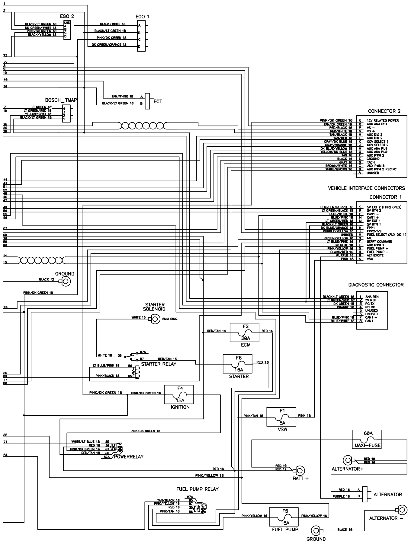
Fig. 92 – GM Electrical Schematic, Gas Engine Harness (0223-0499)
