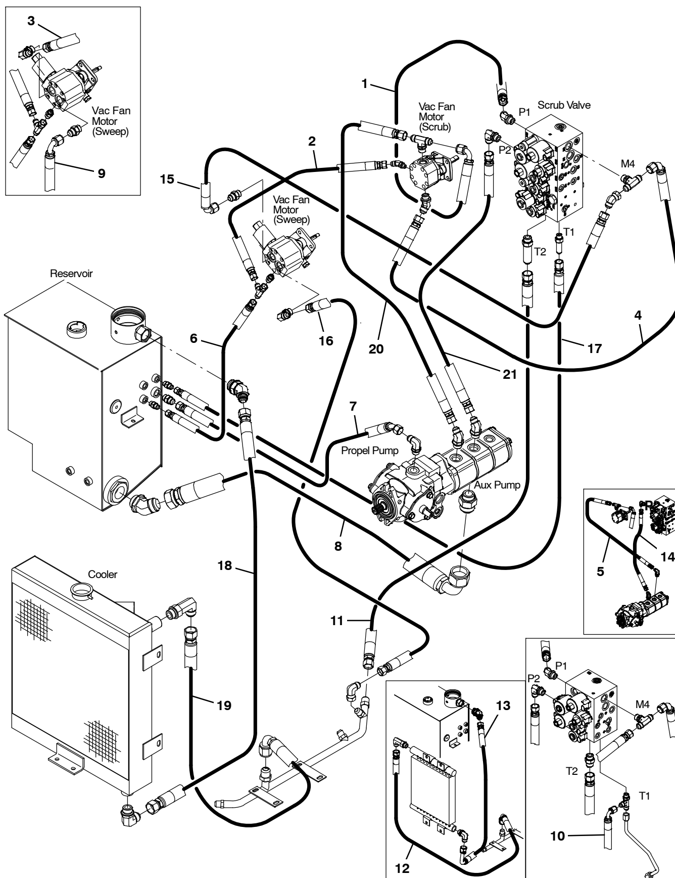
Fig. 77 – Hydraulic Hose Group, Pump and Vacuum Fans (0000-0776)
