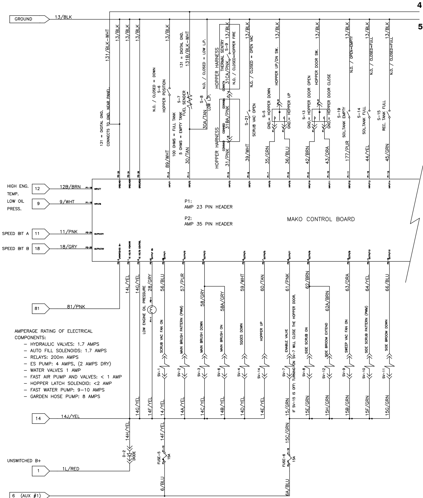
Fig. 88 – GM Electrical Schematic (0145-xxxx)
