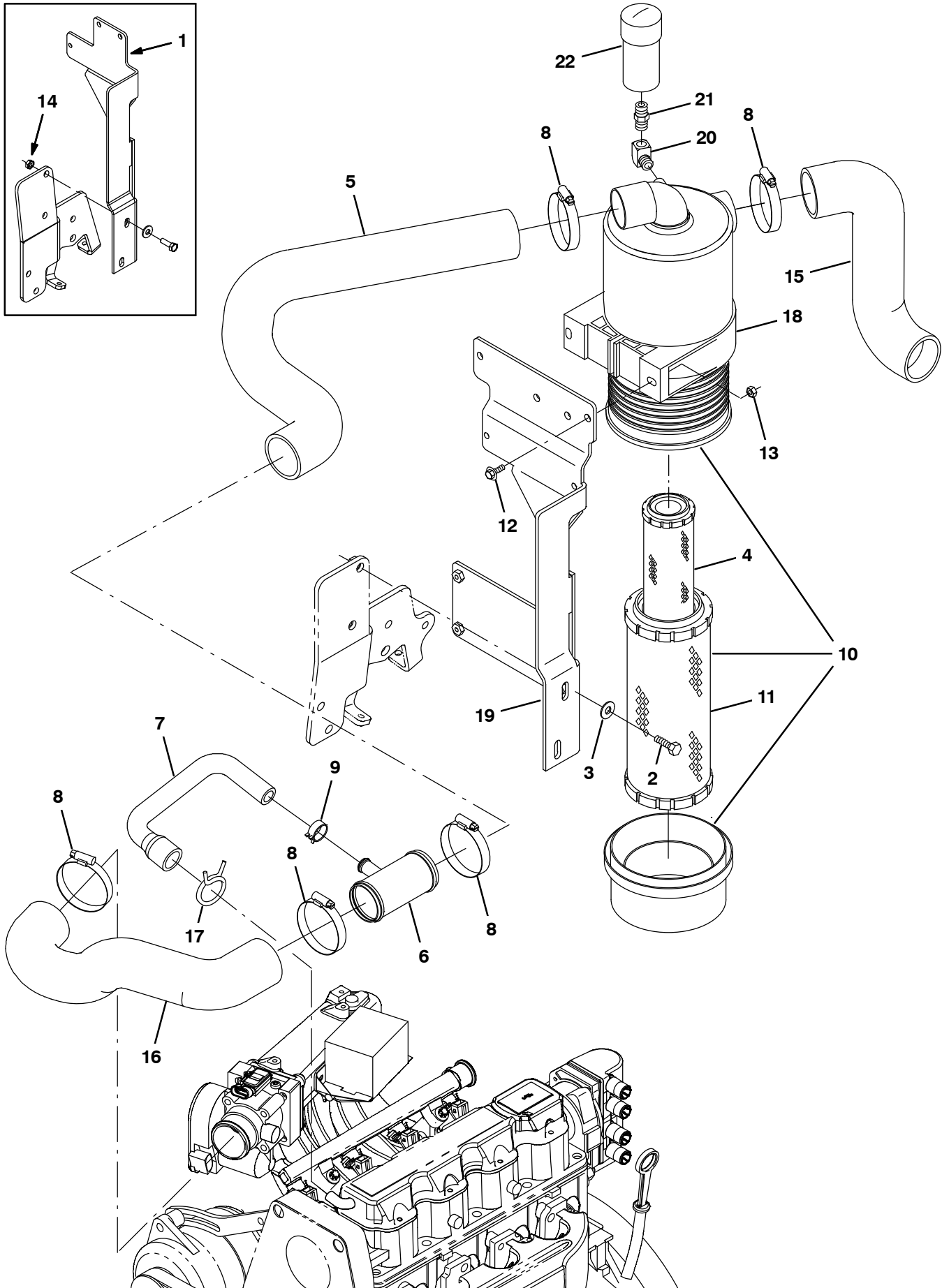
Fig. 21 – GM Engine Air Cleaner Group, Gasoline (0047–0499)
