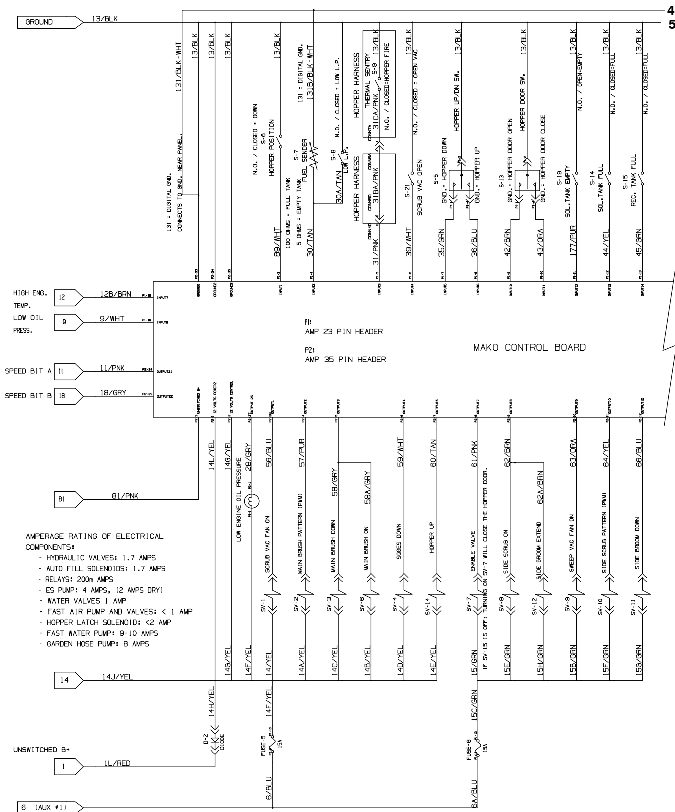
Fig. 87 – GM Electrical Schematic (0047-0145)
