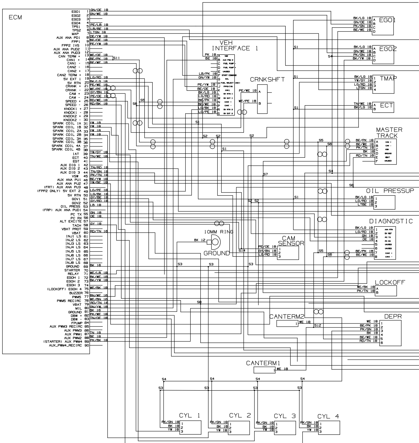
Fig. 97 – Mitsubishi Electrical Schematic, LPG Engine Harness (0500– )
