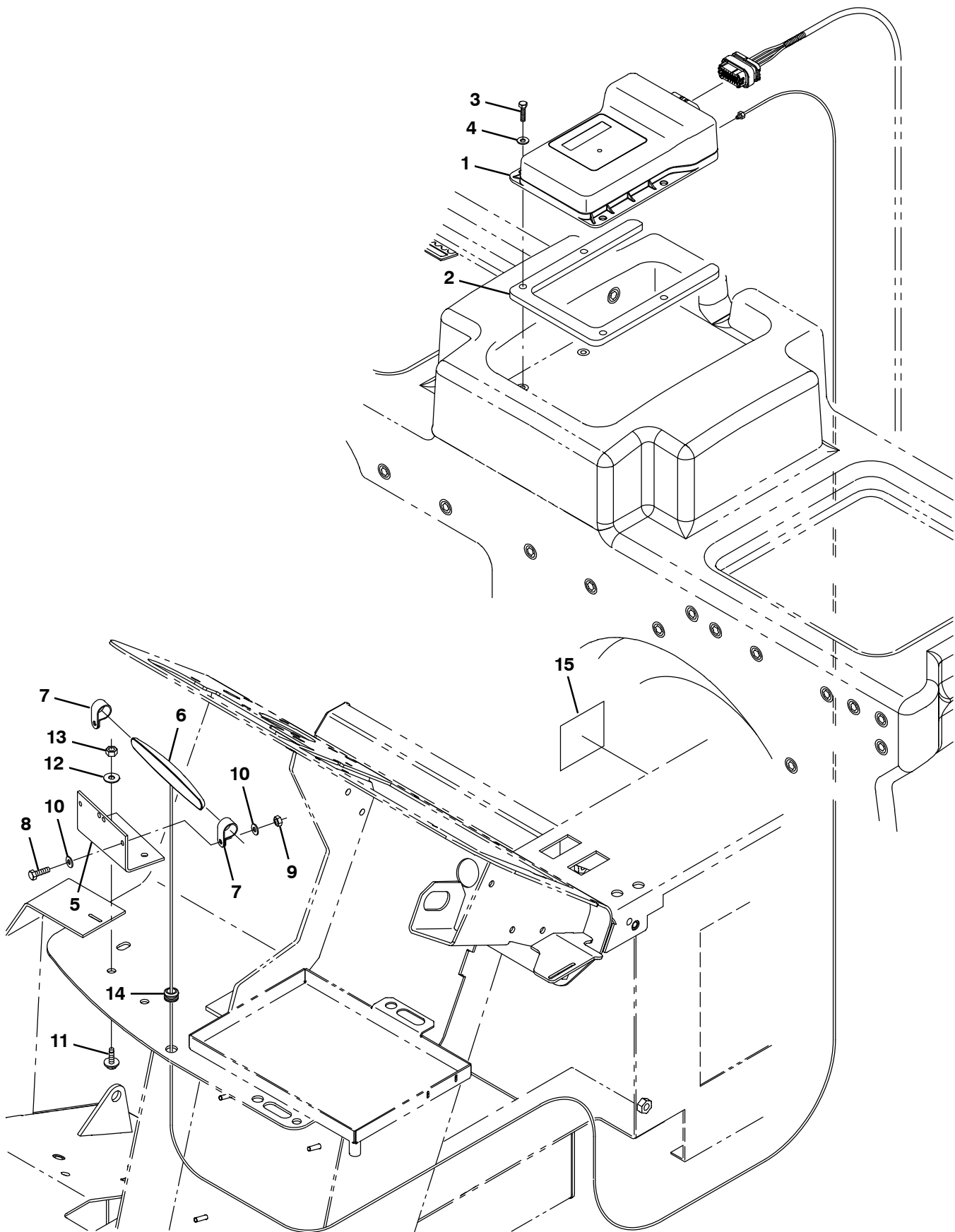
Fig. 31 – Telemetry Group
