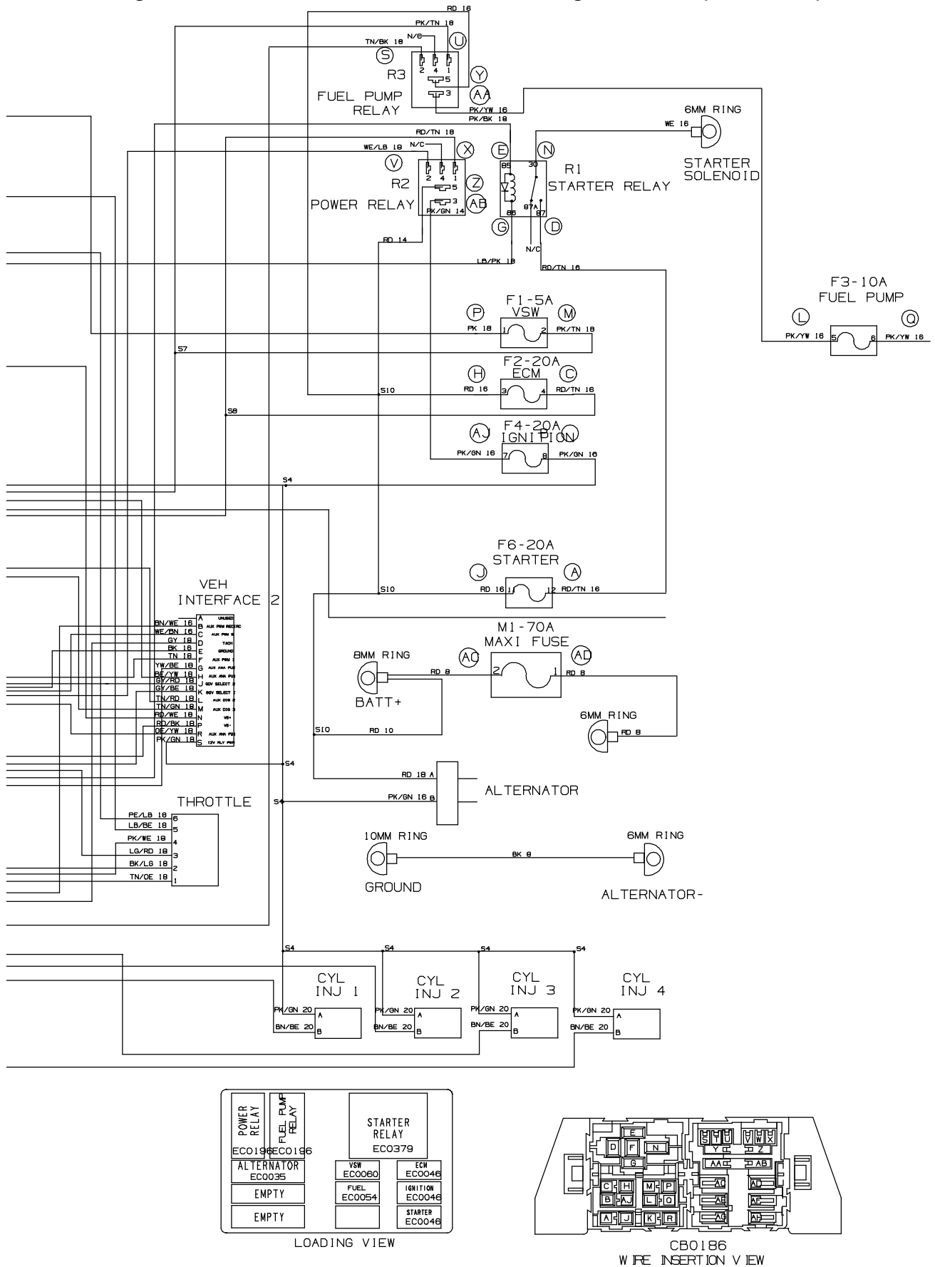
Fig. 96 – Mitsubishi Electrical Schematic, Gas Engine Harness (0500– )
