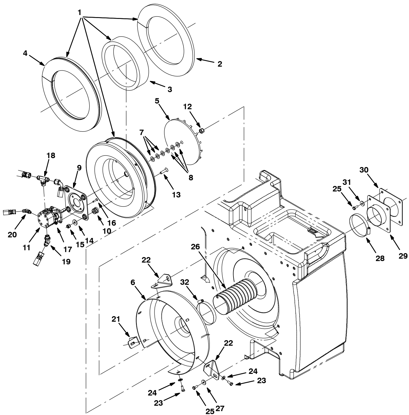
Fig. 70 – Vacuum Fan Group, Scrubbing (0000-0781)
