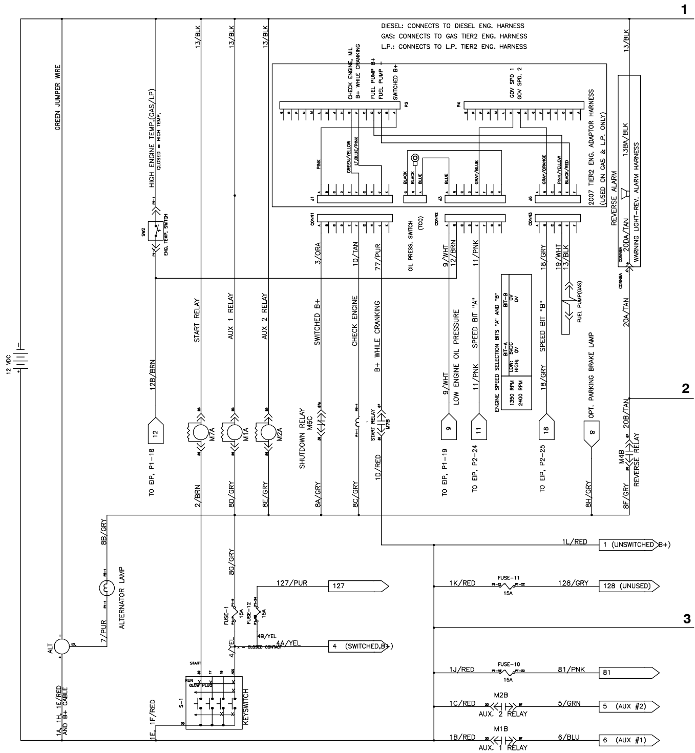
Fig. 89 – GM Electrical Schematic (xxxx-0499)
