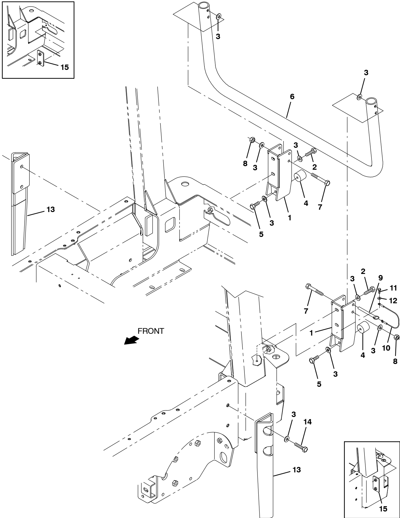
Fig. 30 – Squeegee Guard Kit
