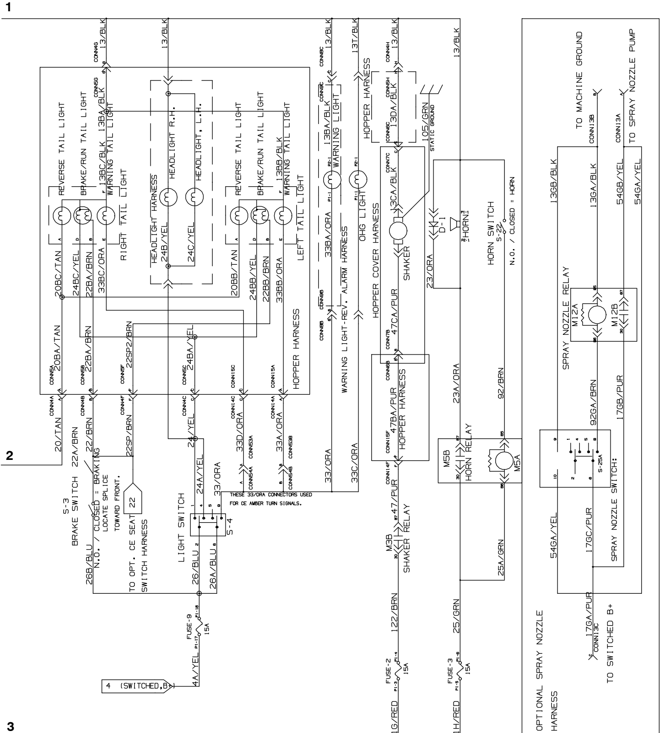
Fig. 95 - Mitsubishi Electrical Schematic (0500-
