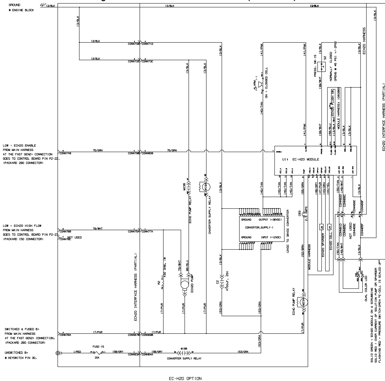
Fig. 95 – Mitsubishi Electrical Schematic (0500– )
