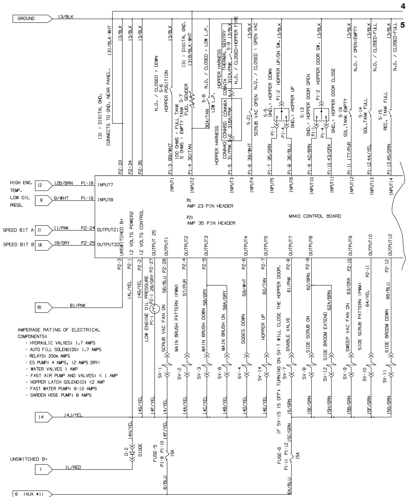
Fig. 86 – GM Electrical Schematic (0000–0046)
