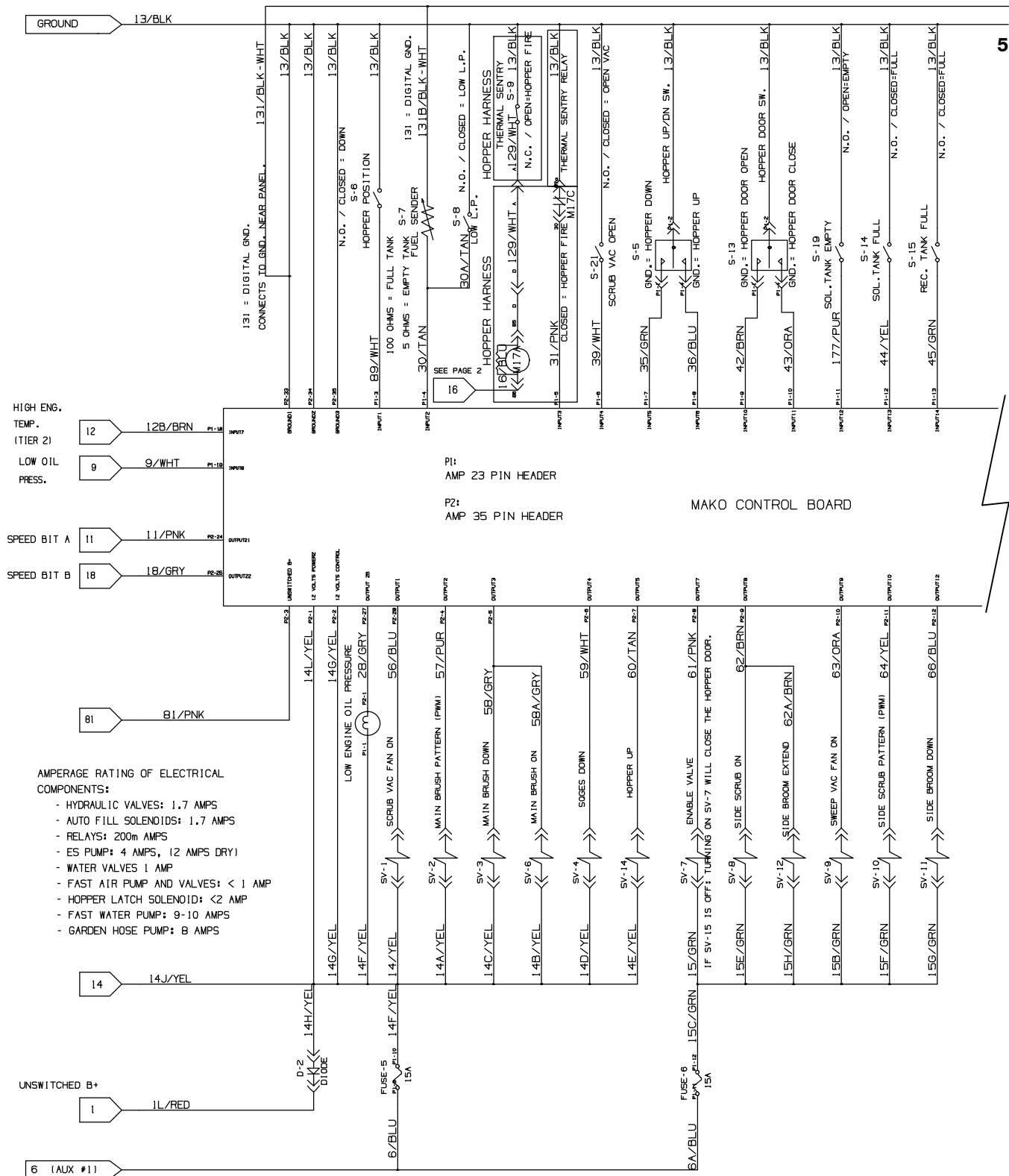
Fig. 95 – Mitsubishi Electrical Schematic (0500– )
