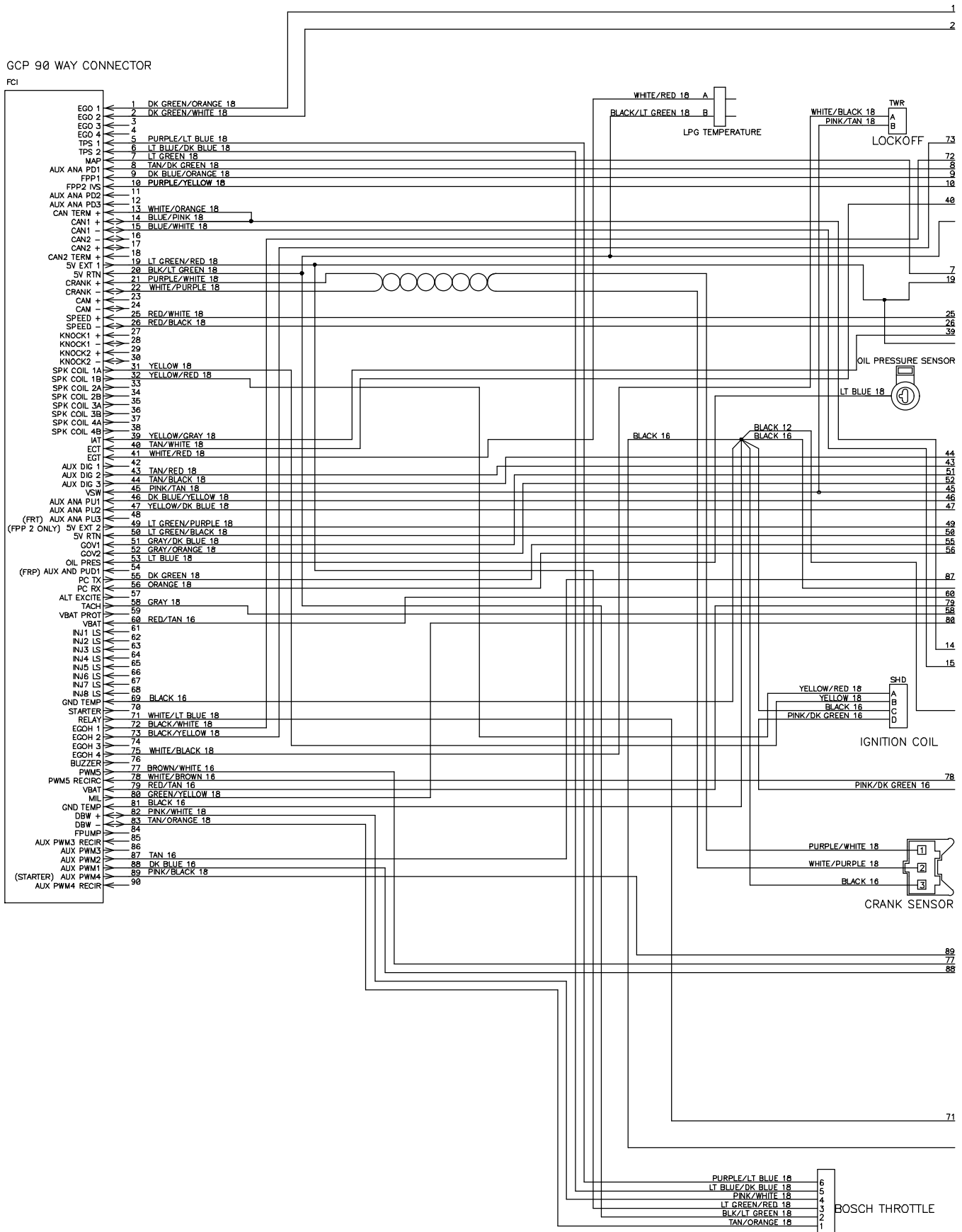
Fig. 93 – GM Electrical Schematic, LPG Engine Harness (0047–0222)
