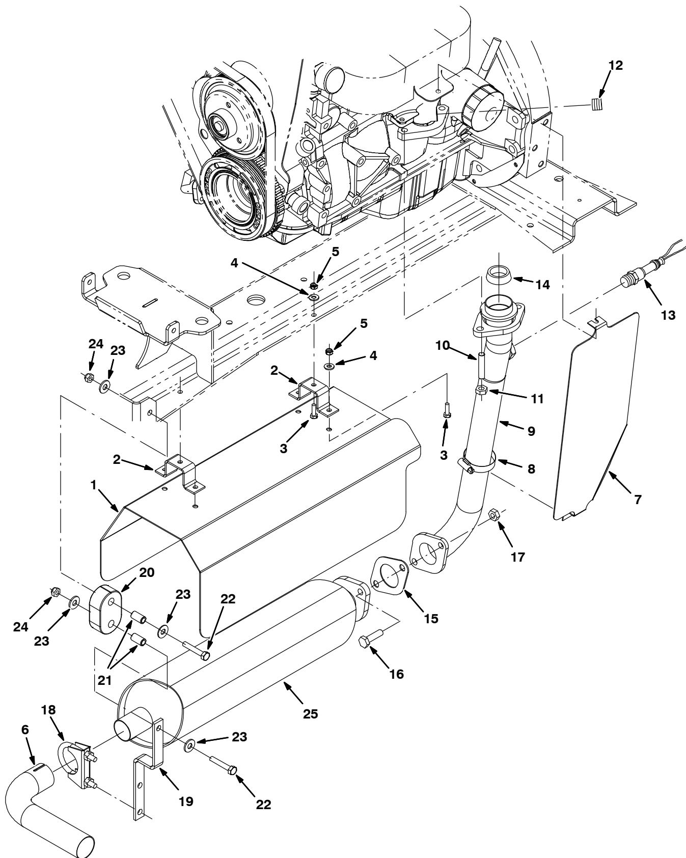
Fig. 25 – GM Engine Muffler Group (0000–0046)
