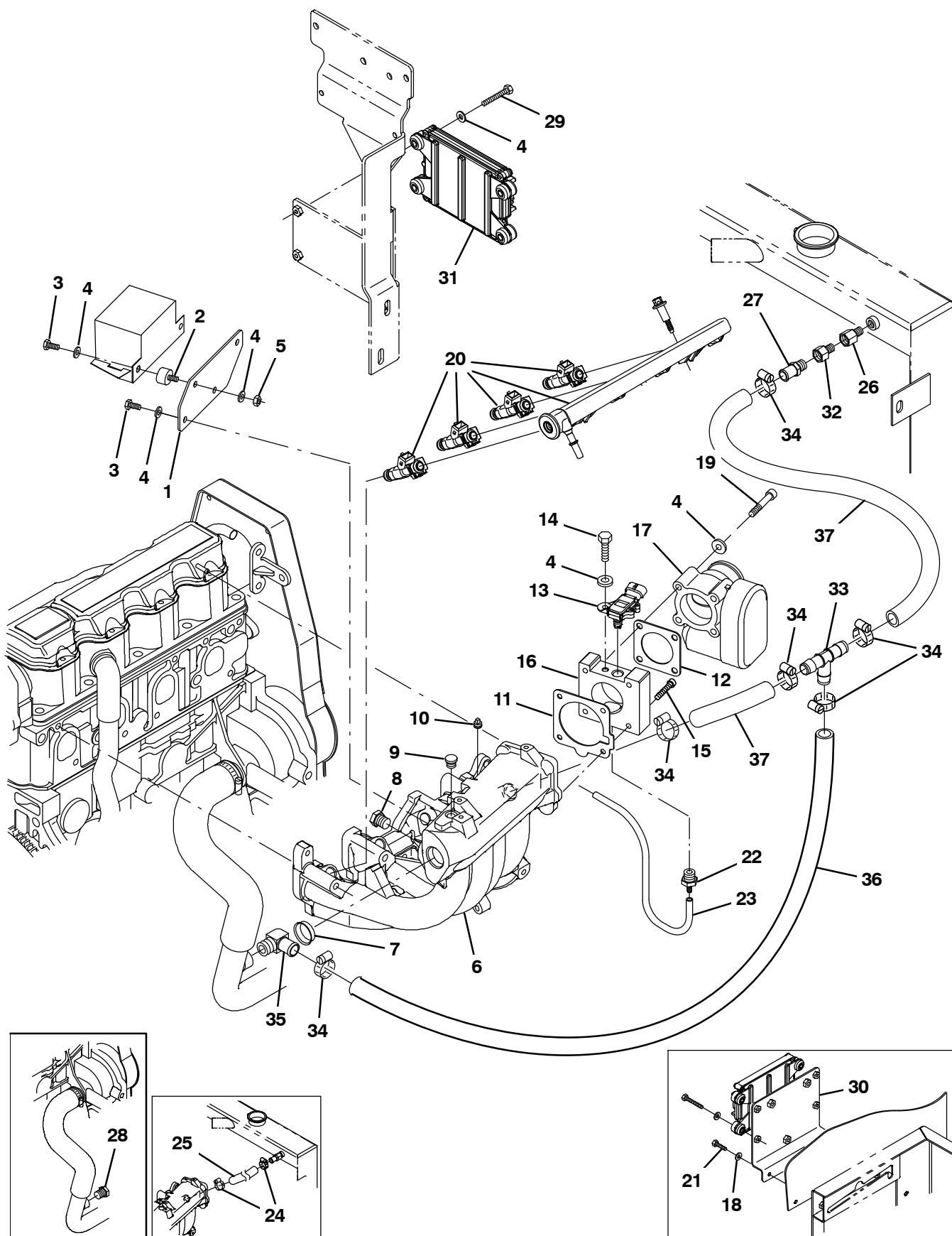
Fig. 14 – GM Engine EFI Group, Gasoline (0223–0499)
