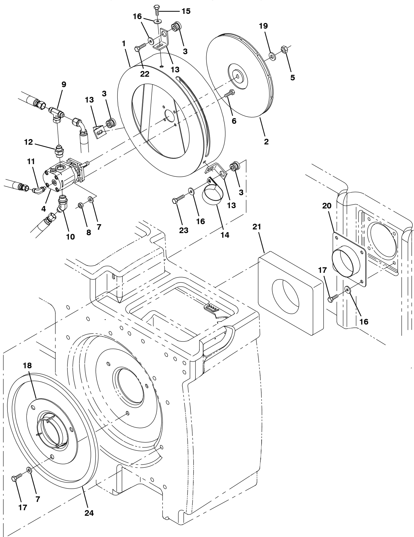
Fig. 71 – Vacuum Fan Group, Scrubbing (0782– )
