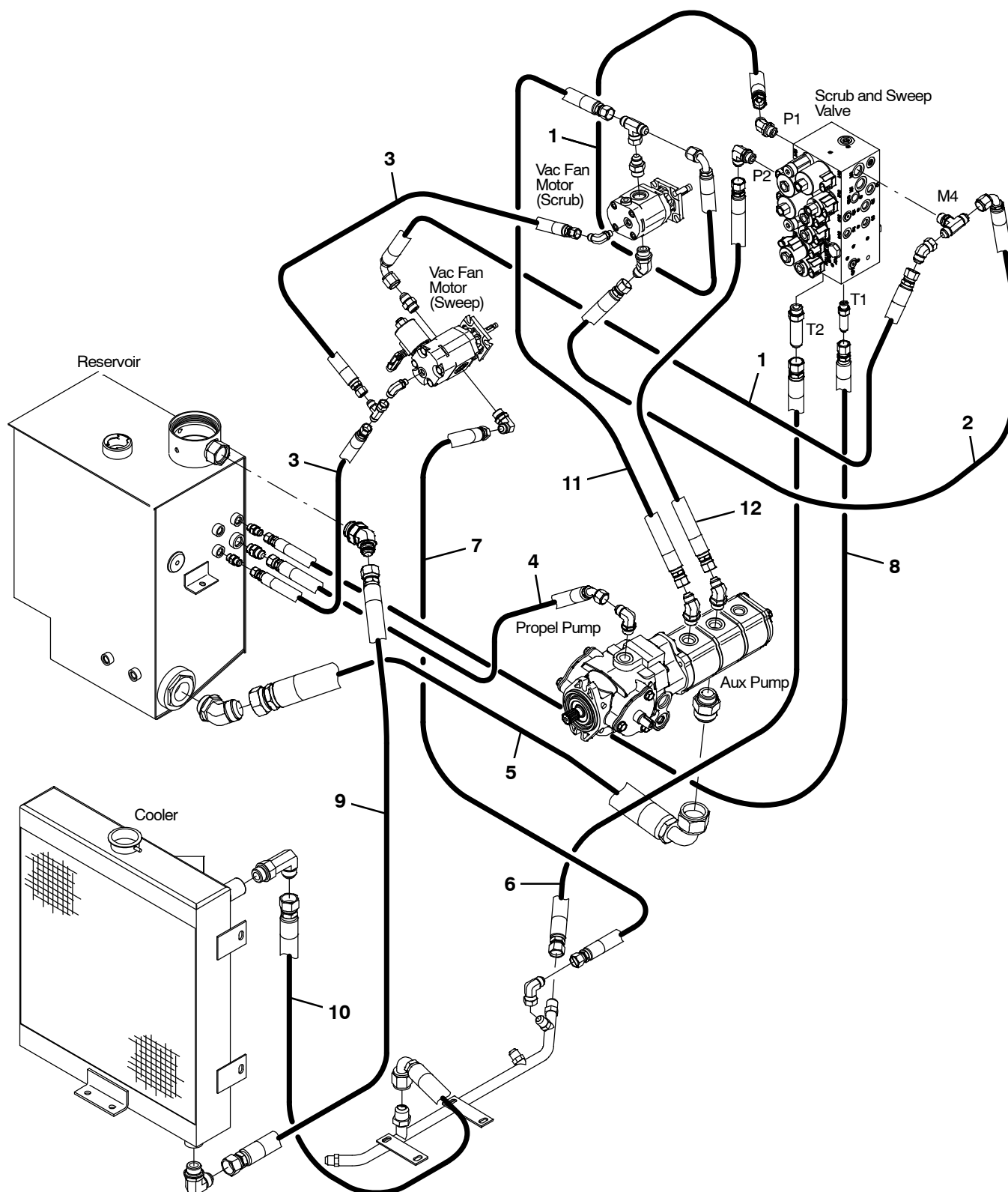
Fig. 78 – Hydraulic Hose Group, Pump and Vacuum Fans (0777– )
