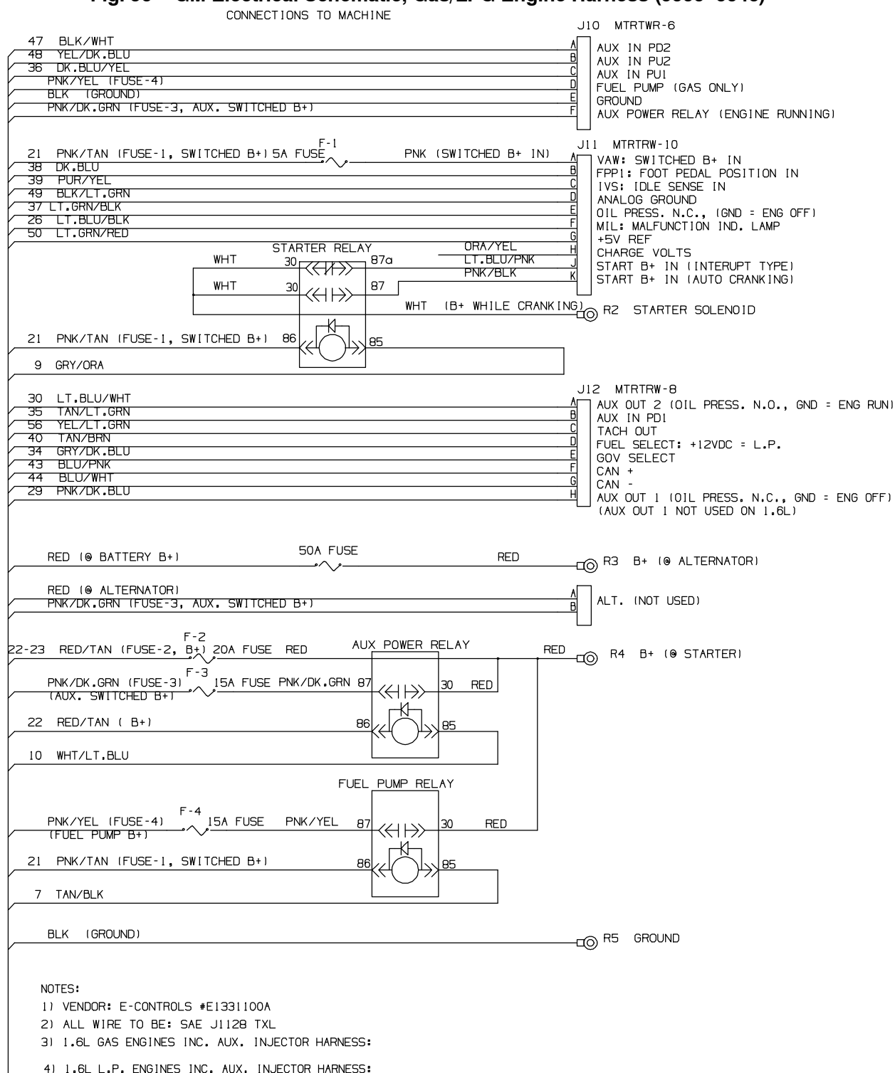
Fig. 90 – GM Electrical Schematic, Gas/LPG Engine Harness (0000–0046)
