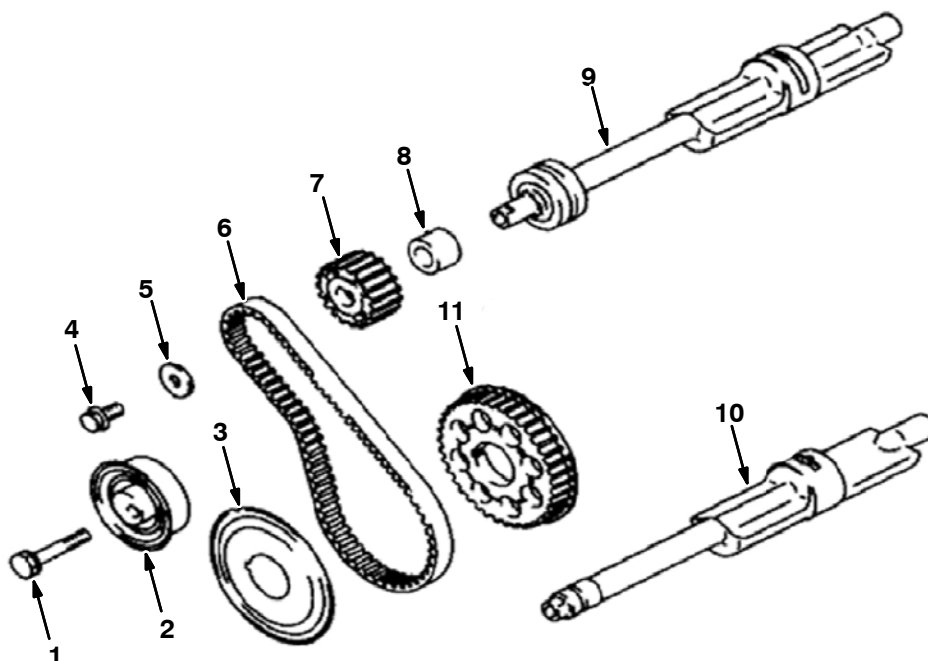
Fig. 7 – Balancer Group
