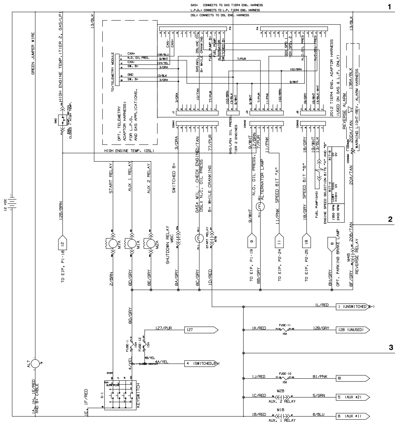
Fig. 95 – Mitsubishi Electrical Schematic (0500– )
