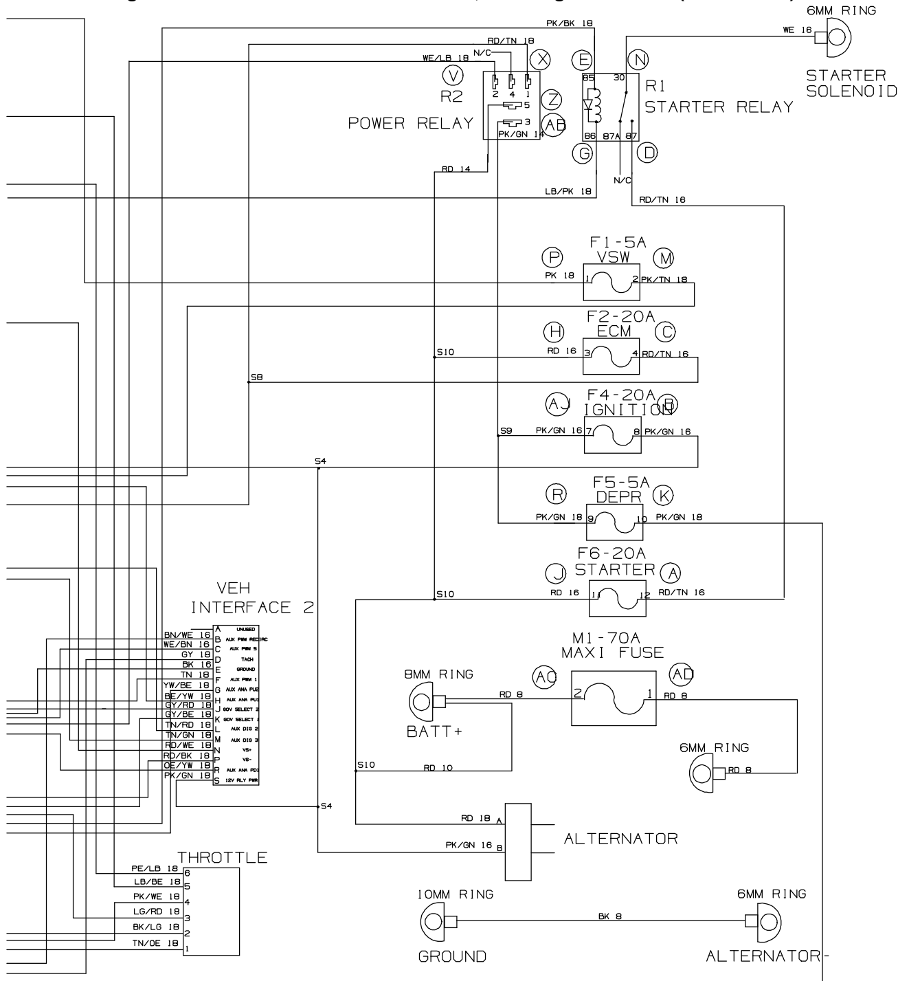
Fig. 97 – Mitsubishi Electrical Schematic, LPG Engine Harness (0500– )
