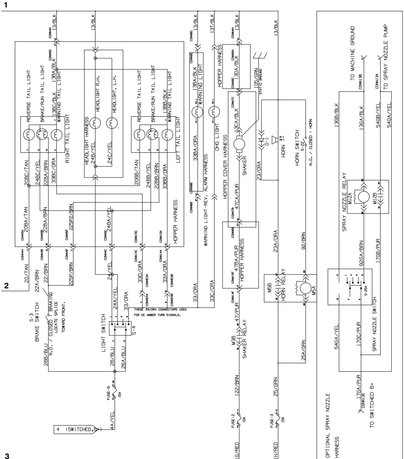
Fig. 87 – GM Electrical Schematic (0047-0145)
