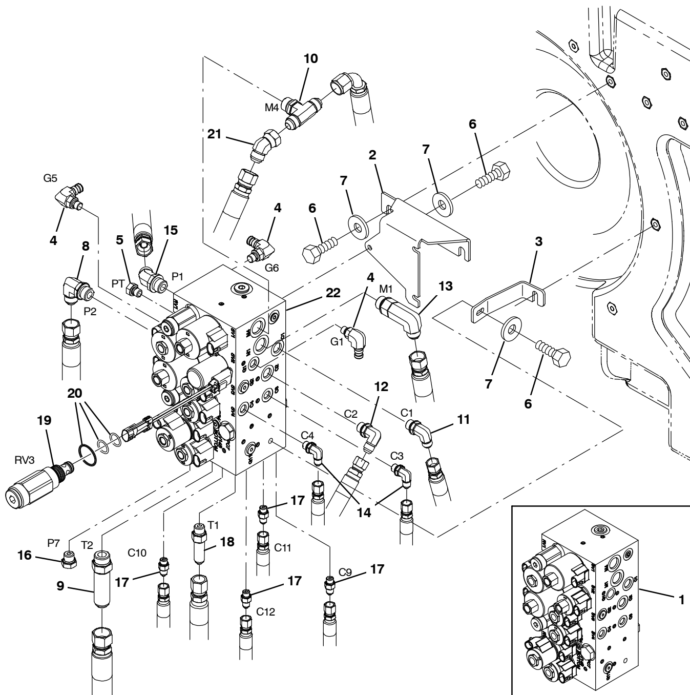
Fig. 85 – Hydraulic Valve Group (0132– )
