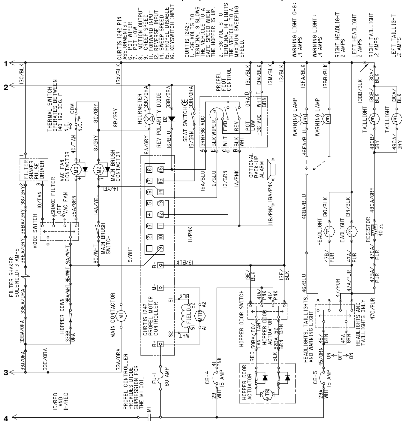
Fig. 30 - Electrical Schematic (6200530 0079 - 1068)
