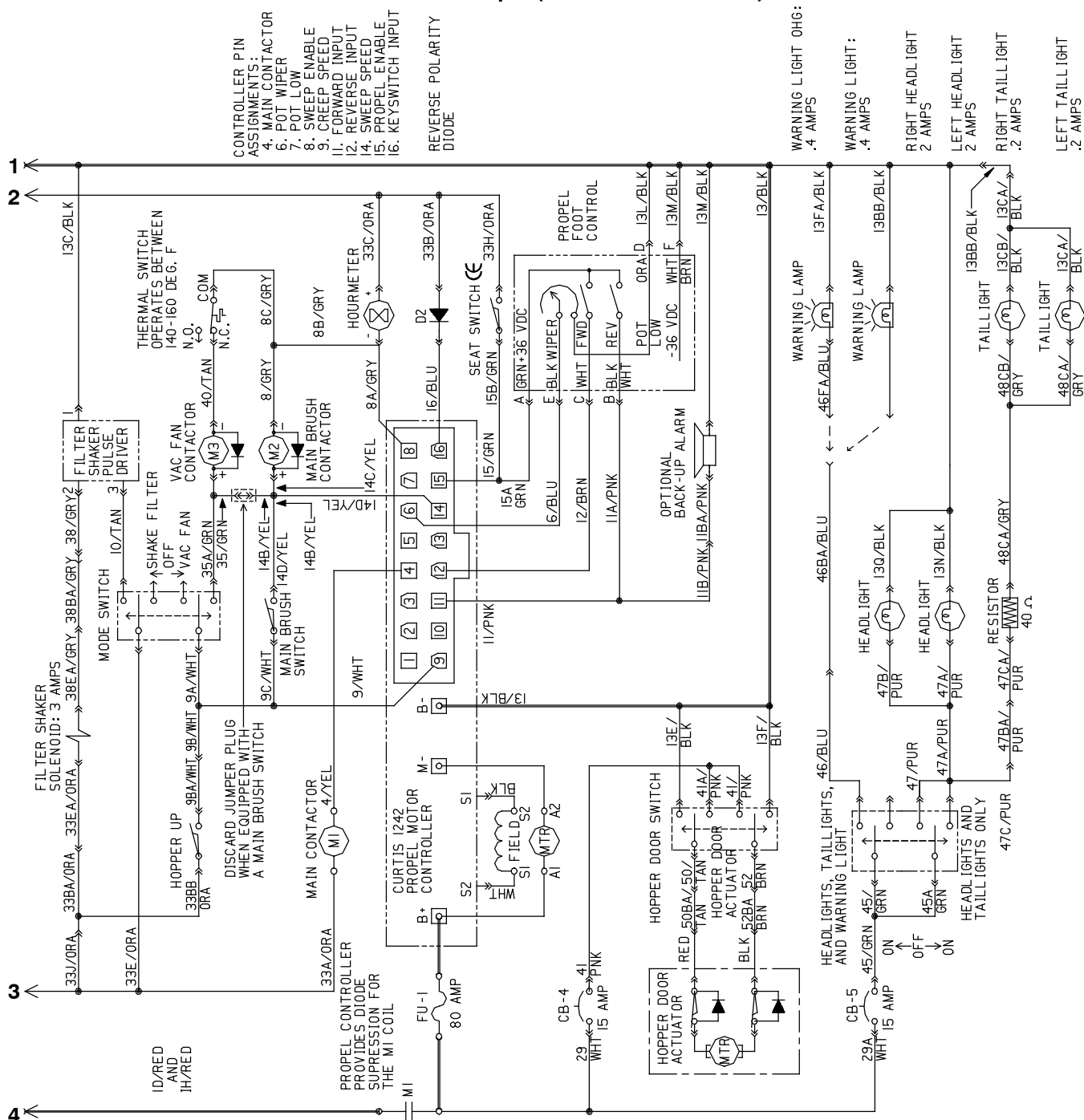
Fig. 29 - Electrical Schematic (6200530 0001 - 0078)
