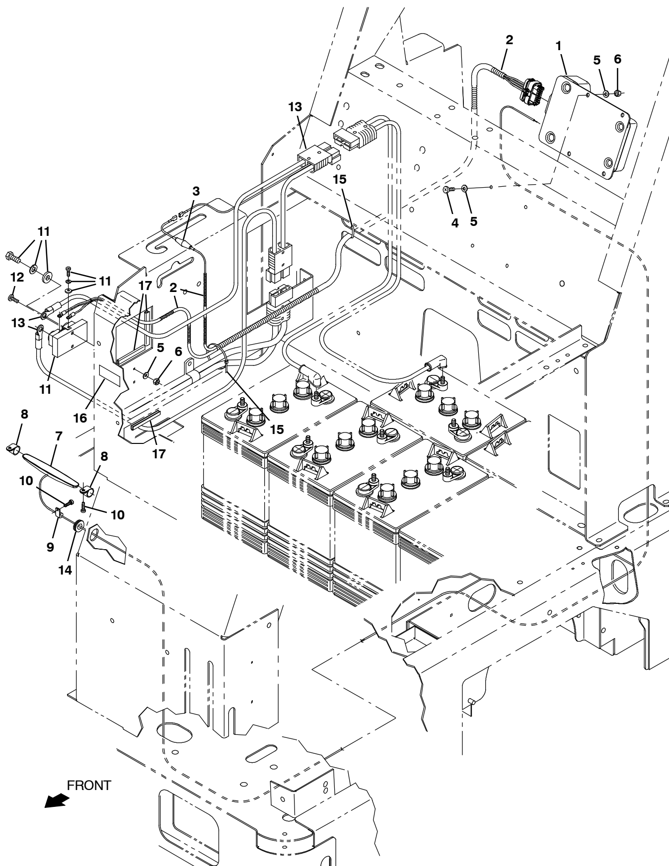
Fig. 26 - Telemetry Group
